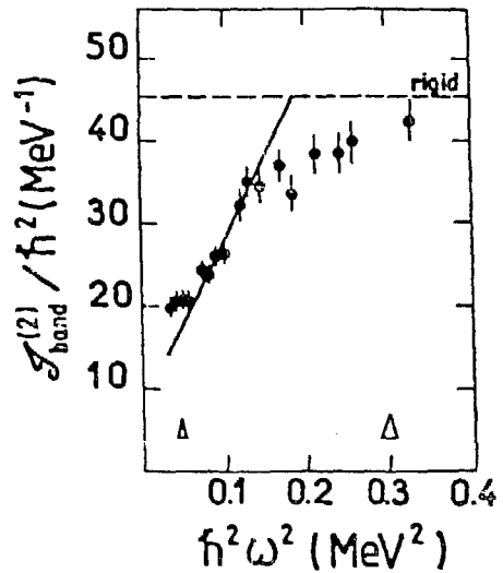
Fig. 4 : The collective moment of inertia of ^{130}\text{Ba} .
