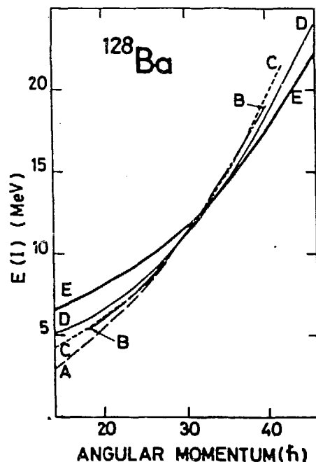
Fig.5 : Calculated bands in ^{128}\text{Ba} .
