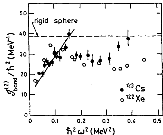
Fig.6 : The collective moment of inertia of ^{123}\text{Cs} .
