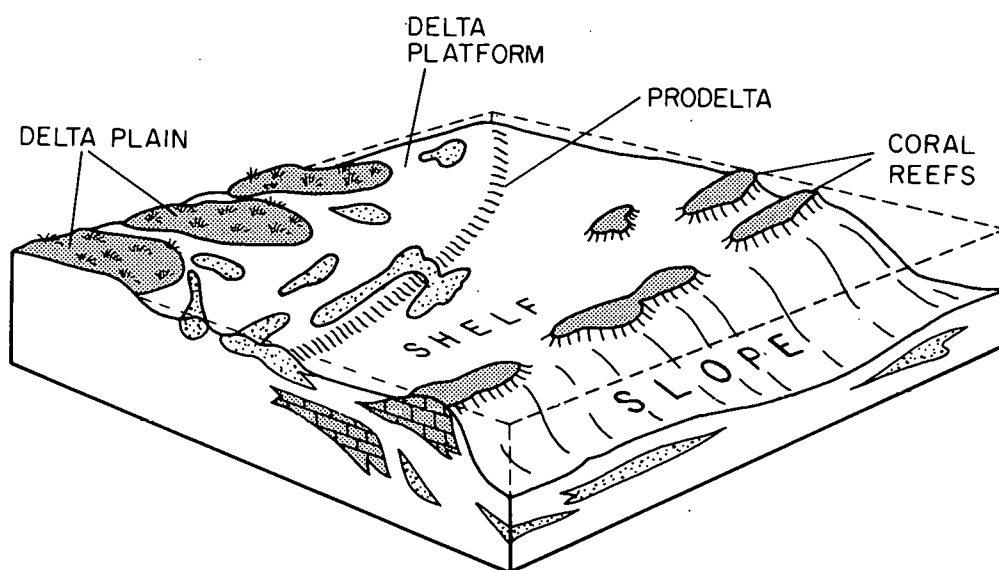
Figure 19. Block diagram of modern Mahakam Delta and shelf. Distribution of facies is analogous to Permian facies systems.
