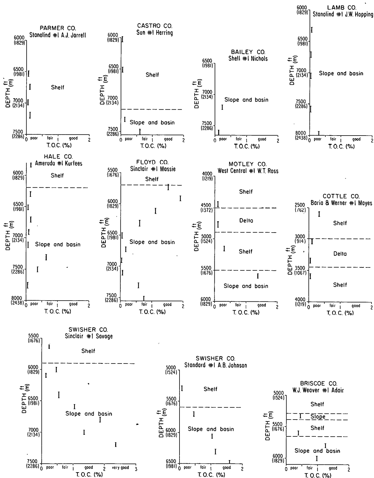
Figure 26. Total organic carbon versus depth for exploratory wells in central and southern Palo Duro Basin. Values are related to depositional systems observed in logs from each well.
