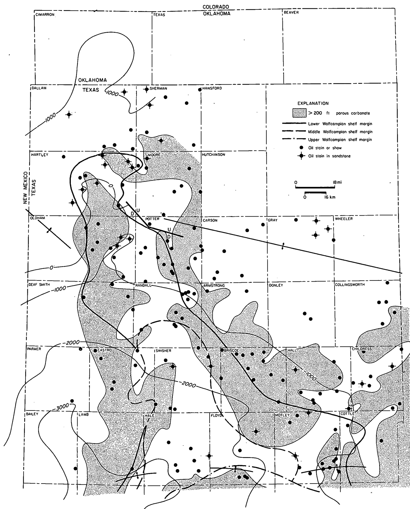
Figure 23. Distribution of oil stains and shows, as reported in sample logs, in relationship to Wolfcamp structure, porous carbonate fairways, and lithology of host rock. Hydrocarbon shows are most common in shelf carbonates and delta sandstones.
