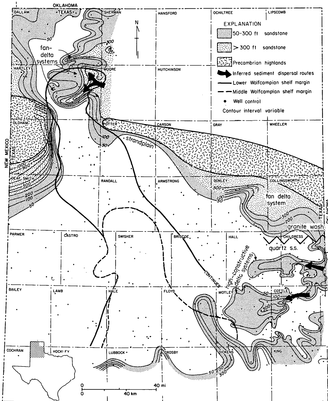
Figure 9. Sandstone isolith map of Lower Permian strata, Palo Duro Basin. Inferred sand dispersal routes highlight delta systems.
