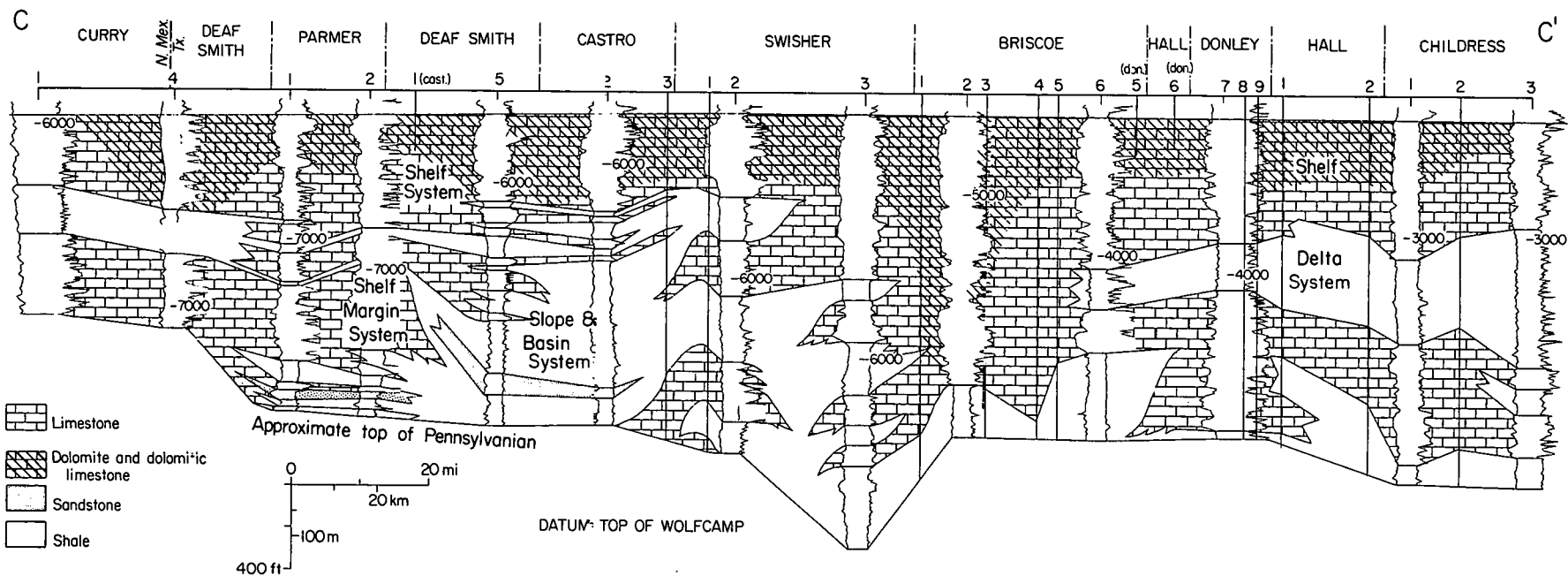
Figure 6. East-west cross section C-C', showing stratigraphic framework and depositional systems, central Palo Duro Basin.
