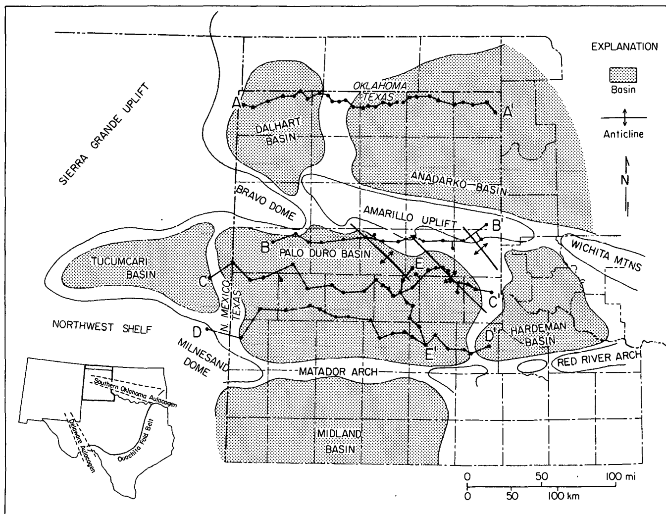
Figure 1. Index map showing major structural features of Texas Panhandle and adjacent areas, and grid of cross sections used to determine regional stratigraphic framework.
