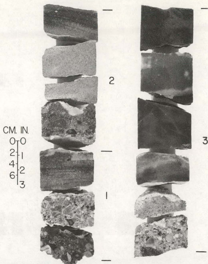
Figure 10. Representative cores from proximal fan-delta environments. (a) Weathered granite or grus directly overlying basement. Hartley County, Standard Bivens no. 12, 5,550 ft (1,690 m). (b) Distributary braided channel-fill sequence composed of three fining-upward sequences numbered 1, 2, and 3. Potter County, Standard Bivens no. 7, 3,606 to 3,618 ft (1,100 to 1,102 m).
