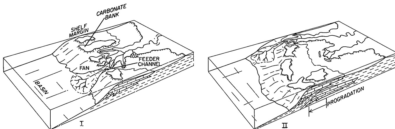
Figure 21. Two-phase model illustrating mechanisms of Lower Permian shelf-margin development assuming continuous subsidence. Phase I: Delta-lobe progradation to shelf margin accompanied by dispersal of fine-grained clastics across shelf margin via inlets between bloherms or banks and deposition of sediment in feeder channels and submarine fan. Phase II: Delta-lobe abandonment or switching and resumption of carbonate productivity over clastic slope wedge. Upbuilding and coalescence of carbonate banks result in net progradation of shelf margin over clastic foundation. Factors that may be considered in alternative models include effects of eustatic sea-level changes, tectonics, and compaction of slope wedge sediments.
