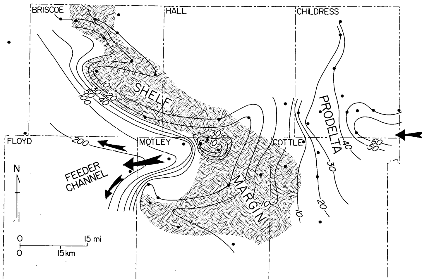
Figure 20. Isopach of shale unit that was traced westward from prodelta, across shelf margin, and into slope environment. Slope or fan-head feeder channel is defined by thick net shale in northwestern Motley County. Shale thins over crest of interpreted shelf margin and thickens toward prodelta environment.
