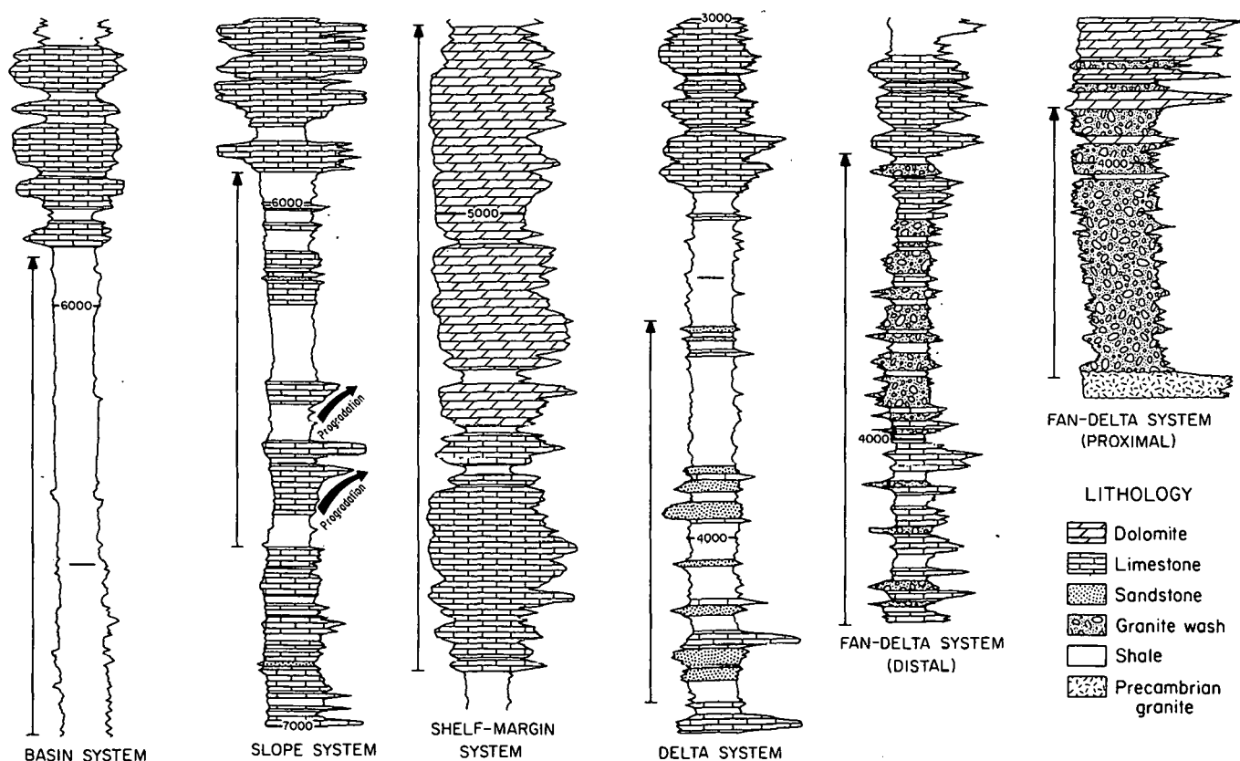
Figure 3. Typical electric log patterns of lithologic facies within sequences that characterize each system. Spontaneous potential and resistivity curves are shown. Vertical scale marked every 500 ft.
