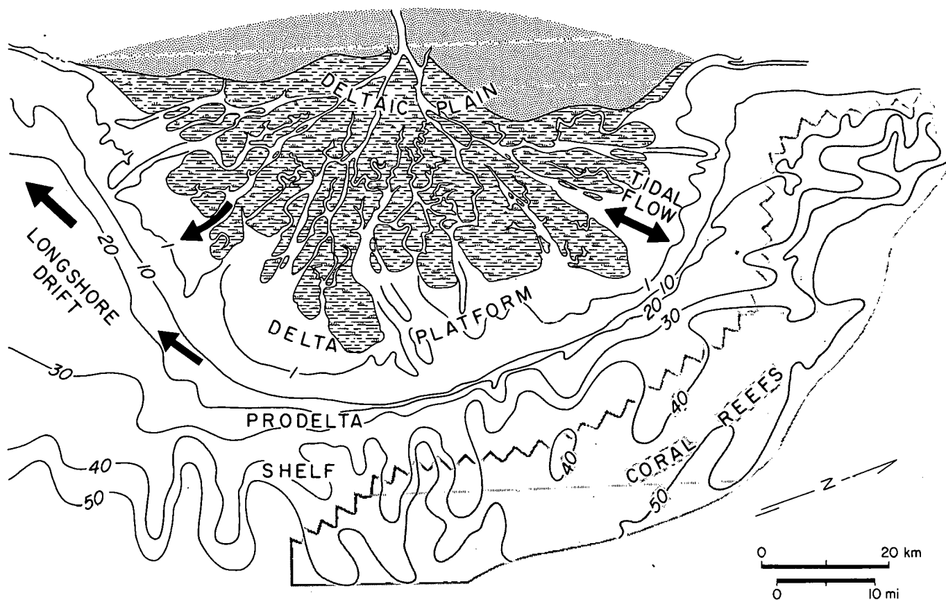
Figure 18. Modern Mahakam Delta of Kalimantan (Borneo) and bathymetry of shelf (contours in fathoms). This locality serves as a modern analog for Permian shelf and shelf-margin carbonates in close association with a high-constructive delta.
