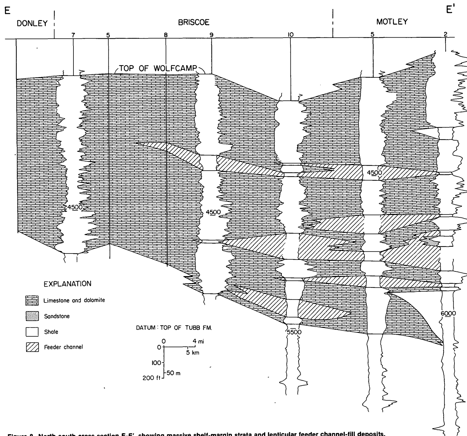
Figure 8. North-south cross section E-E', showing massive shelf-margin strata and lenticular feeder channel-fill deposits.
