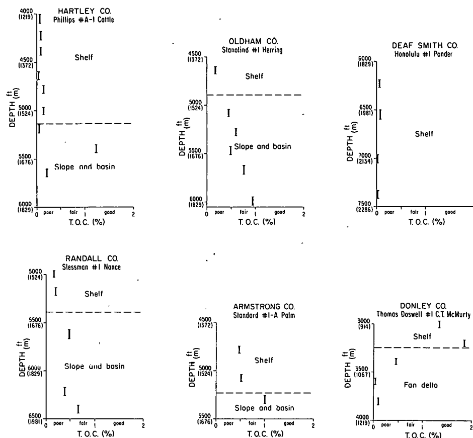
Figure 25. Total organic carbon versus depth for exploratory wells in northern Palo Duro and Dalhart Basins. Values are related to depositional systems observed in logs from each well.
