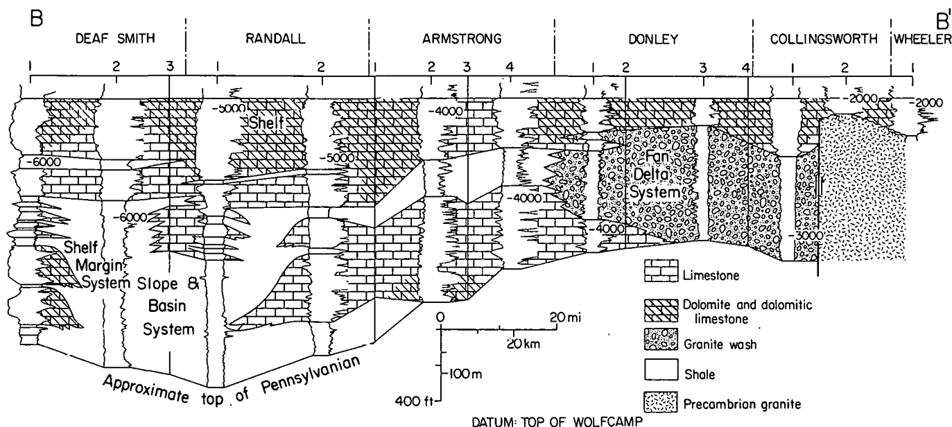
Figure 5. East-west cross section B-B', showing stratigraphic framework and depositional systems, northern Palo Duro Basin. Normal fault in Collingsworth County inferred by abrupt thickening of strata.
