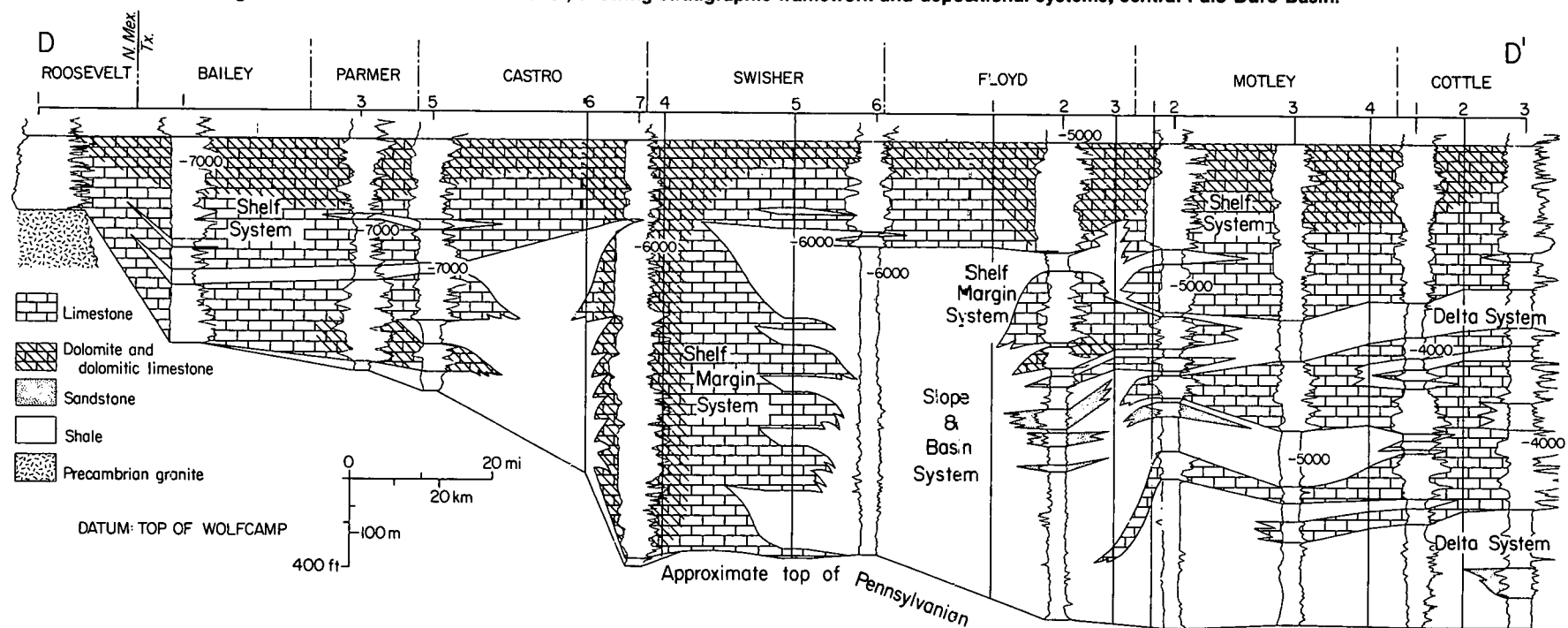
Figure 7. East-west cross section D-D', showing stratigraphic framework and depositional systems, southern Palo Duro Basin. Stacking of shelf margins in western Palo Duro Basin and progradation of shelf margins in eastern Palo Duro Basin are evident.
