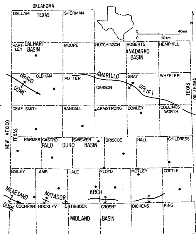
Figure 24. Index map showing locations of exploratory wells from which drill cuttings were analyzed for total organic carbon.
