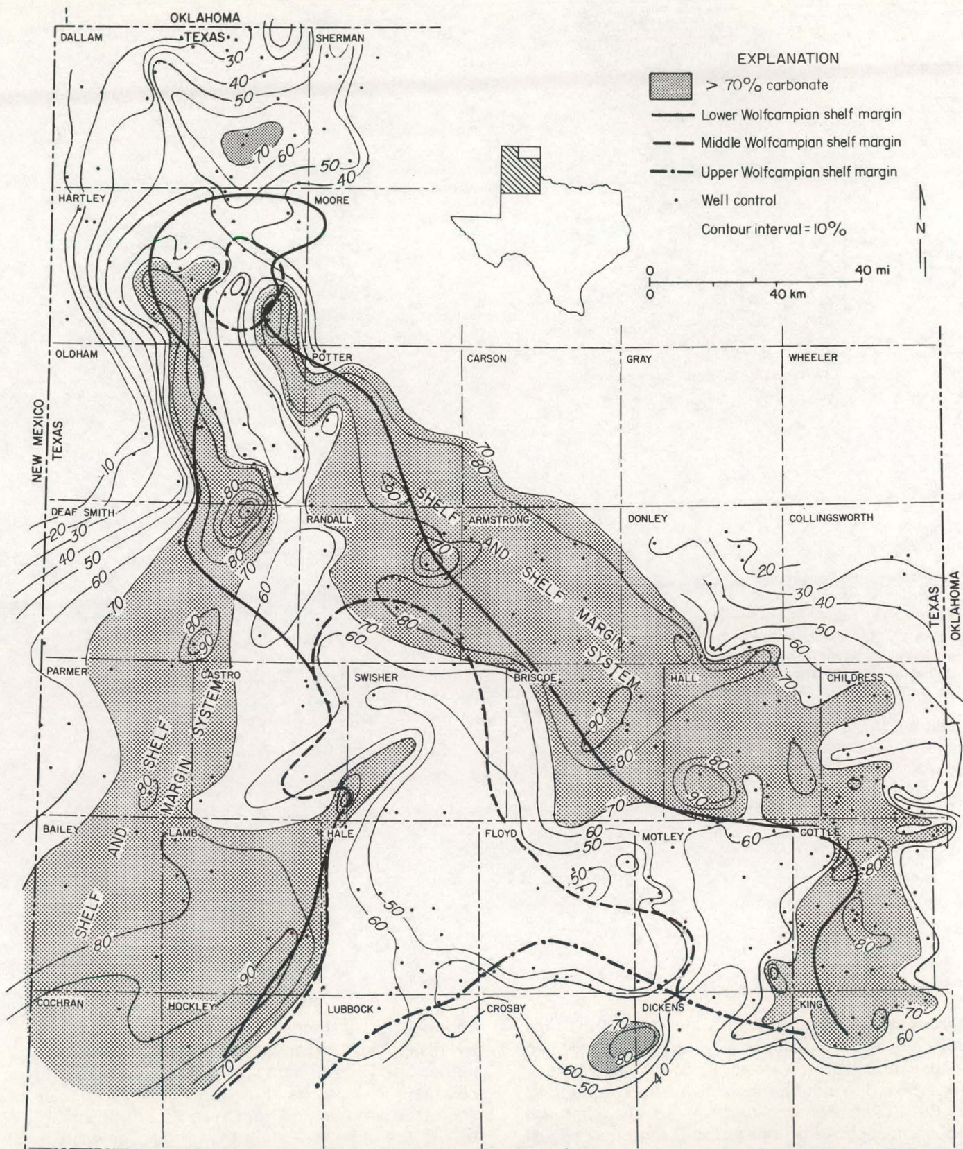
Figure 16. Percent carbonate map of Lower Permian strata in the Palo Duro Basin. Shelf-margin trends correlate with major carbonate occurrence. Lines defining lower, middle, and upper Wolfcampian shelf-margin positions illustrate shelf-margin progradation through time.
