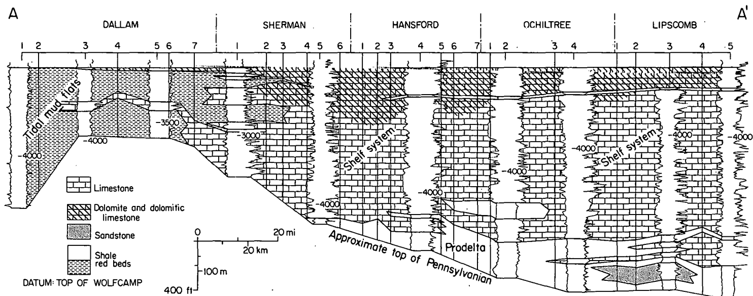
Figure 4. East-west cross section A-A', showing stratigraphic framework and depositional systems across Dalhart and Anadarko Basins. Boundary between Pennsylvanian and Permian systems in all cross sections (figs. 5, 6, 7, and 8) is approximate and based upon sample logs and regional correlations.
