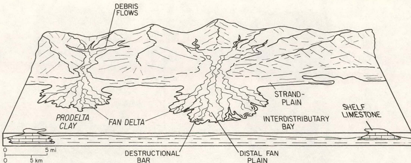
Figure 13. Schematic block diagram showing major subenvironments of a fan-delta system.
