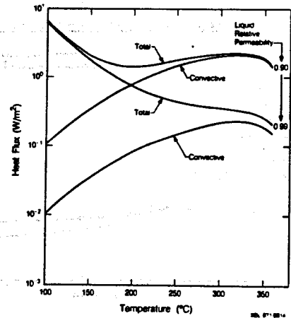
Figure 3. Heat flux for balanced steam-water counterflow in liquid-dominated conditions (permeability 10^{-18} \text{ m}^2 ; formation heat conductivity 2.5 \text{ W/m} \cdot ^\circ\text{C} ).
