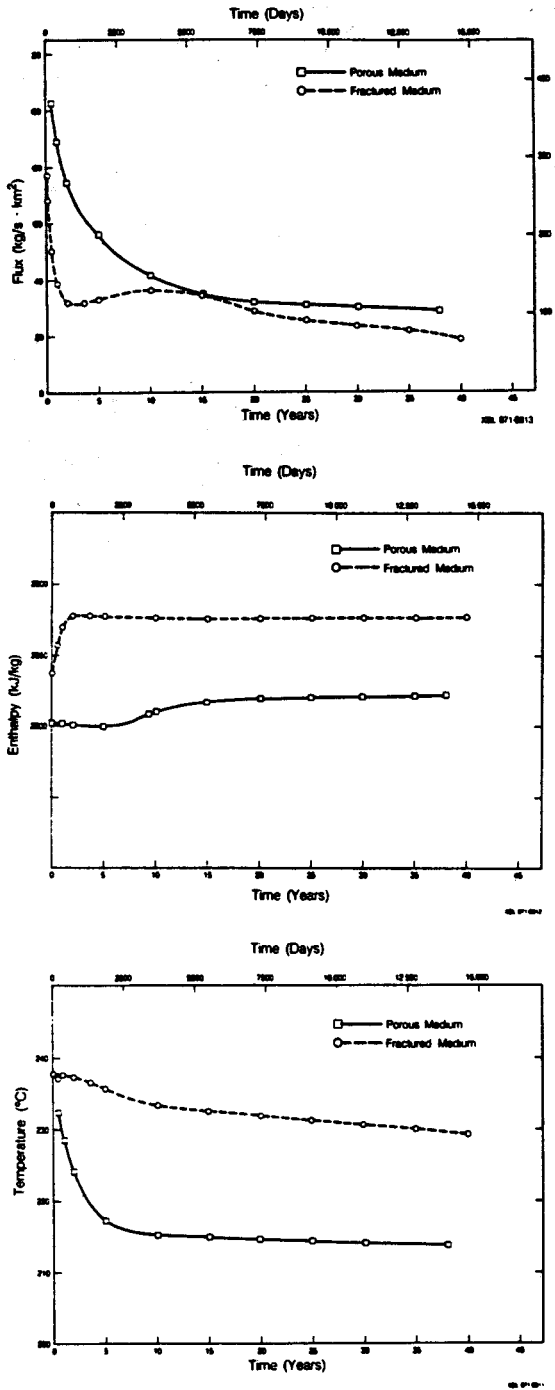
Figure 6. Simulated results for flow rates, enthalpies, and temperatures of produced fluids. Parameters are defined in Tables 1 and 2.
