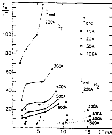
Fig. 3: Ratio I_e/I^- vs I^- for several values of the current in the coil producing the conical dipole field, for hydrogen (dotted) and deuterium (solid lines).
