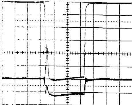
Fig. 6: H^- current (upper trace, 5 mA/div.) and total extractor supply load (lower trace, 50 mA/div.). Time Scale = 0.5 ms/div. Taken with cesium in the source.
