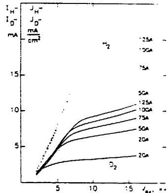
Fig. 1: Negative ion field vs the extraction voltage V ext with arc current as parameter, for hydrogen (dotted) and deuterium (solid lines).
