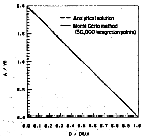
Figure 6. (b) 50,000 integration points.
