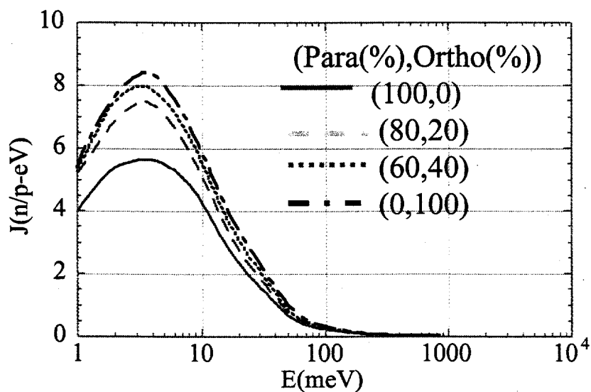
Fig. 6. Neutron spectra from cryogenic \text{H}_2 moderator for varying ortho/para admixtures.
