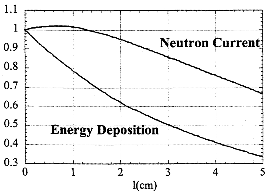
Fig. 3. Thermal neutron current and energy deposition vs the premoderator thickness ( l ).
