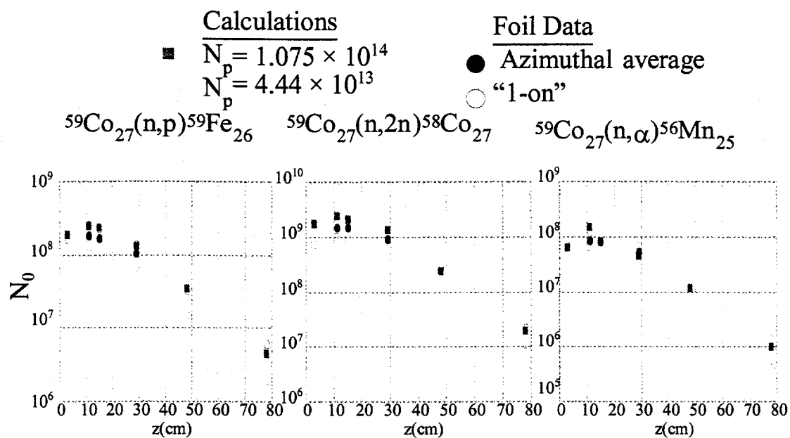
Fig. 5. Comparison between calculational and experimental results show good spatial agreement.
