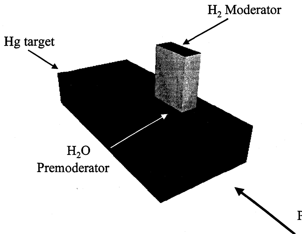
Fig. 2. Model geometry used for the premoderator study.
