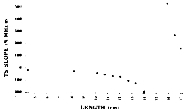
Fig. 4 Tilt sensitivity slope versus post-coupler length for the 1.84 m long, 40 cell DTL equipped with double stems and 19 post couplers. There is no stabilization point below 17 cm
