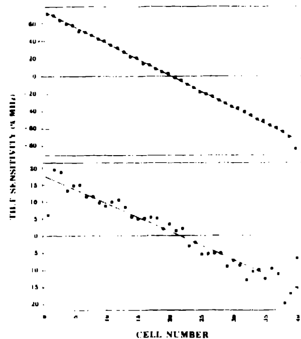
Fig. 1. Tilt sensitivity without post couplers for the 1.84-m long, 40-cell DTL. The upper plot corresponds to single stems and has a slope of -80\%/MHz/m . The lower plot corresponds to double stems 180° apart, with a slope of -18\%/MHz/m .
