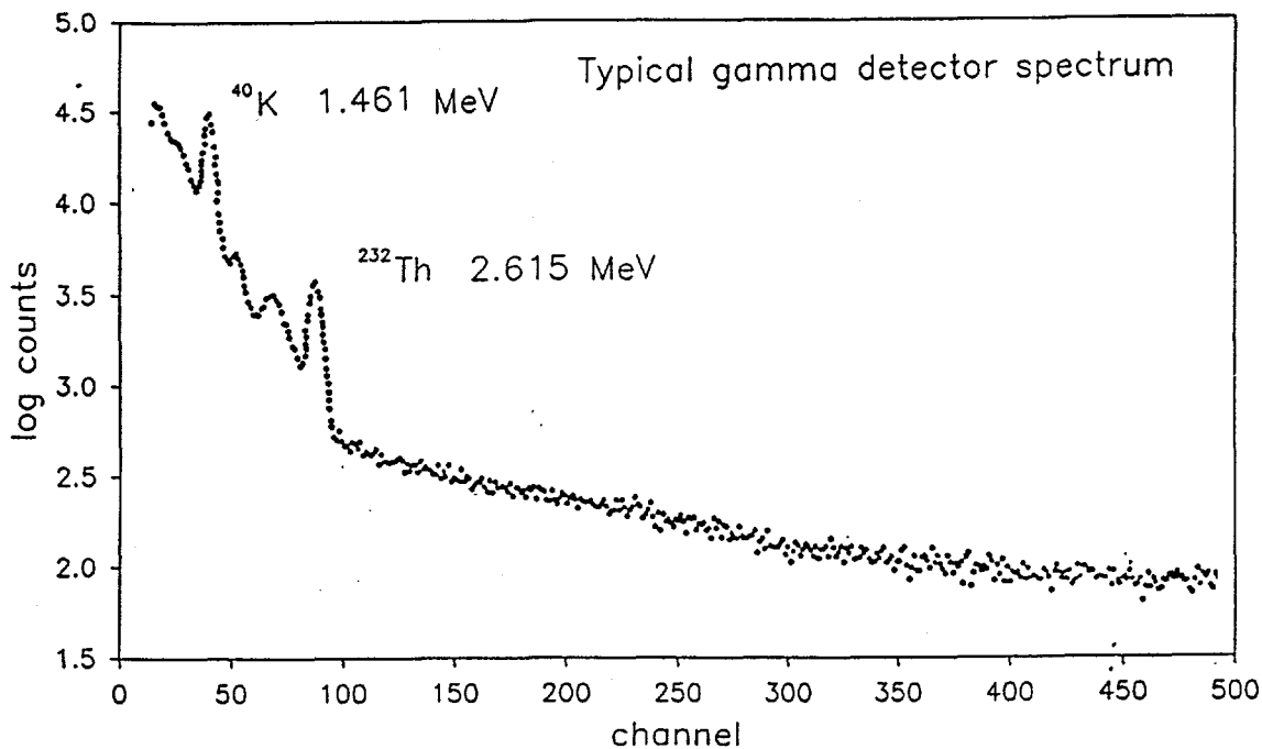
Figure 1. Unattenuated energy spectrum from the reference gamma detector, CSSL, winter 1996.
