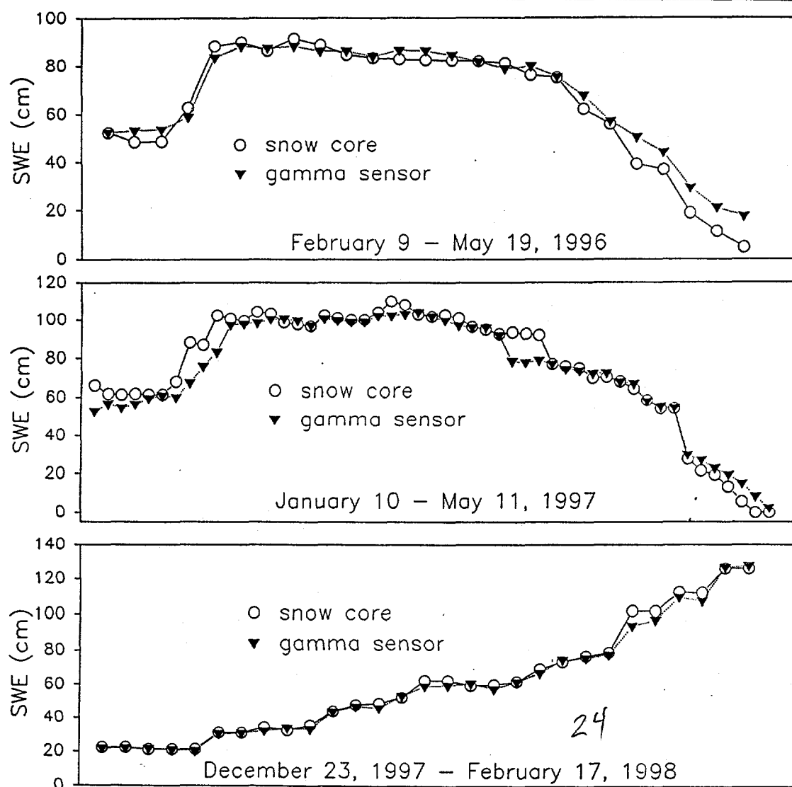
Figure 2. Coincident SWE measurements from the gamma detectors and hand measured snow cores, CSSL.
