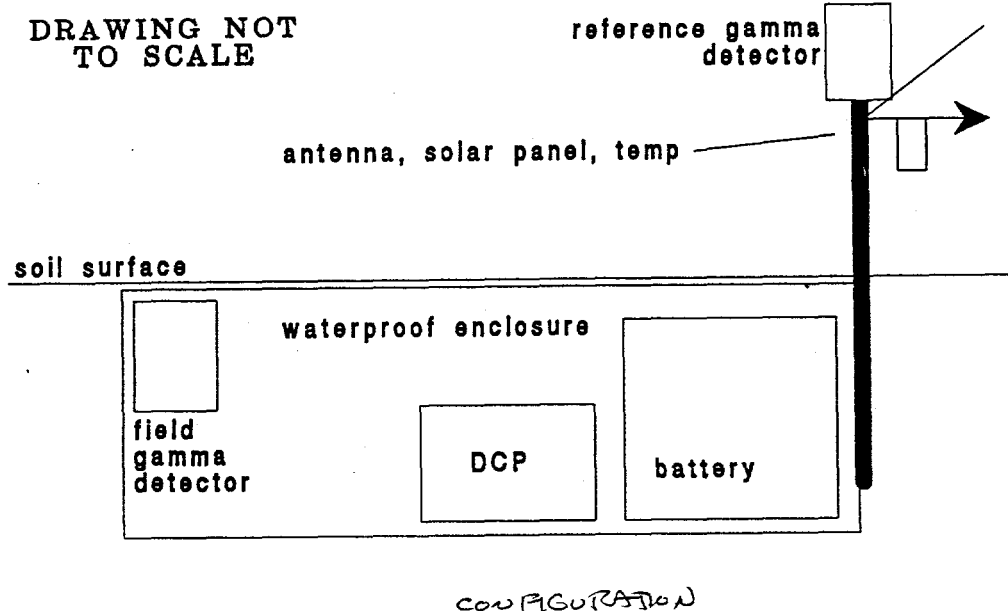
Opt. Figure 4. Generalized schematic of a remote site installation including gamma reference and field detectors.
