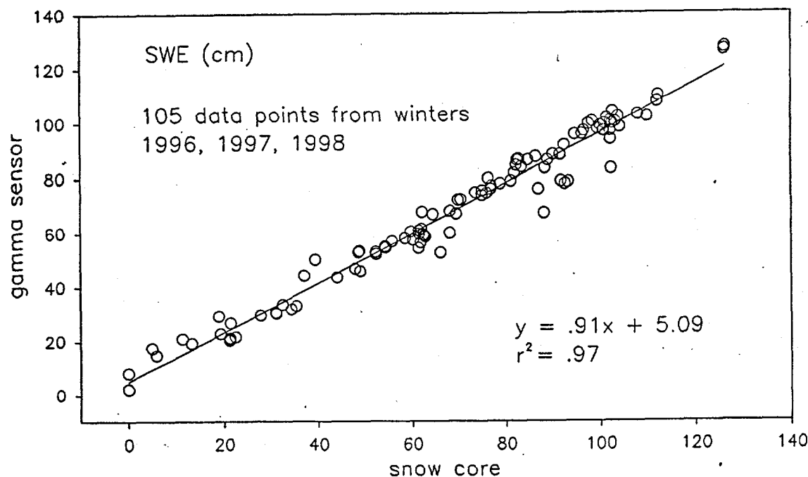
Figure 5. Snow core and gamma detector SWE for winter 1996, 1997, and through February 24, 1998, at the CSSL.
