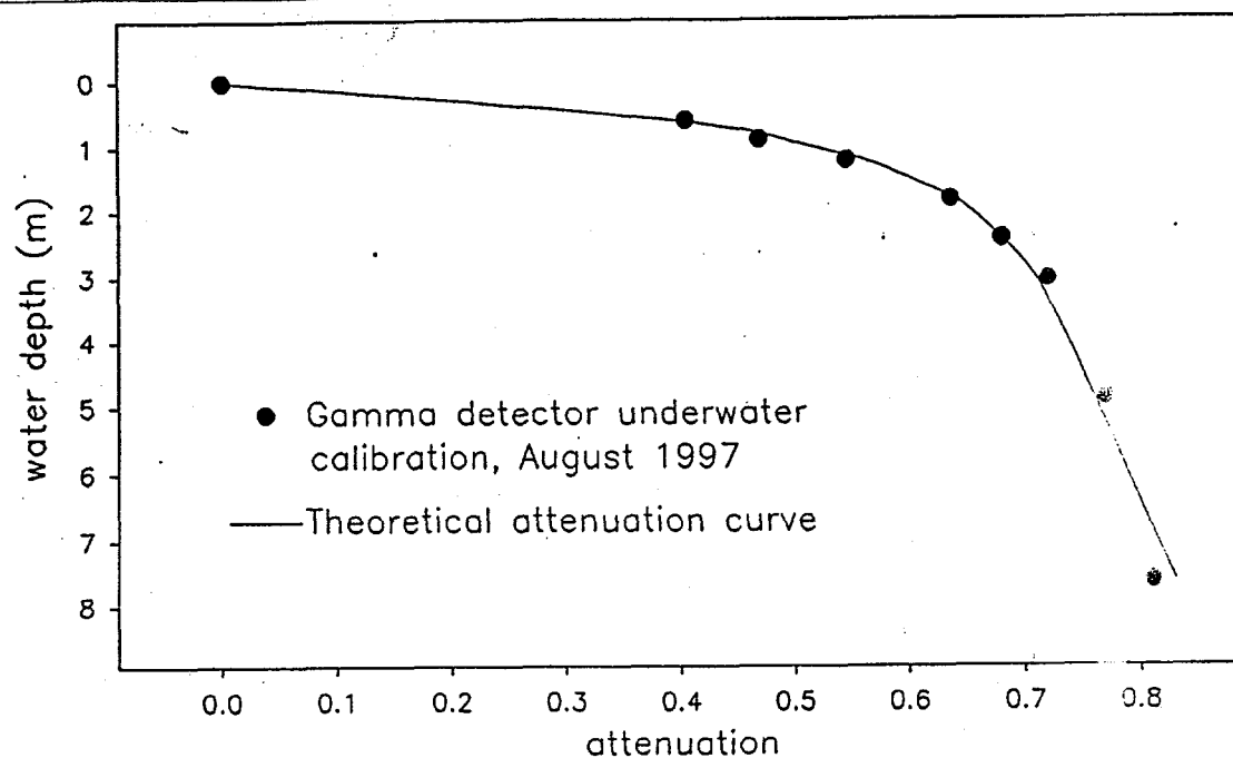
Figure 3. Gamma detector underwater calibration data, San Vicente Reservoir.
