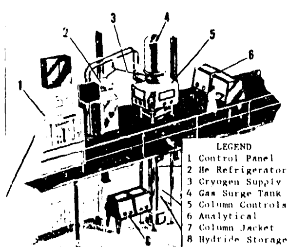
Fig. 7. TSTA Isotope Separation System (ISS).
