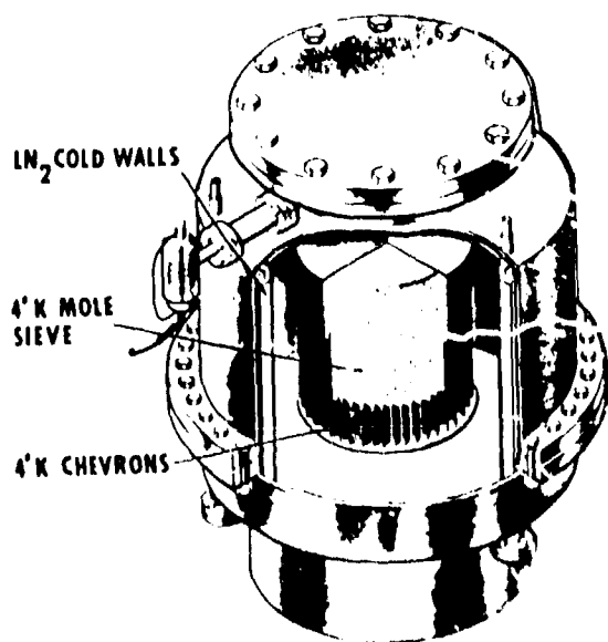
Fig. 5. TSTA Prototype compound cryopump.
