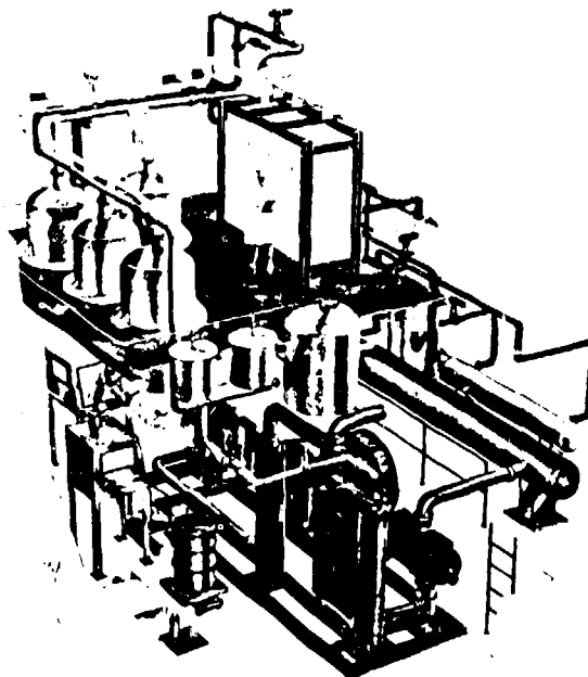
Fig. 3. TSTA Emergency Tritium Cleanup (ETC).
