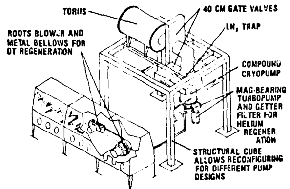
Fig. 6. TSTA plasma chamber vacuum system (VAC).
