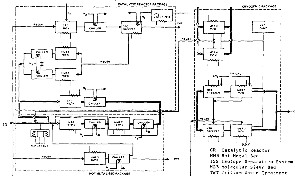
Fig. 8. TSTA Fuel Clean-Up Module (Schematic).
