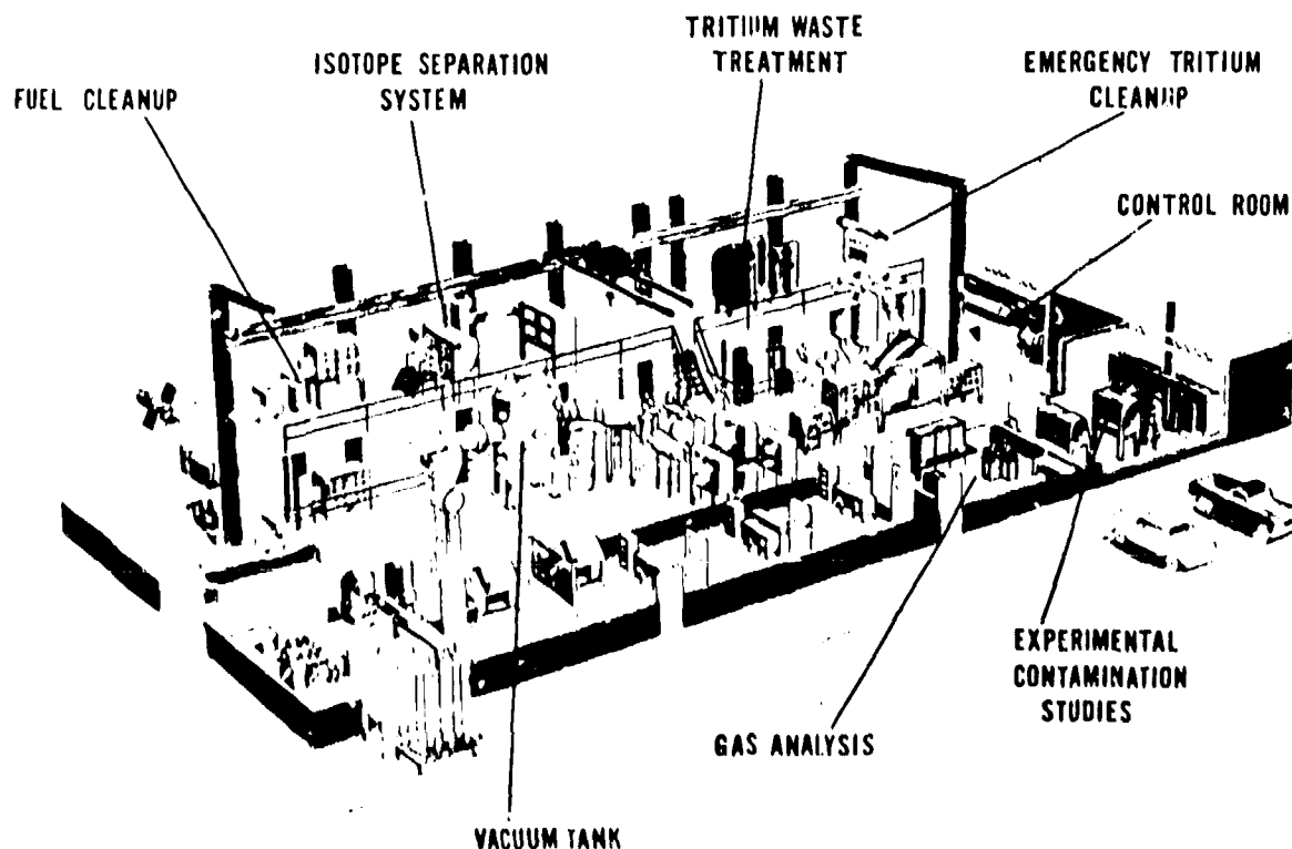
Fig. 1. Physical layout of the Tritium Systems Test Assembly.
