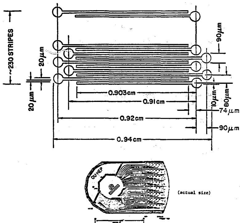
Figure 1. Layout of stripes and PC mounting board for 40 micron prototype.
