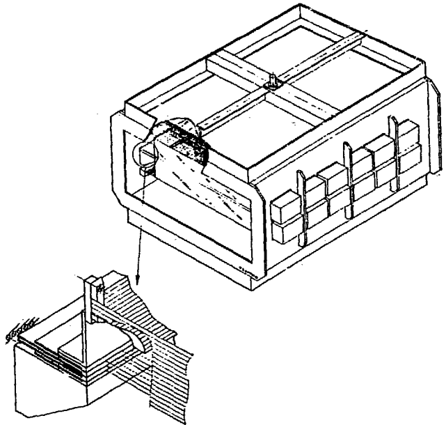
Figure 1. The chamber has a size of 1 \times 0.8 \times 0.4 m with \pm 10 cm of drift distance. Field shaping foils provide excellent drift field homogeneity.
