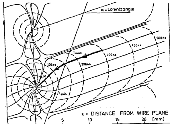
Fig. 10 Electrical field lines and isochronous lines for the JADE chamber.
