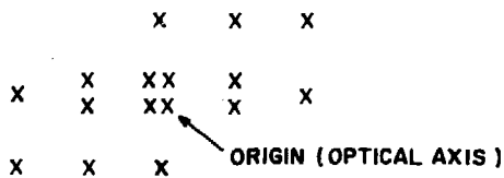
Fig. 2c DISTRIBUTION OF LIGHT INTENSITY IN THE DETECTOR PLANE WHEN THE INPUT PLANE IS ILLUMINATED WITH THE DESIRED BIT PATTERN. THE NUMBER OF 'X's IS PROPORTIONAL TO THE LIGHT INTENSITY AT EACH POINT.
