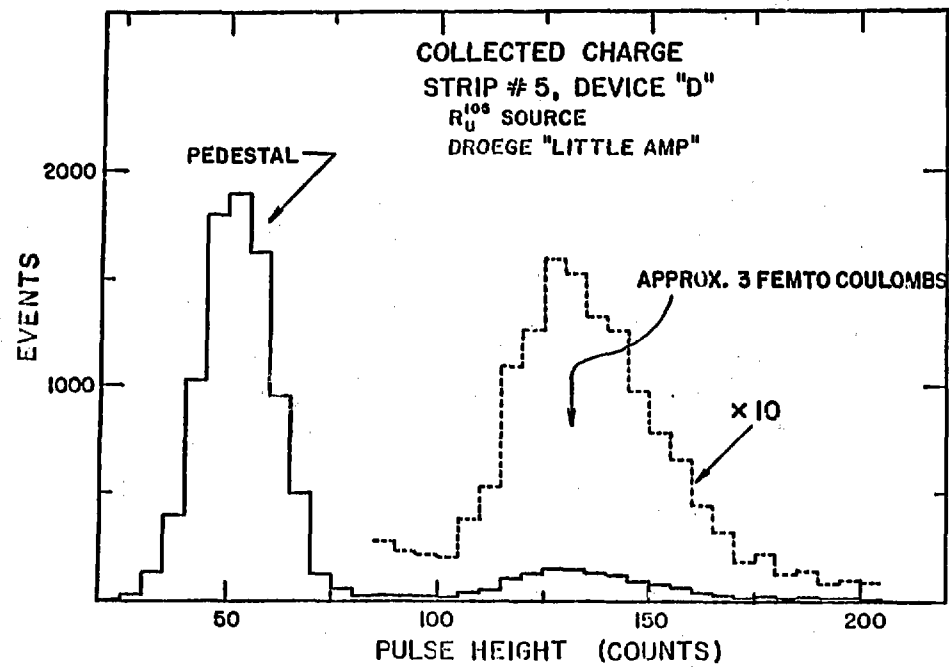
Figure 2. Pulse height spectrum for one mu prototype.
