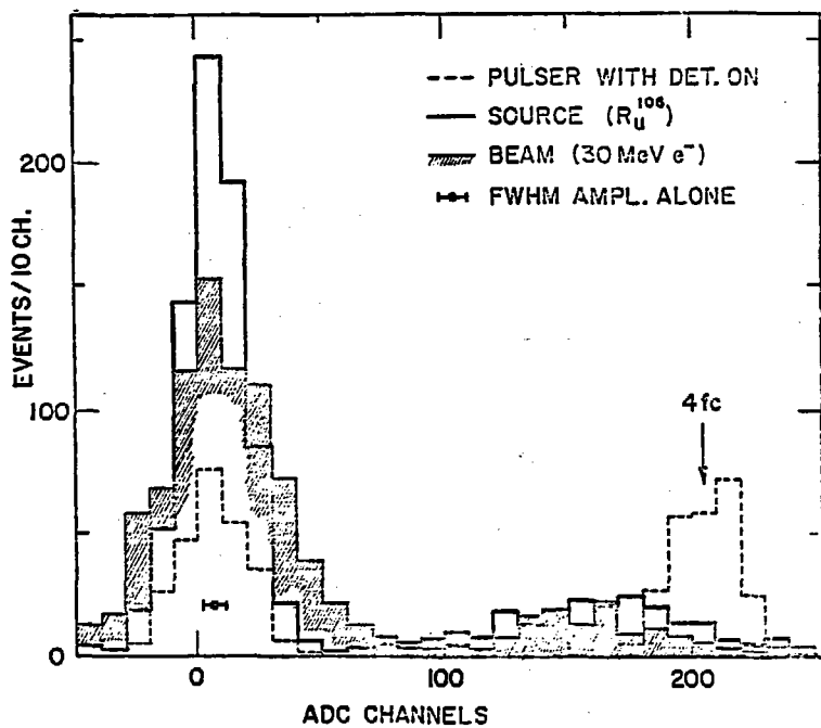
Figure 1. Pulse height spectrum for one mm prototype.
