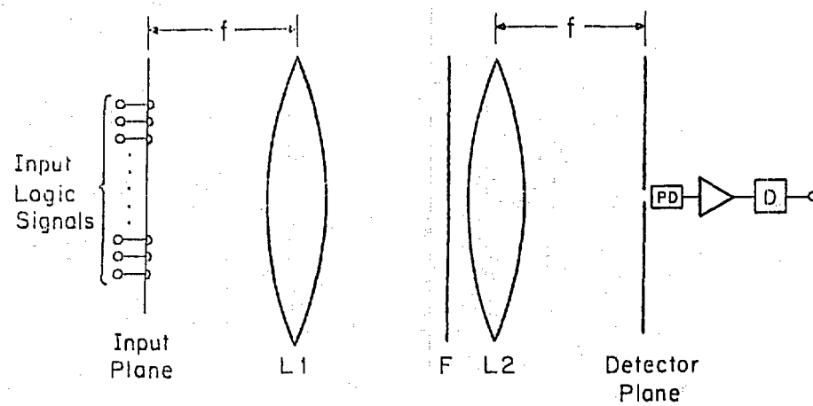
Fig. 1 Optical Processor with a Single Filter F
