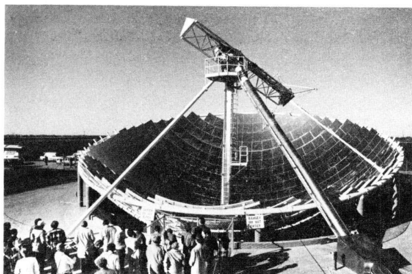
Crosbyton Solar Power Project Using Hemispherical Bowl
