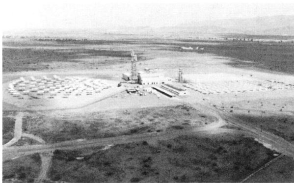
Field of Heliostats and Parabolic Troughs at Small Solar Power System Project in Almeria, Spain
