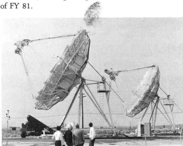
Parabolic Dishes Under Test at Parabolic Dish Test Site
