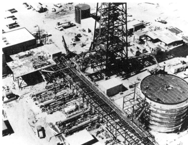
Aerial View of Storage, Piping and Control Room at 10-MWe Solar Central Receiver Pilot Plant
