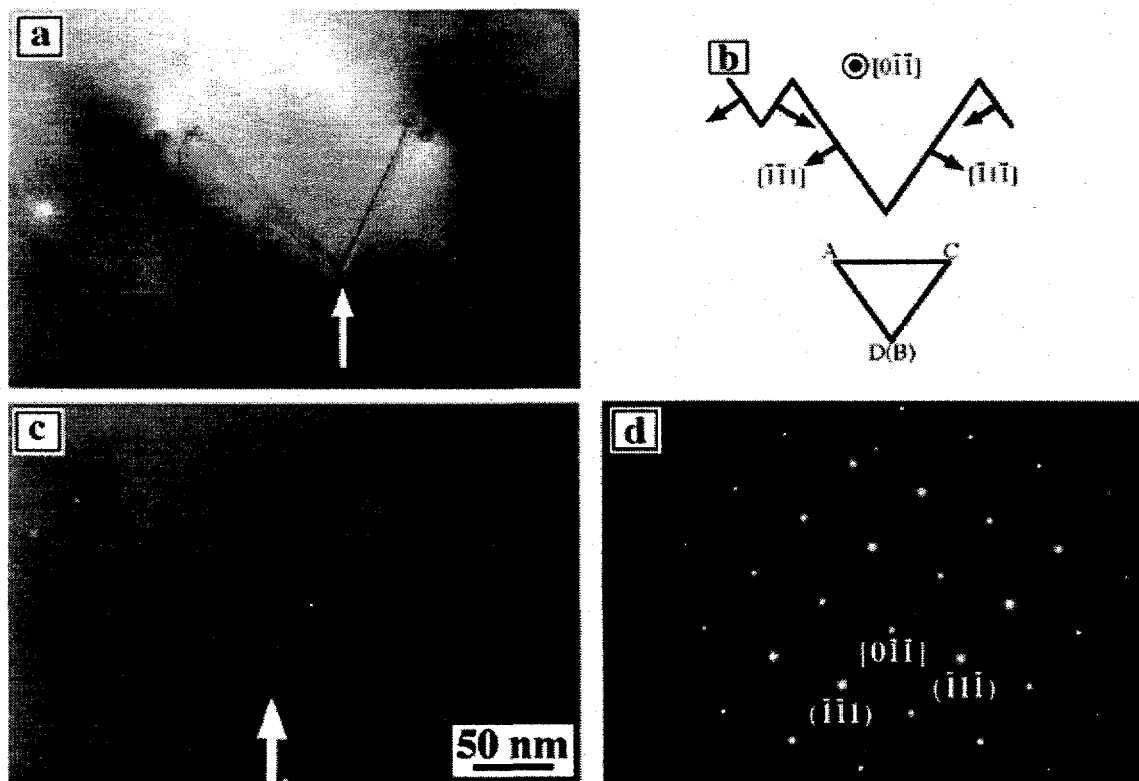
Figure 4. BF TEM of the same defect as in 3(a) viewed nearly edge on. (b) Schematic of (a). (c) BF TEM image taken on [0\bar{1}1] showing no residual contrast from the dislocations. The arrows in (a) and (c) mark the same part of the defect. (d) SAD pattern on [0\bar{1}1] .
