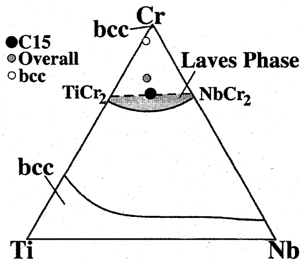
Figure 1. Nb-Cr-Ti phase diagram (950°C isothermal section) (8).
