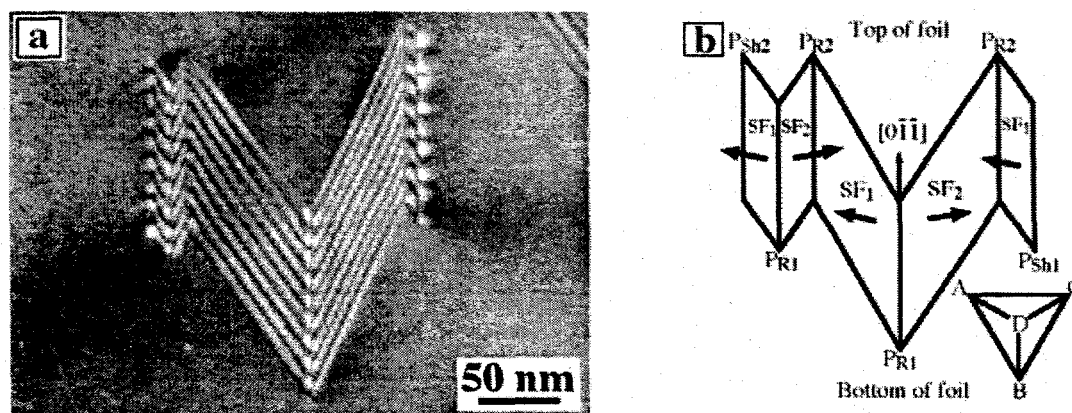
Figure 3. (a) 'WB'DF TEM image of a multiply-faulted dipole. (b) Schematic of (a). \text{P}_{\text{Sh}1} and \text{P}_{\text{Sh}2} are Shockley partials, \text{P}_{\text{R}1} and \text{P}_{\text{R}2} are stair-rod dislocations and \text{SF}_1 and \text{SF}_2 are stacking faults. Inset is the Thompson tetrahedron.
