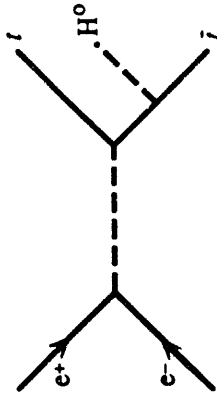
Figure 17. The t\bar{t}H bremsstrahlung process for m_{Higgs} < m_{top} .
