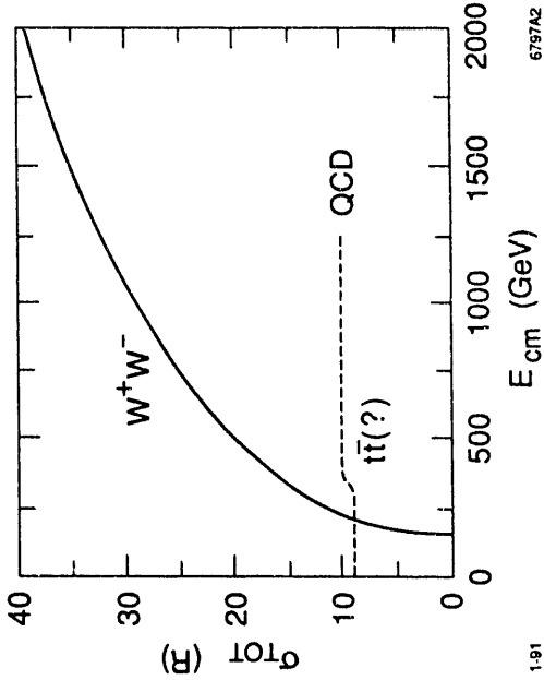
Figure 4. Production cross-sections for the dominant Standard Model processes at high energy.
