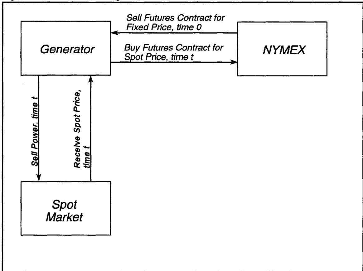
Figure 3-1. Generator's Hedge
