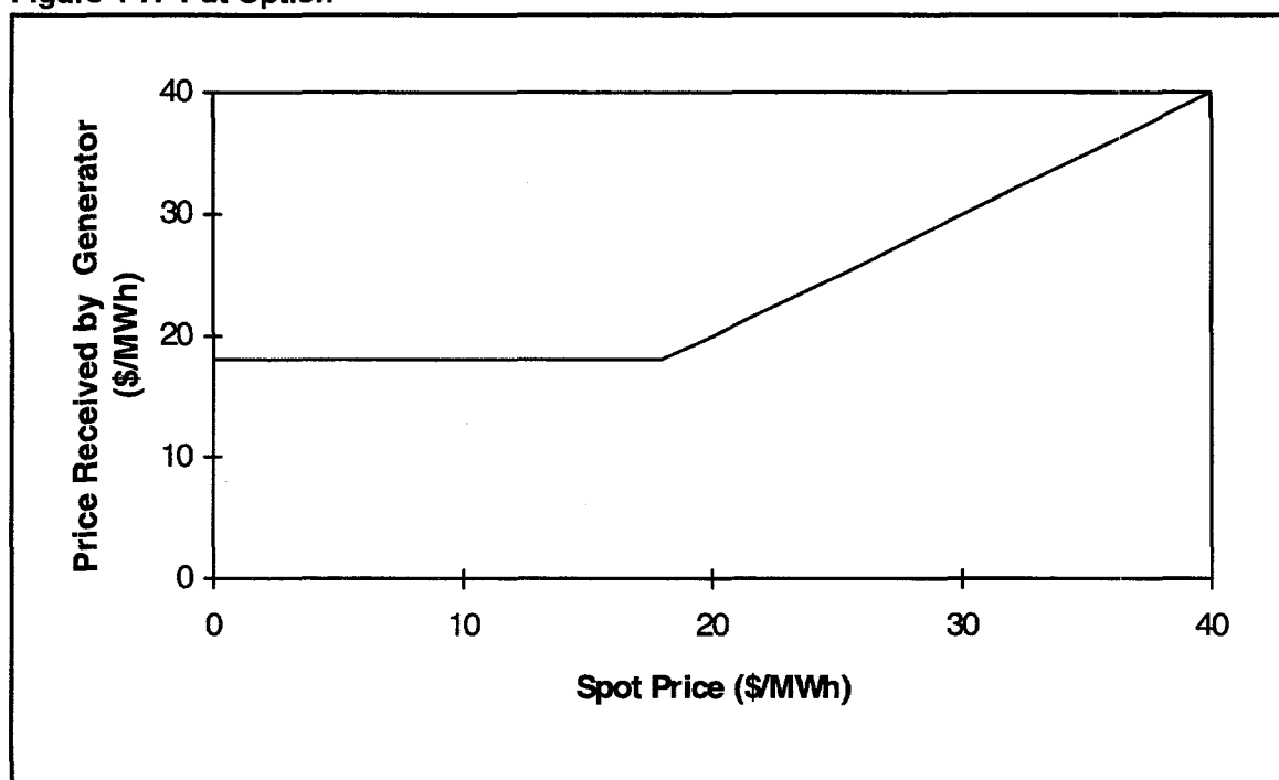
Figure 4-7. Put Option
