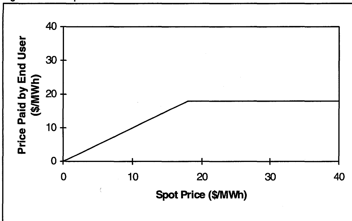
Figure 4-8. Call Option
