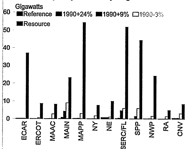
Figure 81. Estimated Biomass Resource Availability and Projected Generating Capacity in 2020 by Region
