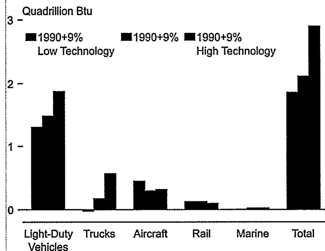
Figure 64. Projected Reductions From Reference Case Projections of Transportation Sector Fuel Consumption in High and Low Technology Sensitivity Cases, 2010
