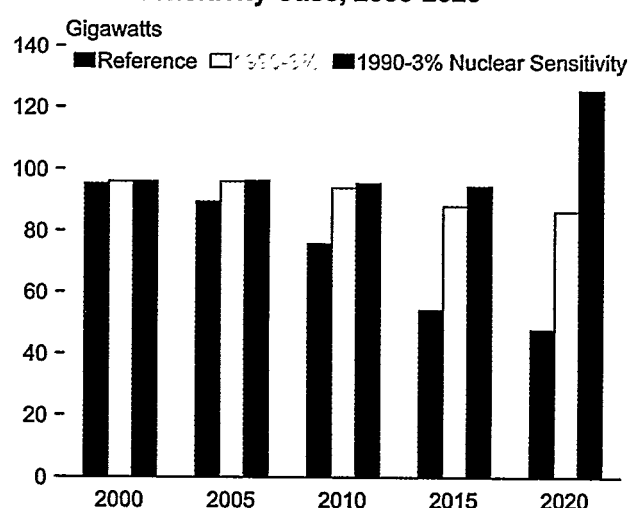
Figure 92. Projections of Nuclear Generating Capacity in the 1990-3% Nuclear Sensitivity Case, 2000-2020
