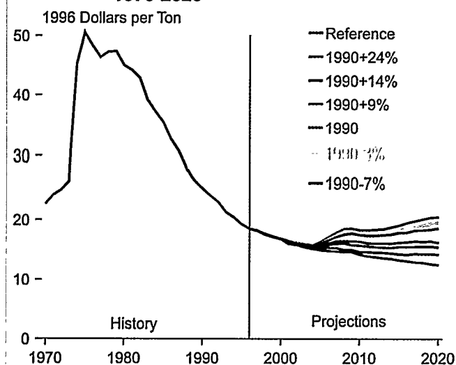
Figure 107. Average U.S. Minemouth Coal Prices, 1970-2020
