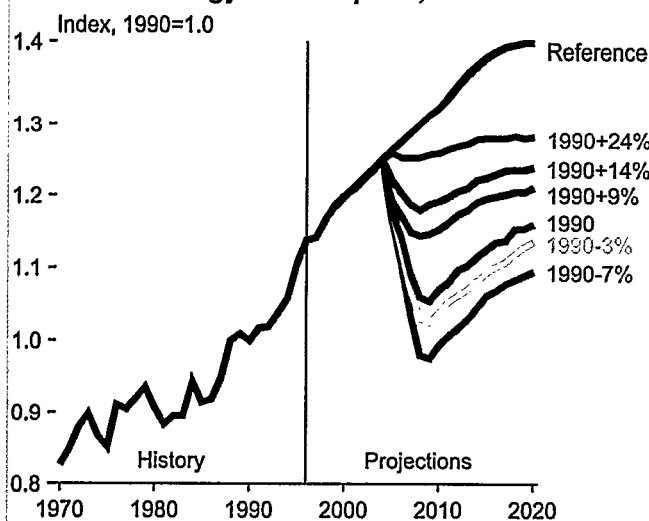
Figure 38. Index of Commercial Sector Delivered Energy Consumption, 1970-2010
