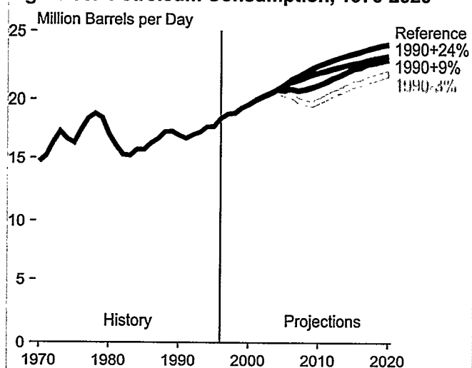
Figure 98. Petroleum Consumption, 1970-2020
