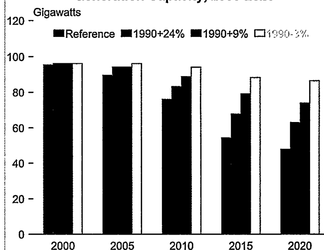
Figure 83. Projections of Nuclear Electricity Generation Capacity, 2000-2020
