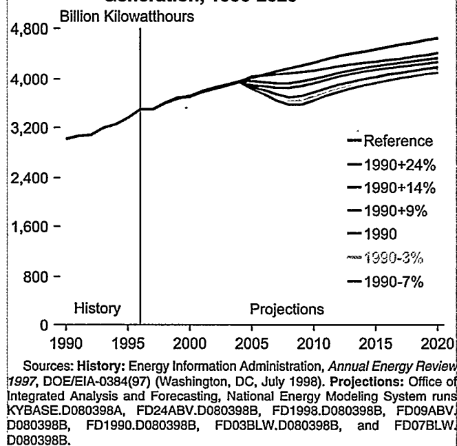
Figure 14. Projections of U.S. Electricity Generation, 1990-2020
