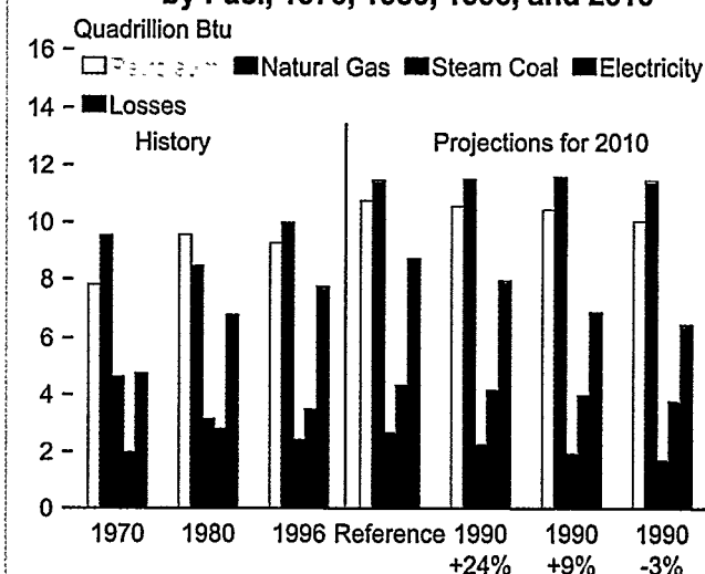
Figure 47. Industrial Sector Energy Consumption by Fuel, 1970, 1980, 1996, and 2010
