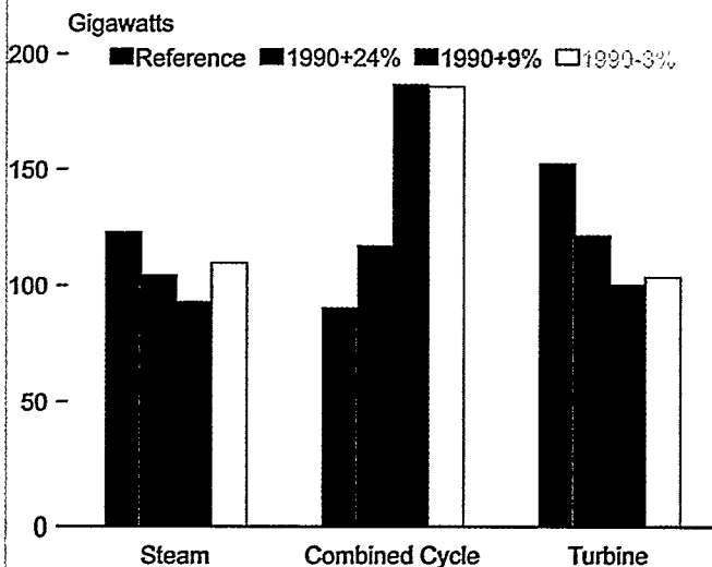
Figure 77. Projections of Natural-Gas-Fired Electricity Generation Capacity, 2010
