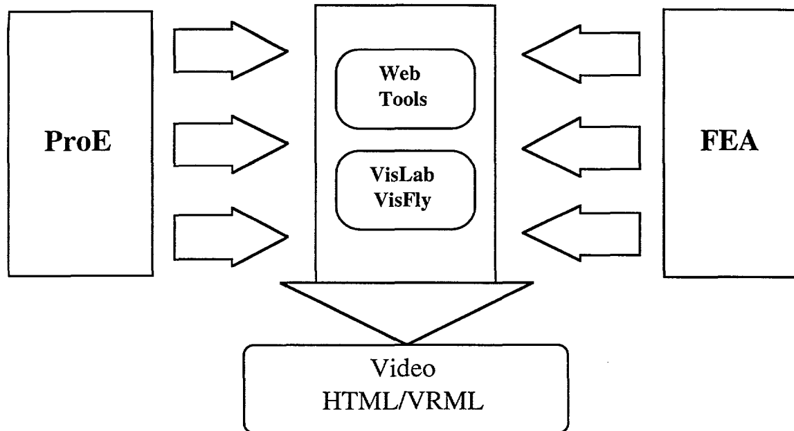
Figure 3. Software Environment
