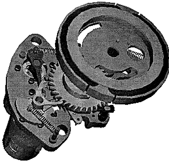
Figure 4. MC4438 Single Stronglink Assembly
