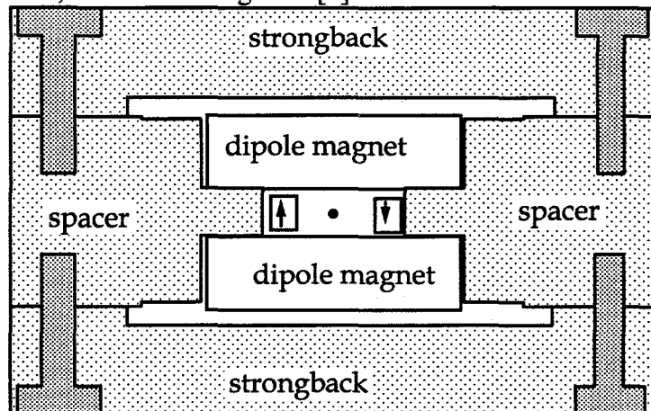
Figure 4: Schematic end view of the VISA undulator. The spacers assure a precise gap between the dipole magnets. Focusing magnets are shown as rectangles on either side of the central beam. For a beam coming out of the page, the arrows indicating the easy axis of magnetization correspond to a horizontally focusing, vertically defocusing (F) quadrupole. Reversing the magnetization gives a horizontally defocusing, vertically focusing (D) quadrupole. The superposition of focusing fields has the desirable effect of suppressing walkoff, in addition to its role in maintaining beam size.
