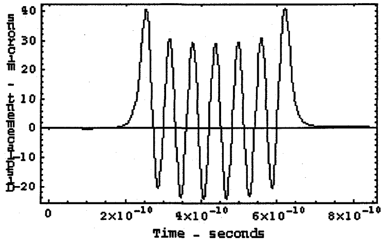
Figure 2: Numerical trajectory calculation for 6 periods of VISA undulator, with symmetric two-half-block termination. The displacement amplitude, peak-to-peak, is about half the beam diameter.
