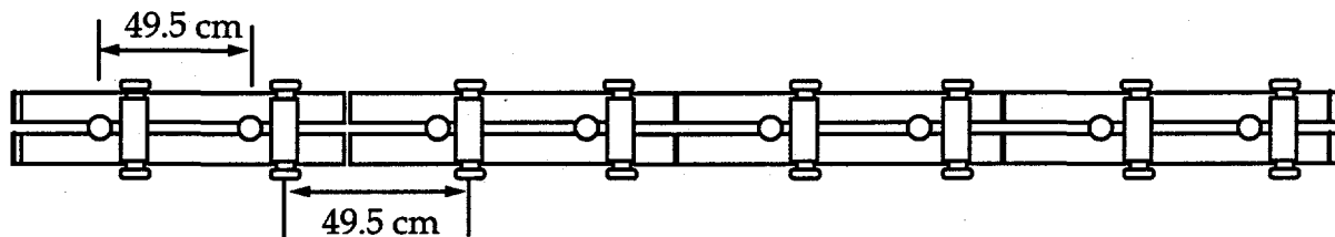
Figure 3: Schematic side view of the VISA undulator, with end terminating magnets on both ends, pop-in diagnostic ports (circles) and steering trim coils (vertical oblong shapes).
