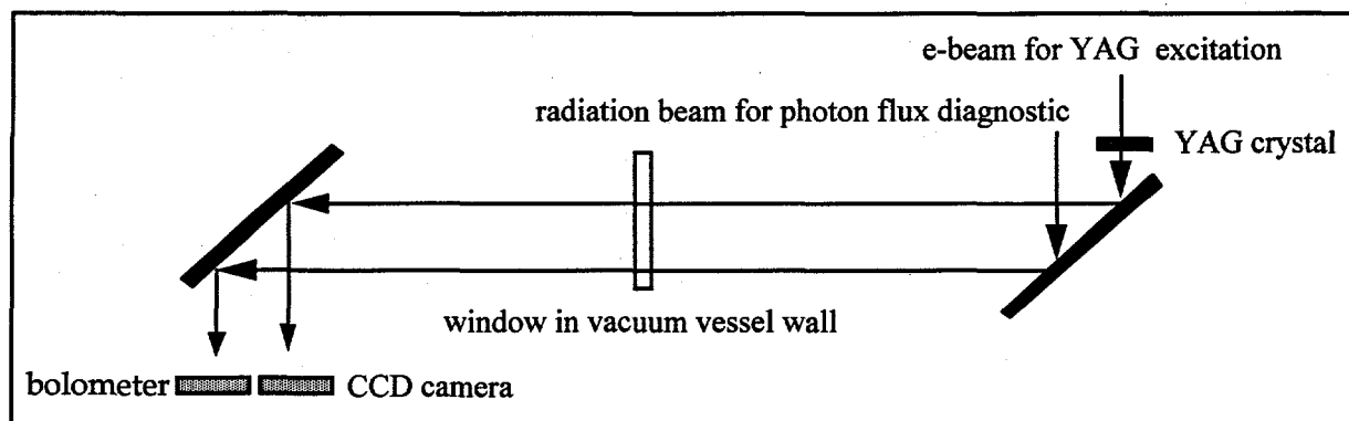
Figure 6: Schematic view of pop-in diagnostic. The mirrors and YAG crystal are translated into two positions that intercept the combined photon and electron beams. The diagram reflects two positions of the periscope; the beams are in the same place with respect to the undulator.
