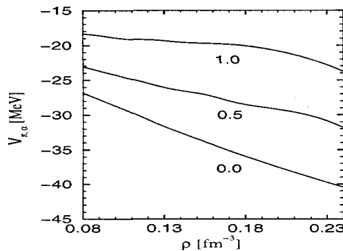
Fig. 2. Plots of \langle NM | V_{\pi} | NM \rangle with the parameters of Ref. [8]. In the G-matrix calculations S is replaced with \alpha S . The plots are for \alpha = 0., 0.5 and 1.0 . The last one is the result of a D-B self-consistent calculation. The other two are not self consistent.
