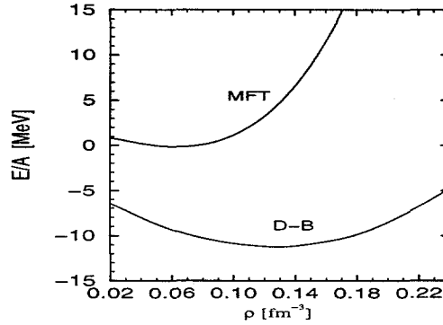
Fig. 3. Plots of E/A from a Dirac-Brueckner and a MFT calculation with the same quasipotential.
