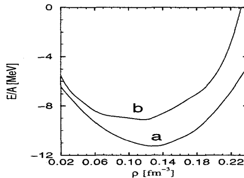
Fig. 1. Plots of the Dirac-Brueckner predictions of E/A (curve a) and E/A - \langle NM | v_\pi | NM \rangle - 17 \text{ MeV} (curve b).
