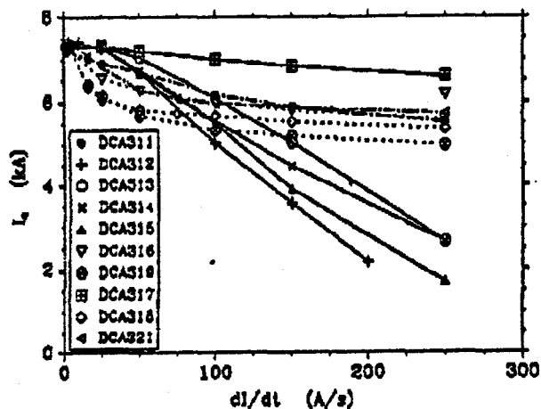
Figure 2. Ramp rate ( di/dt ) dependence of quench current.
