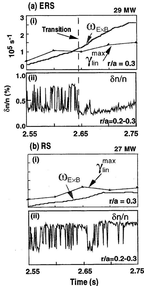
Fig. 11. E×B shearing rate exceeds the linear growth rate at the ERS transition: (a) P_{NBI} = 29 MW i) \omega_{E \times B} and \gamma_{\max} ii) density fluctuations \delta n/n ; (b) P_{NBI} = 27 , no transition i) \omega_{E \times B} and \gamma_{\max} (Synakowski 1997b).
