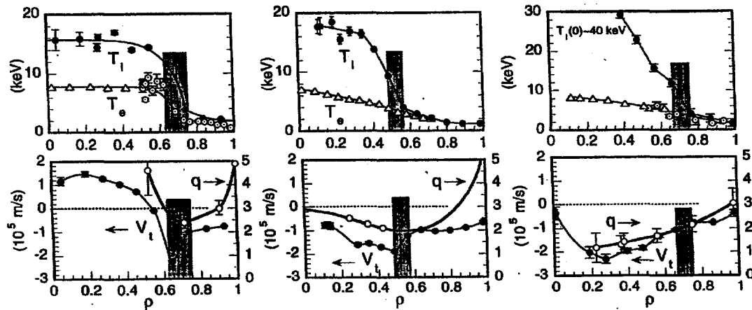
Fig. 8. The profiles in which the ITB is observed is affected by the extent of the shear reversal (Koide 1997); (a) strongly reversed (b) weakly reversed, (c) monotonic.
