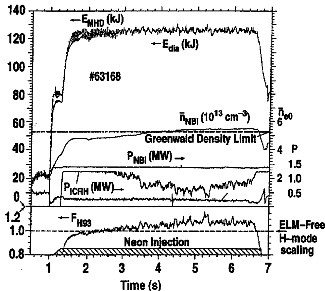
Fig. 3. Radiative I-mode: A.M. Messiaen Phys. Plasmas 4, 1690 (1997).
