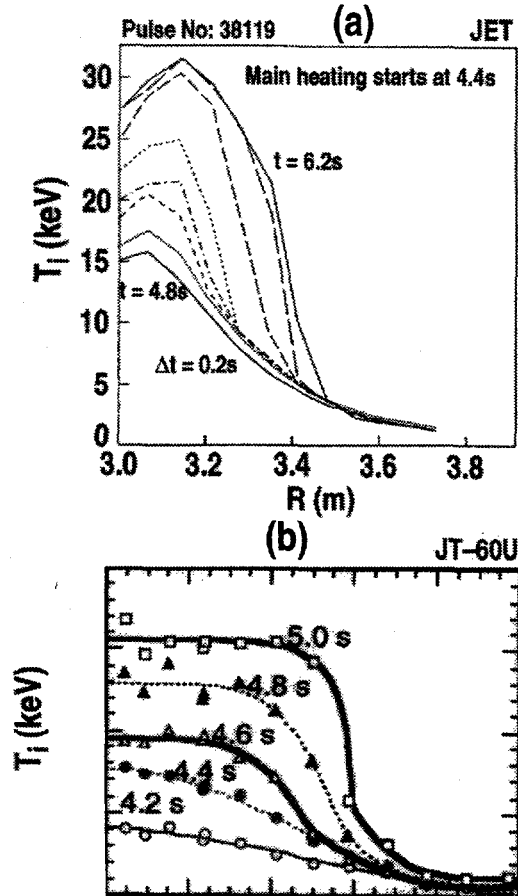
Fig. 12. Local transition starts first in the core and propagates outward (a) T_i profiles from JET discharge [Jones, Phys. Plasmas 4, 1731 (1997)]; and (b) T_i profiles from JT-60U discharge [Fujita, 1996 IAEA, Montreal, IAEA-CN-64/A1-4].
