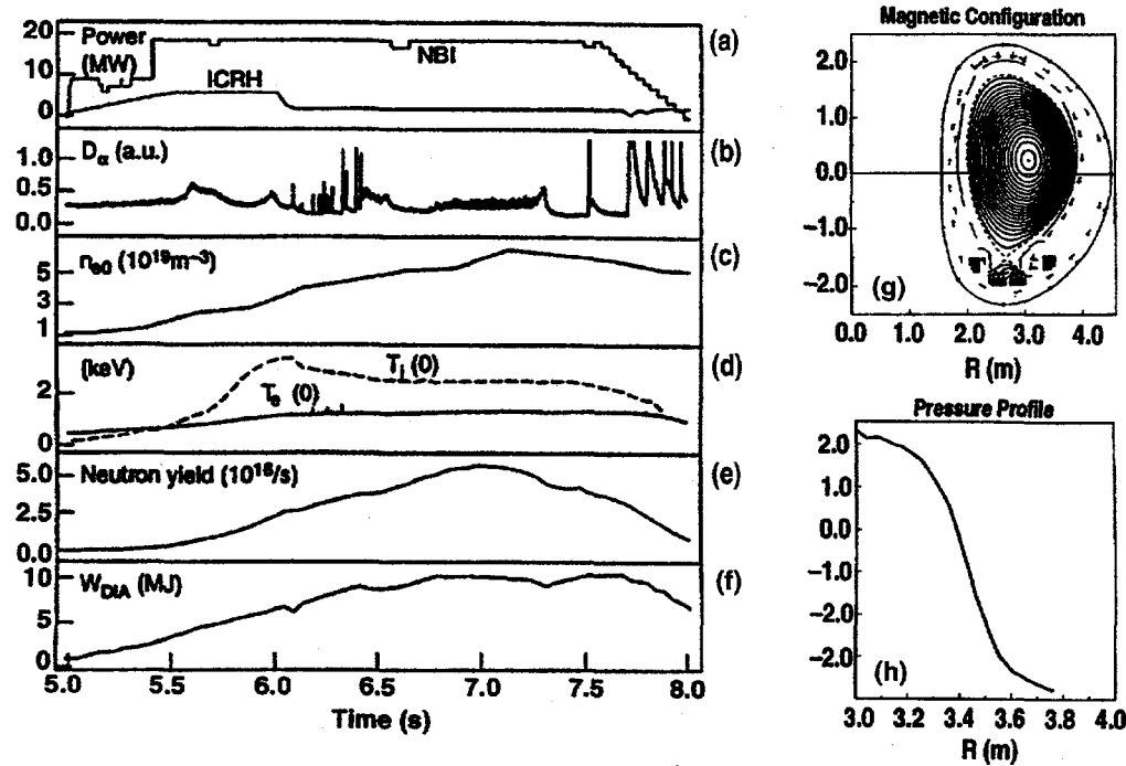
Fig. 18. Record DD JET performance is in optimized shear scenario (Gormezano 1997, Söldner 1997). (a) Neutral beam ICRH heating, (b) divertor D_{\alpha} emission, (c) central electron density, (d) ion and electron temperature, (e) neutron yield, (f) plasma stored energy, (g) magnetic configuration (h) pressure profile.
