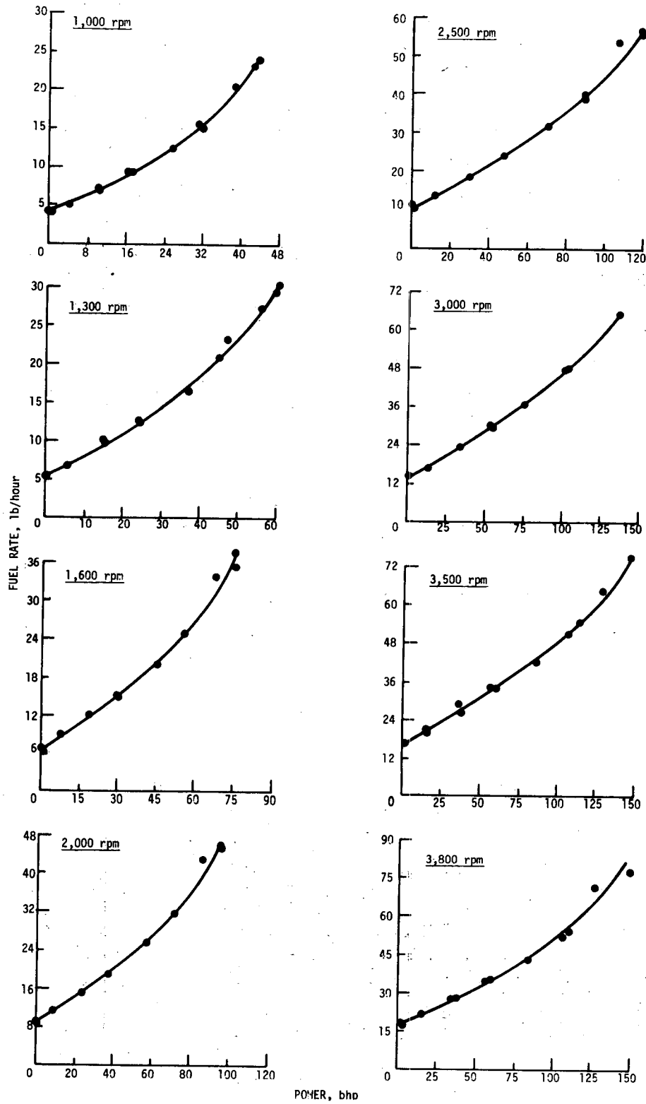
FIGURE 6. Fuel Rate versus Power at Various Speed and Load Conditions--Chevrolet 305-CID Engine.
