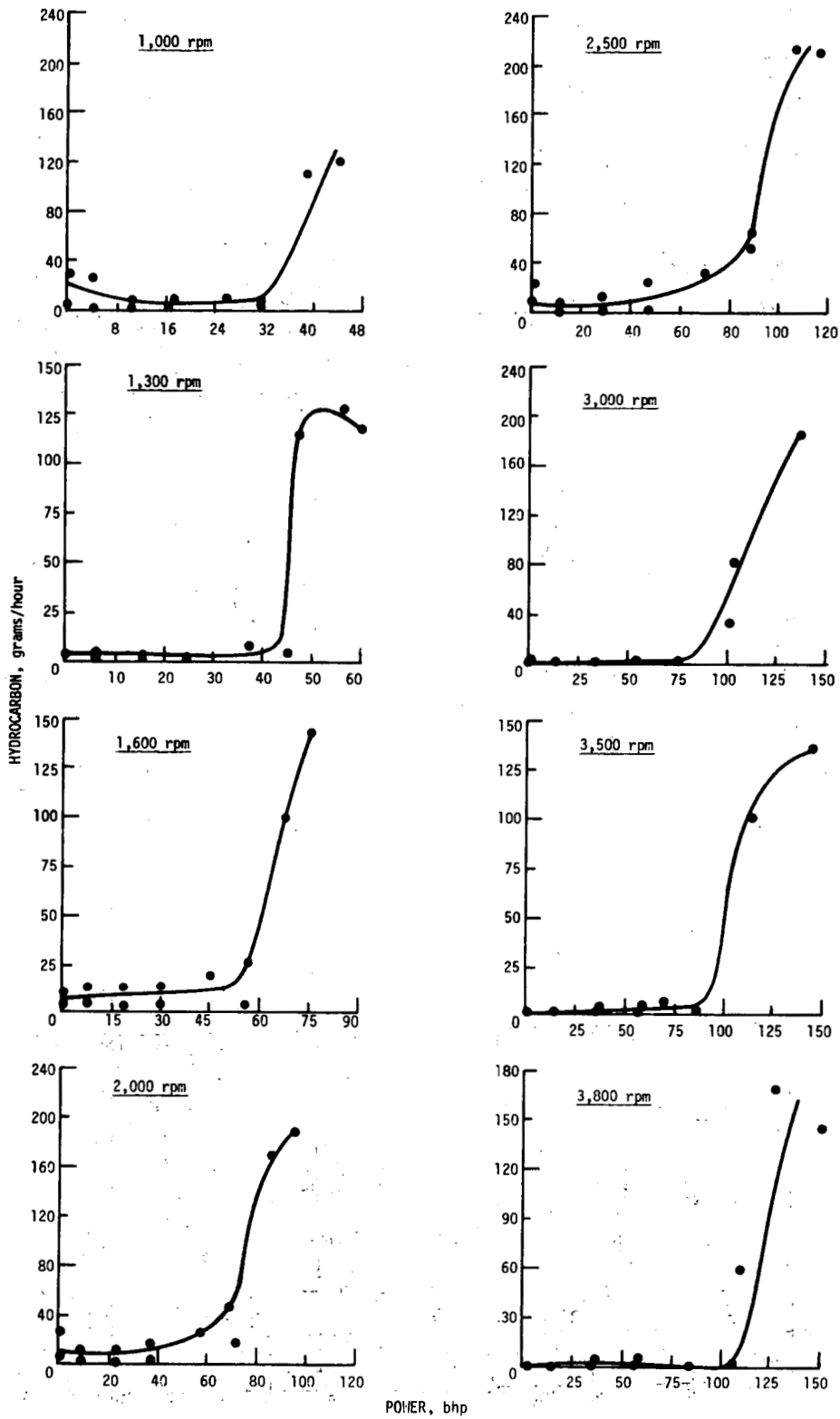
FIGURE 4. Hydrocarbon Emissions versus Power at Various Speed and Load Conditions-- Chevrolet 305-CID Engine.
