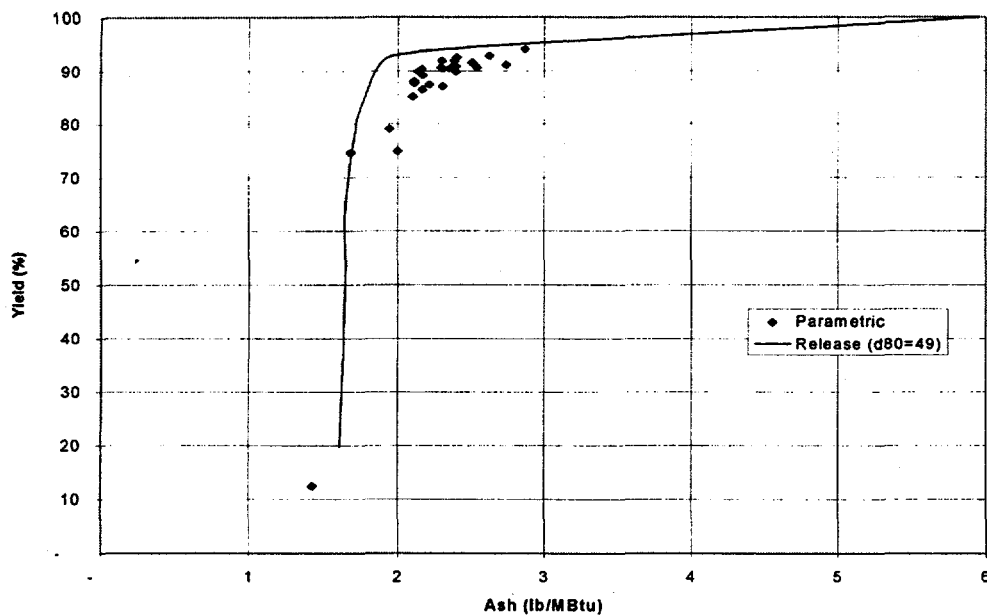
Figure 16. Parametric Testing of Hiawatha Coal - Yield vs. Ash
