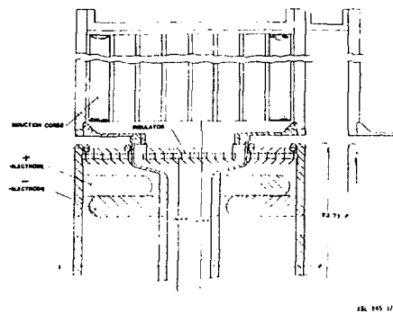
Fig. 7. Cross section of an MBE induction unit.
