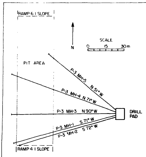
Fig. 3. Orientation of core holes beneath Pit 3, Area G.
