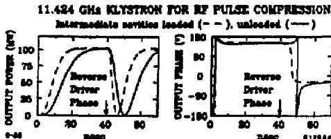
FIG. 4. Transient analysis of a 100 MW, 11.424 GHz five-cavity conventional klystron design for RF pulse compression. In this linear calculation, the RF generator is switched on at 0 nsec in the presence of a DC beam. The generator phase is reversed at 40 nsec, after the switch-on transient has subsided. Dashed curves show that improved risetime is obtained by adding external loads with Q_e = 150 to the gain cavities. Input Q_e = 190 . Output Q_e = 26 . The klystron cavity frequencies without beam are tuned to 21, 16, 40, 500, and 20 MHz, respectively, above 11424 MHz. The DC, 511 A, 440 kV beam detunes the cavities by -21 MHz and loads them with Q_e = 210 . For the five cavities, R/Q = 36, 36, 36, 29 , and 200, respectively. Intercavity spacings are 6, 6, 8, 3 cm.
