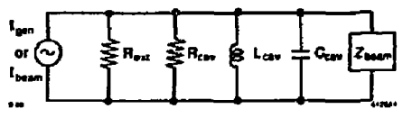
FIG. 1. Each beam loaded klystron cavity is modeled as a parallel network of cavity and beam impedances. External resistance includes additional resistive loading by iris coupled waveguides. The input cavity is driven by an RF generator current. Downstream cavities are driven by the bunched beam current.
