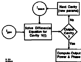
FIG. 2. Flowchart for klystron transient calculations.
