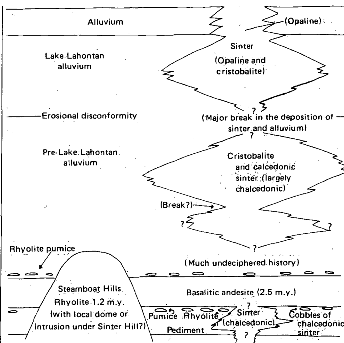
FIGURE 3.—Composite stratigraphic relations at Steamboat Springs, Nevada. Constructed from geologic data of White, Thompson, and Sandberg (1964) and Thompson and White (1964).
