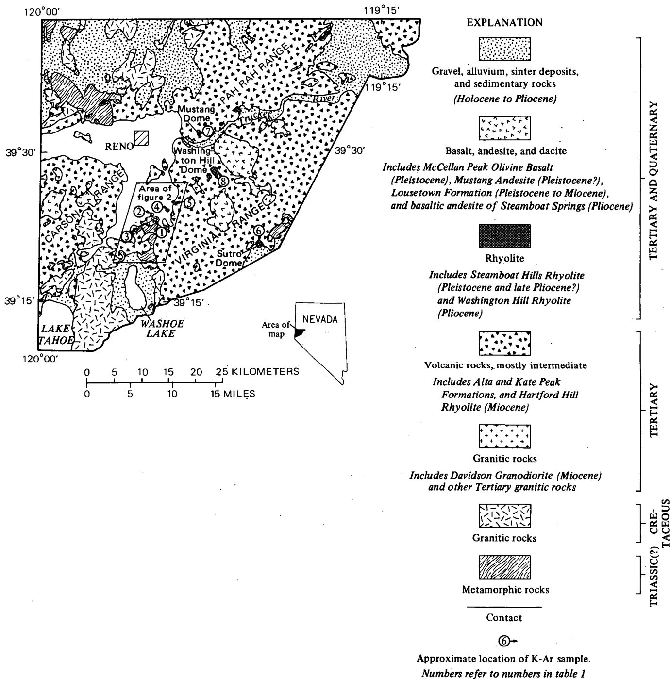
FIGURE 1.—Generalized geologic map of Storey and southern Washoe Counties, Nevada. Geology modified from Bonham (1969).
