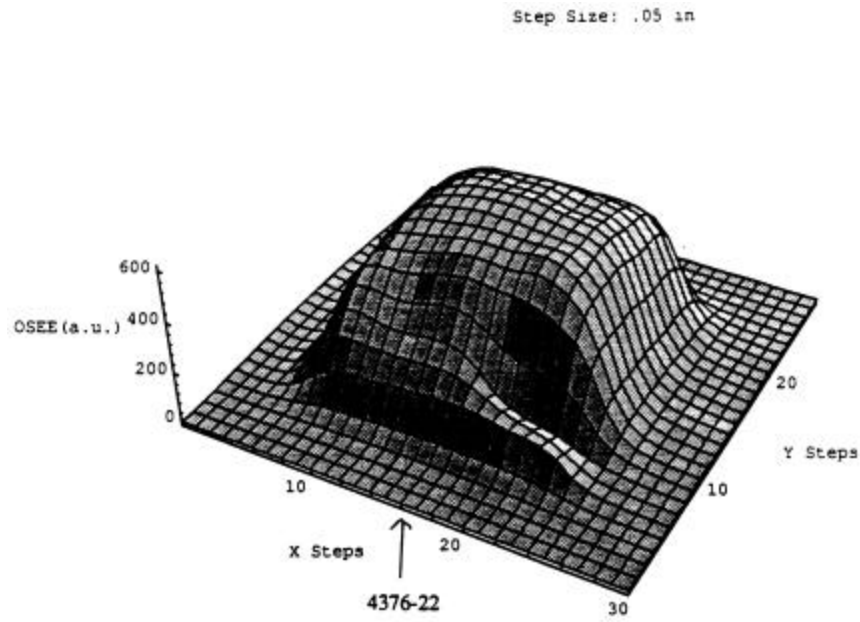
Figure 23. Photoemission in air from sample 4376-22: 200 Å a-SiC p-layer deposited at IEC on 4375-22, textured layer ZnO from Harvard (Prof. Gordon's Group).
