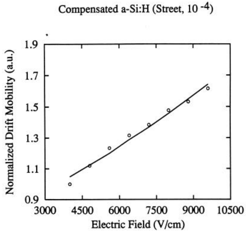
Figure 17. Drift mobility of compensated a-Si:H film with compensation level of 10^{-4} versus electric field.
