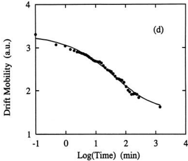
Figure 5(d). The drift mobility \mu_d for the intrinsic a-Si:H sample versus light soaking time. The solid line is curve fit to the stretched exponential law (Eq. (22)). In addition to the decay of the dc photoconductivity and lifetime, continuous decay of the drift mobility can be seen due to light soaking. Different stretched exponential parameters were found, which are shown in Table I. The drift mobility \mu_d was determined by Eq. and \mu_{mix} was determined by P_{mix} .
