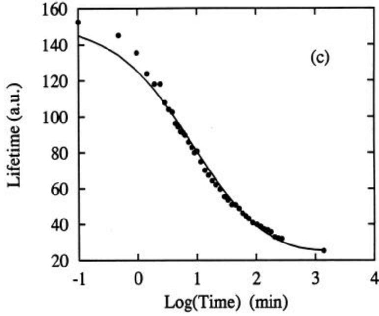
Figure 5(c). The lifetime \tau for the intrinsic a-Si:H sample versus light soaking time. The solid line is curve fit to the stretched exponential law (Eq. (22)).
