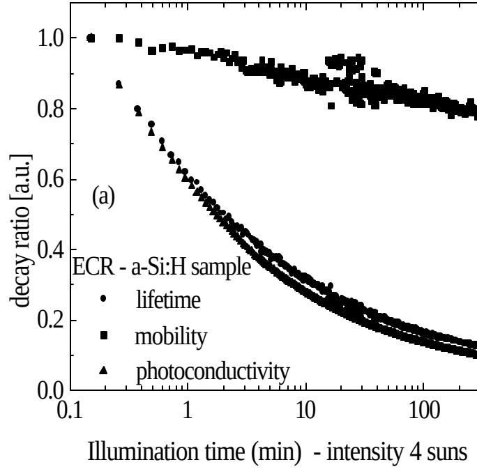
Figure 61. The decay of mobility ( \mu ), lifetime ( \tau ), and photoconductivity ( \sigma ).
