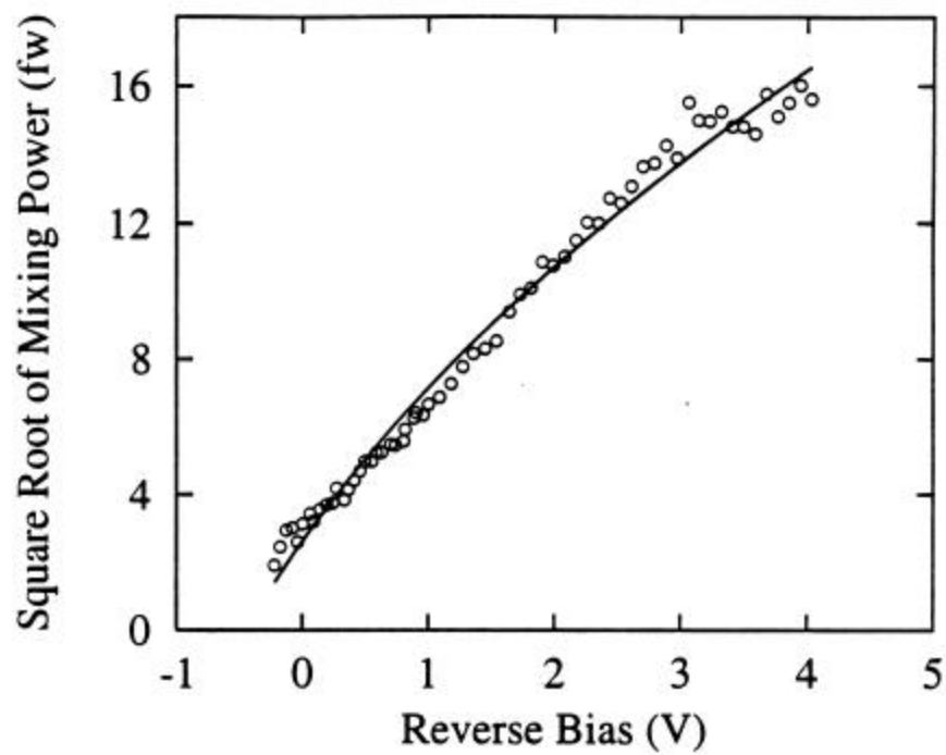
Figure 47, The mixing power vs. reverse bias for Schottky sample THDni50.
