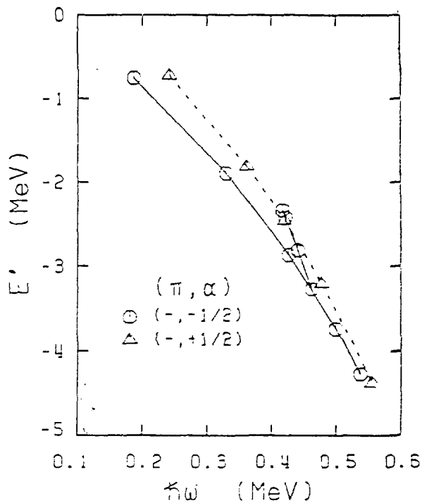
Fig. 4. Energy in the rotation frame vs. rotational frequency.
