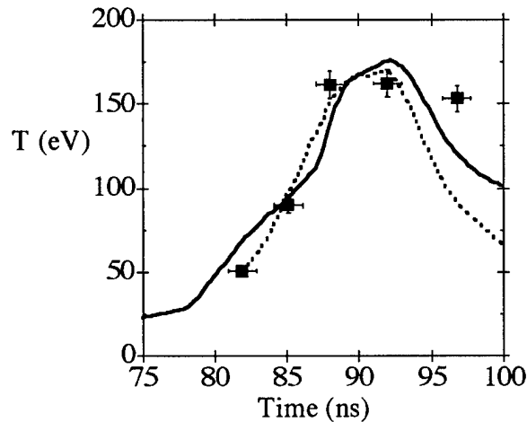
Fig. 6. a) Brightness temperature obtained on-axis and calculated, 2-D RMHD, electron temperature in the foam (solid line). Square points are the data using the size from the framing camera. Dashed line was generated using the size from a quadratic fit to the first four frames of the framing camera.
