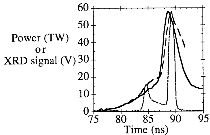
Fig. 2. XRD traces and X-ray emitted power. The solid trace is the measured Kimfol (200-280 eV) XRD output. The dotted curve is the calculated XRD voltage using 1D LASNEX normalized to the experimental data. The dashed line is the 3T diffusion estimate (2-D RMHD) of the calculated power-radiated.
