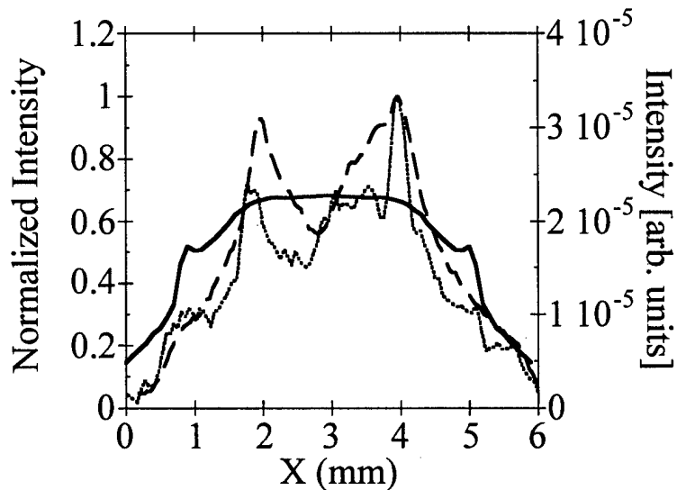
Fig. 5. Comparison of emission profiles for radial lineouts of the 85 ns framing camera image. \Delta y \sim 1 mm (dotted trace), and \Delta y \sim 5 mm (dashed trace) compare the experimental result to the calculated profile at 85 ns with the modeled image for \Delta y = 5 mm (solid curve).
