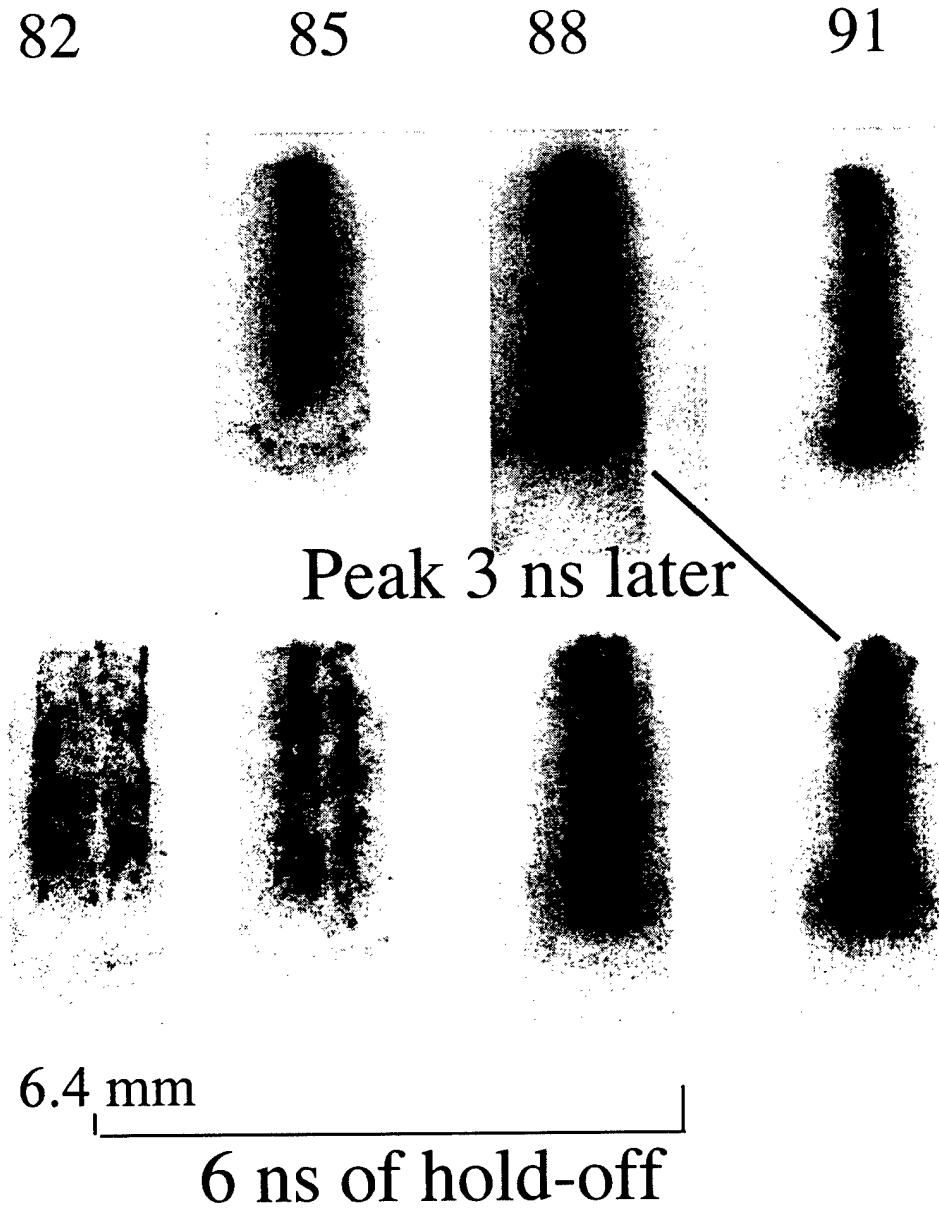
Fig. 3. Soft x-ray (200-280 eV) framing camera images of pinches without (top) and with (bottom) the central foam. The time in ns, with respect to figure 1, is shown above the images.
