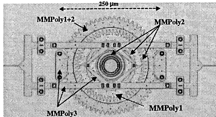
Figure 1. The Micromachine Wedge Stepper Motor designed by James Allen of Sandia National Laboratories and fabricated using the SUMMiT process.
