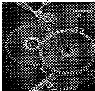
Micro Torque Converter
