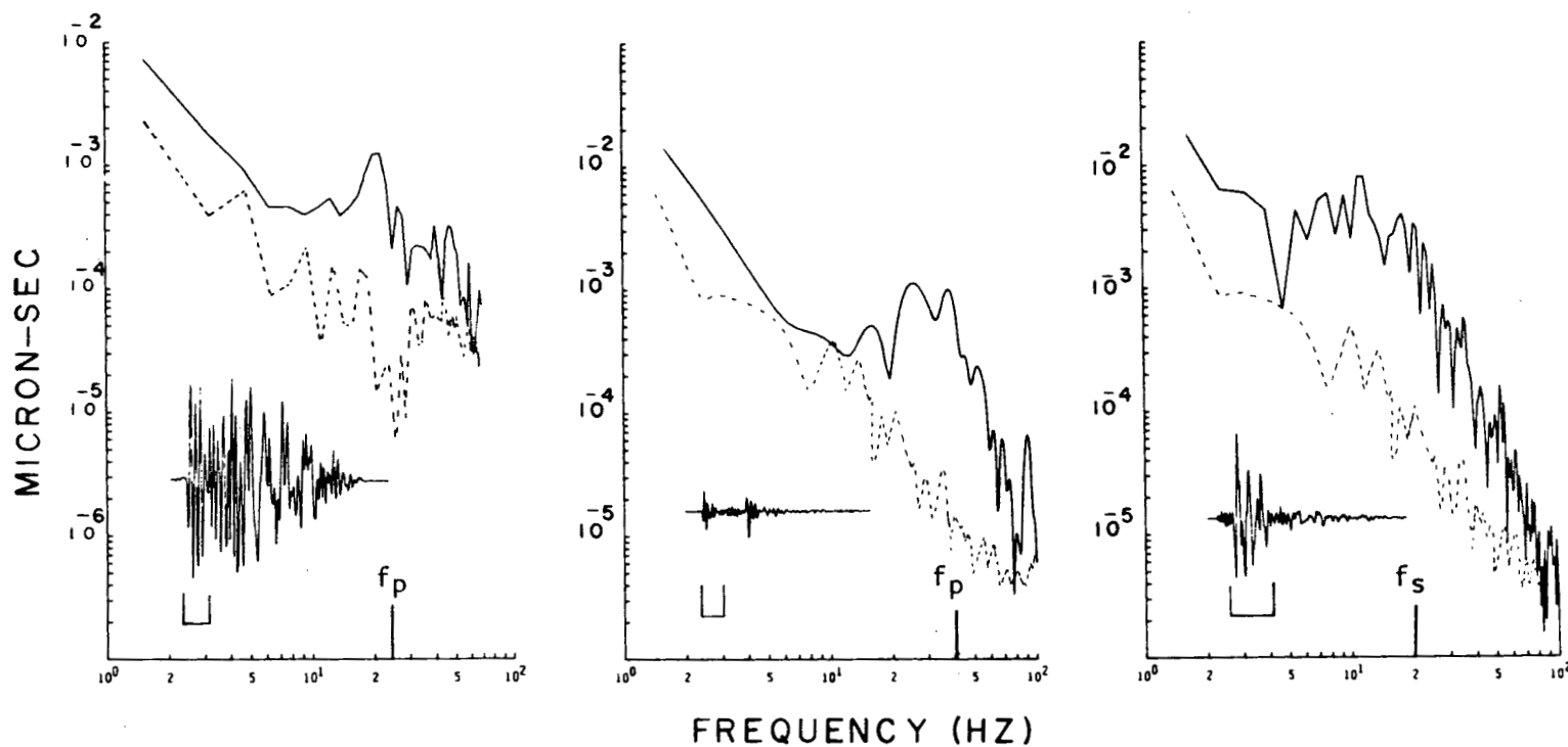
Typical displacement spectra used in source studies. On left is P-wave recorded on FM tape system, center is P-wave recorded on digital system, and right is S-wave recorded digitally. FM signal is shown at higher gain than other two. Corner frequencies and data windows are indicated. Note the higher quality data obtained with the digital system.
