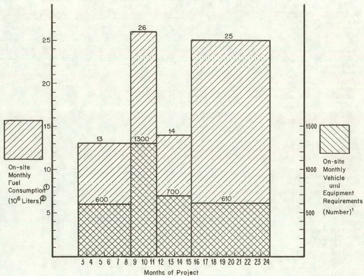
Figure 19. GRS MONTHLY CONSTRUCTION VEHICLE AND EQUIPMENT REQUIREMENTS AND ASSOCIATED FUEL CONSUMPTION
