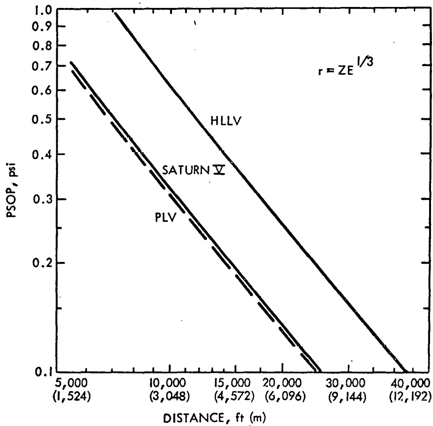
Figure 13. Variation of Peak Side-On Overpressure with Distance for Catastrophic Explosion
