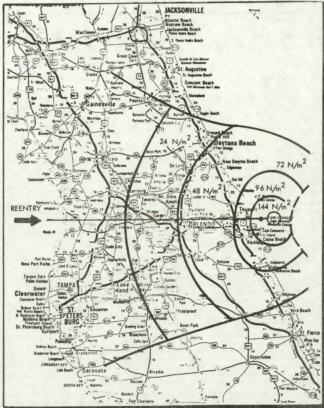
Figure 11. SONIC BOOM OF HLLV ORBITER ON RETURN TO LAUNCH SITE
