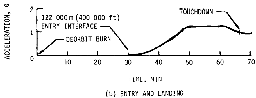
Figure A-6. ACCELERATION PROFILES OF THE SPACE SHUTTLE VEHICLE AS A FUNCTION OF TIME.
