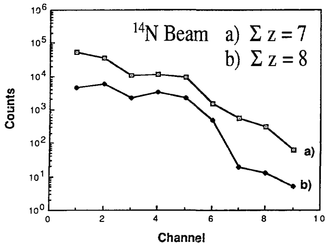
Fig. 9 Comparison of the relative intensities for (a) inelastic scattering and (b) the pickup of one H from a C target. The channels are listed in the adjacent table.
