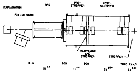
Fig. 1. Overall layout schematic showing the ion source, RFQ, and two Alvarez cavities. The poststripper consists of the last 51 cells of the original injector linac.
