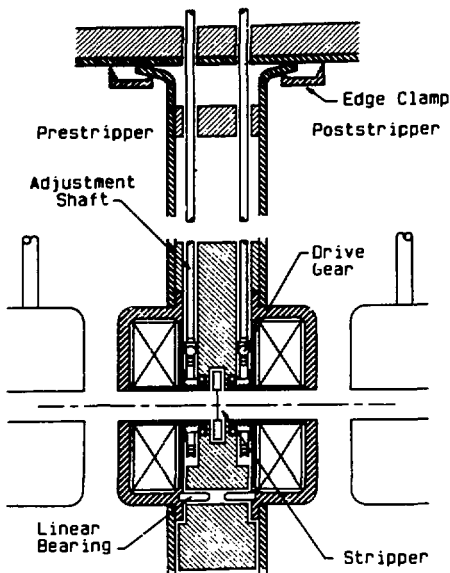
Fig. 3 Prestripper-poststripper transition schematic showing the two half drift tubes, quadrupoles, channel for insertion of stripper, and connection of diaphragm periphery to tank wall. The drive gear, turned by the adjustment shaft, moves the drift tube longitudinally
