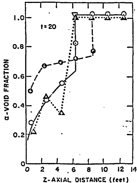
Figure 8 Comparison Between the Measured and Predicted Axial Void Distributions in the GE Level Swell Test
