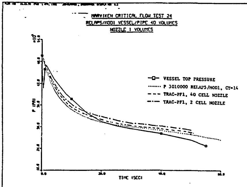
Figure 2 Comparison Between the Measured and Predicted Vessel Top Pressure for Marviken Test 24
