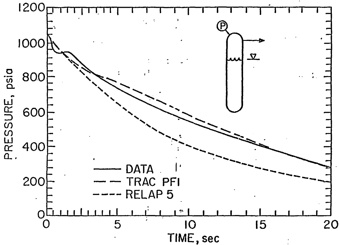
Figure 7 Comparison Between the Measured and Predicted Vessel Pressures in the GE Large Vessel Level Swell Test
