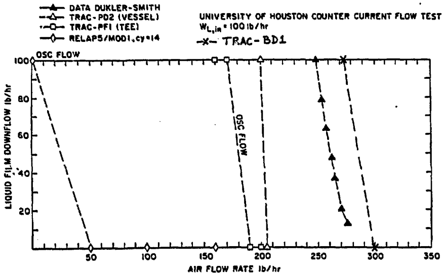
Figure 3 Comparison Between the Measured and Predicted Water Downflow Rate vs. Air Flow Rate for Water Feed Rate of 100 lb/hr
