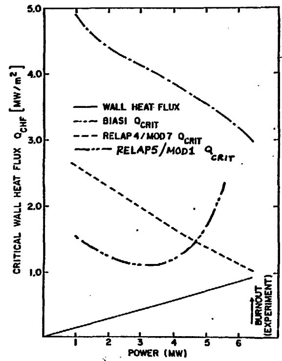
Figure 15 Comparison Between the Measured and Predicted Power for CHF or Burnout
