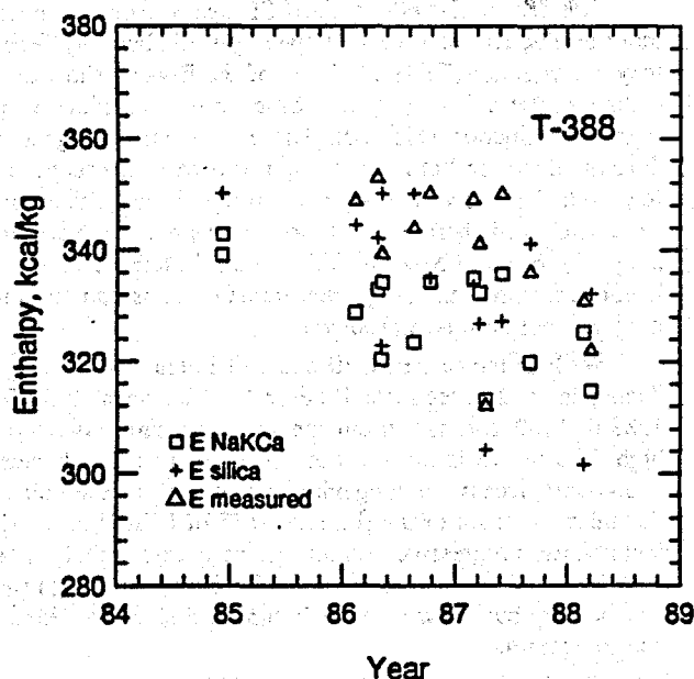
Figure 7. Indicated aquifer liquid enthalpy and wellhead total fluid enthalpy values for well T-388 (see caption of Fig. 4).
