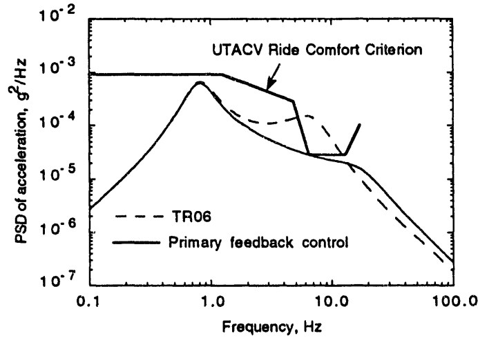
Fig. 34. PSD of vehicle acceleration using active feedback controls in primary suspension with vehicle speed v = 100 \text{ m/s} and guideway roughness amplitude A = 10^{-6} \text{ m}
