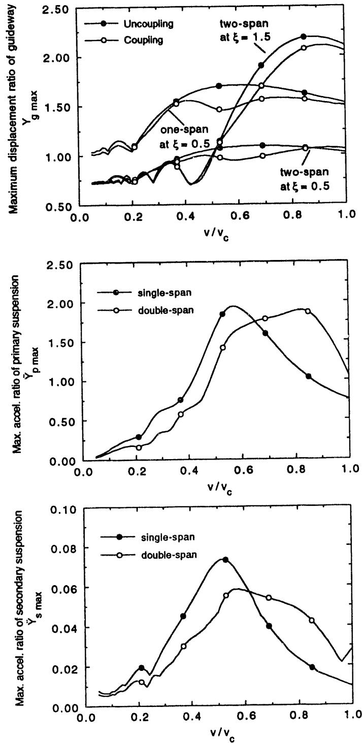
Fig. 5. Effects of single-span and double-span beams on maximum guideway displacement and vehicle acceleration ratios for a two-degree-of-freedom vehicle
