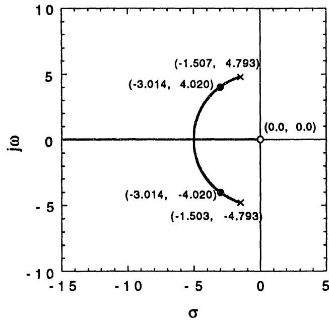
Fig. 42. Root-locus diagram for secondary suspension feedback control design
