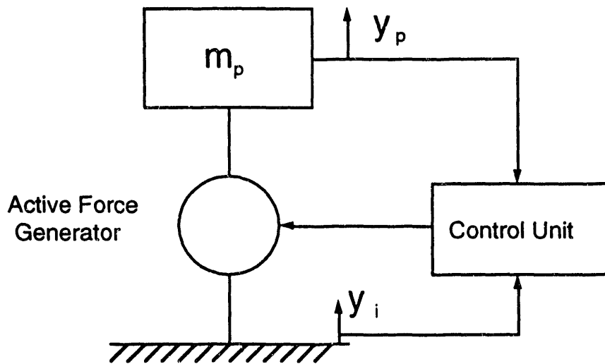
Fig. 30. Active control configuration for primary suspension
