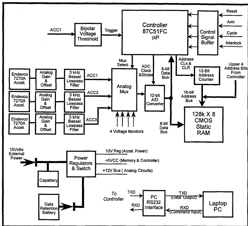
Figure 2: MinPen Block Diagram
