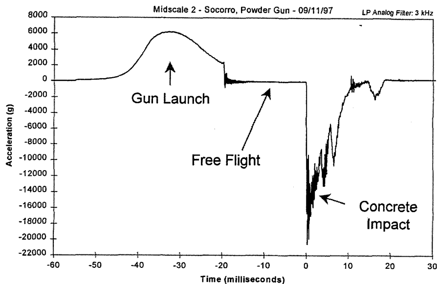
Figure 6: Midscale #2 Axial Acceleration Record
