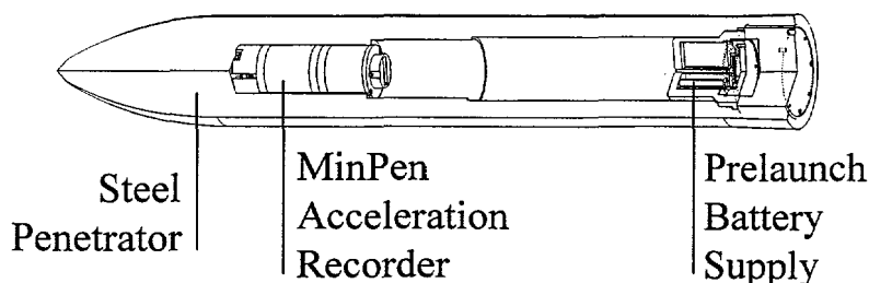
Figure 4: MinPen secured inside Penetrator
