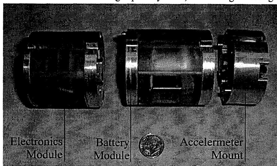
Figure 1: Photograph of MinPen Acceleration Recorder
