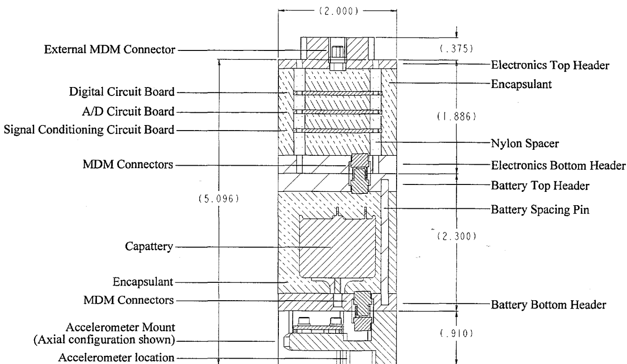
Figure 3: Cross-section of MinPen Acceleration Recorder MECHANICAL ASSEMBLY AND PROCESSES
