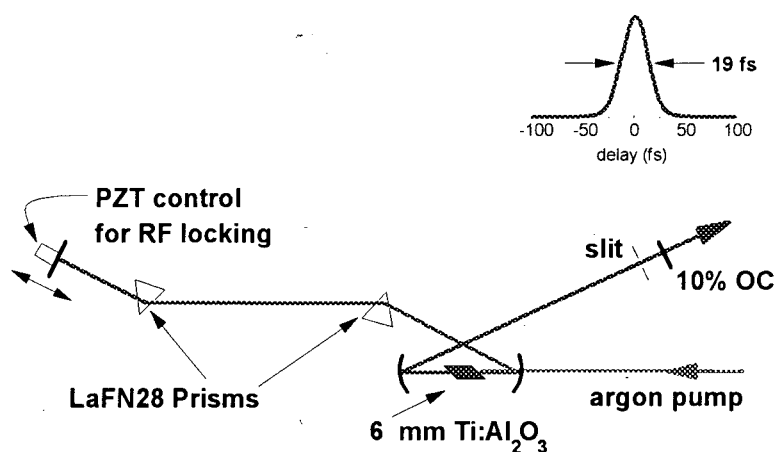
Figure 2.7: Ti:Sapphire based Kerr lens modelocked laser.
