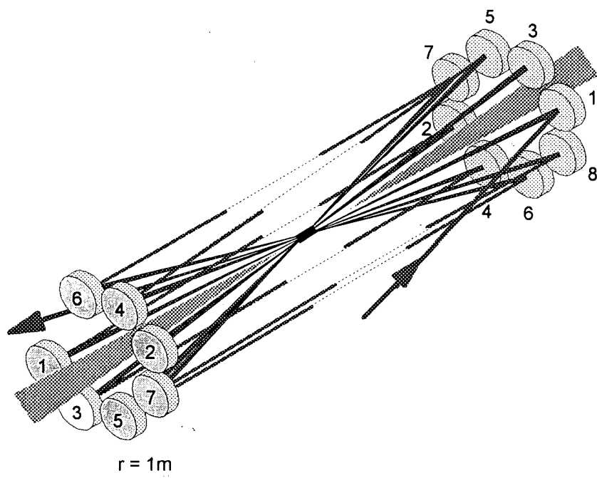
Figure 2.10: Novel preamplifier configuration in the terawatt laser system.
