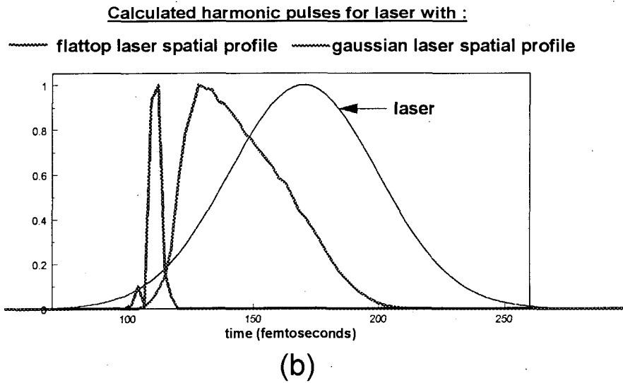
Figure 4.8: Spatial profile effects on the harmonic generation process. (a) illustrates temporal broadening due to spatial intensity variation. (b) compares high-order harmonic temporal profiles for Gaussian and flat-top laser spatial profiles.
