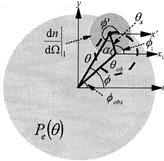
Figure 2.6: Defining the constant energy path of integration. The angle \theta from the electron beam axis ( z ) corresponds to a distance on the x - y plane at a fixed distance from the generation point.
