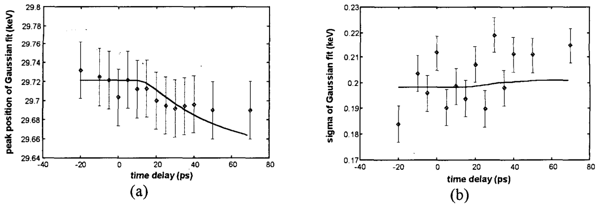
Figure 3.9: Parameters of Gaussian fits to x-ray diffraction spectra versus time delay: (a) spectral peak position, and (b) spectral width. The curve is from the same fit in Figure 3.7.
