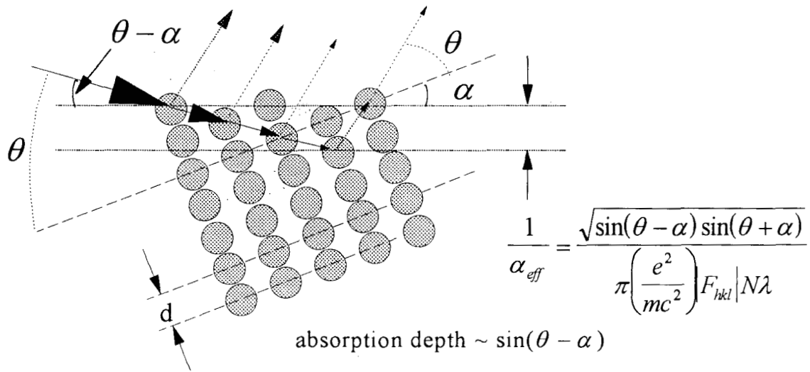
Figure 3.3: Asymmetric Bragg diffraction.
