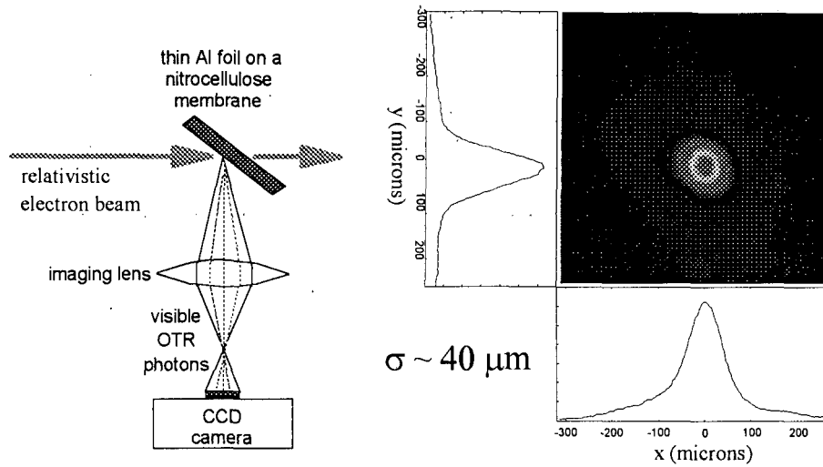
Figure 2.13: Optical transition radiation (OTR) electron beam profile diagnostic.
