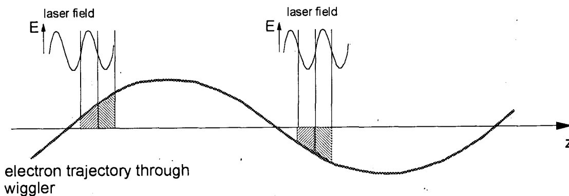
Figure 5.2: Acceleration of an electron slice in a wiggler with a co-propagating laser pulse.
