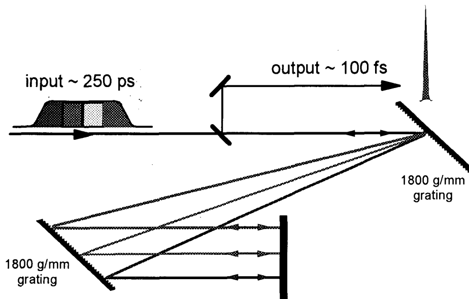
Figure 2.12: Pulse compressor.
