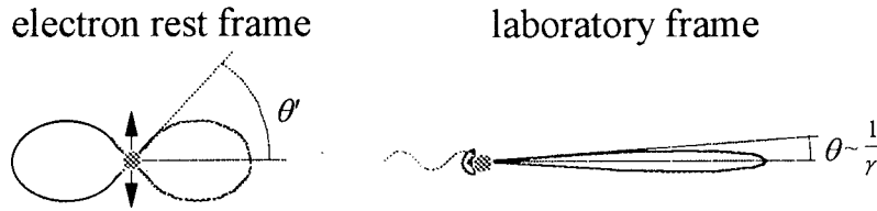
Figure 2.3: Relativistic transformations.
