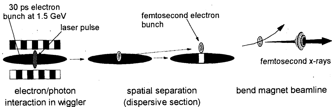
Figure 5.1: Electron bunch slicing in a storage ring.
