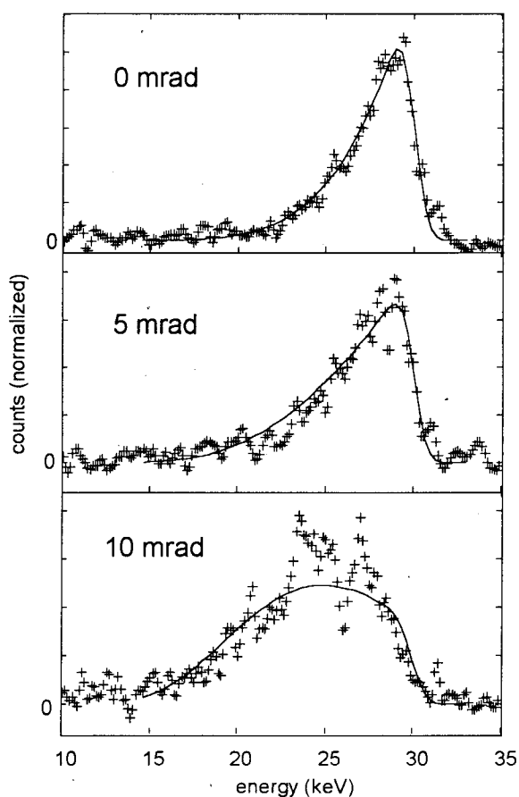
Figure 2.19: Normalized x-ray spectra at observation angles of 0 mrad, 5 mrad, and 10 mrad from the center of the beam.
