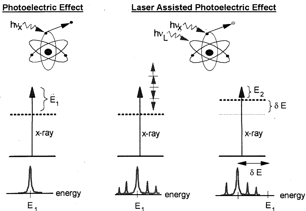
Figure 4.1: Laser-assisted photoelectric effect (LAPE).
