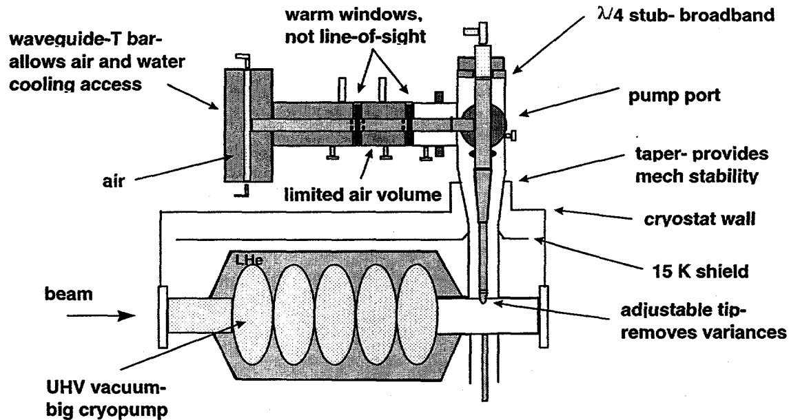
Fig. 6. Schematic diagram showing the design features being included in the 210-kW cw power coupler.
