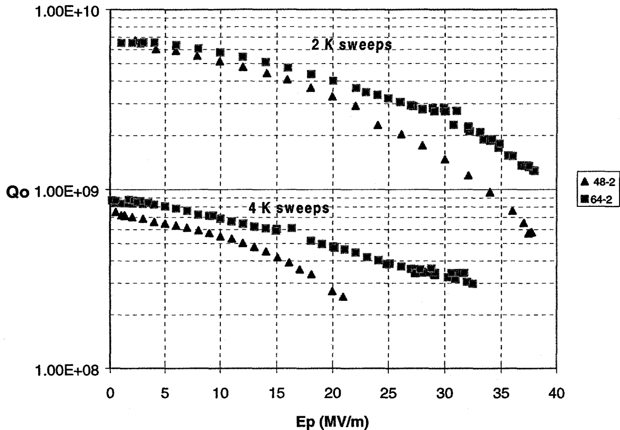
Fig. 2. Q_0 vs E_p curves for \beta=0.48 and 0.64 cavities at both 2 and 4 K. Neither cavity exhibited signs of multipacting, and field performance was acceptable.
