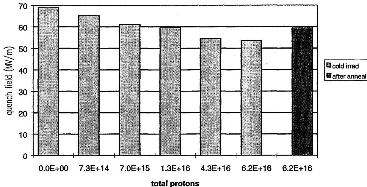
Fig. 5. Plot showing the maximum peak electric field achieved prior to quench related to the total number of protons irradiating the cavity. Note that the abscissa is not linear.
