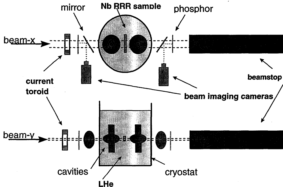
Fig. 3. Layout of the Proton Effects Experiment, showing the relative beam envelope to scale in the x and y planes. The 800 MeV proton beam passed through the entire assembly, including cavities, cryostat, and liquid helium. Approximately 10% of the beam was lost in transmission.
