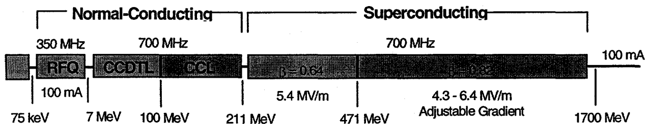
Fig. 1. Schematic layout of a cw proton linac showing the transition energies between various linac structures.
