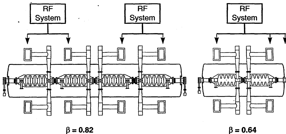
Fig. 7. Schematic representations of the \beta=0.64 and \beta=0.82 cryomodules.
