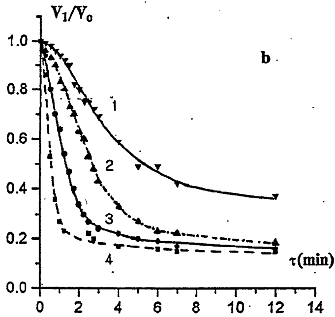
Figure 3.7. Sedimentation of \text{PuO}_2 \cdot x\text{H}_2\text{O} in 1 - 3 M NaOH / 3 M \text{NaNO}_3 2 - 3 M NaOH 3 - 1 M NaOH 4 - \text{H}_2\text{O} at 20^\circ\text{C} \text{PuO}_2 \cdot x\text{H}_2\text{O} aging conditions: a) 1 M NaOH, 100^\circ\text{C} , five hours; b) 1 M NaOH, 200^\circ\text{C} , five hours
