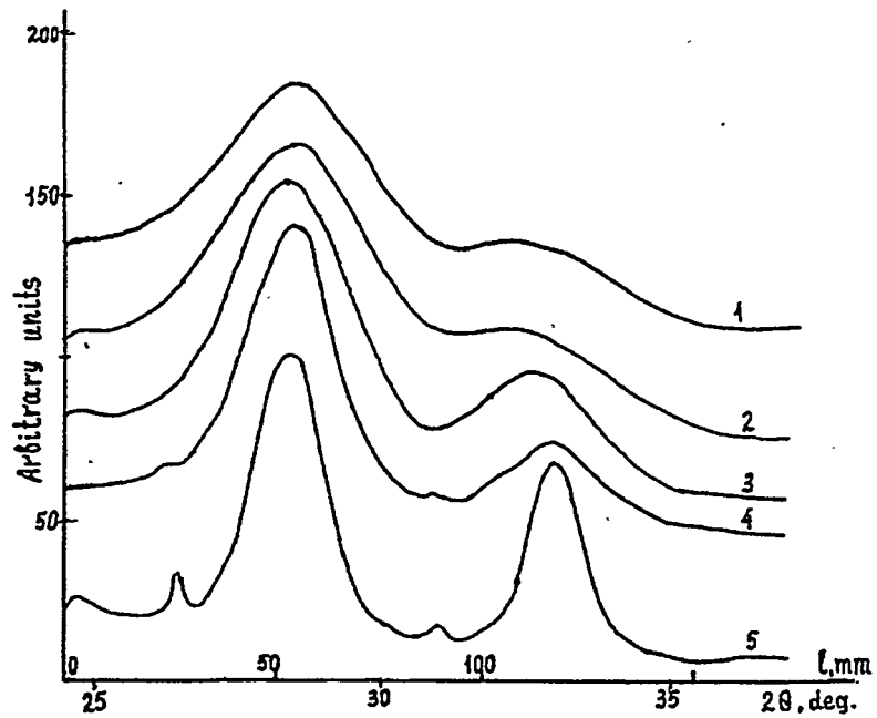
Figure 3.2. X-Ray Diffraction Patterns of \text{PuO}_2 \cdot x\text{H}_2\text{O} and the Shape of the (111) Line as a Function of Heating Temperature (in ^\circ\text{C} ): 1 - 75 2 - 200 3 - 300 4 - 400 5 - 800
