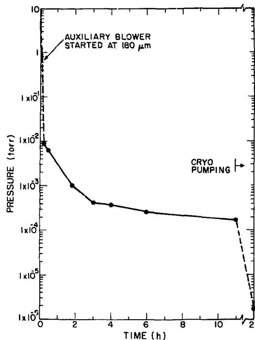
Fig. II-6. Electron-gun pumpdown time with cryogenic pump.
