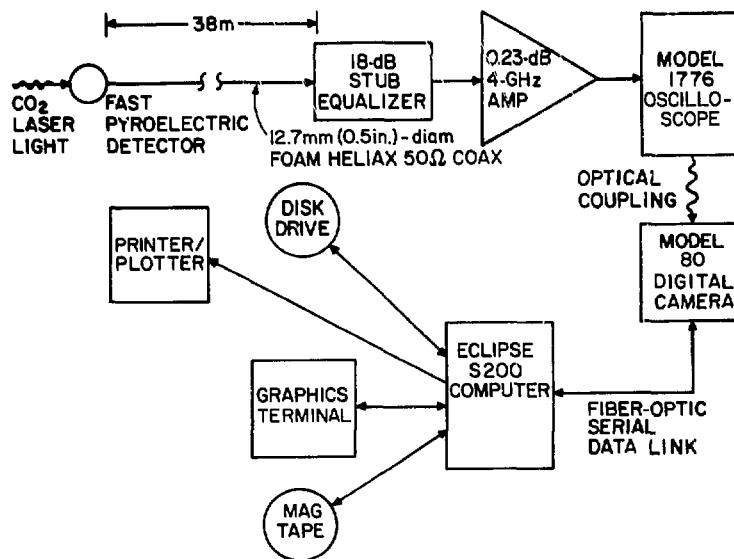
Fig. II-19. Schematic for testing fast oscilloscopes.
