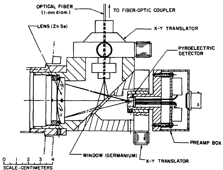
Fig. II-11. The DVS projects visible light from the target position to the alignment station telescope and detects \text{CO}_2 laser light from the alignment station.
