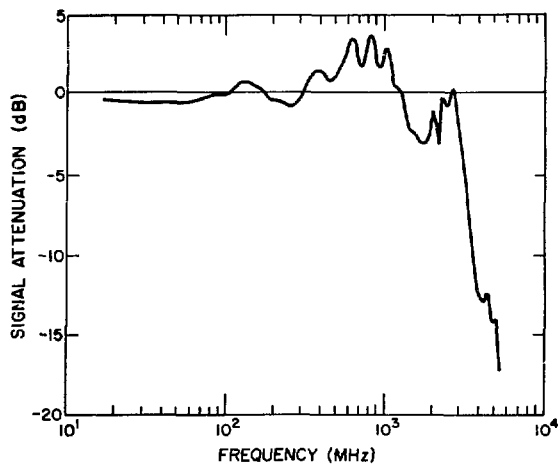
Fig. II-20. Model-1776 oscilloscope system response.
