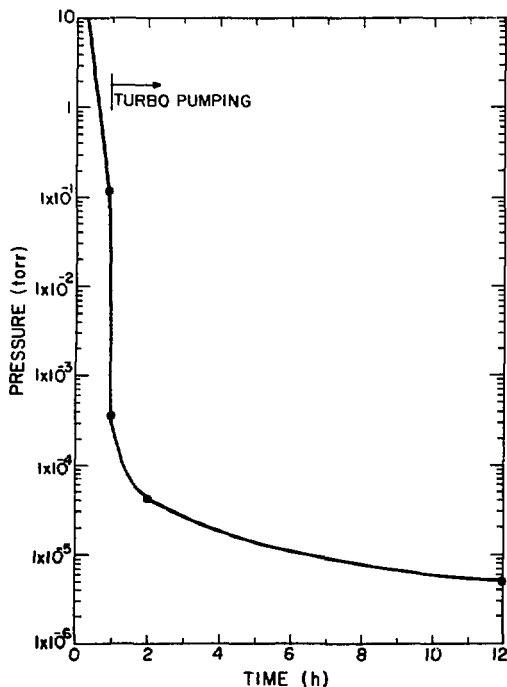
Fig II-5. Electron-gun pumpdown time with turbomolecular pump.
