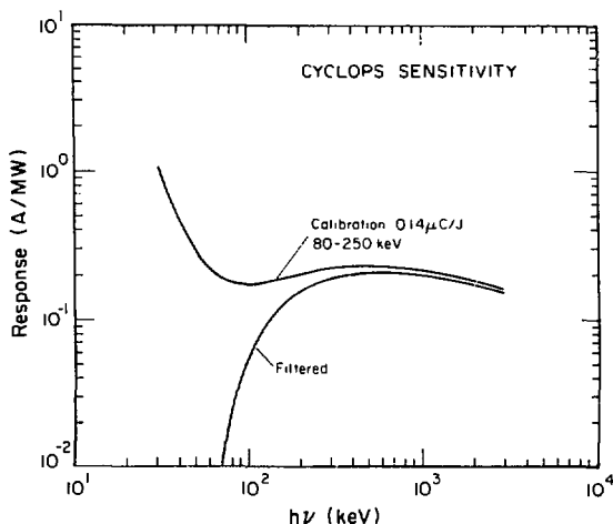
Fig. III-10. Spectral response of CYCLOPS.
