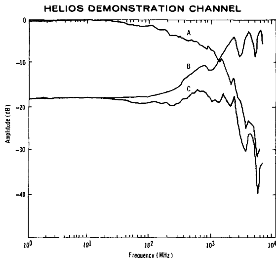
Fig. V-16. Measured system frequency response (curve A) for the Helios beam-diagnostic channel, which consists of 38 m of 1.27 cm coaxial cable, an amplifier, a 1776 oscilloscope, and a scope trace digitizer. Calculated equalizer response (B) and anticipated system response (C) are also shown.
