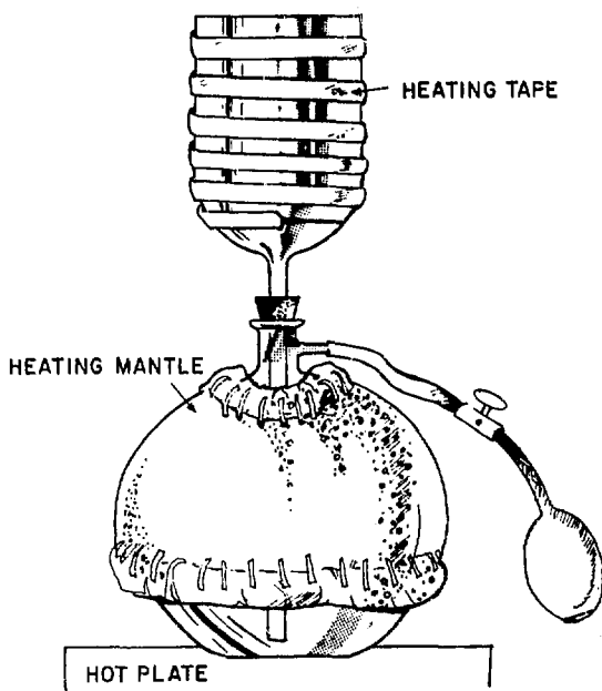
Fig. VI-5. Film-casting apparatus with heating tape and mantle.
