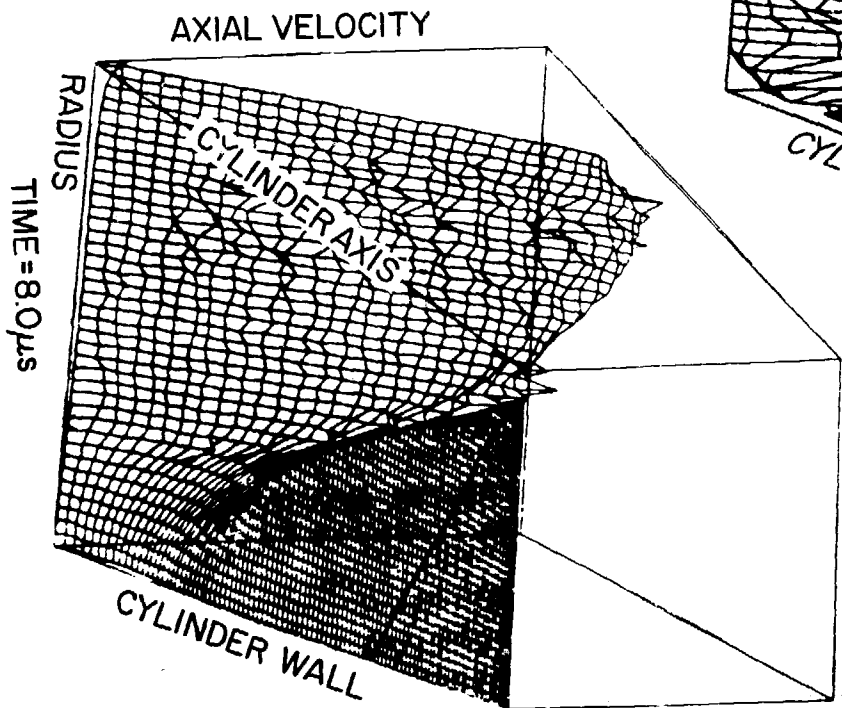
Fig. IX-12. Axial velocity distribution of back-ground fluid.
