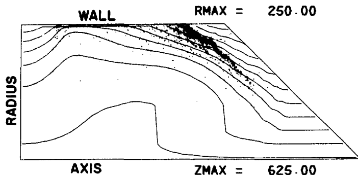
Fig. IX-7. Ion cloud in fluid density of n = 10^{13} atom/cm 3 .
