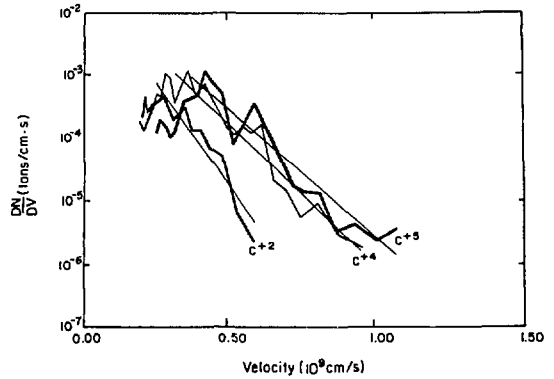
Fig. III-8. Experimental ion velocity distribution for C^{+2} , C^{+4} , and C^{+5} in pure carbon plasma. Electron temperature \sim 31 keV, errors for velocity less than 10%.
