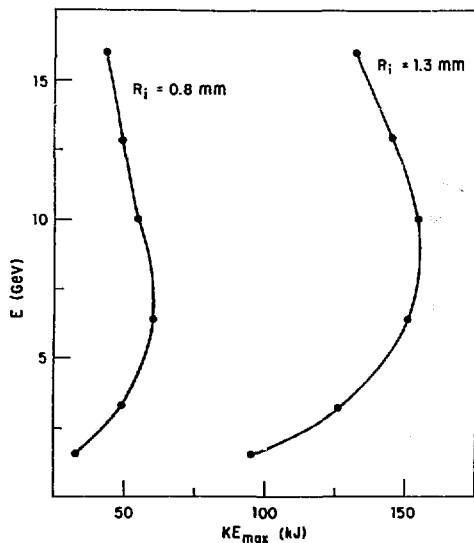
Fig. VIII-14. Ion particle energy vs maximum kinetic energy.
