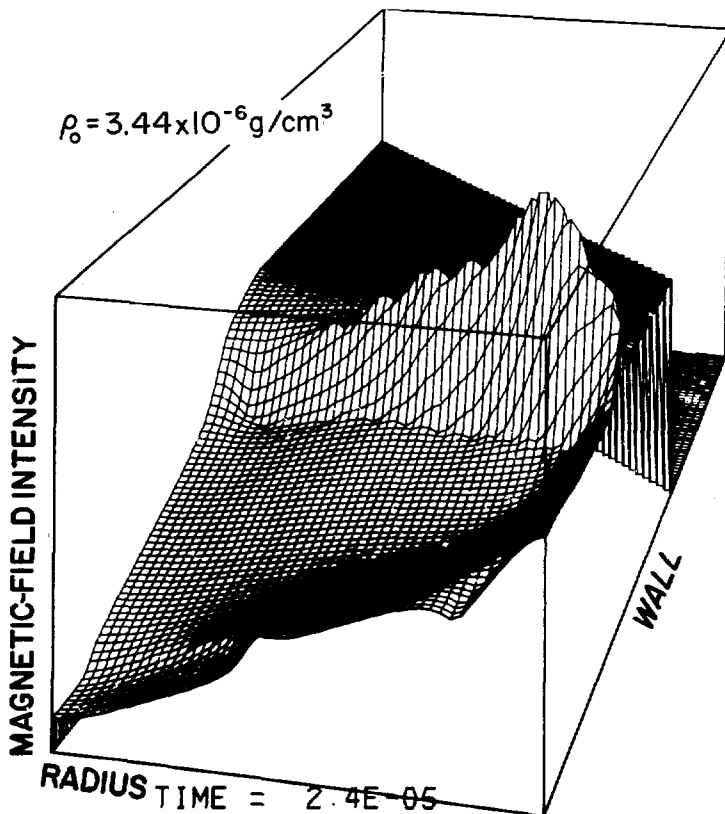
Fig. IX-10. Magnetic-field intensity in fluid density of n = 10^{17} \text{ atom/cm}^3 .
