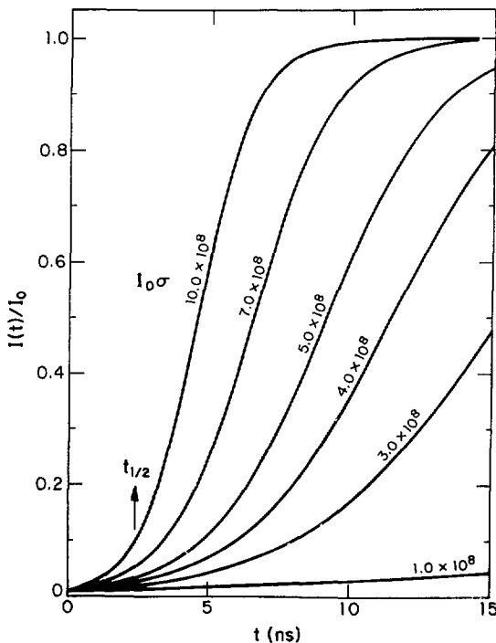
Fig. VII-2. Time-dependent transmission by reversible photodissociative absorbers.
