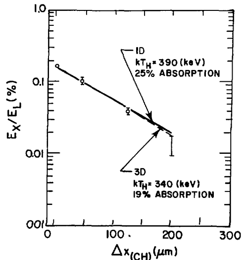
Fig. IV-10. Interpolated LASNEX suprathermal x-ray yield.
