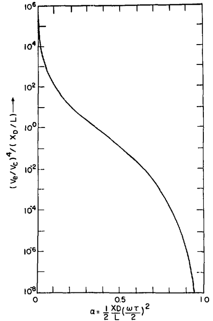
Fig. IV-2. Solution of Eq. (IV-25) of the text, (v_e/v_e)^4/(x_D/L) vs a , provides approximate wave-breaking or convective saturation time given driver amplitude, background plasma temperature, and density scale length.
