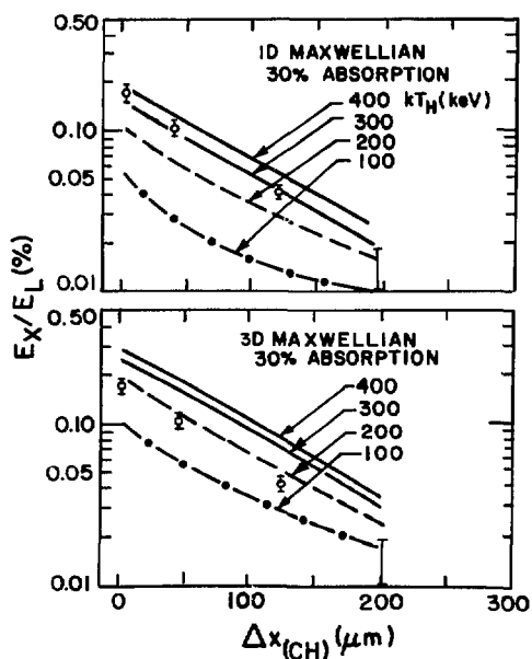
Fig. IV-8. Comparison of LASNEX and APACHE suprathermal x-ray yields.
