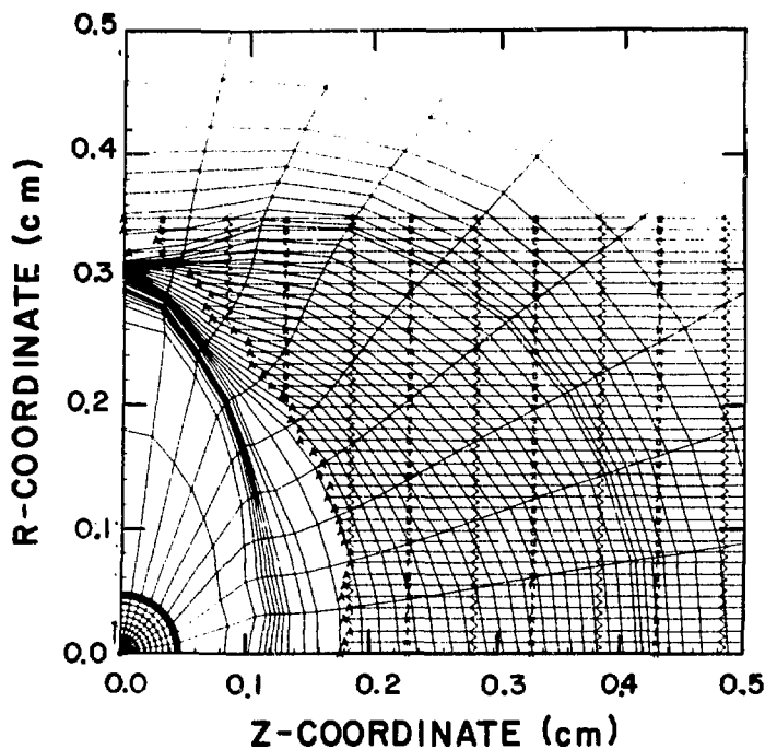
Fig. VIII-19. Lagrangian mesh with ion rays at 35 ns for the cylindrical beam case.
