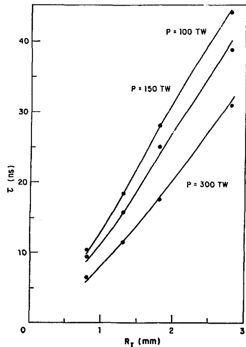
Fig. VIII-9. Collapse time vs initial inner radius for 200- \mu m-thick gold shells.
