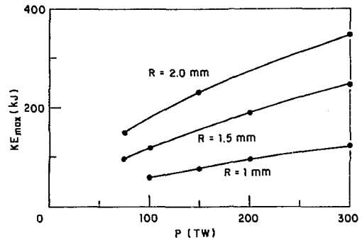
Fig. VIII-8. Maximum kinetic energy vs power for 200- \mu m-thick gold shells.
