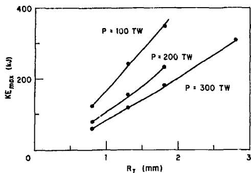
Fig. VIII-10. Maximum kinetic energy vs initial inner radius for 200- \mu m-thick gold shells.
