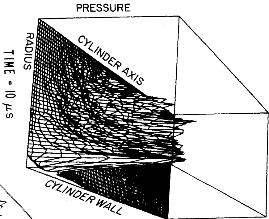
Fig. IX-11. The pressure wave and the low-temperature region inside reactor cavity.
