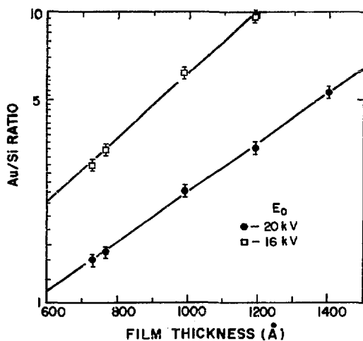
Fig. VI-7. X-ray peak ratioing calibration curve.
