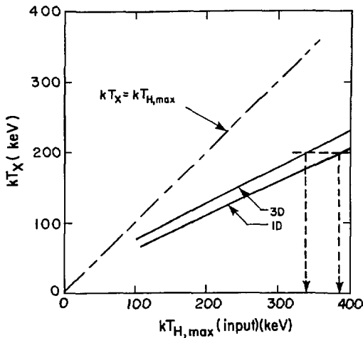
Fig. IV-9. Suprathermal x-ray temperature vs peak suprathermal electron temperature (LASNEX).
