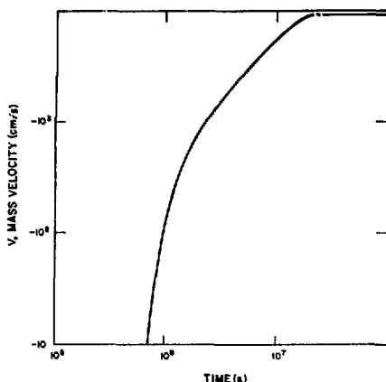
Fig. IX-6. The development of mass velocity associated with x-ray energy deposition ( S_0 = 5 \times 10^{17} erg/cm 2 ·s).
