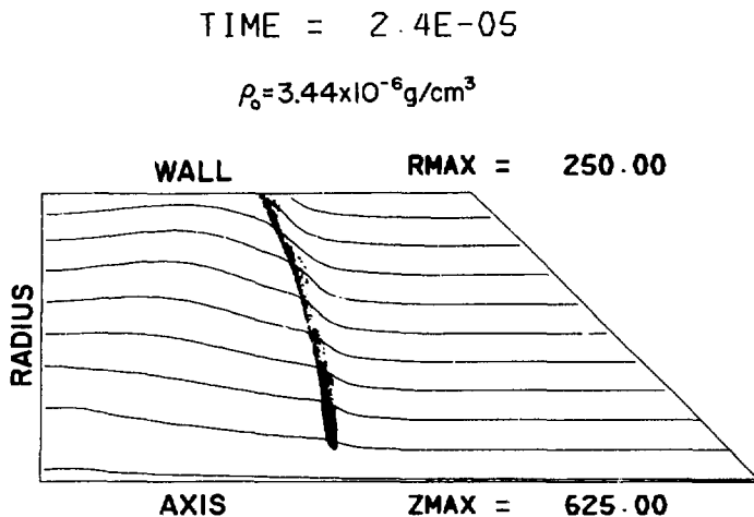
Fig. IX-9. Ion sheet in fluid density of 10^{17} \text{ atom/cm}^3 .
