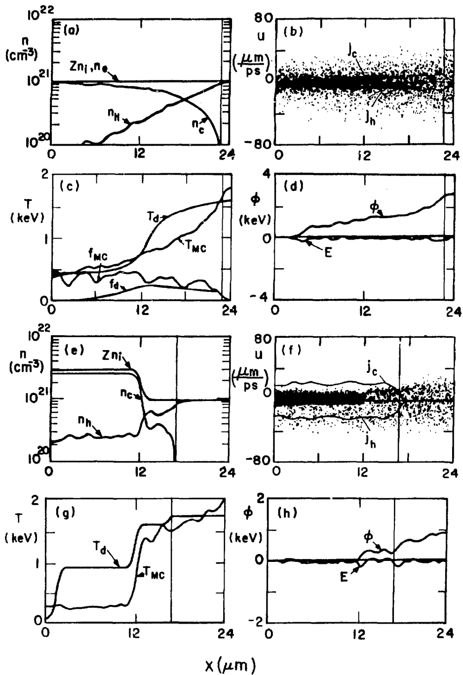
Fig. IV-6. An end-heated uniform plasma. (a)-(d). Transport through a density gradient. (e)-(h). j_{h,c} \approx 5 \times 10^{-21} n_{h,e} u_{h,e} ( u - \text{cm}^{-3}/\text{ps} ), E in arbitrary units.
