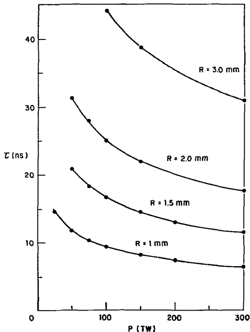
Fig. VIII-7. Collapse time vs power for 200- \mu m-thick gold shells.
