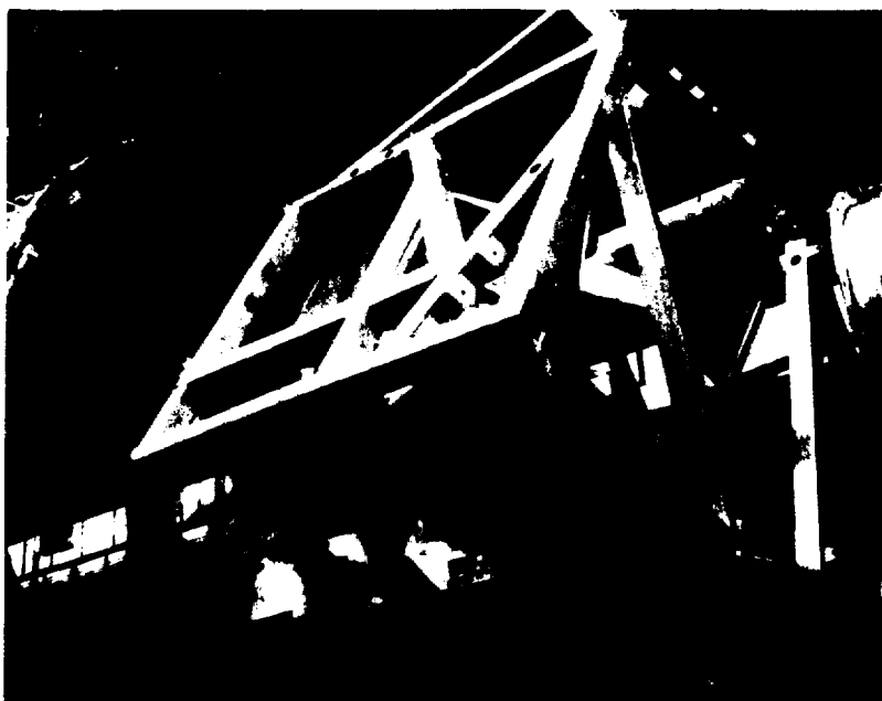
Fig. II-8. Antares target chamber and space frame.
