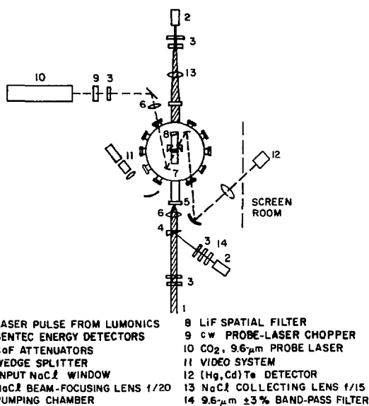
Fig. II-25. Experimental setup to investigate plasma formation.
