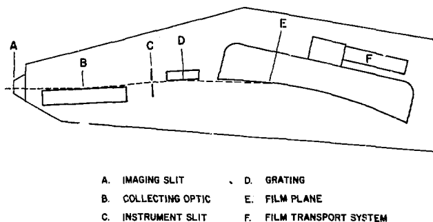
Fig. V-7. Grazing-incidence grating spectrograph.
