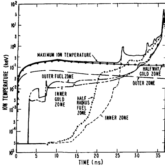
Fig. VIII-6. Plots of ion temperature vs time.
