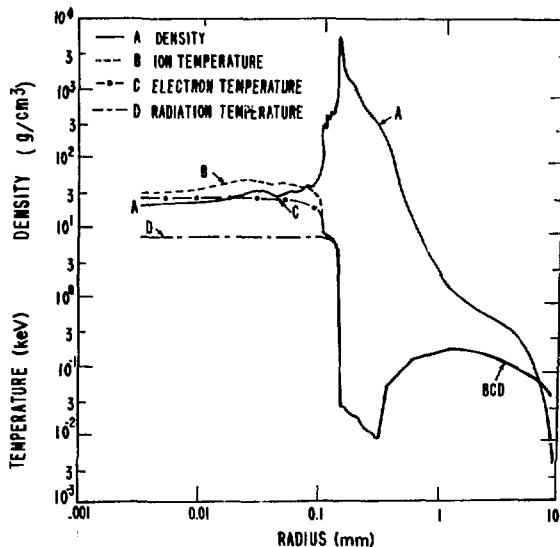
Fig. VIII-5. Temperature and density profiles of pellet near peak burn.
