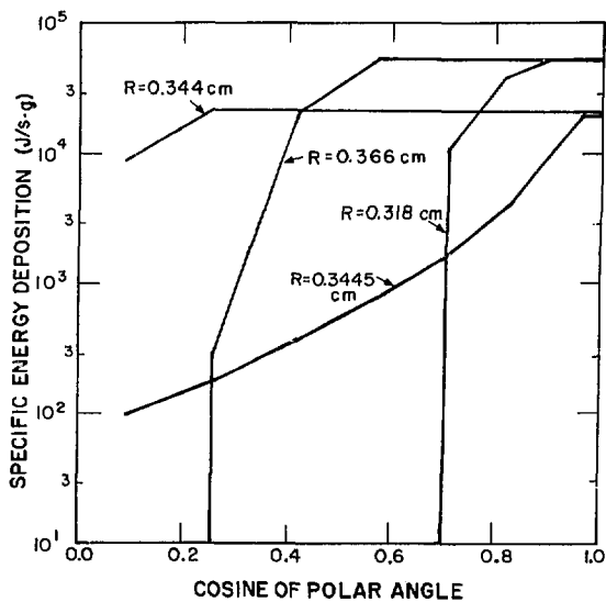
Fig. VIII-20. Plot of initial specific energy deposition as a function of the cosine of the polar angle for different radii for the cylindrical beam case.
