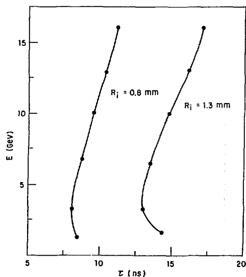
Fig. VIII-13. Ion particle energy vs collapse time.
