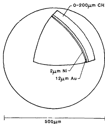
Fig. III-12. Target configuration for hot-electron deposition experiment.
