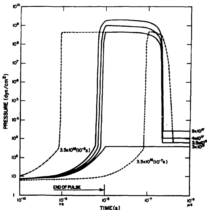
Fig. IX-5. Pressure increase in the 1-mm-thick layer adjacent to the free surface induced by x-ray energy deposition (source strengths in \text{erg/cm}^2 \cdot \text{s} ).
