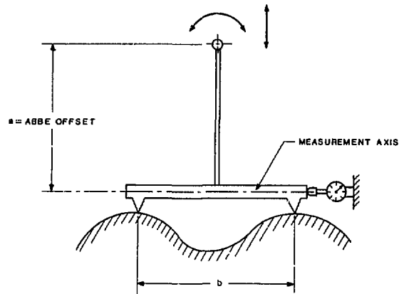
Fig. II-13. Abbe offset error description.
