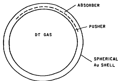
Fig. VIII-3. Single-shell gold target.
