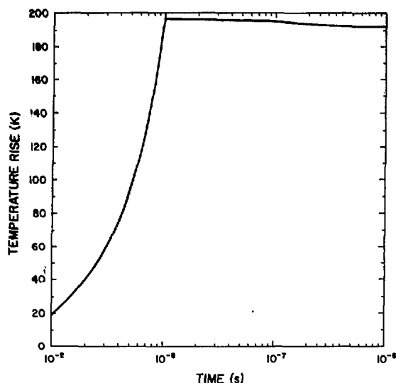
Fig. IX-4. Temperature rise in the 1-mm-thick layer adjacent to the free surface induced by x-ray energy deposition ( S_0 = 3.5 \times 10^{17} \text{ erg/cm}^2 \cdot \text{s} ).
