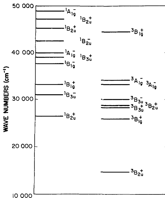
Fig. VII-3. Electronic energy level structure for anthracene.
