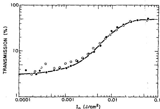
Fig. VII-6. Saturable absorption in 1.25 \times 10^{-5} molecules/cm 2 anthracene in n-hexane in the absence of O_2 . Theory (solid line), data set 1 (closed circles), and data set 2 (open circles.)
