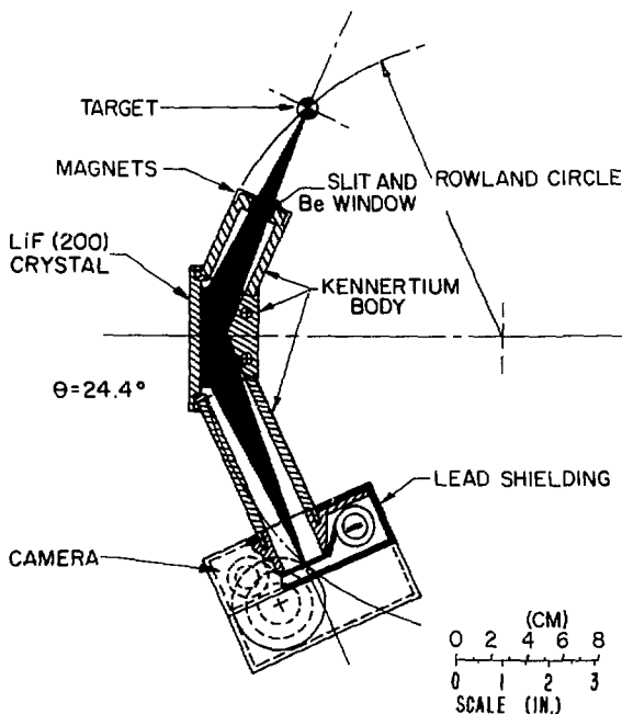
Fig. V-12. Curved-crystal spectrograph.
