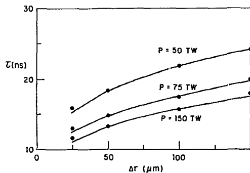
Fig. VIII-12. Collapse time vs shell thickness for 1.5-mm-radius targets.
