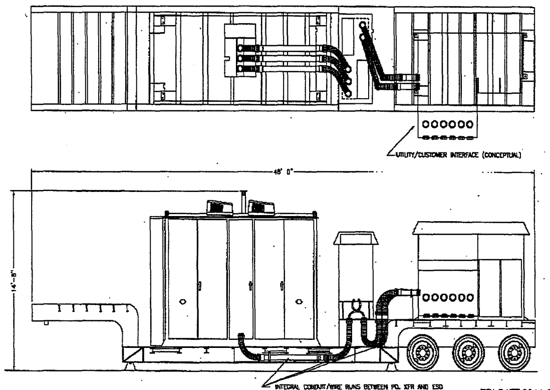
Figure 2-1. Final TBESS Trailer Equipment Layout.
