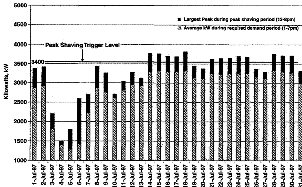
Figure 2-16. Largest Peak Shaving Period for the Month of July.
