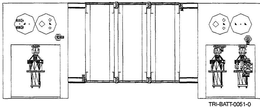
Figure 2-7. Top View Schematic of ZBB 50-kWh Battery Module (module = 98" length \times 38" width \times 34" height).
