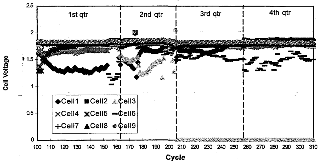
Figure 3-5. Cell Voltages at EOD for the Yuasa-Exide Battery for FY97.
