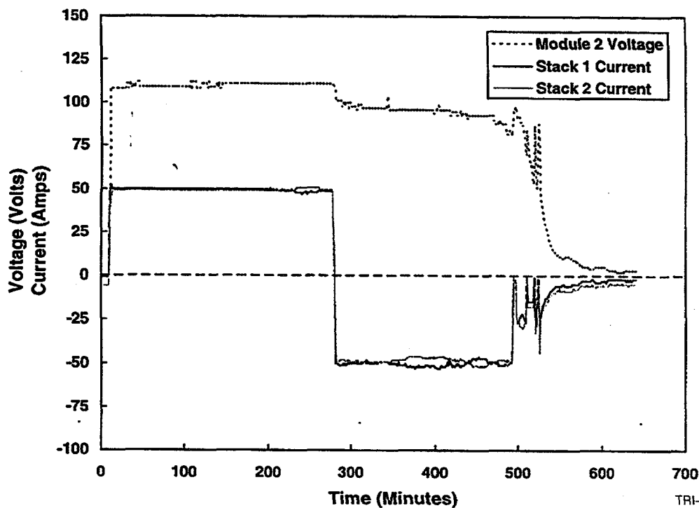
Figure 2-25. Voltage and Current Profiles for Module 2 of the ZBB 100-kWh Zinc/Bromine Battery During a Baseline Cycle.
