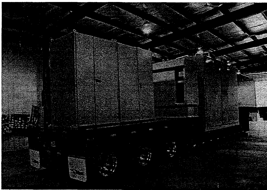
Figure 2-2. TBESS with Major Components Mounted in Place.
