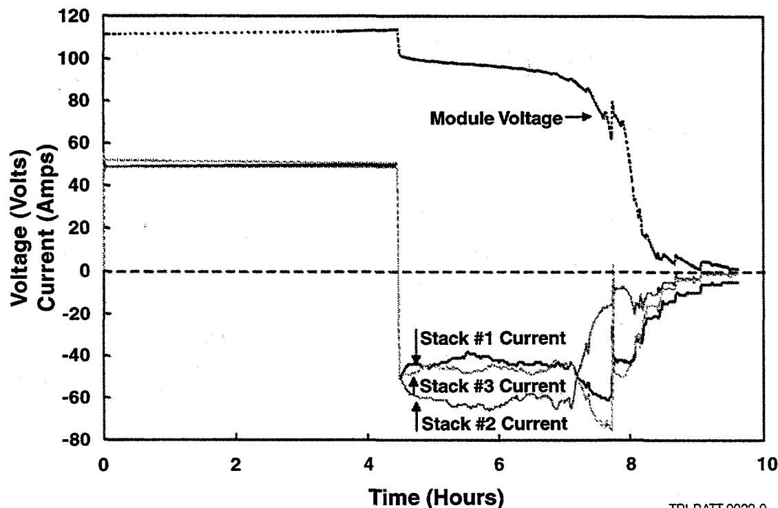
Figure 2-9. 50-kWh Module Data Collection Profiles.
