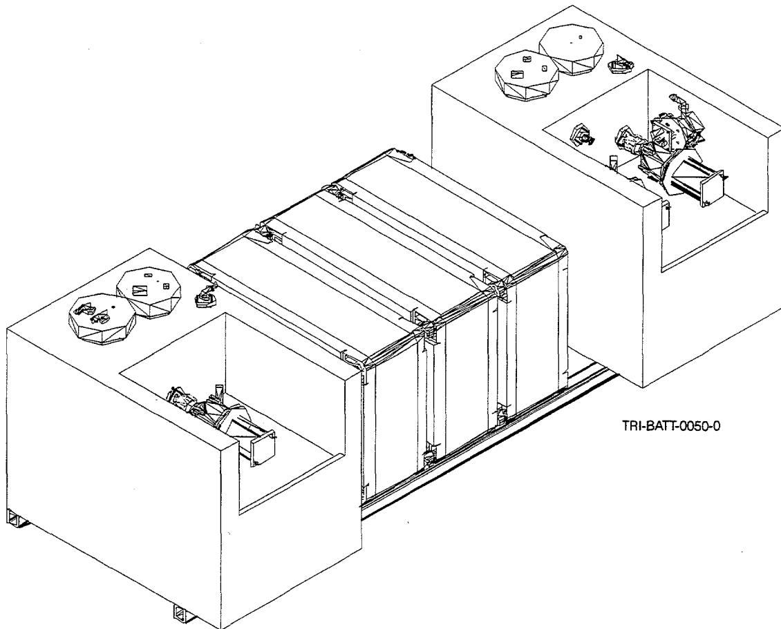
Figure 2-6. Left View Schematic of ZBB 50-kWh Battery Module (module = 98" length \times 38" width \times 34" height).
