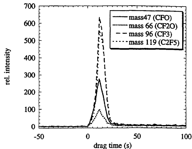
Figure 10: Mass spectrum for CH x sample.
