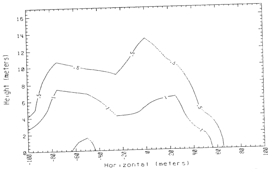
Time = 320 sec. Data avg. over 5. sec. 150m Row Falcon 4 1987
