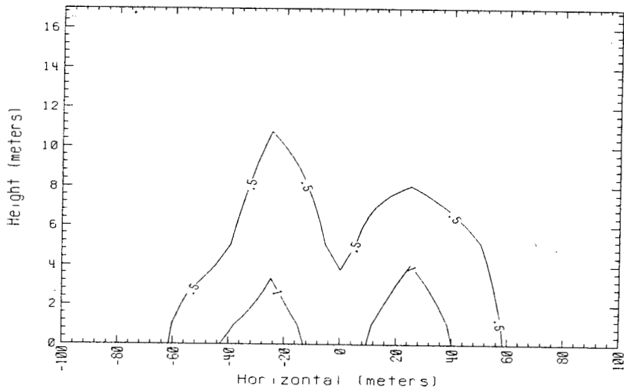
Time = 120 sec. Data avg. over 5. sec. 150m Row Falcon 4 1987
