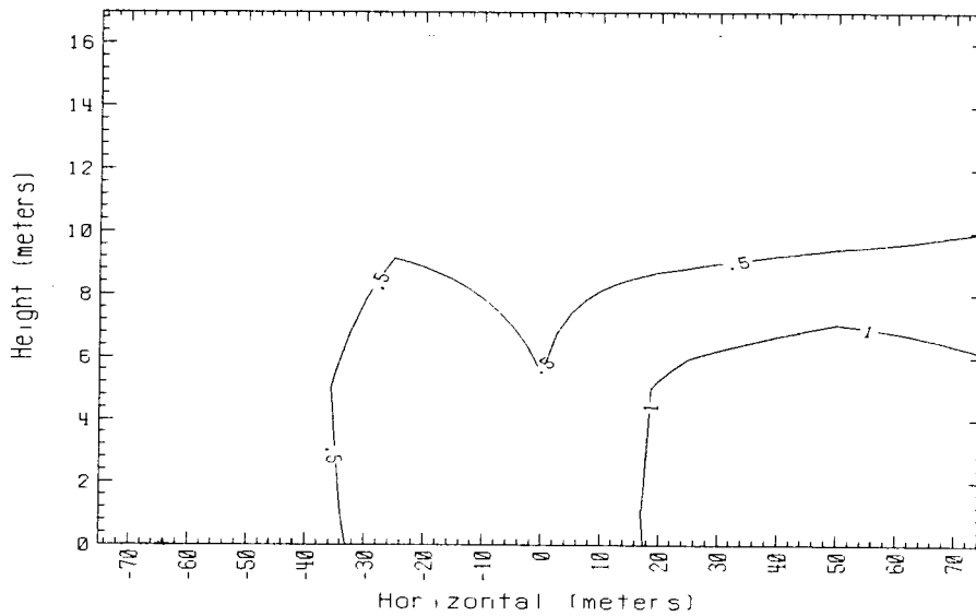
Time = 120 sec. Data avg. over 5. sec. 150m Row Falcon 3 1987
