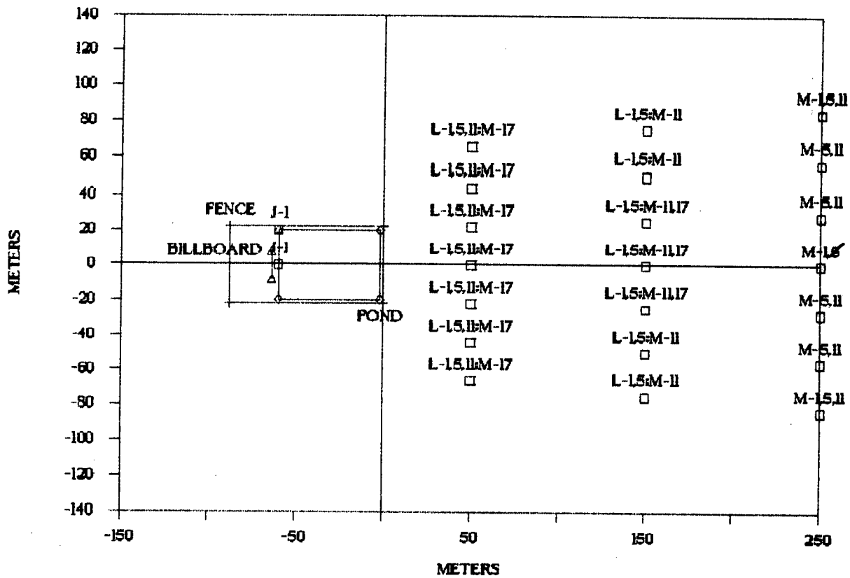
Figure 9. Falcon 1 gas array.
