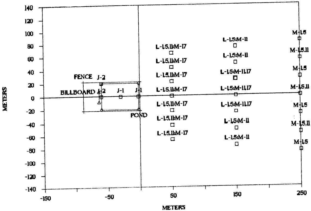
Figure 11. Falcon 3 gas array.
