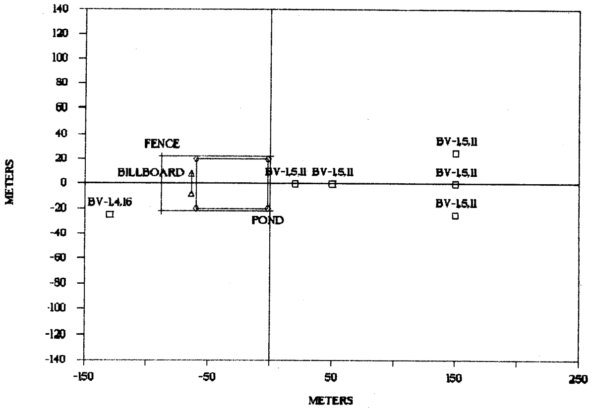
Figure 1. Falcon Series bivane array.
