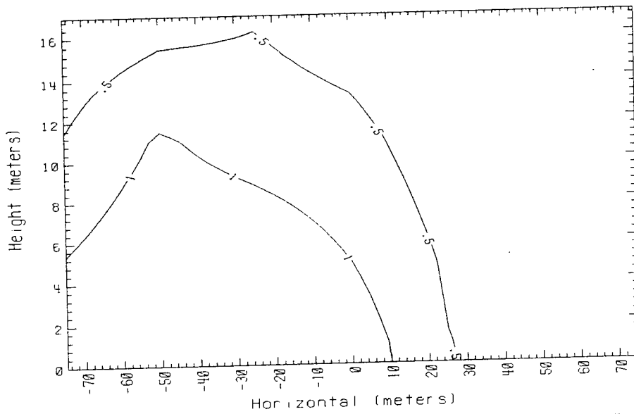
Time = 380 sec. Data avg. over 5. sec. 150m Row Falcon 3 1987
