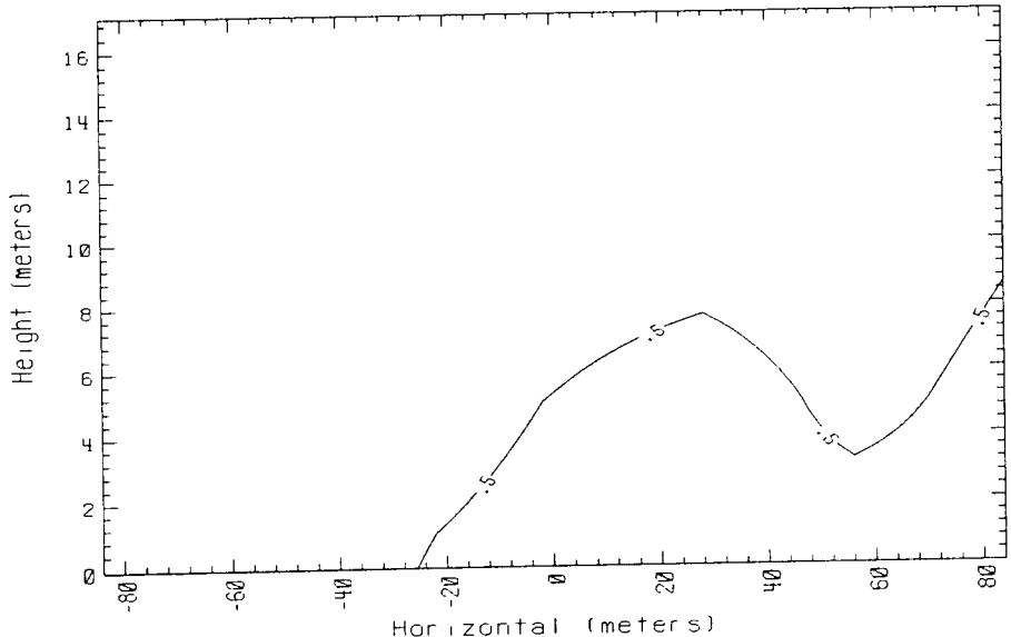
Time = 290 sec. Data avg. over 5. sec. 250m Row Falcon 2 1987
