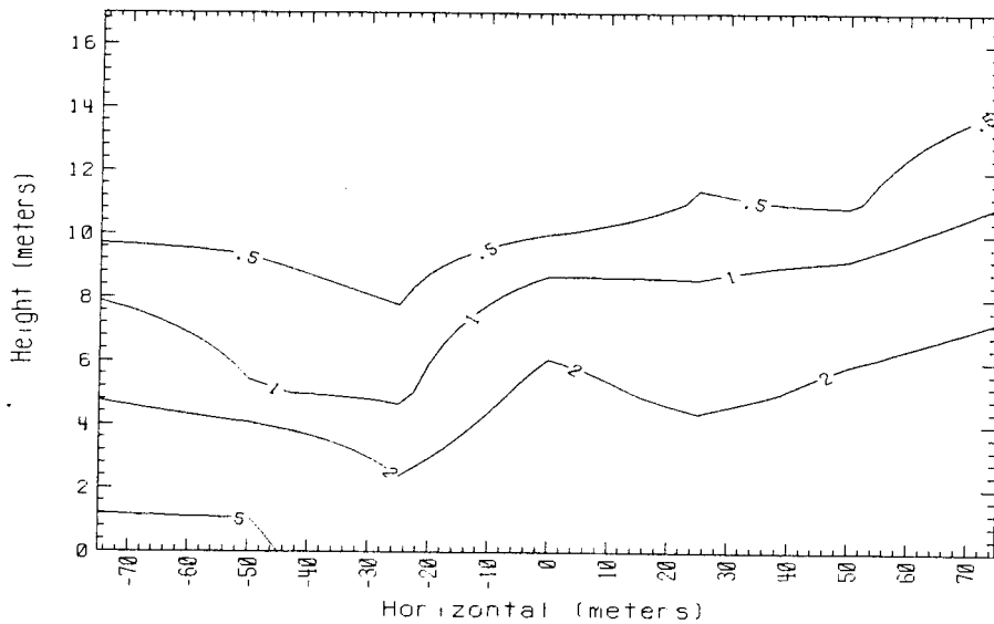
Time = 200 sec. Data avg. over 5. sec. 150m Row Falcon 3 1987
