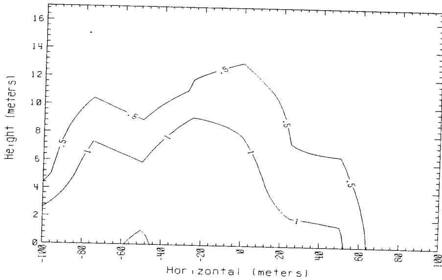
Time = 280 sec. Data avg. over 5. sec. 150m Row Falcon 4 1987
