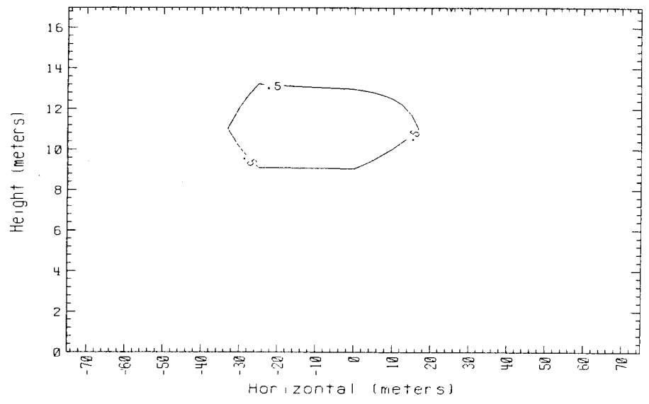
Time = 750 sec. Data avg. over 5. sec. 150m Row Falcon 3 1987
