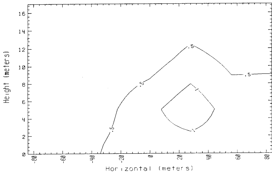
Time = 270 sec. Data avg. over 5. sec. 250m Row Falcon 2 1987
