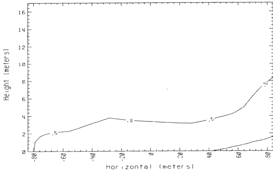
Time = 180 sec. Data avg. over 5. sec. 250m Row Falcon 2 1987
