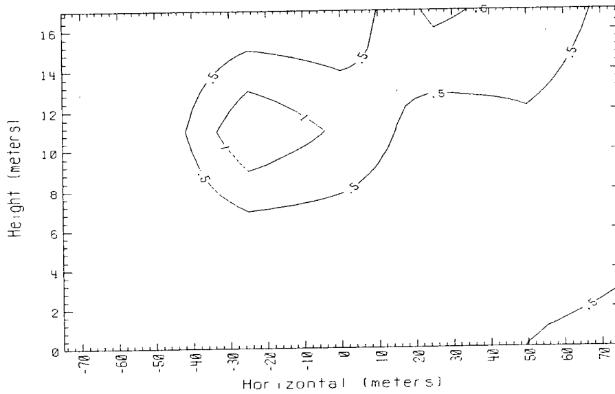
Time = 480 sec. Data avg. over 5. sec. 150m Row Falcon 3 1987
