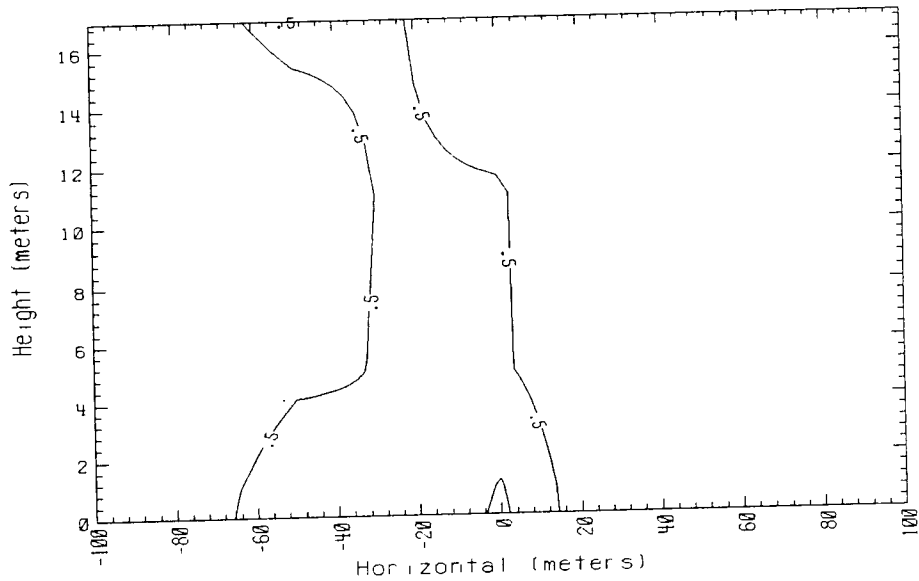
Time = 460 sec. Data avg. over 5. sec. 150m Row Falcon 4 1987
