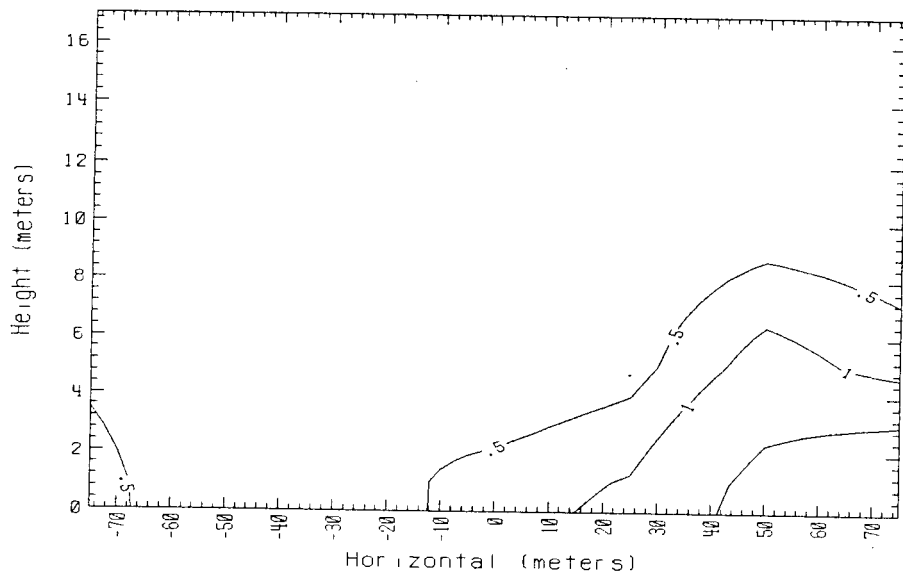
Time = 340 sec. Data avg. over 5. sec. 150m Row Falcon 1 1987
