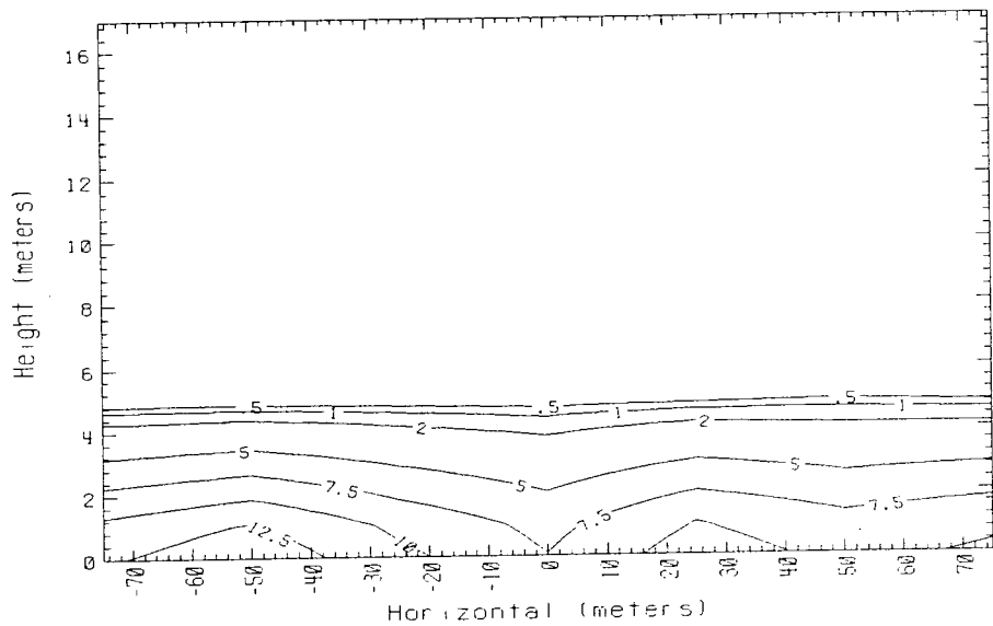
Time = 160 sec. Data avg. over 5. sec. 150m Row Falcon 1 1987
