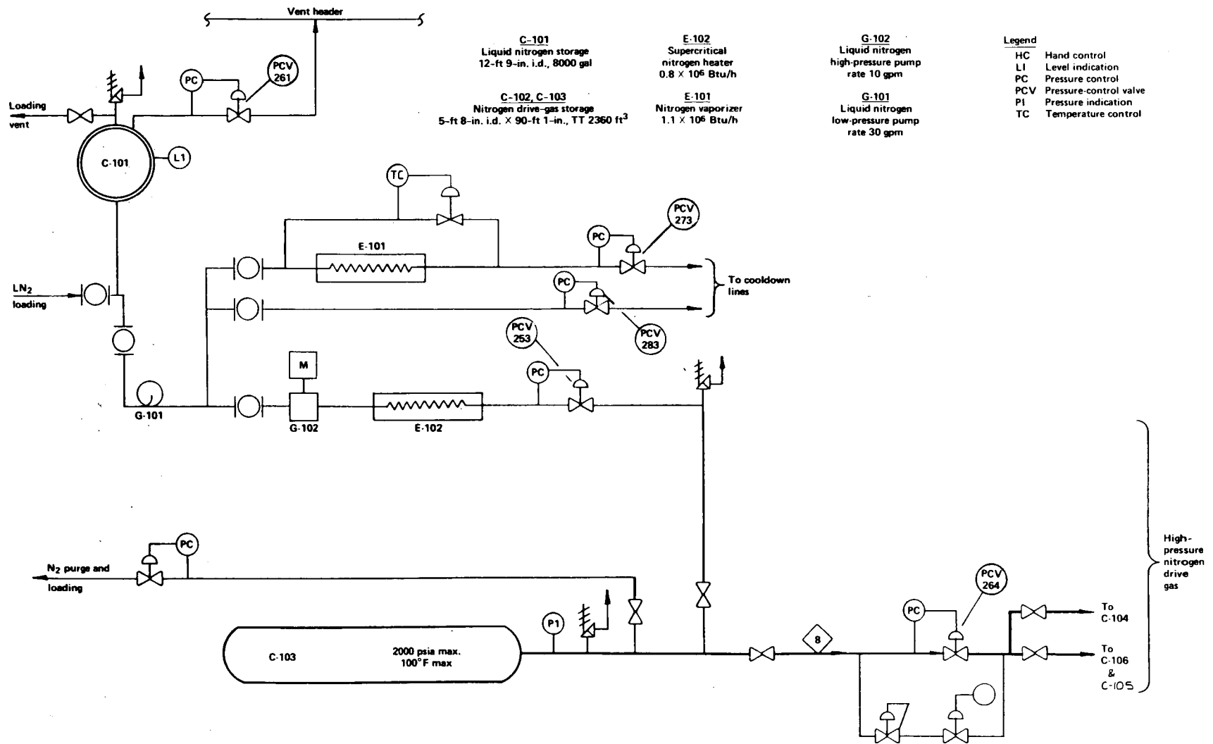
Figure 14. Nitrogen storage and supply system.
