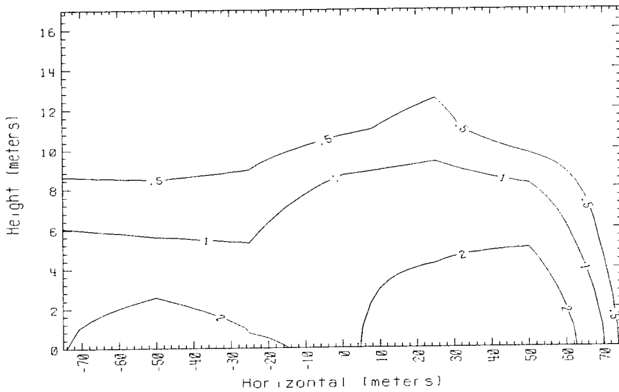
Time = 320 sec. Data avg. over 5. sec. 150m Row Falcon 3 1987
