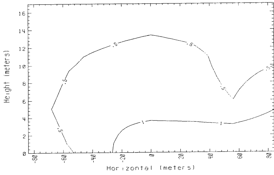
Time = 220 sec. Data avg. over 5. sec. 250m Row Falcon 2 1987
