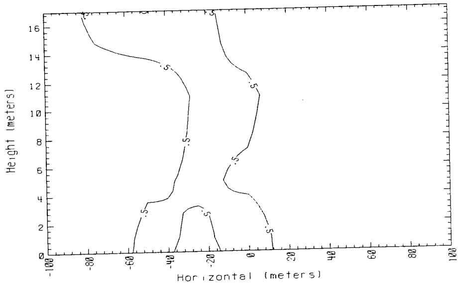
Time = 480 sec. Data avg. over 5. sec. 150m Row Falcon 4 1987
