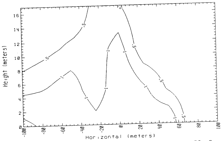
Time = 380 sec. Data avg. over 5. sec. 150m Row Falcon 4 1987
