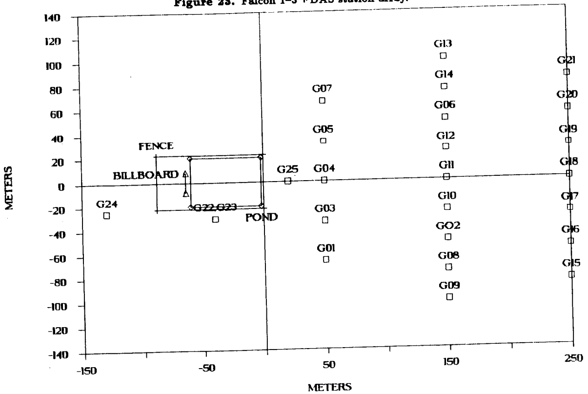
Figure 24. Falcon 4-5 FDAS station array.
