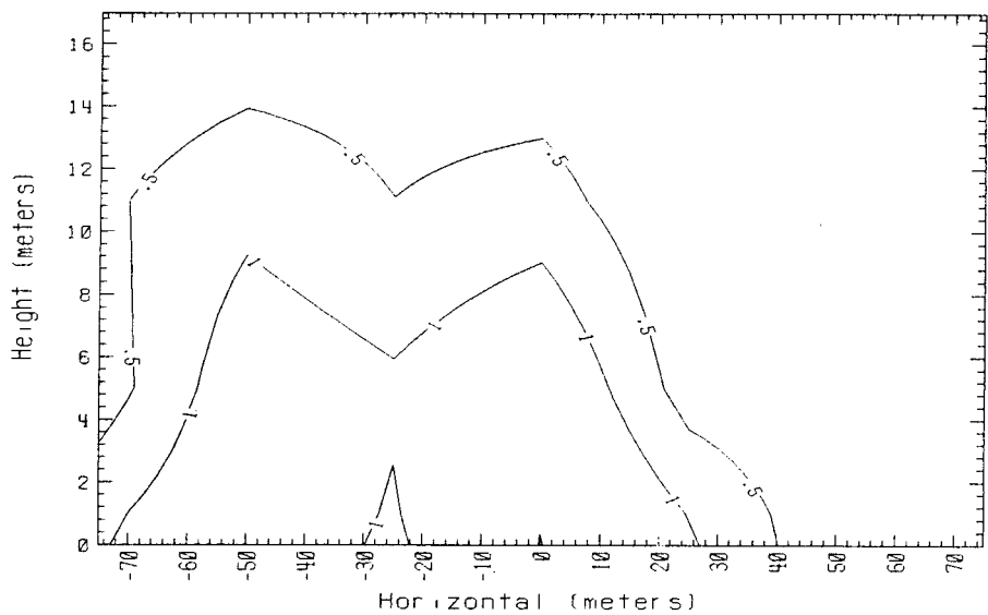
Time = 360 sec. Data avg. over 5. sec. 150m Row Falcon 3 1987
