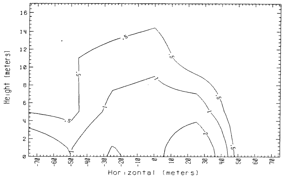
Time = 340 sec. Data avg. over 5. sec. 150m Row Falcon 3 1987
