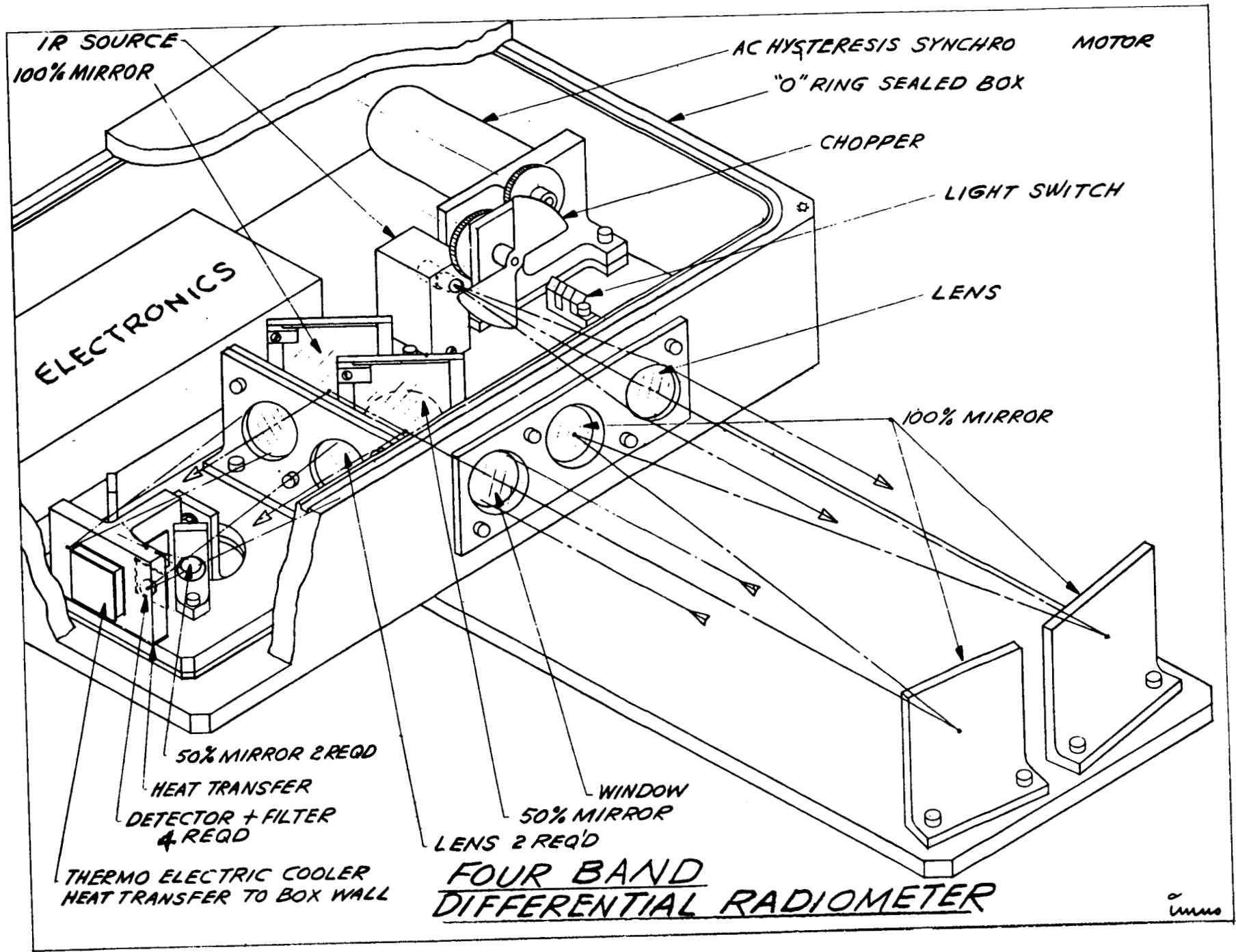
Figure 20. Pictorial sketch of the JPL-IR sensor.
