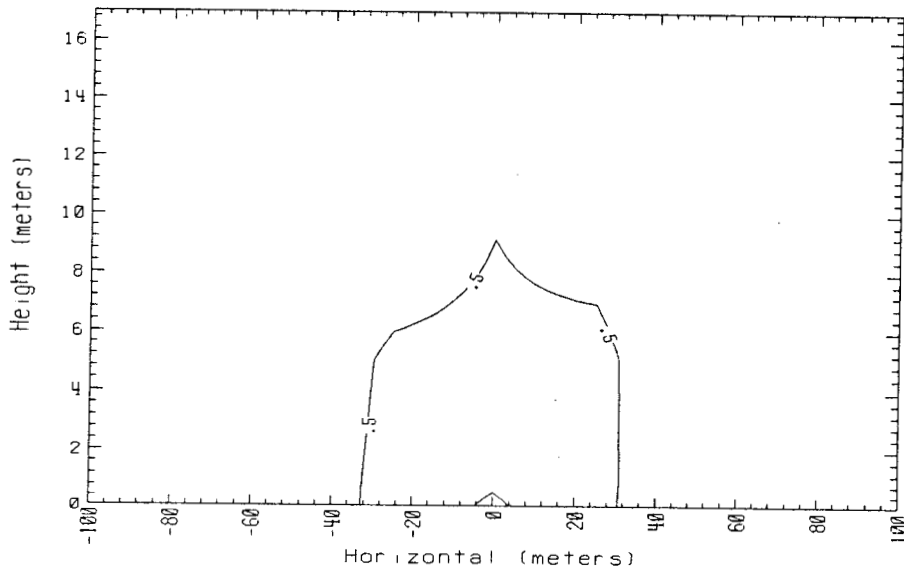
Time = 100 sec. Data avg. over 5. sec. 150m Row Falcon 4 1987
