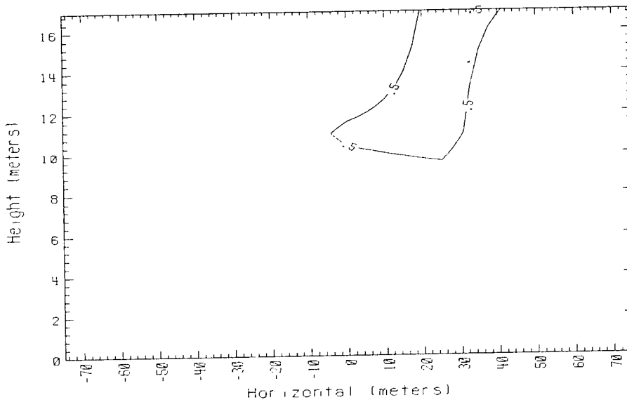
Time = 640 sec. Data avg. over 5. sec. 150m Row Falcon 3 1987
