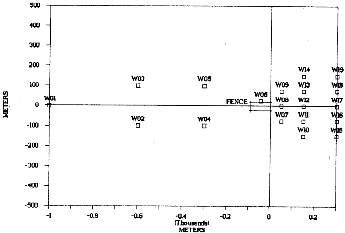
Figure 2. Falcon Series windfield array.
