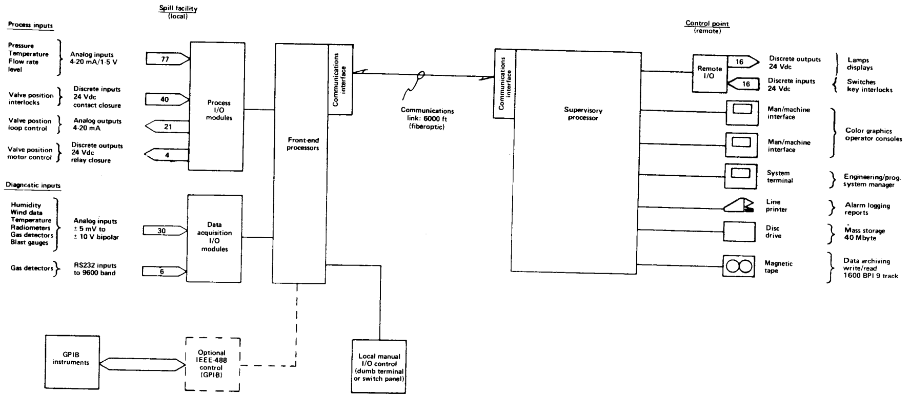
Figure 18. Command, control, and data acquisition system.
