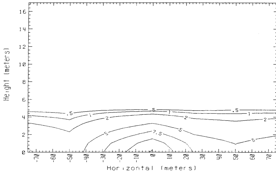
Time = 120 sec. Data avg. over 5. sec. 150m Row Falcon 1 1987
