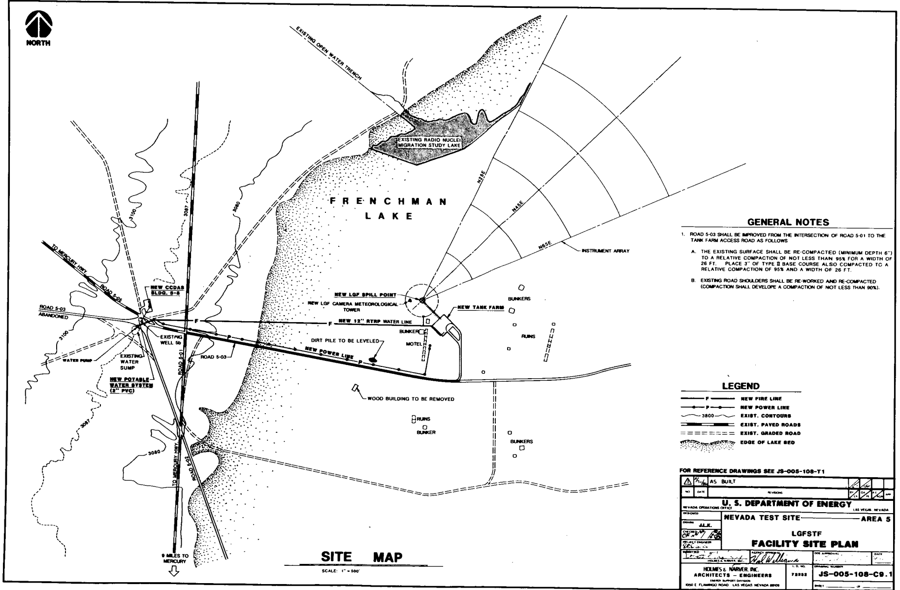
Figure 13. Site plan of LGF Spill Test Facility.
