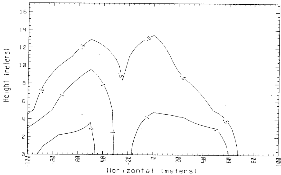
Time = 360 sec. Data avg. over 5. sec. 150m Row Falcon 4 1987
