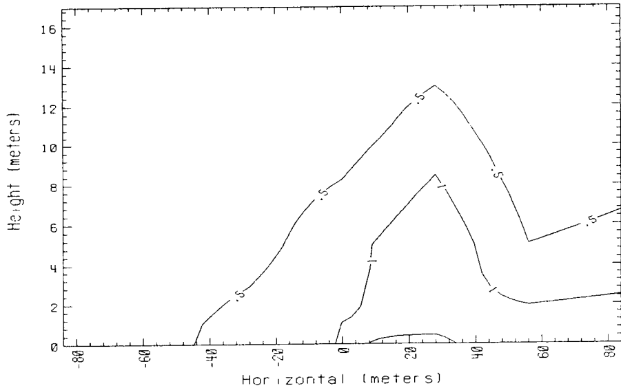
Time • 260 sec. Data avg. over 5. sec. 250m Row Falcon 2 1987
