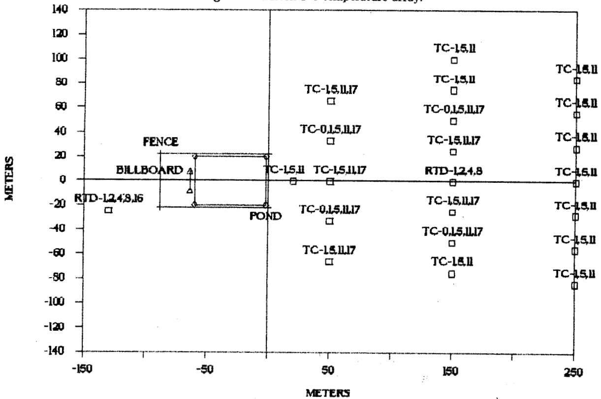
Figure 6. Falcon 4-5 temperature array.
