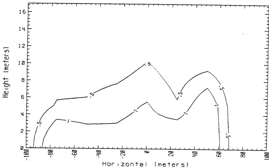
Time = 200 sec. Data avg. over 5. sec. 150m Row Falcon 4 1987
