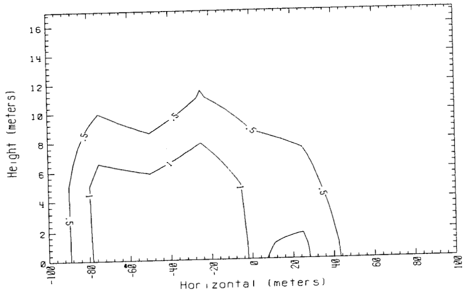
Time - 140 sec. Data avg. over 5. sec. 150m Row Falcon 4 1987
