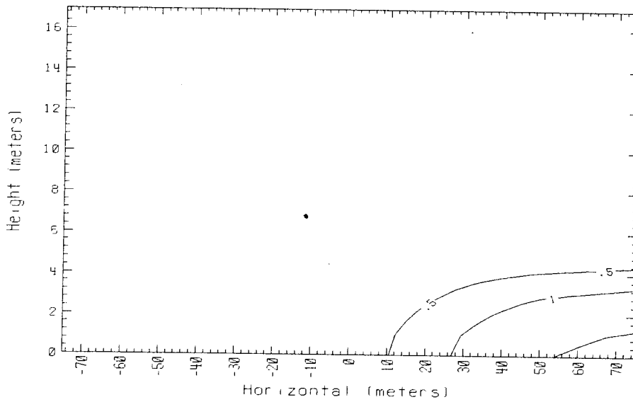
Time = 440 sec. Data avg. over 5. sec. 150m Row Falcon 1 1987
