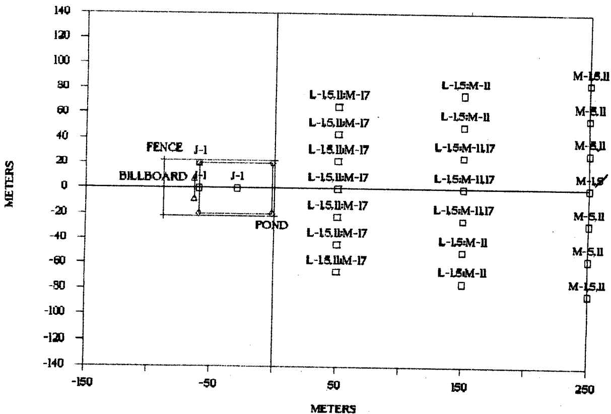
Figure 10. Falcon 2 gas array.
