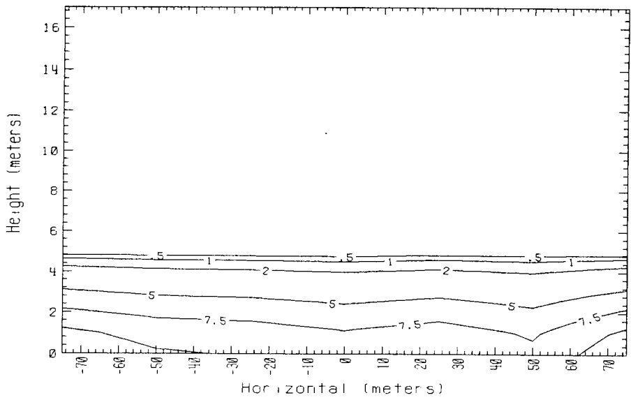
Time = 180 sec. Data avg. over 5. sec. 150m Row Falcon 1 1987
