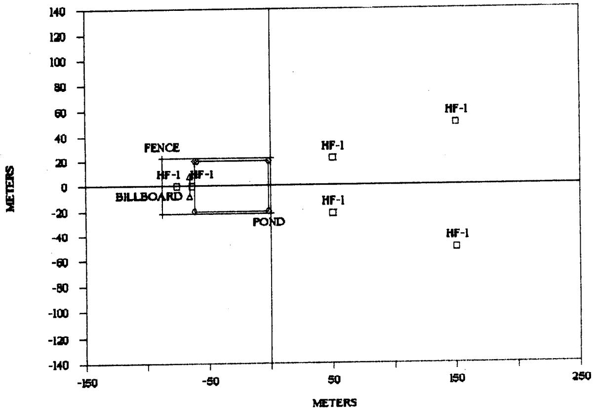
Figure 7. Falcon Series heat flux array.
