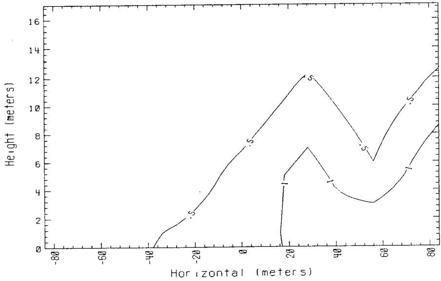
Time • 250 sec. Data avg. over 5. sec. 250m Row Falcon 2 1987
