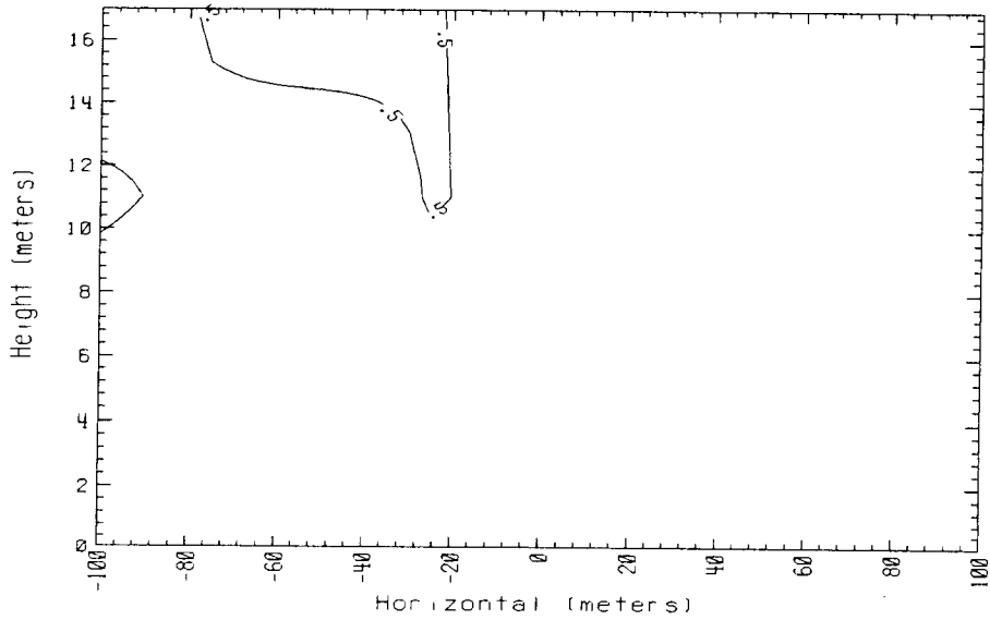
Time = 580 sec. Data avg. over 5. sec. 150m Row Falcon 4 1987
