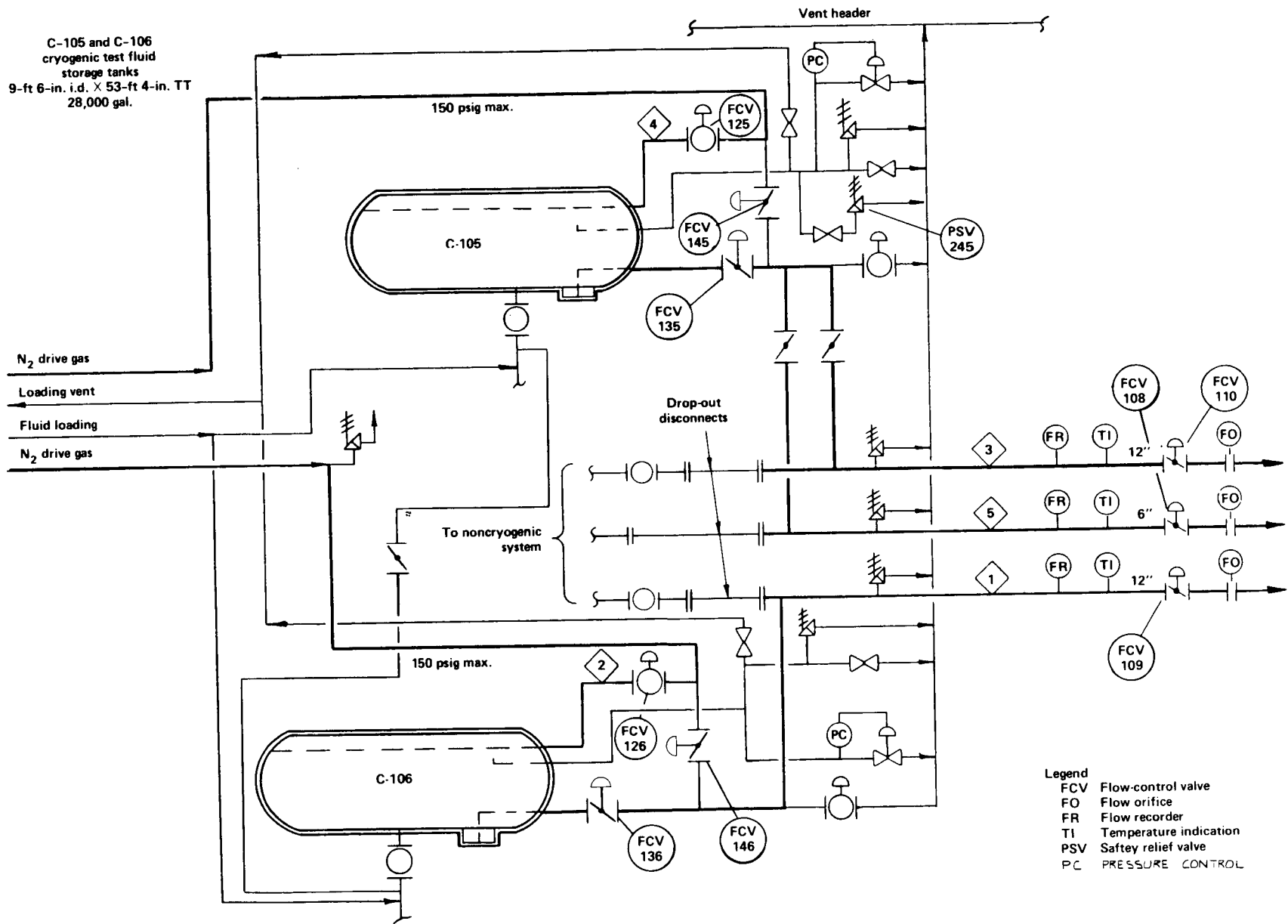
Figure 15. Cryogenic spill system.
