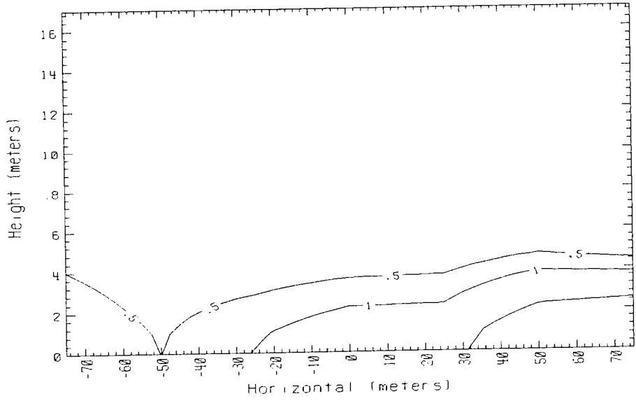
Time = 320 sec. Data avg. over 5. sec. 150m Row Falcon 1 1987
