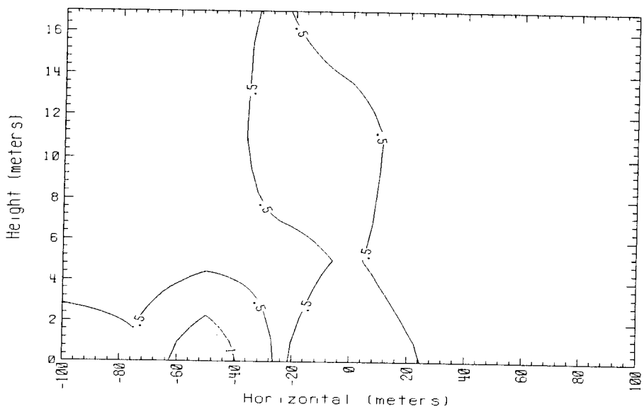
Time = 420 sec. Data avg. over 5. sec. 150m Row Falcon 4 1987
