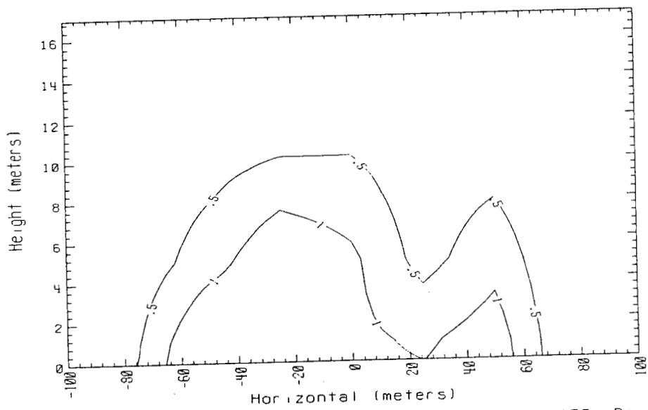
Time - 160 sec. Data avg. over 5. sec. 150m Row Falcon 4 1987
