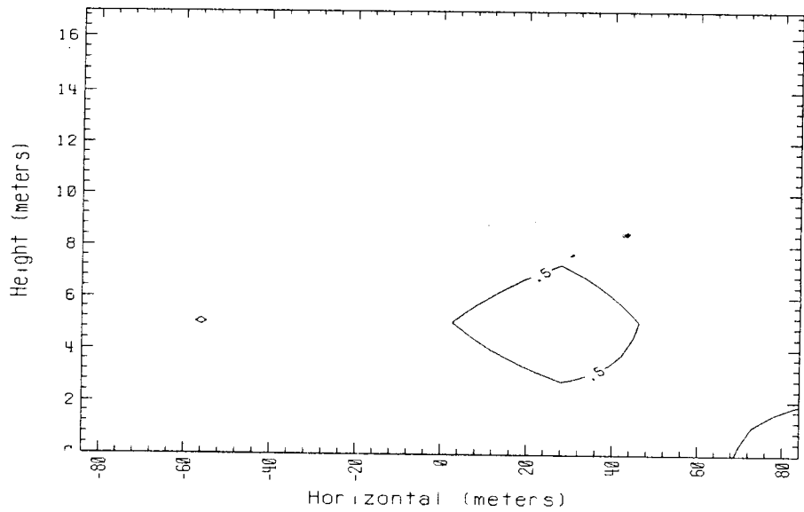
Time = 310 sec. Data avg. over 5. sec. 250m Row Falcon 2 1987
