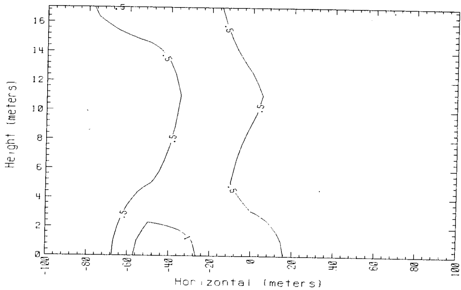
Time = 440 sec. Data avg. over 5. sec. 150m Row Falcon 4 1987
