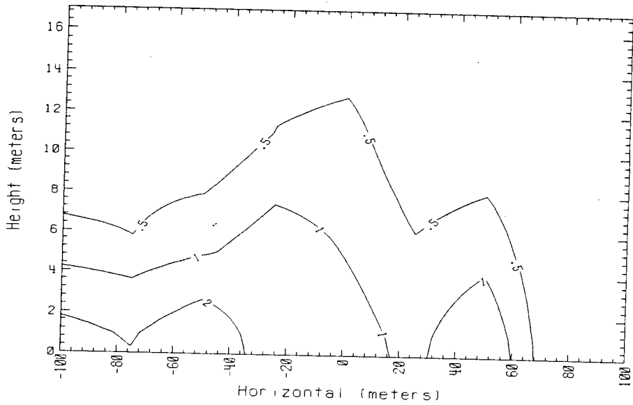
Time = 260 sec. Data avg. over 5. sec. 150m Row Falcon 4 1987
