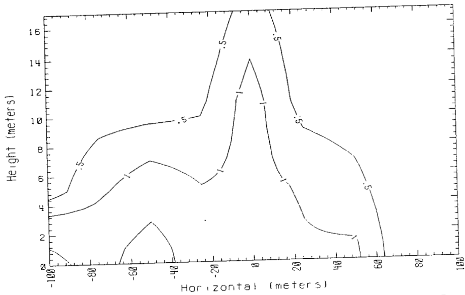
Time = 300 sec. Data avg. over 5. sec. 150m Row Falcon 4 1987
