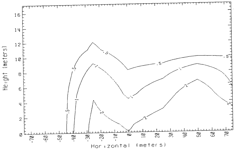
Time = 140 sec. Data avg. over 5. sec. 150m Row Falcon 3 1987
