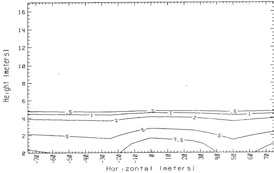
Time = 220 sec. Data avg. over 5. sec. 150m Row Falcon 1 1987
