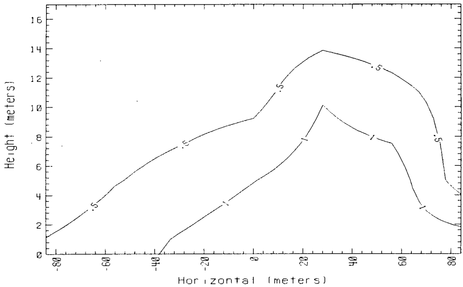
Time = 240 sec. Data avg. over 5. sec. 250m Row Falcon 2 1987
