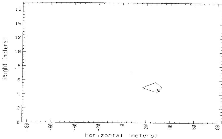
Time = 320 sec. Data avg. over 5. sec. 250m Row Falcon 2 1987
