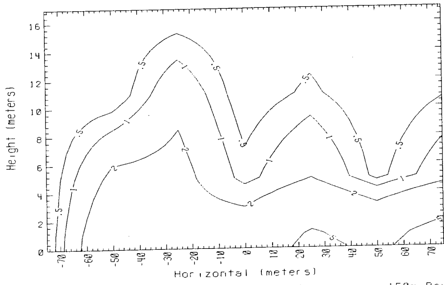
Time = 160 sec. Data avg. over 5. sec. 150m Row Falcon 3 1987
