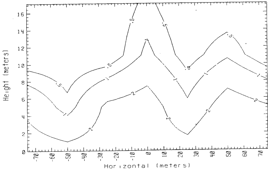
Time = 300 sec. Data avg. over 5. sec. 150m Row Falcon 3 1987
