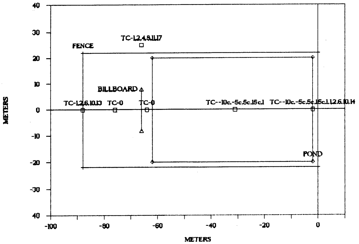
Figure 3. Falcon 1-2 spill area temperature array.
