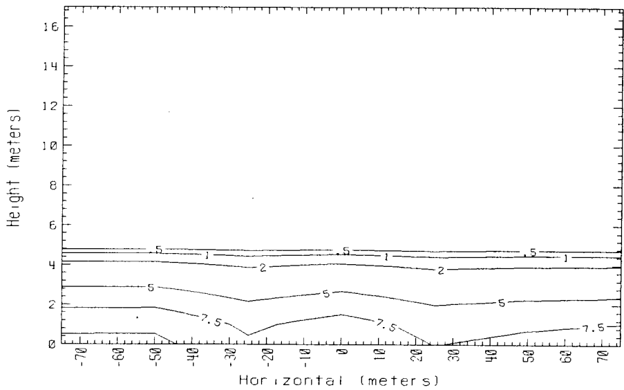
Time = 200 sec. Data avg. over 5. sec. 150m Row Falcon 1 1987
