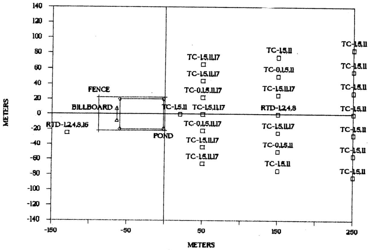
Figure 5. Falcon 1-3 temperature array.
