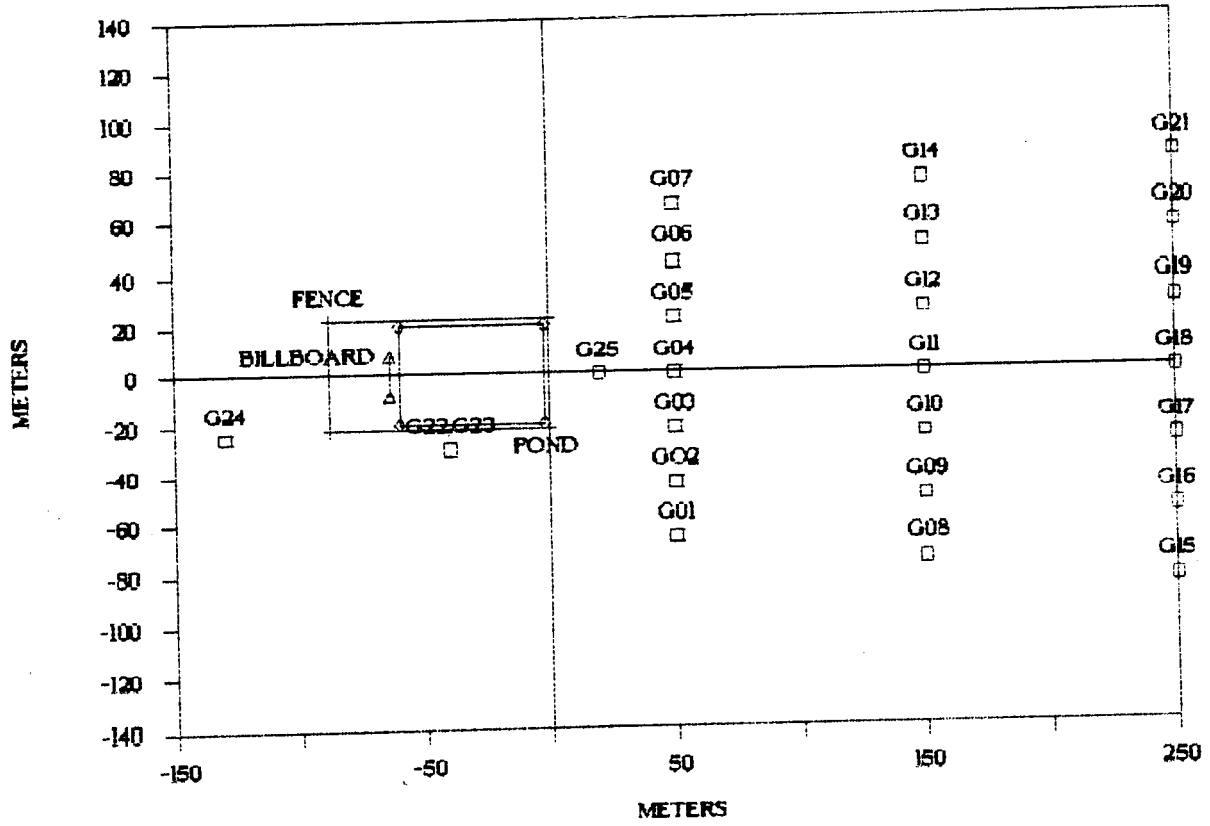
Figure 23. Falcon 1-3 FDAS station array.
