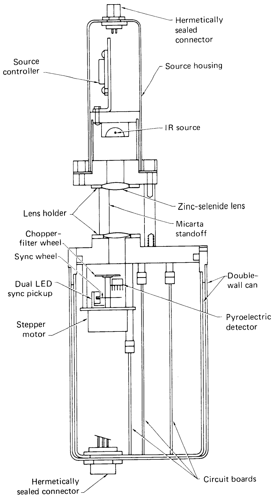
Figure 19. Cross section of the LLNL-IR sensor.
