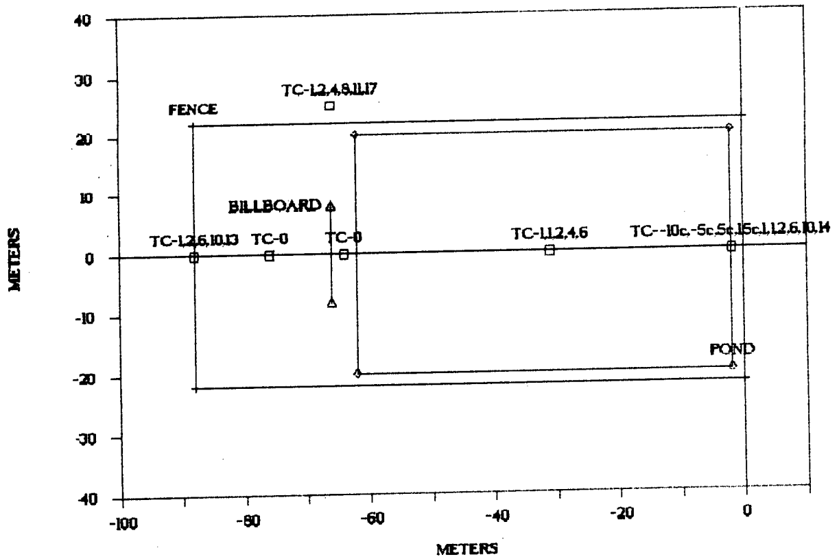
Figure 4. Falcon 3-5 spill area temperature array.
