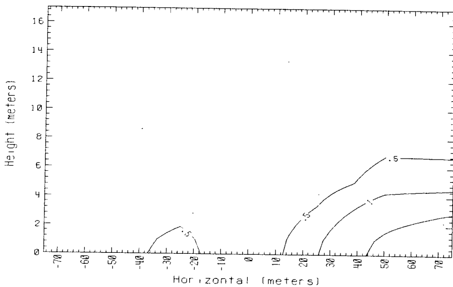
Time = 360 sec. Data avg. over 5. sec. 150m Row Falcon 1 1987
