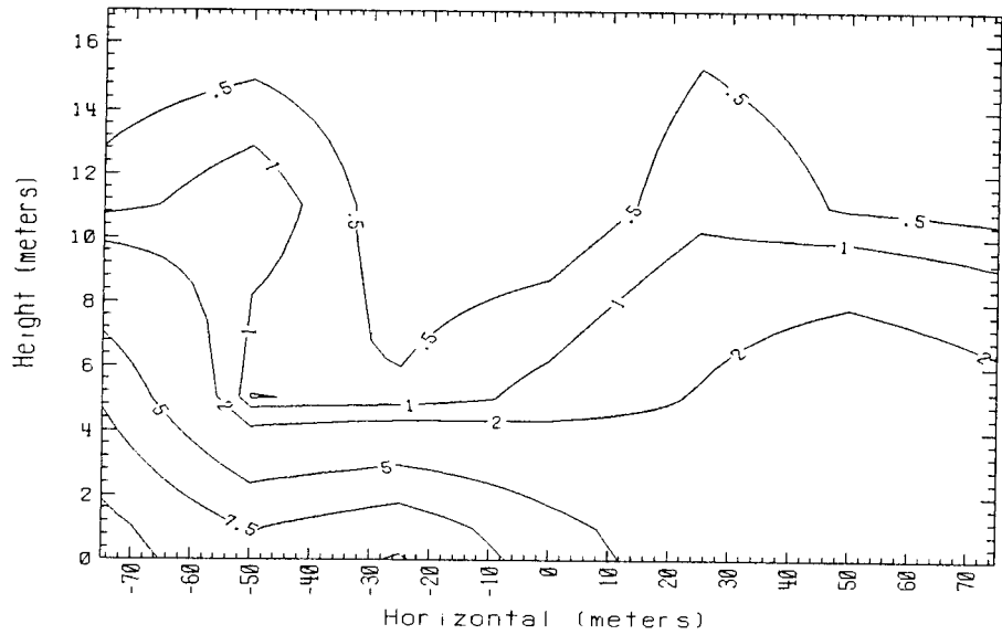
Time = 180 sec. Data avg. over 5. sec. 150m Row Falcon 3 1987
