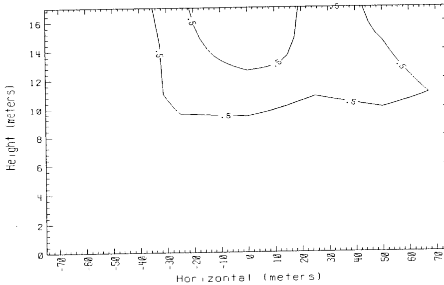
Time = 800 sec. Data avg. over 5. sec. 150m Row Falcon 3 1987
