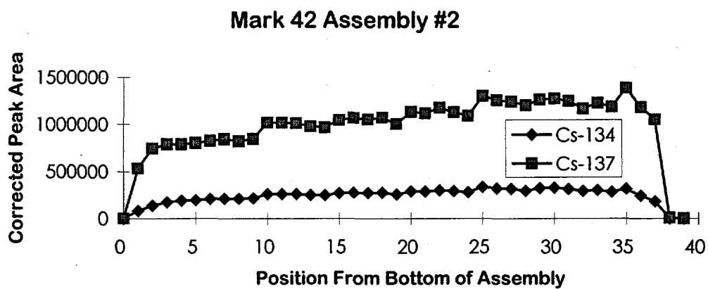
Figure 3. Corrected peak area counts for ^{134}\text{Cs} at 605 keV and ^{137}\text{Cs} - ^{137m}\text{Ba} 662 keV as measured on 15-April-92
