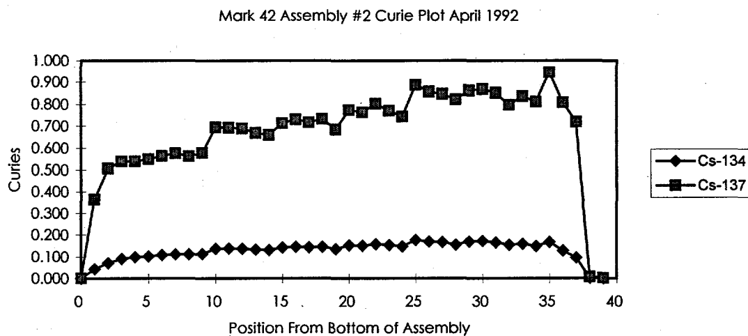
Figure 4. Curie plot of ^{134}\text{Cs} and ^{137}\text{Cs} - ^{137m}\text{Ba} as measured on 15-April-92
