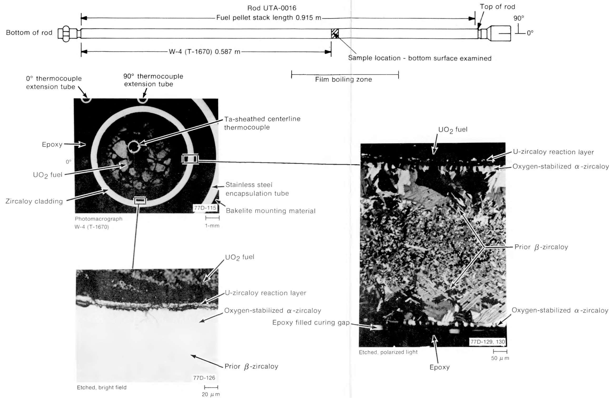
Fig. D-33 Transverse section (W-4) of Rod UTA-0016 (0.587 m) showing cladding microstructure.
