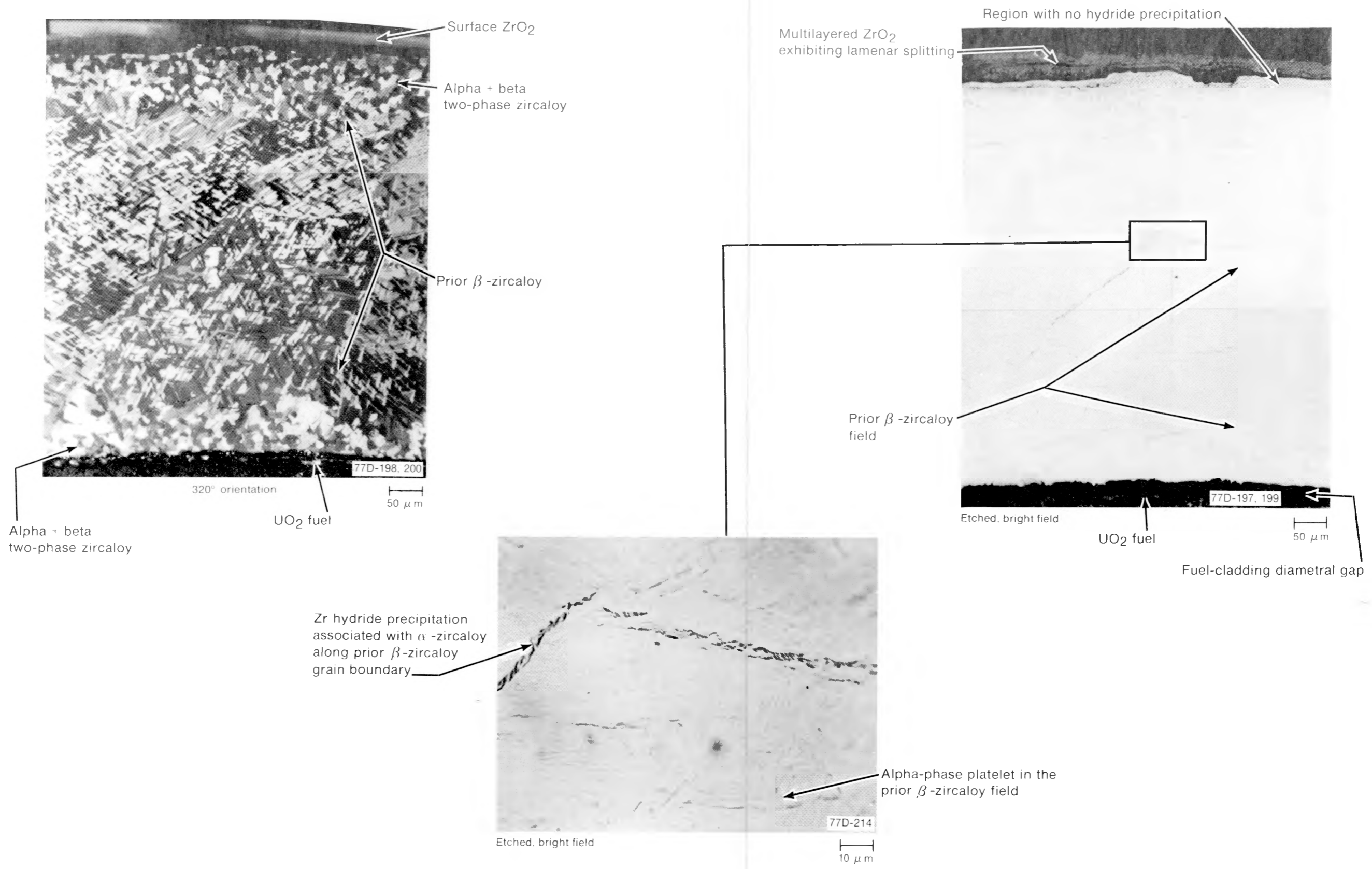
Fig. D-56 Hydride precipitation at 0.686-m and 320° circumferential orientation in Sample X-1 of Rod UTA-0015.
