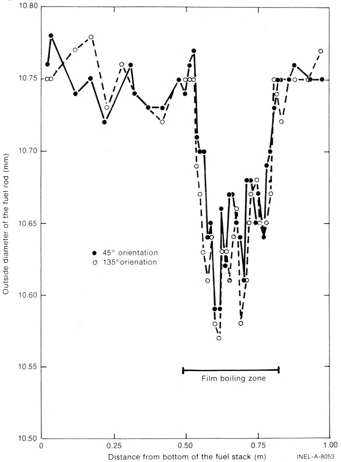
Fig. 23 Diametral measurements of collapse for Rod UTA-0016.
