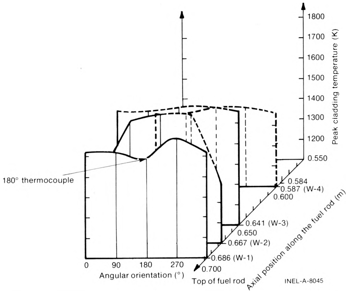
Fig. 15 Isometric plot of the modified BUILD5 peak cladding temperature as a function of angular orientation and axial position for Rod UTA-0016.
