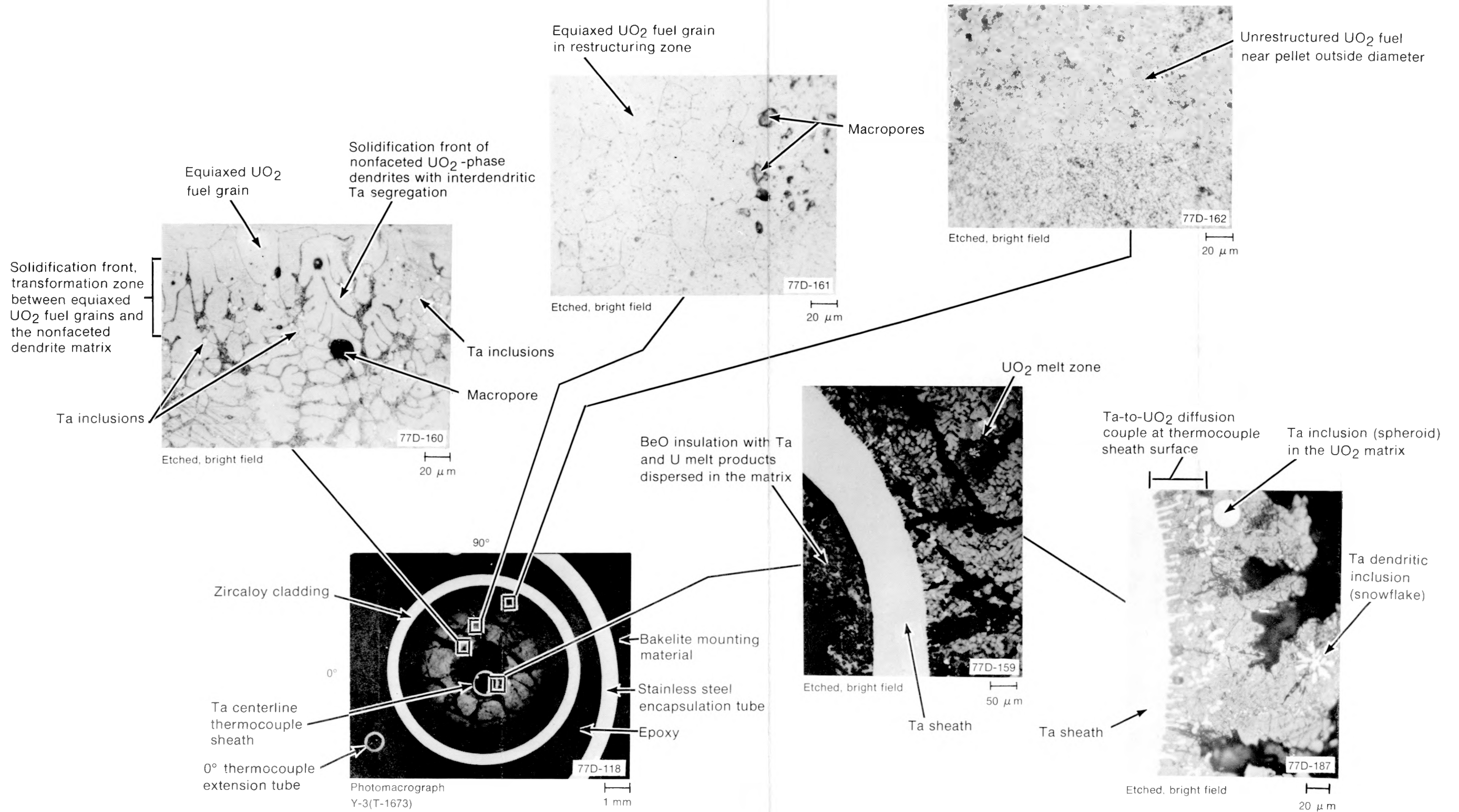
Fig. D-6 Transverse section (Y-3) of Rod UTA-0014 showing fuel microstructure.
