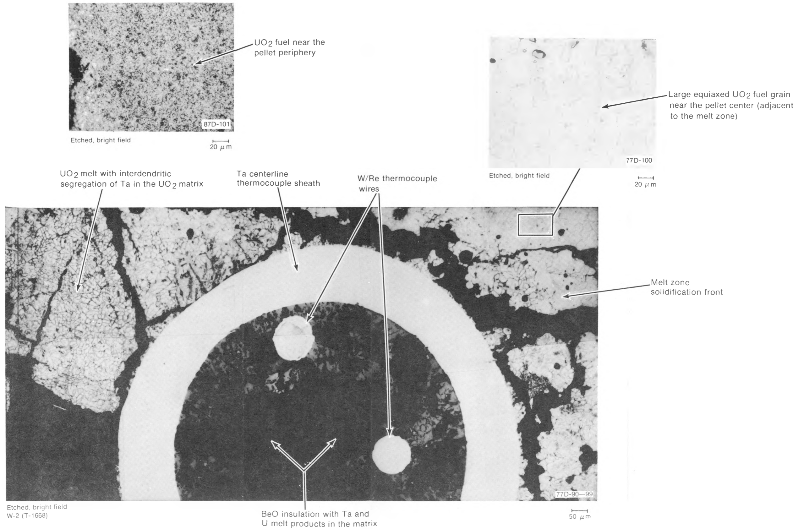
Fig. D-29 Transverse section (W-2) of Rod UTA-0016 showing fuel restructuring and tantalum thermocouple sheath melting with the UO 2 fuel.
