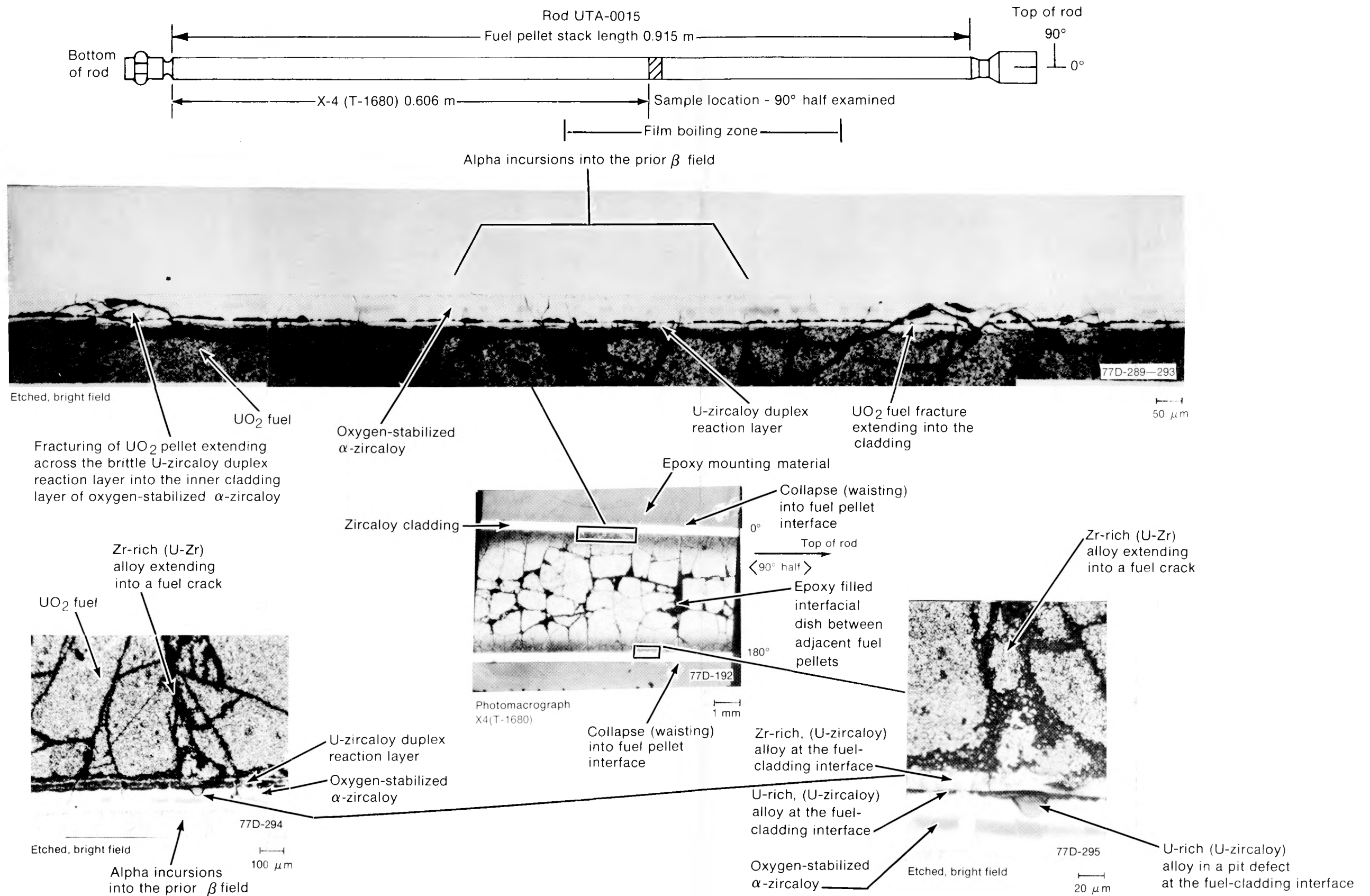
Fig. D-20 Longitudinal section (X-4) of Rod UTA-0015, between 0.606 and 0.625 m.
