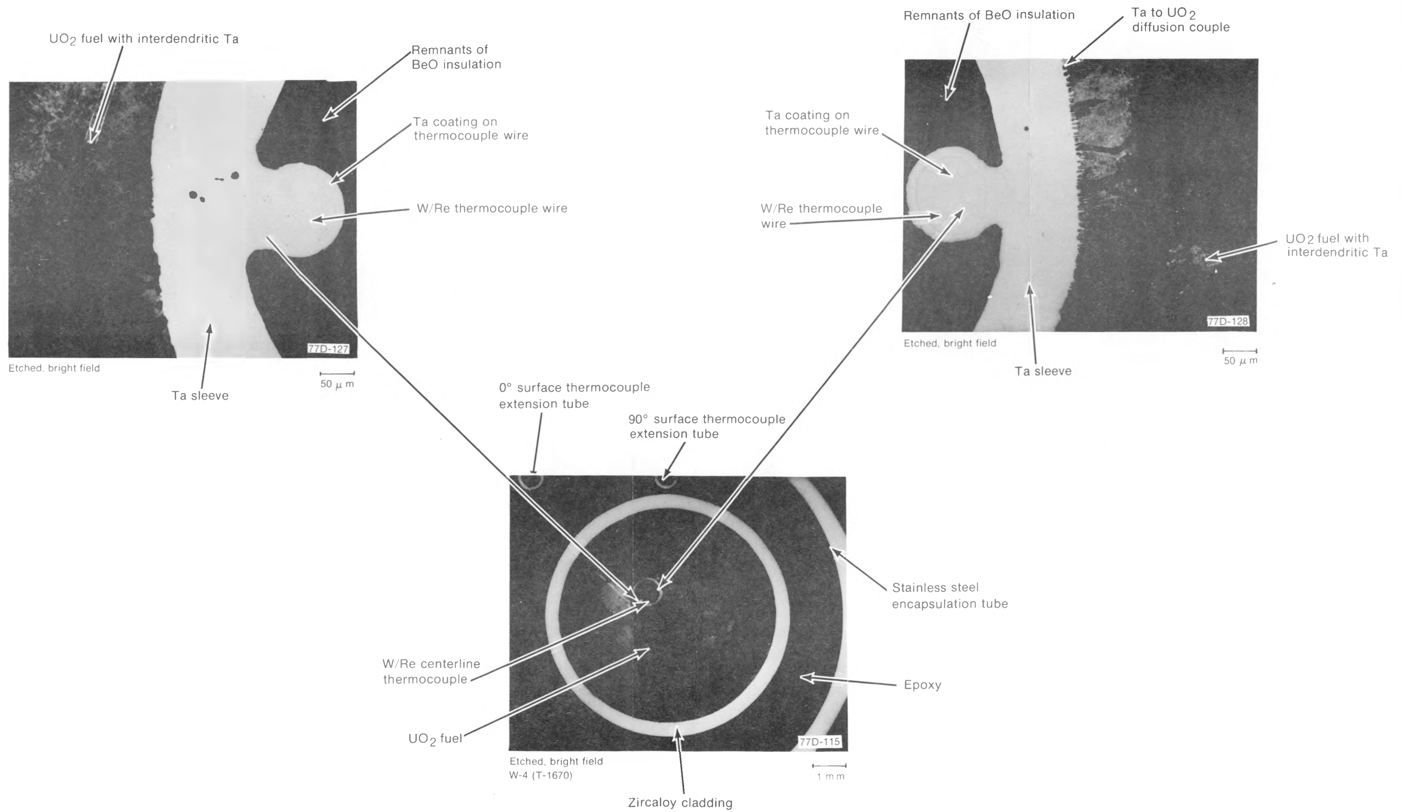
Fig. E-5 Centerline thermocouple near the junction in Rod UTA-0016.
