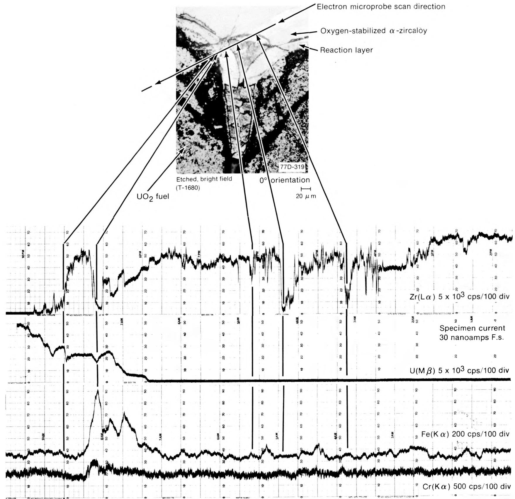
Fig. D-42 Electron microprobe scan across the collapsed cladding material at a fuel pellet interfacial gap in Rod UTA-0015.
