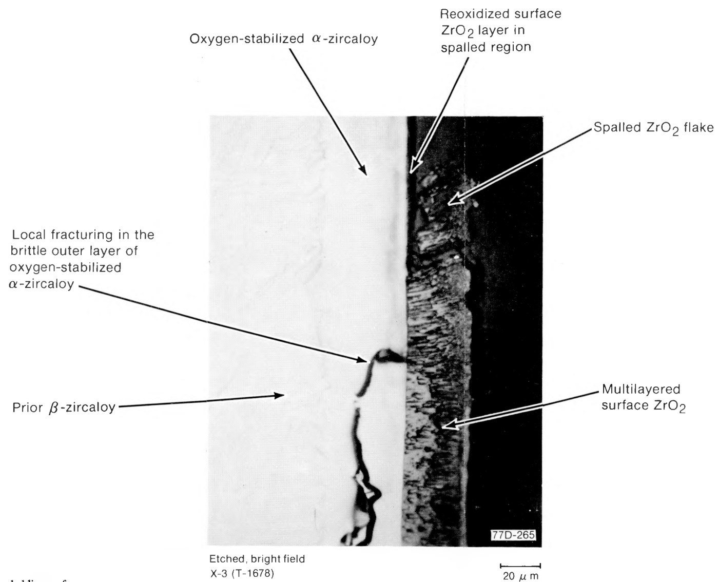
Fig. 26 Multilayered oxide on cladding surface.
