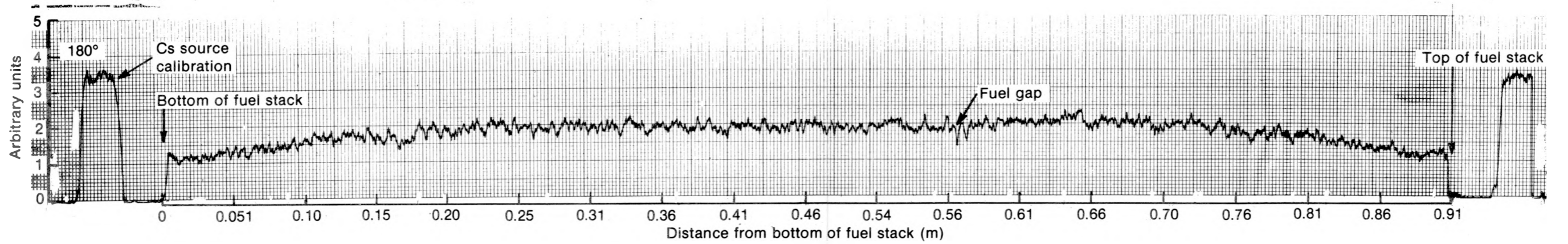
Fig. A-6 Gross gamma scan of Rod A-0017 at 180° orientation.
