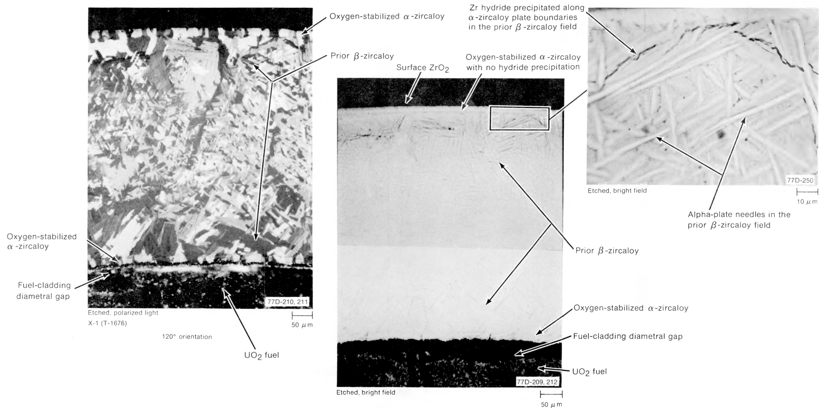
Fig. D-55 Hydride precipitation at 0.686-m and 120° circumferential orientation in Sample X-1 of Rod UTA-0015.
