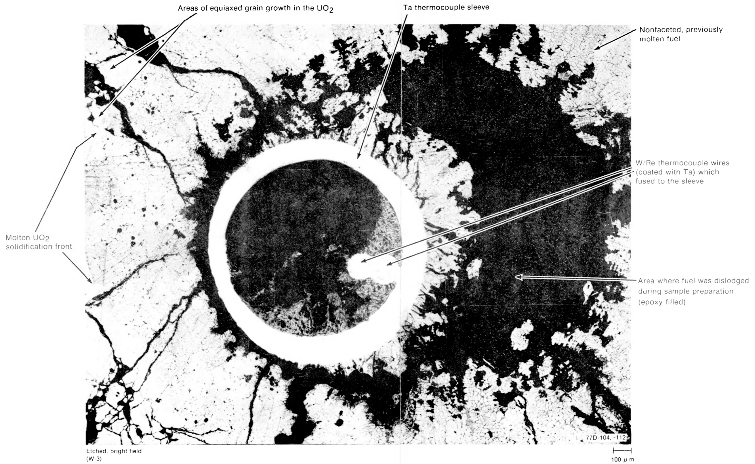
Fig. E-6 Centerline thermocouple above the junction in Rod UTA-0016.
