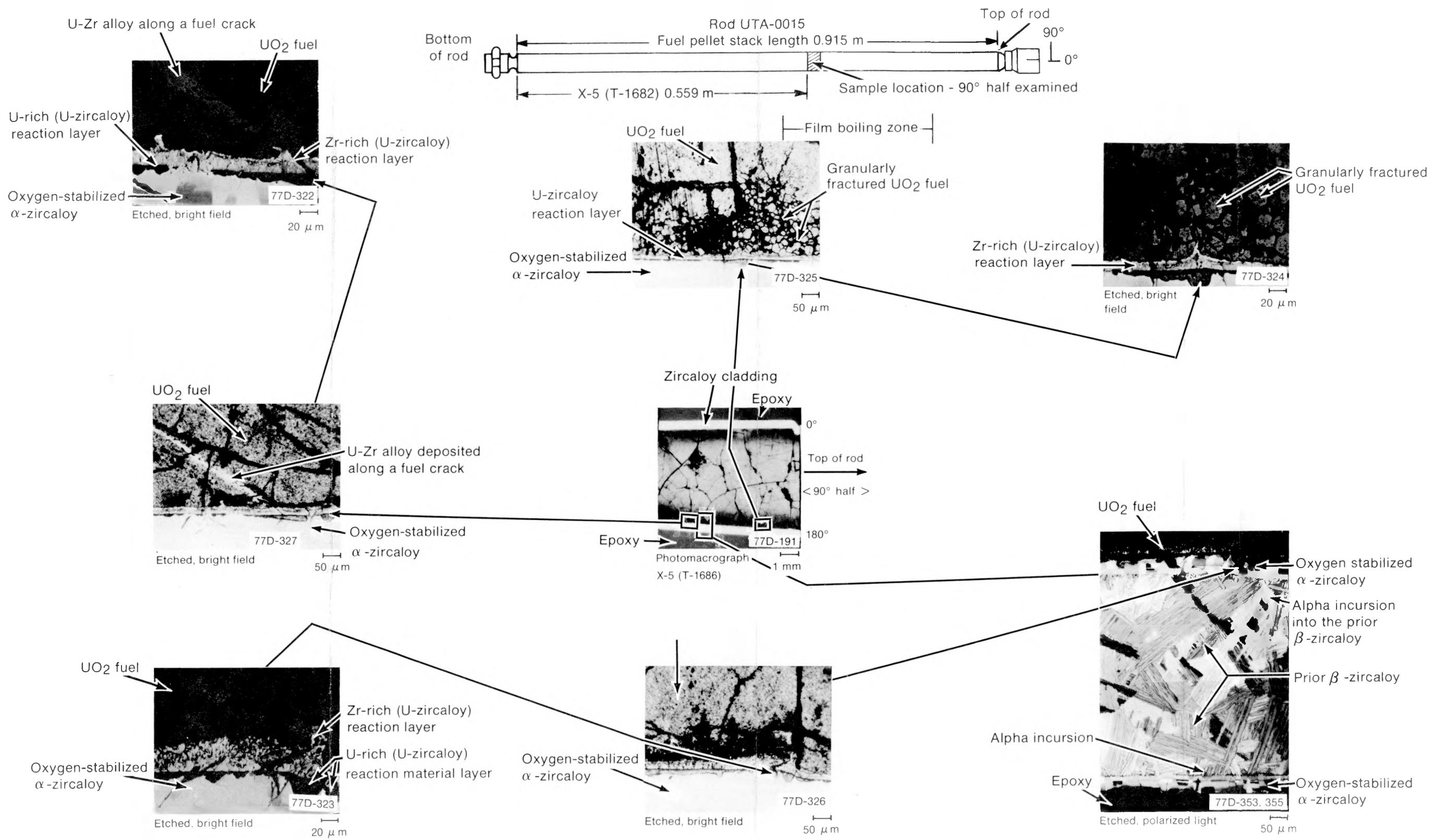
Fig. D-23 Longitudinal section (X-5) of Rod UTA-0015 between 0.559 and 0.571 m.
