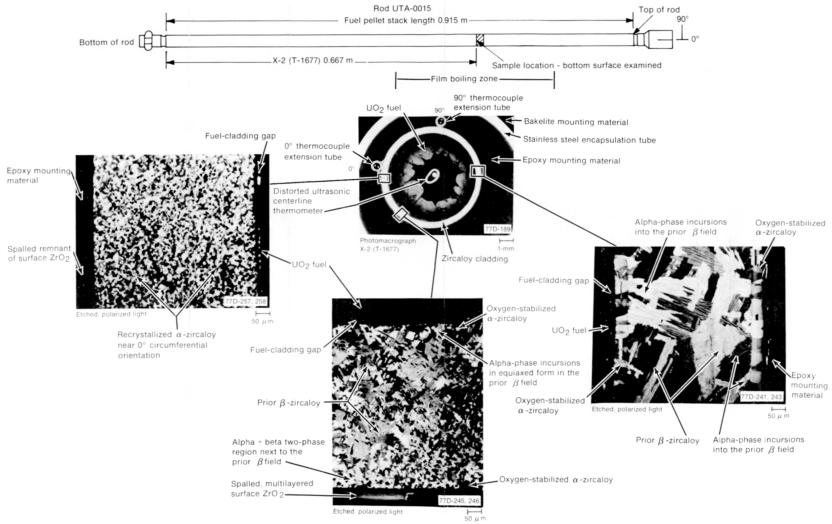
Fig. D-14 Transverse section (X-2) of Rod UTA-0015 (0.667 m) showing cladding microstructure.
