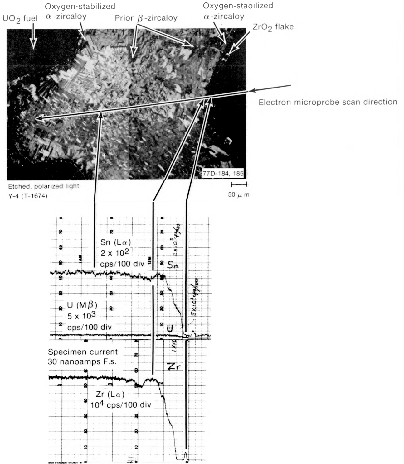
Fig. 51 Electron microprobe scan across the surface oxide and zircaloy cladding of Rod UTA-0014.
