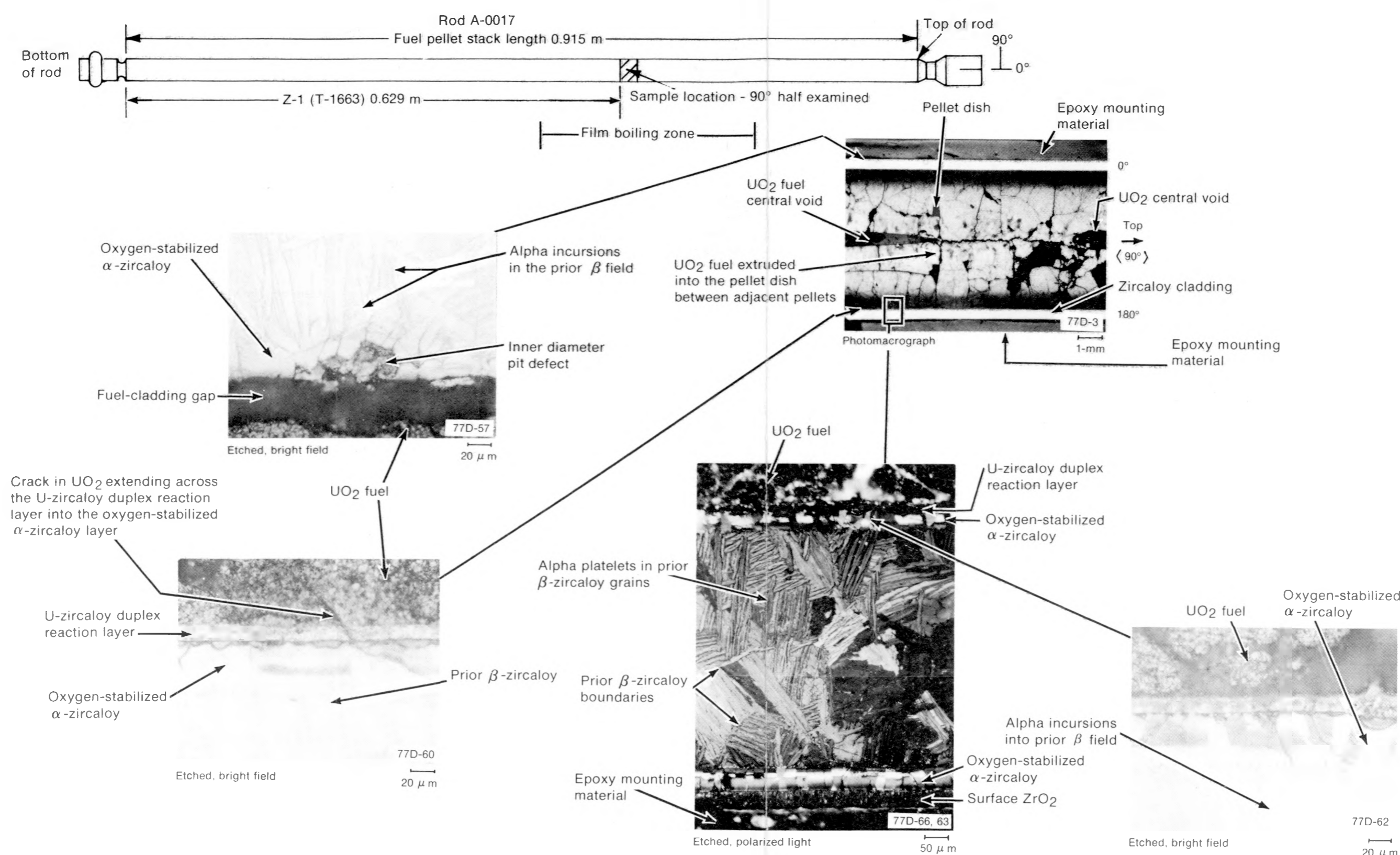
Fig. D-35 Longitudinal section (Z-1) of Rod A-0017 (between 0.629 and 0.648 m) showing cladding microstructure.
