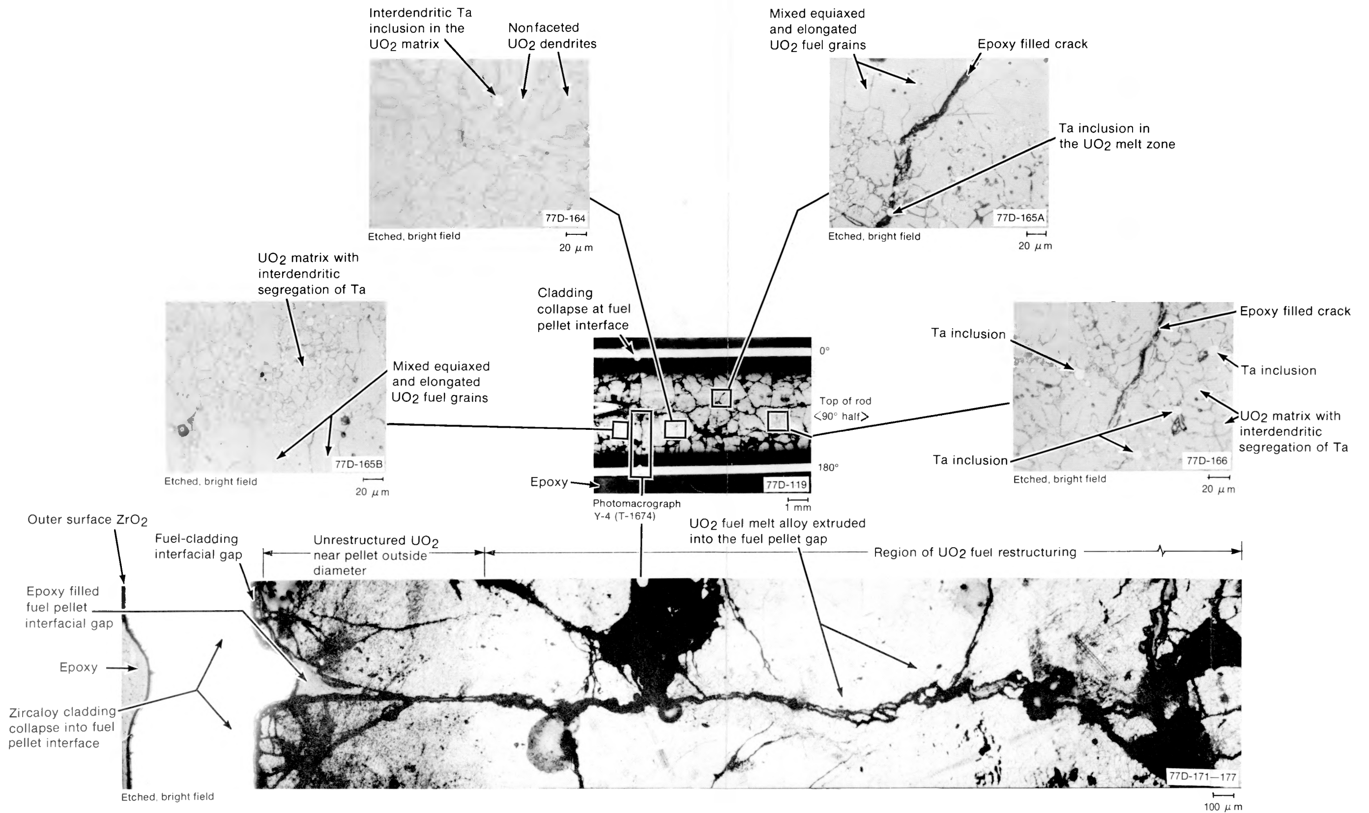
Fig. D-8 Longitudinal section (Y-4) of Rod UTA-0014 showing fuel microstructure.
