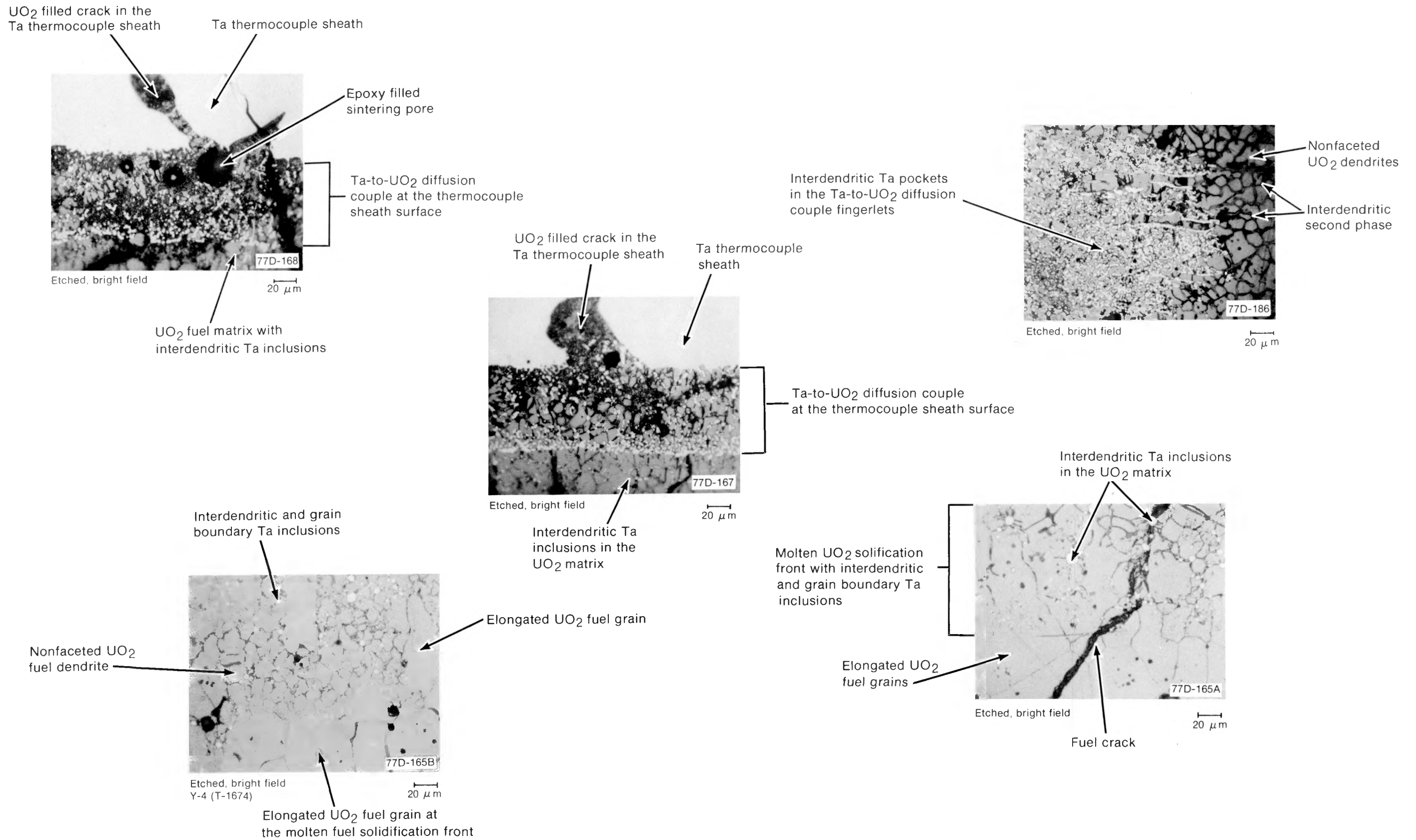
Fig. D-45 Molten UO 2 zone associated with tantalum melting into the fuel matrix.
