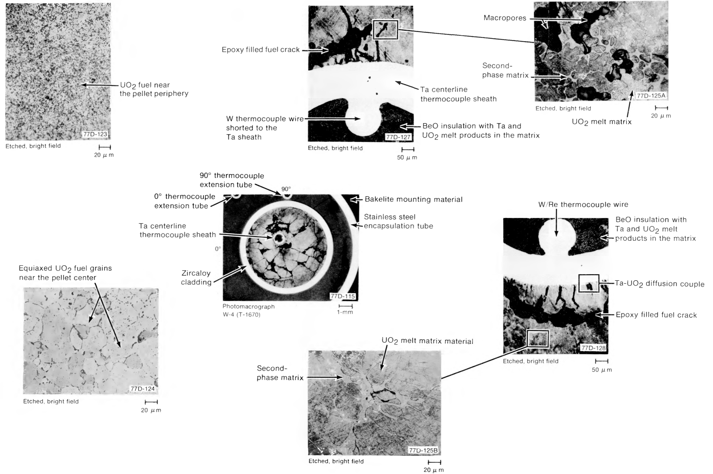
Fig. D-34 Transverse section (W-4) of Rod UTA-0016 showing fuel restructuring and fuel melting zone.
