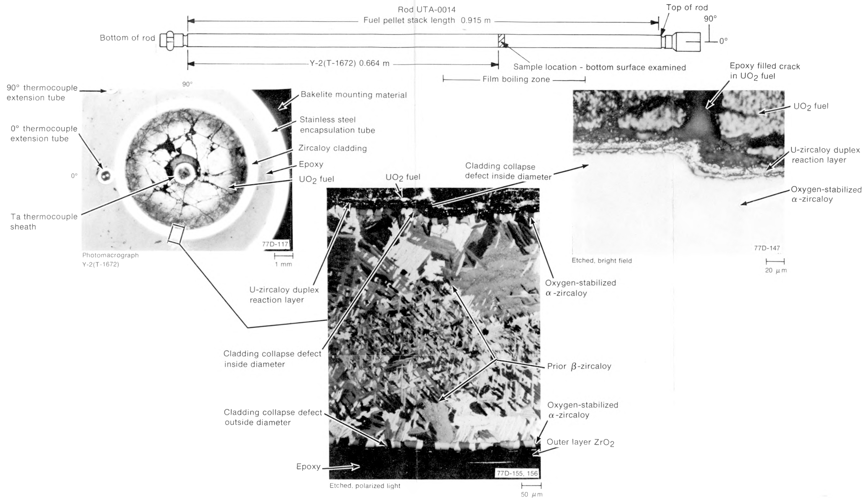
Fig. D-3 Transverse section (Y-2) of Rod UTA-0014 (0.664 m) showing cladding microstructure.
