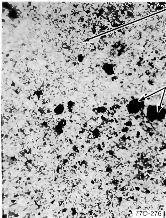
Fig. D-19 Transverse section (X-3) of Rod UTA-0015 showing fuel restructuring.
