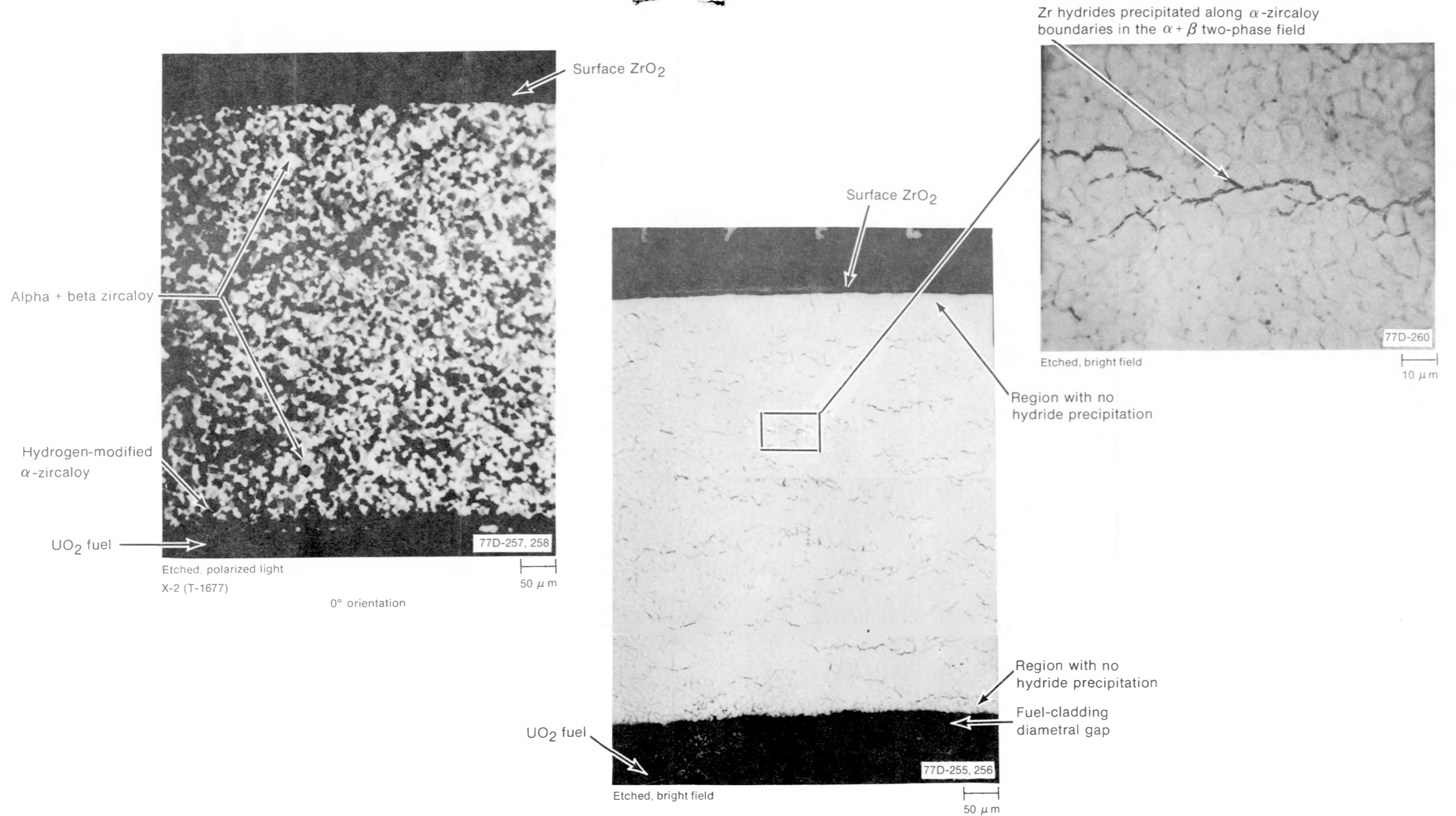
Fig. D-57 Dispersed hydriding at 0.667-m in Sample X-2 of Rod UTA-0015.
