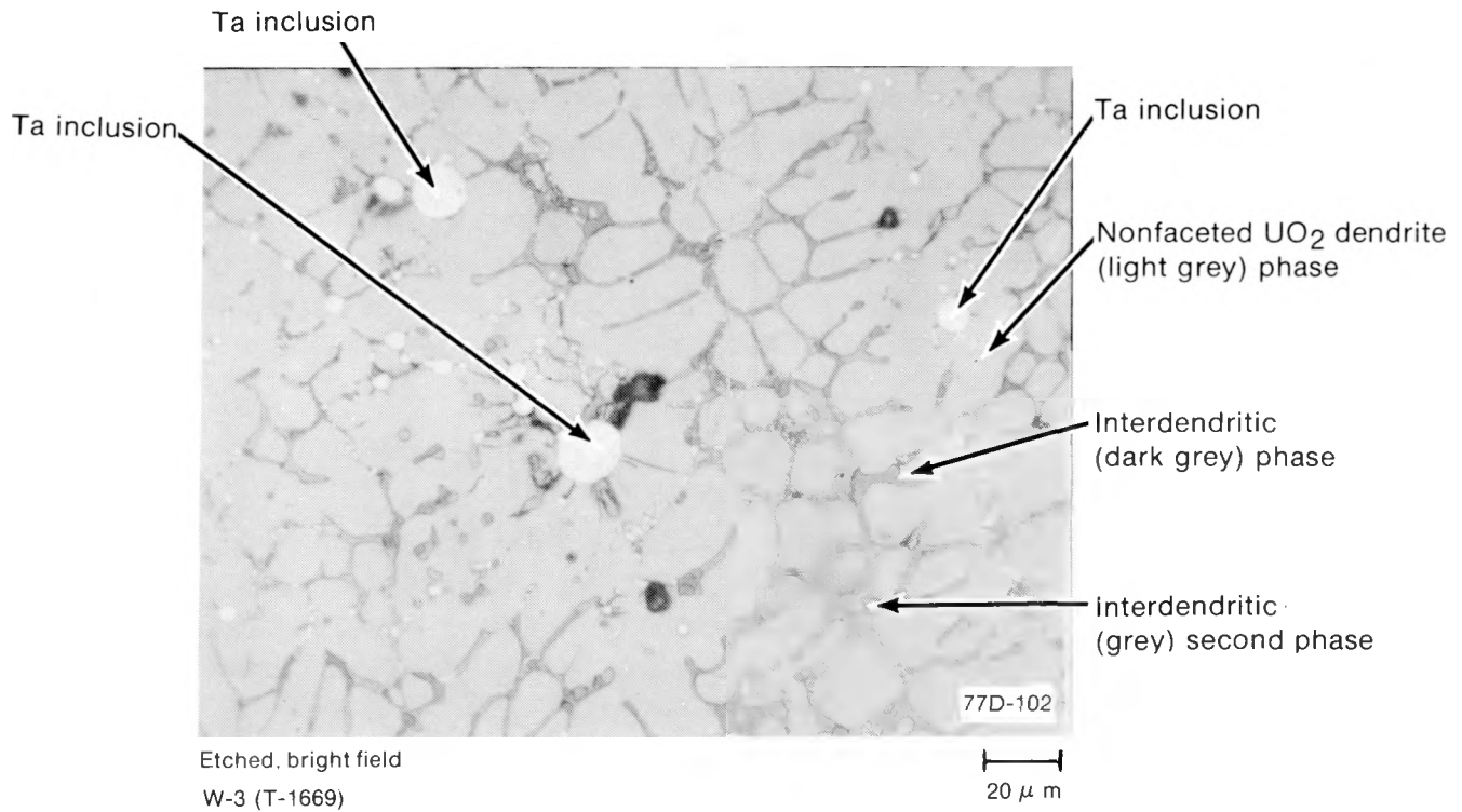
Fig. D-48 Nonfaceted UO 2 dendrites with interdentritic tantalum inclusions in the tantalum-UO 2 melt zone.
