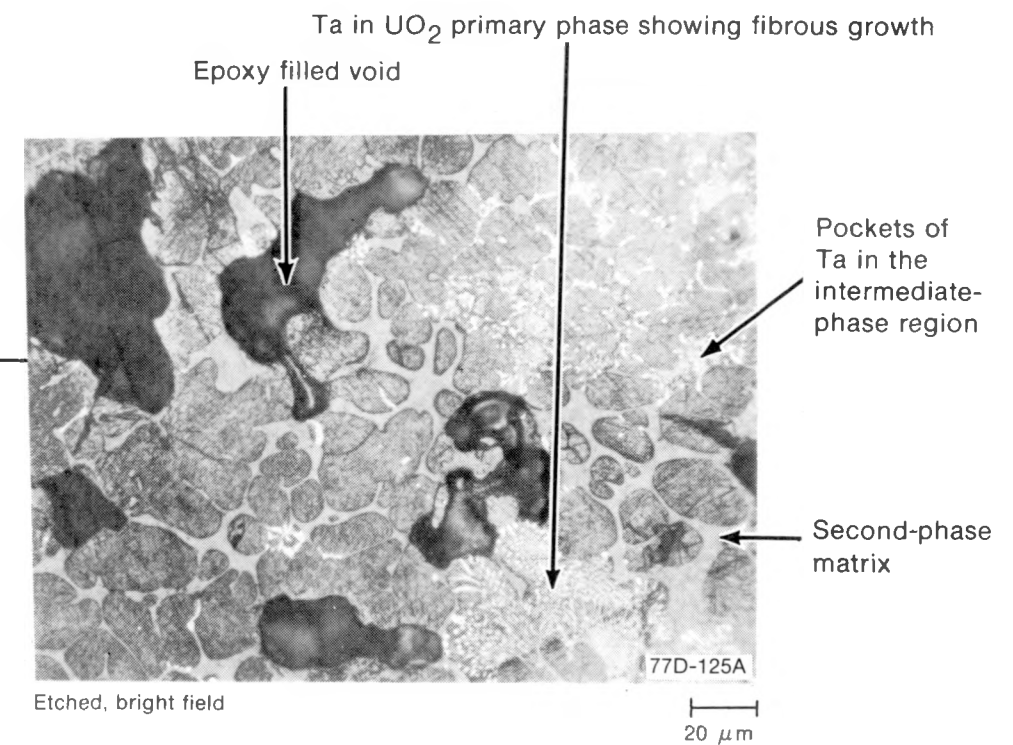
Fig. D-46 Tantalum and UO 2 diffusion couple with interdendritic tantalum inclusion and a second phase surrounding the UO 2 matrix dendrites in Rod UTA-0016.
