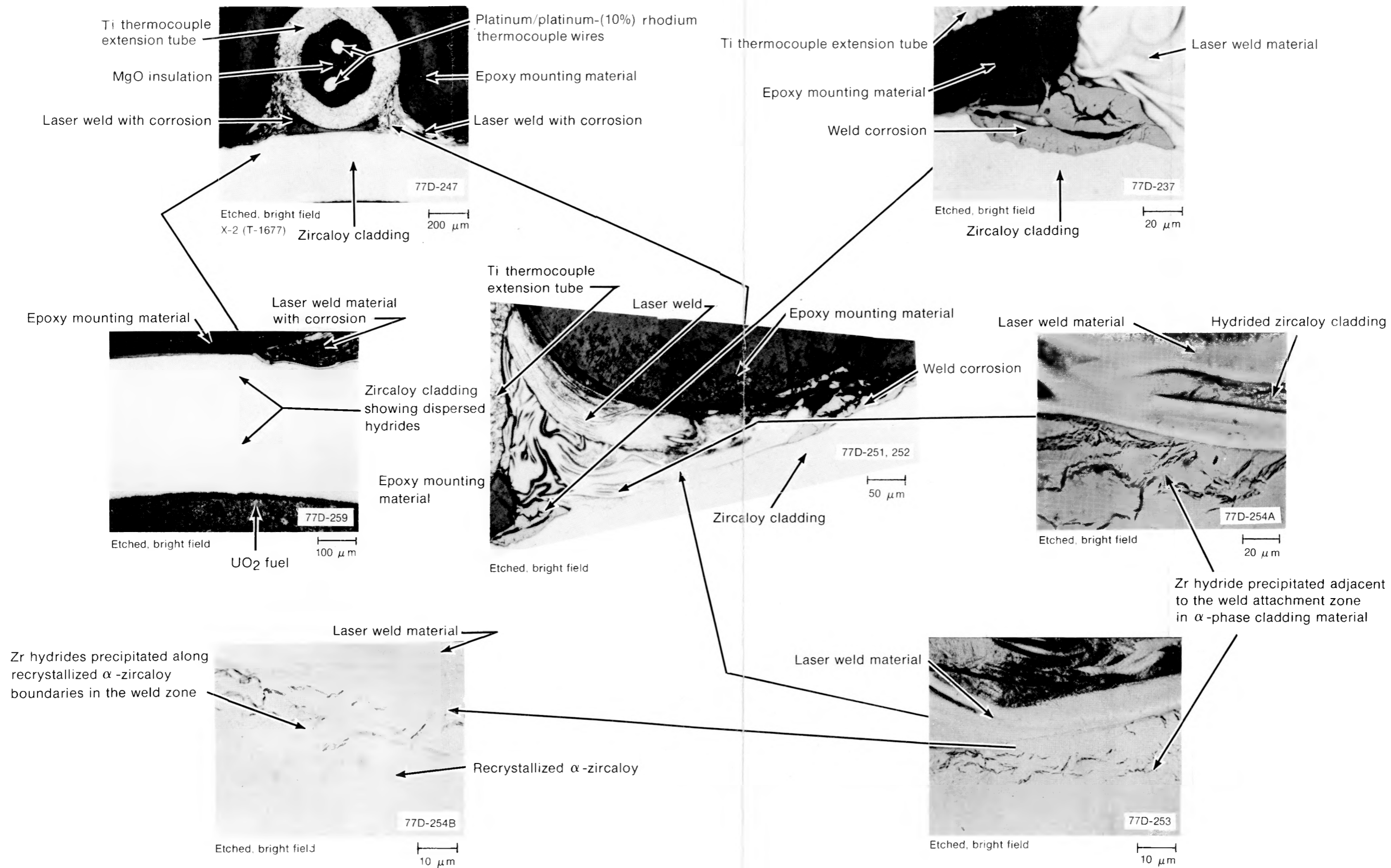
Fig. E-3 The 0^{\circ} thermocouple extension tube weld at 0.667 m on Rod UTA-0015.
