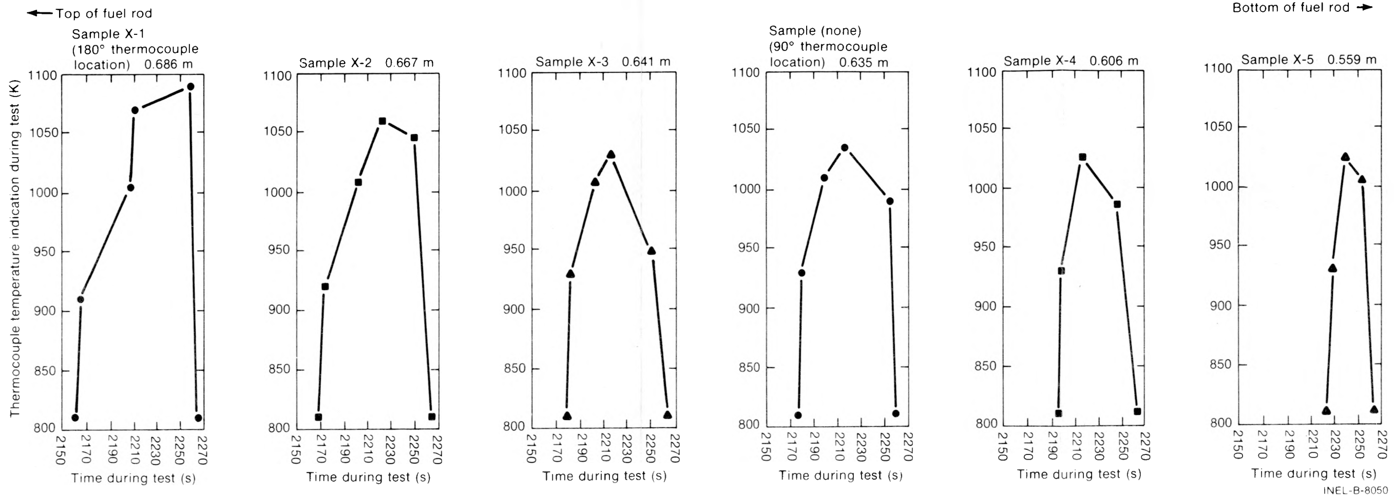
Fig. F-6 Linearized time-temperature profile computer code input for Rod UTA-0015.
