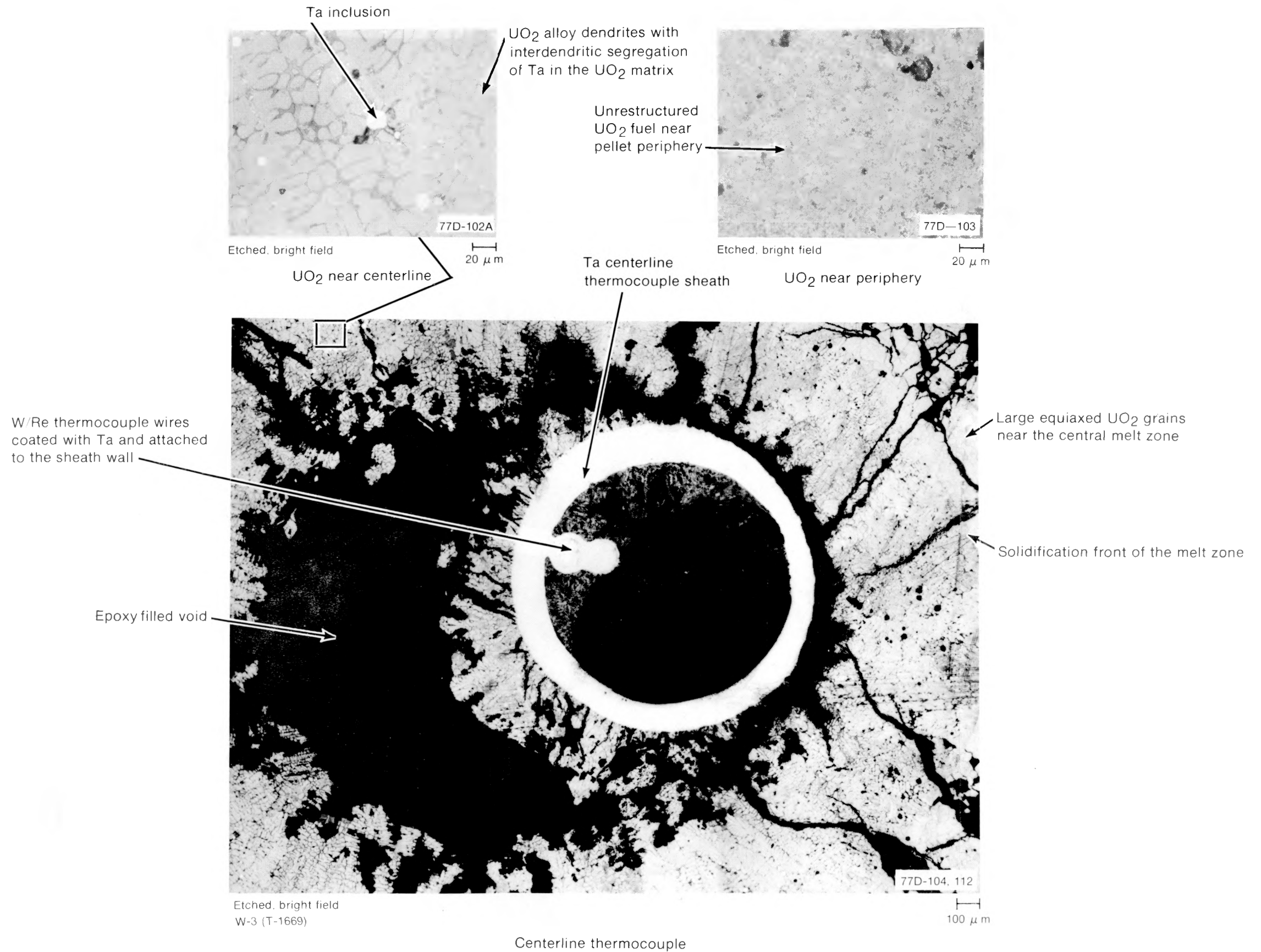
Fig. D-32 Transverse section (W-3) of Rod UTA-0016 showing fuel restructuring and fuel melting with the tantalum centerline thermocouple sheath.
