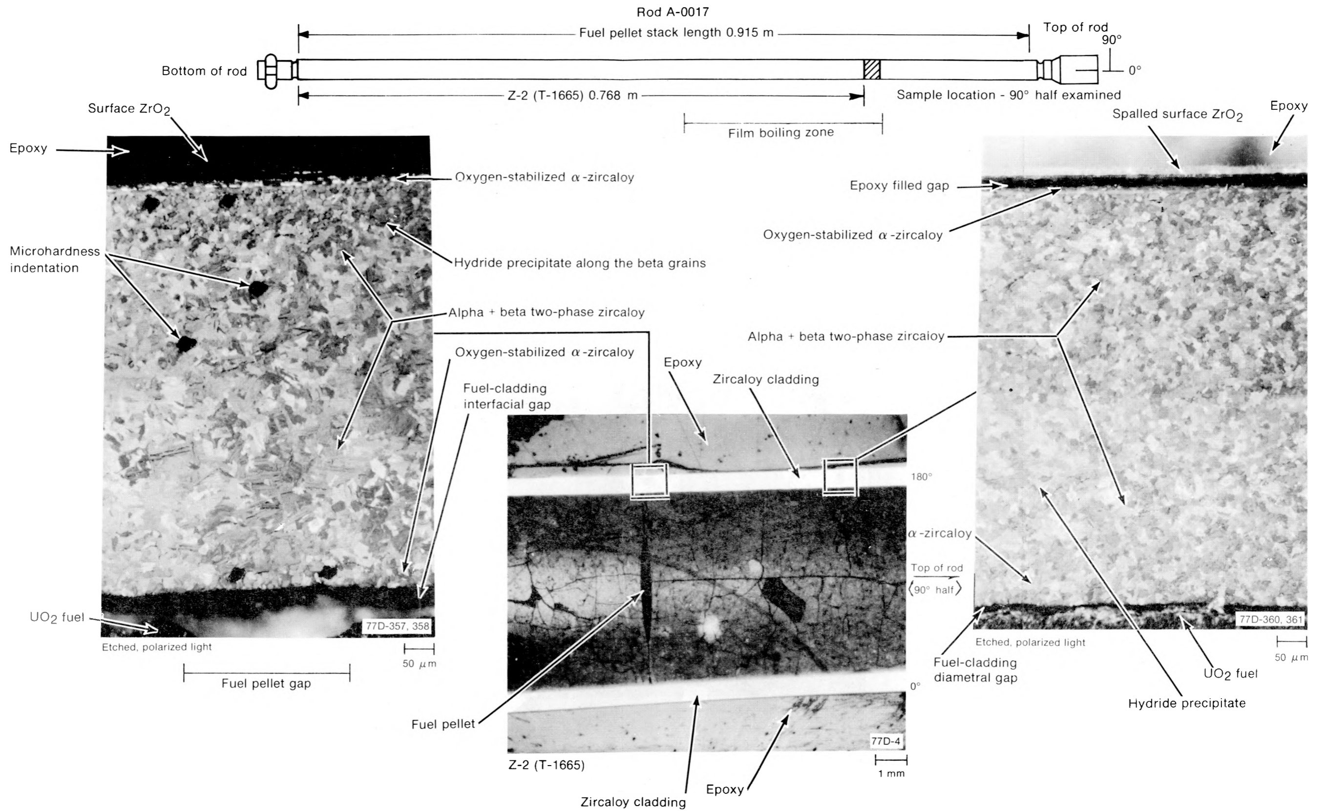
Fig. D-37 Longitudinal section (Z-2) of Rod A-0017 (between 0.768 and 0.87 m) showing cladding microstructure.
