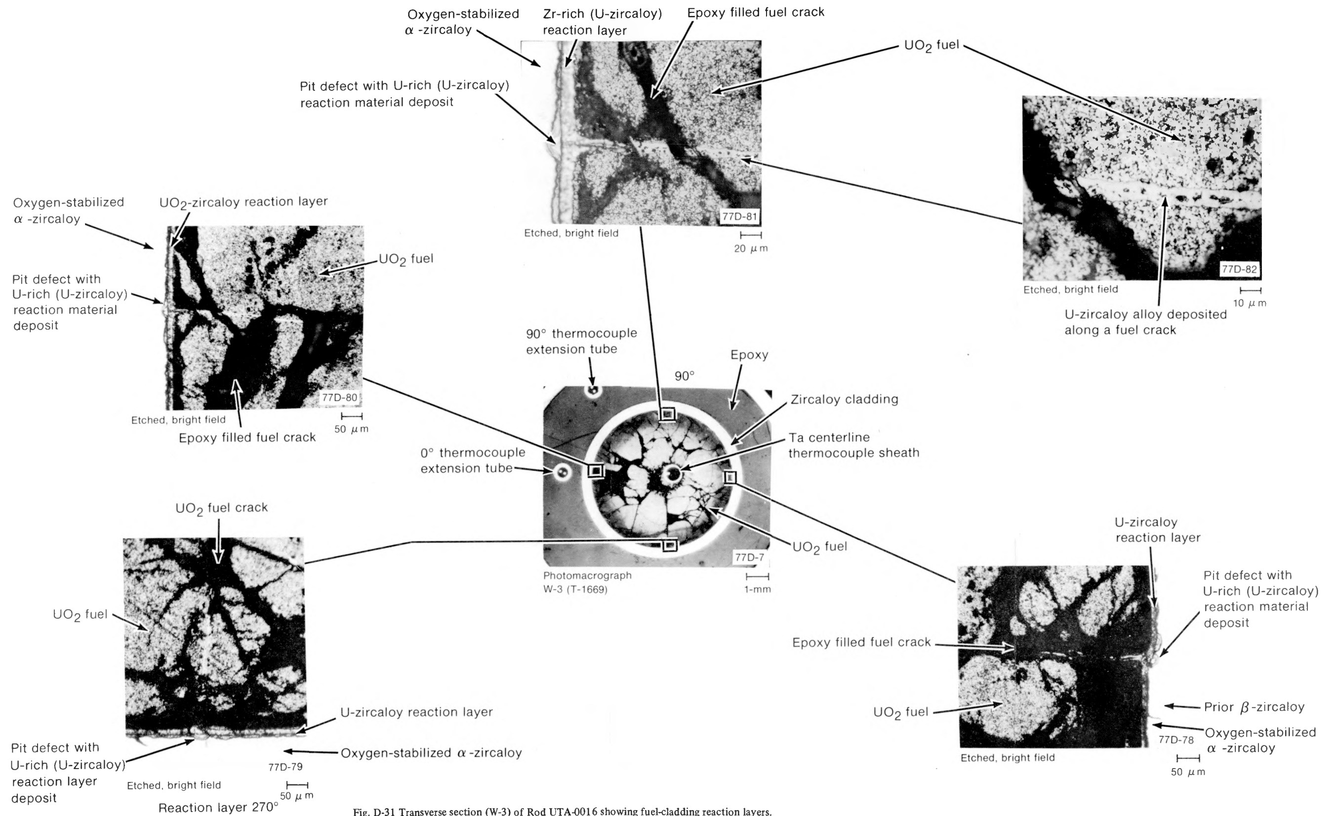
Fig. D-31 Transverse section (W-3) of Rod UTA-0016 showing fuel-cladding reaction layers.
