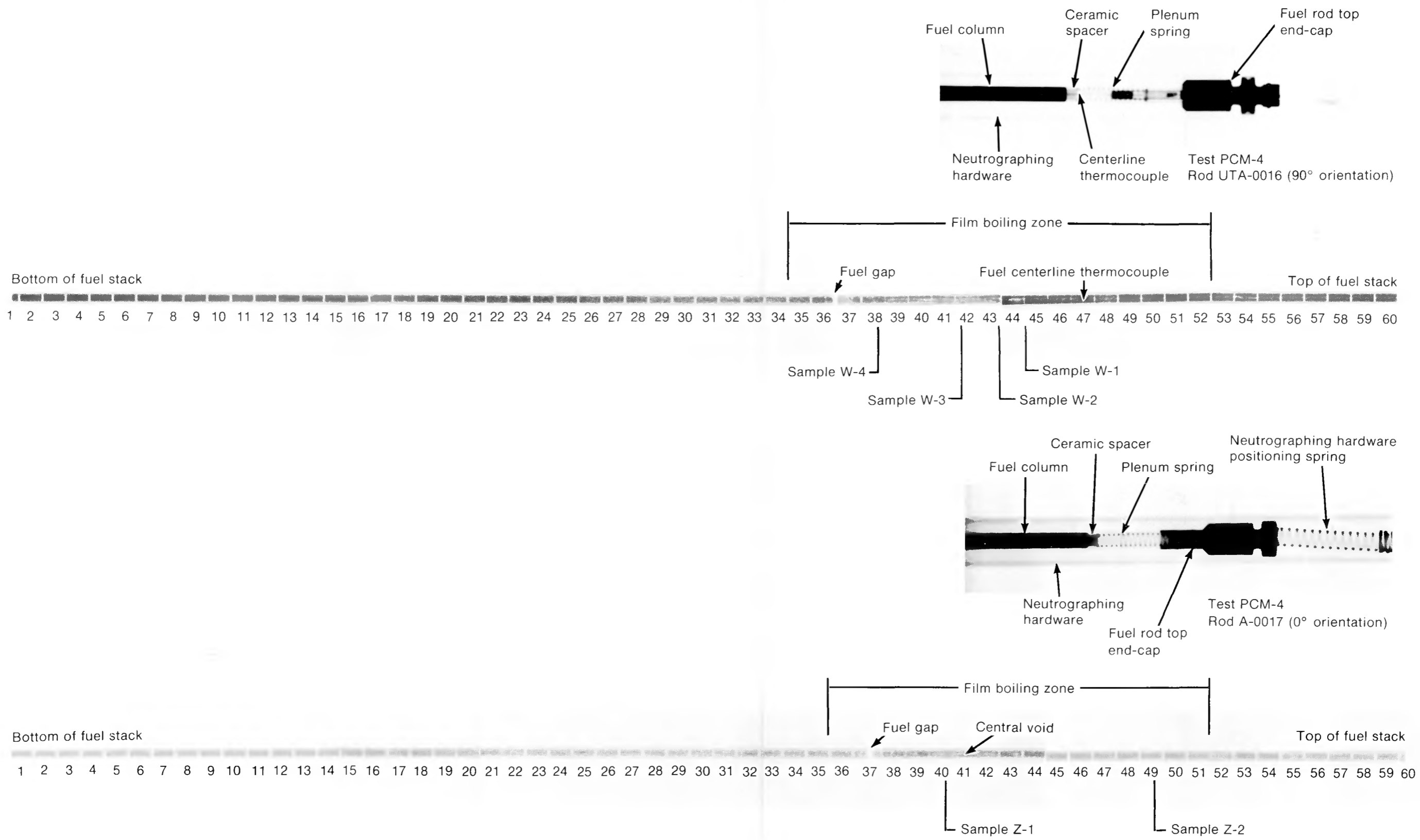
Fig. 10 Composite posttest neutrographs of the fuel stacks of Rods UTA-0016 and A-0017.
