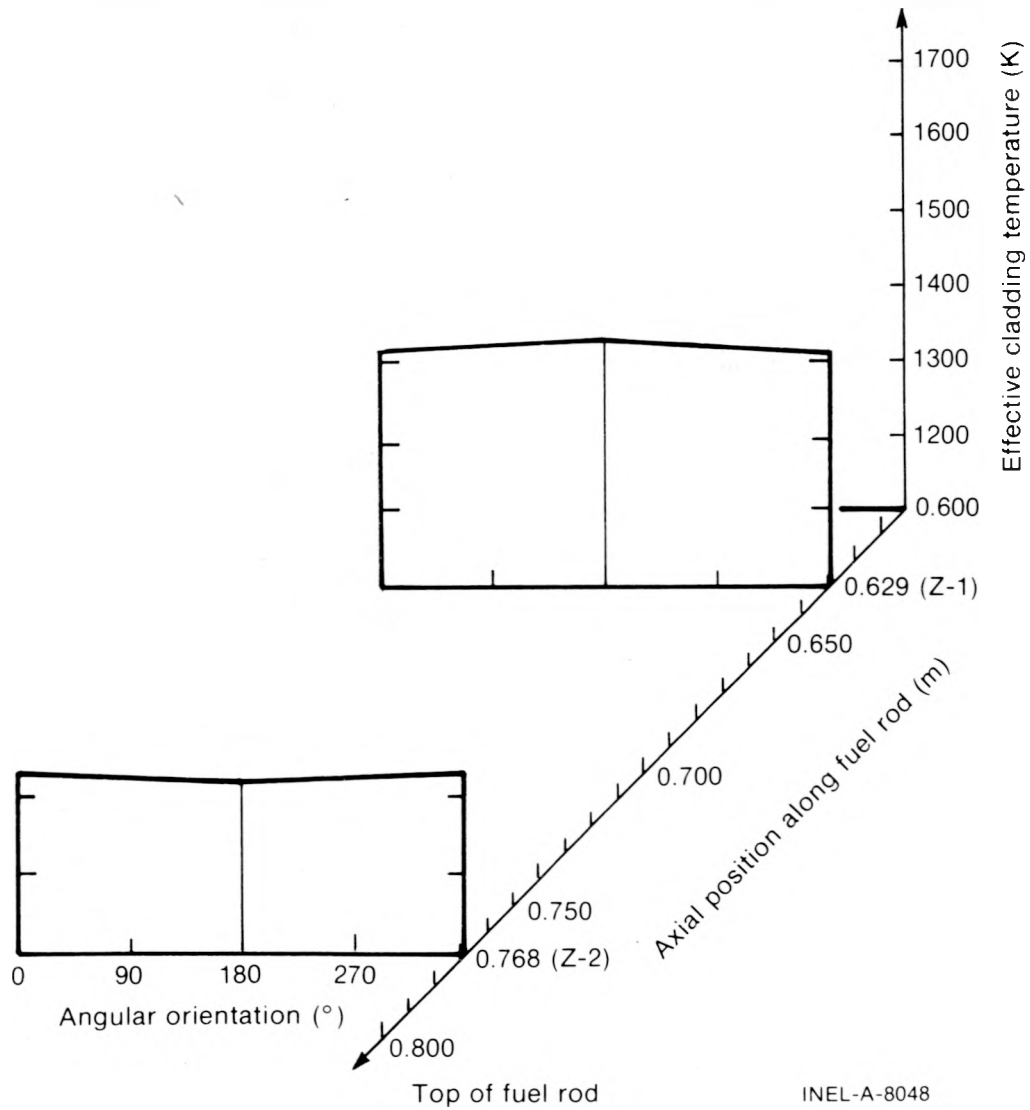
Fig. 20 Isometric plot of the isothermal effective cladding temperature as a function of angular orientation and axial position for Rod A-0017.
