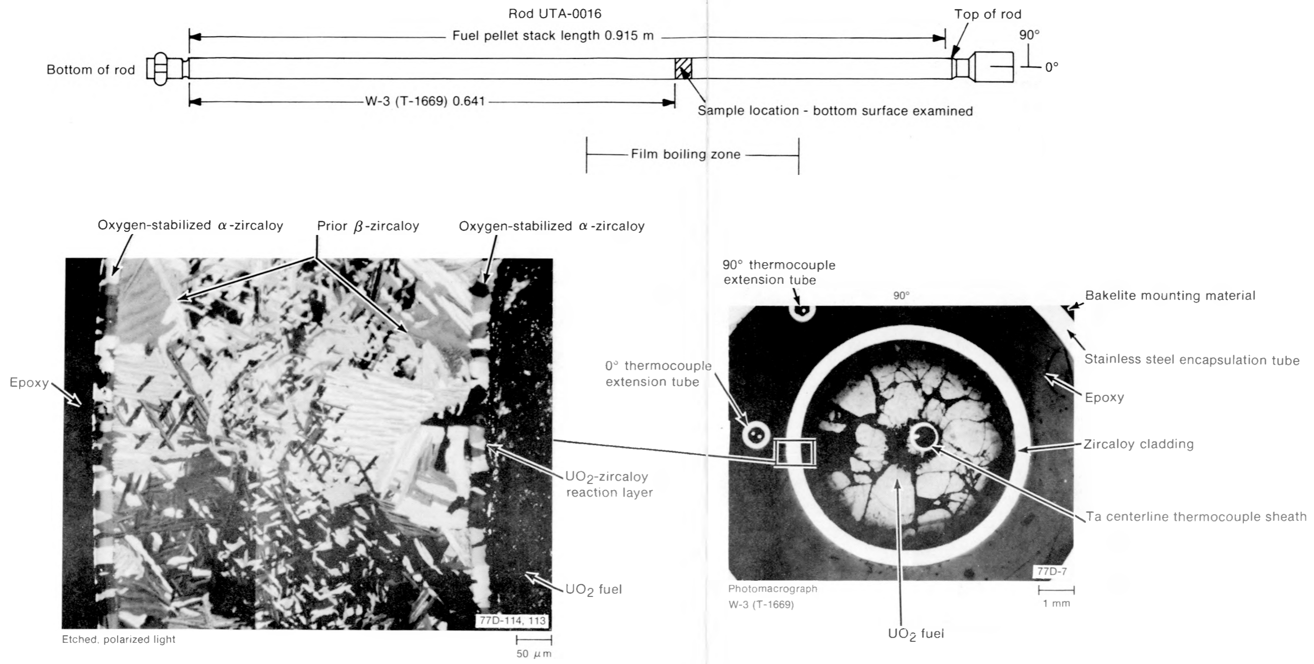
Fig. D-30 Transverse section (W-3) of Rod UTA-0016 (0.641 m) showing cladding microstructure.
