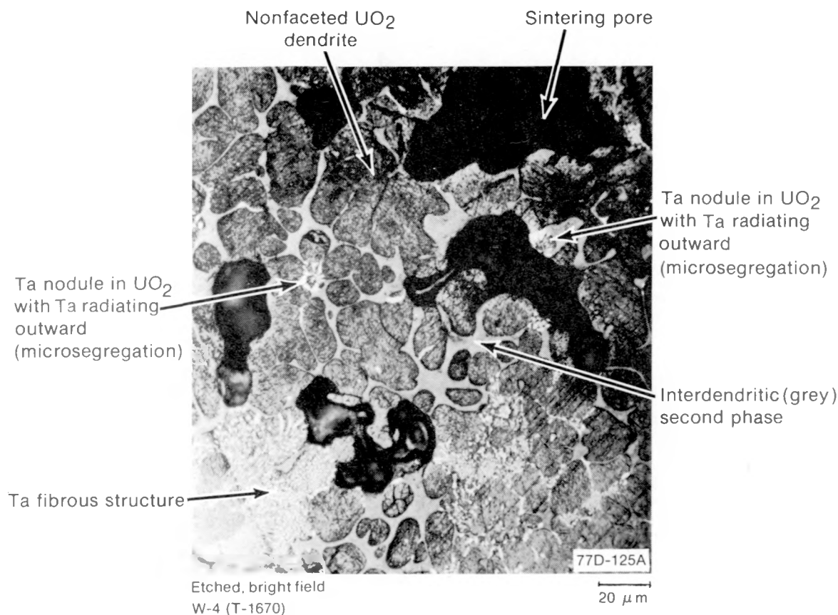
Fig. D-49 Tantalum and UO 2 molten zone with eutectic-like tantalum nodules in the UO 2 matrix.
