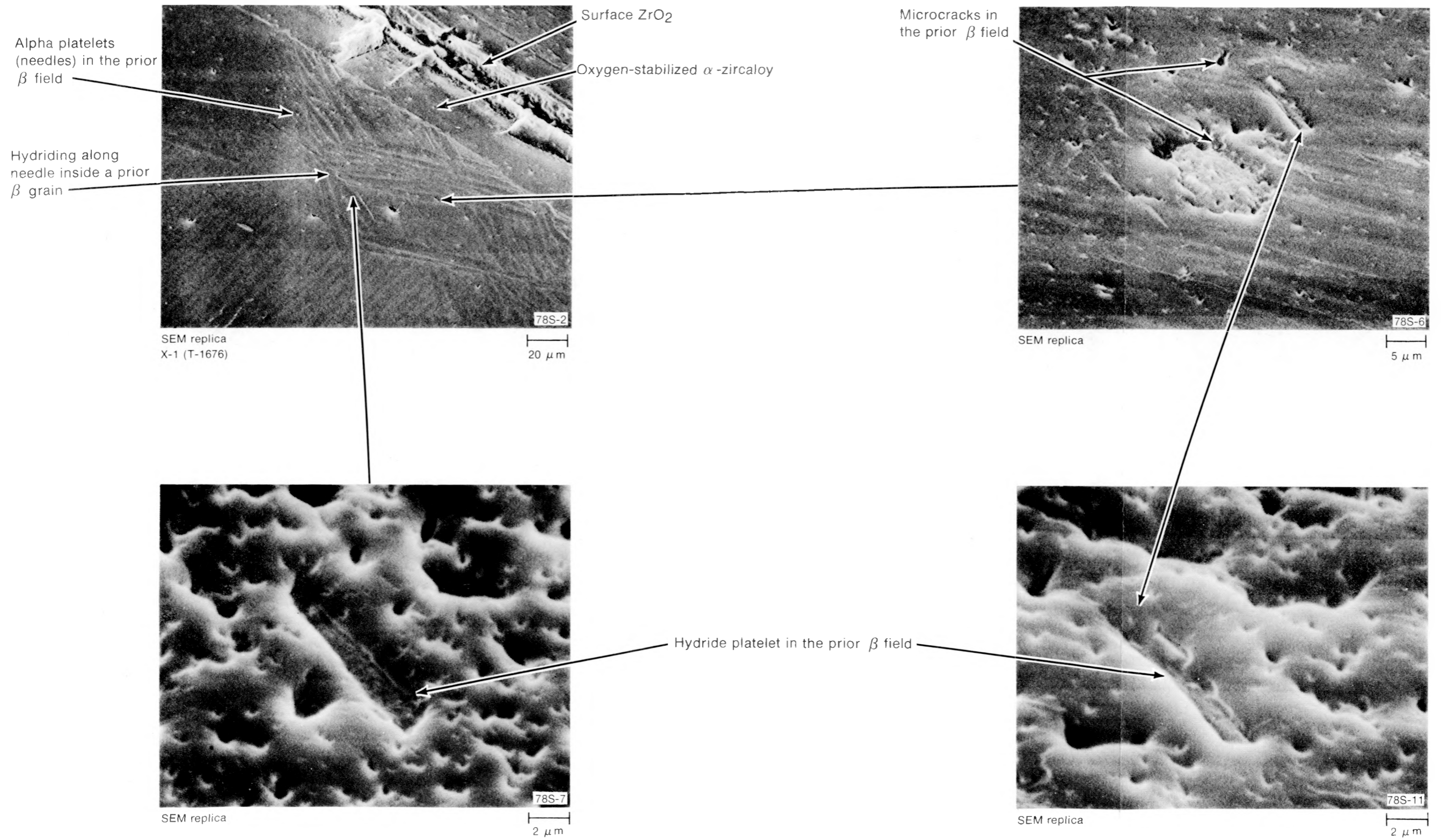
Fig. D-62 Hydride precipitation platelets in a replica of Sample X-1 of Rod UTA-0015 examined by scanning electron microscope.
