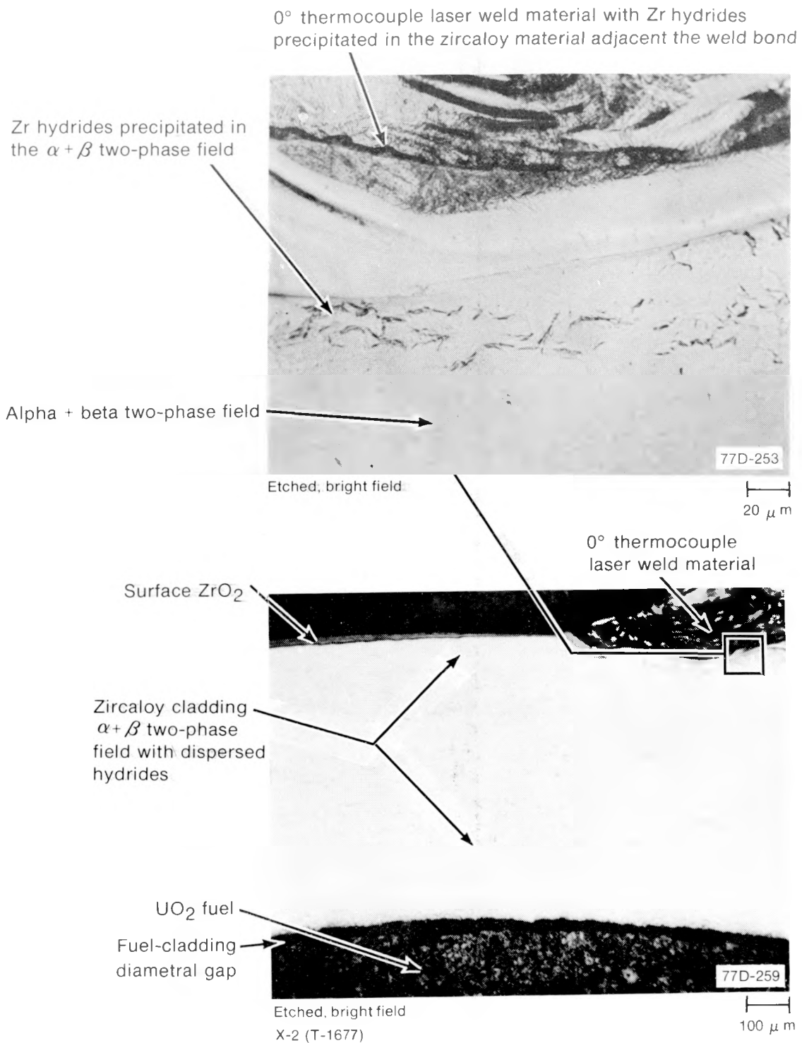
Fig. D-58 Dispersed hydriding at 0.667 m near the 0° thermocouple extension tube weld in Sample X-2 of Rod UTA-0015.
