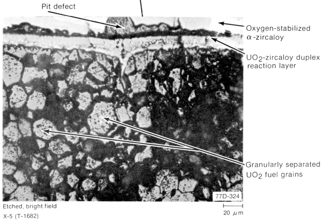
Fig. 39 Granular fracture of UO_2 fuel.
