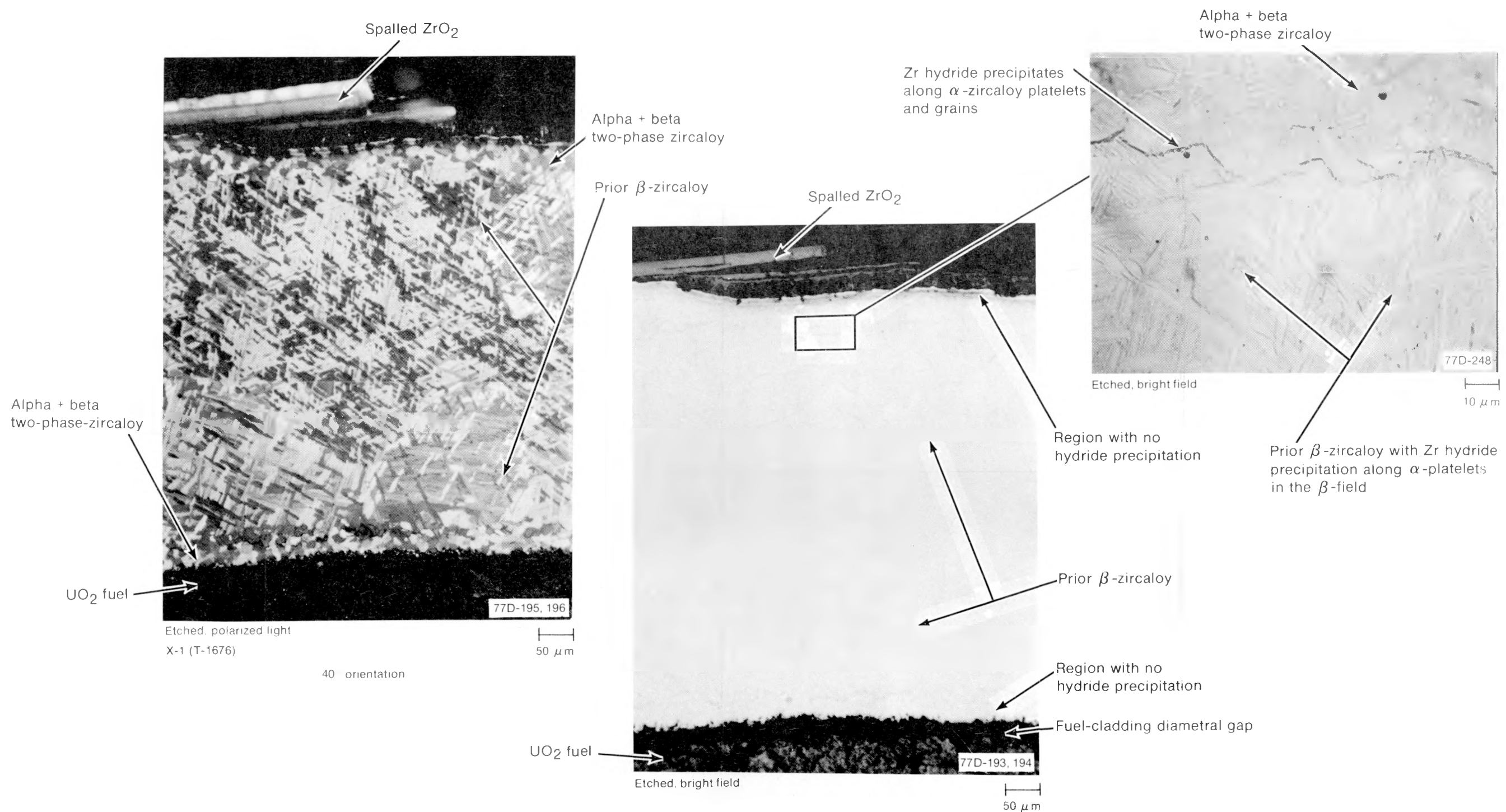
Fig. D-53 Hydride precipitation at 0.686-m and 40° circumferential orientation in Sample X-1 of Rod UTA-0015.
