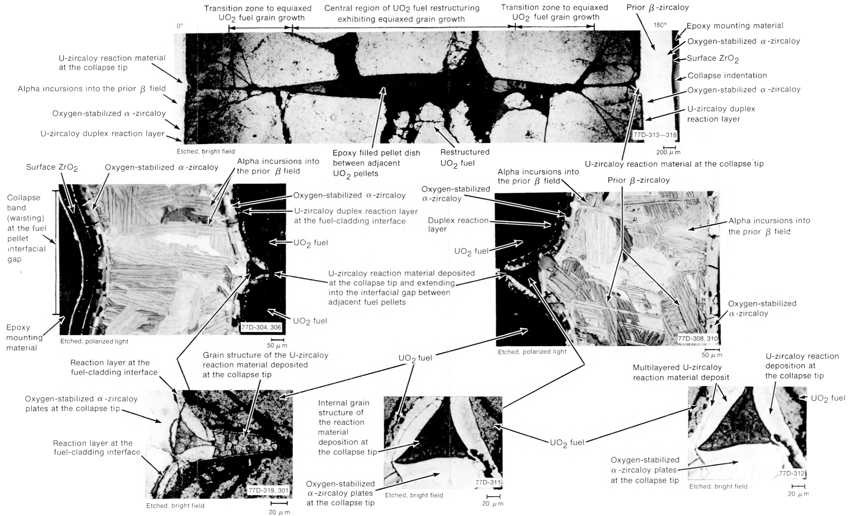
Fig. D-21 Longitudinal section (X-4) of Rod UTA-0015 showing fuel-cladding reaction.
