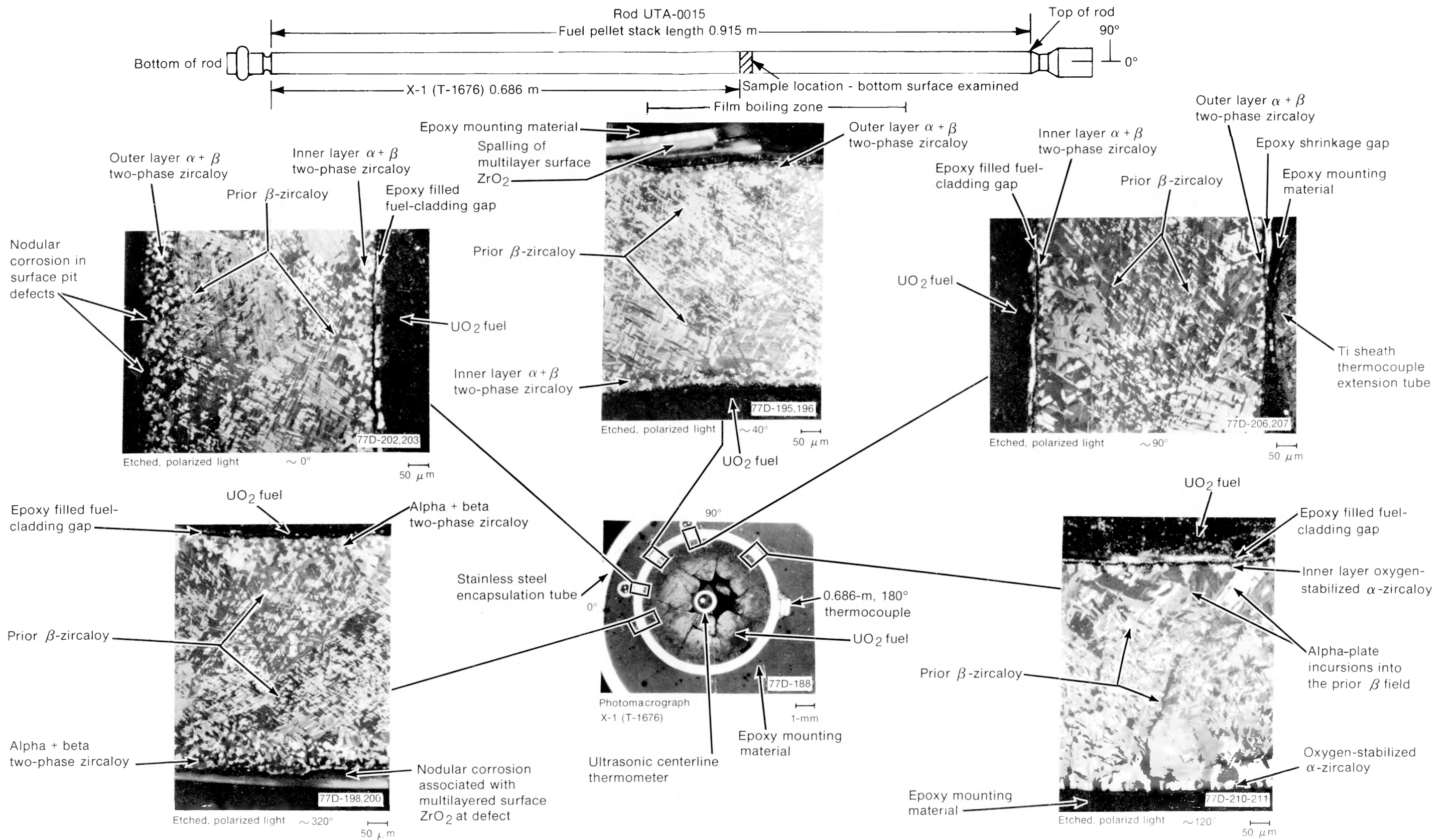
Fig. D-10 Transverse section (X-1) of Rod UTA-0015 (0.686 m) showing cladding microstructure.
