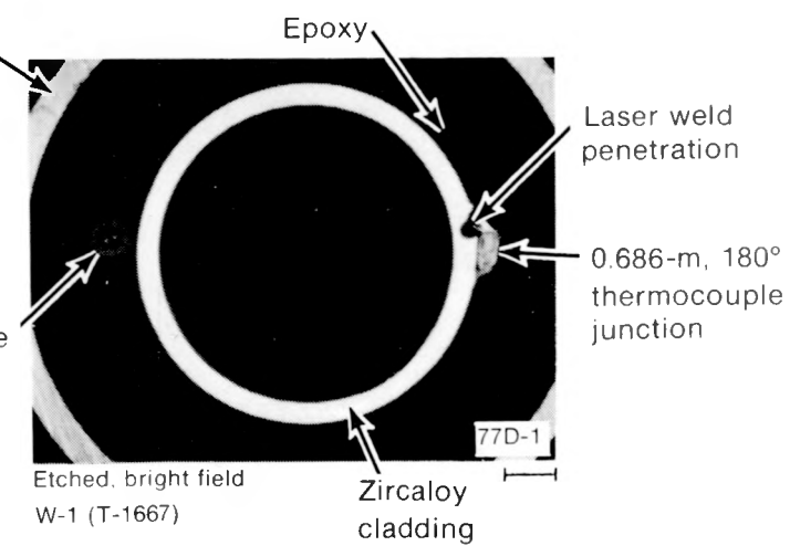
Fig E-4 View of the 0.686-m, 180° thermocouple junction from Rod UTA-0016.
