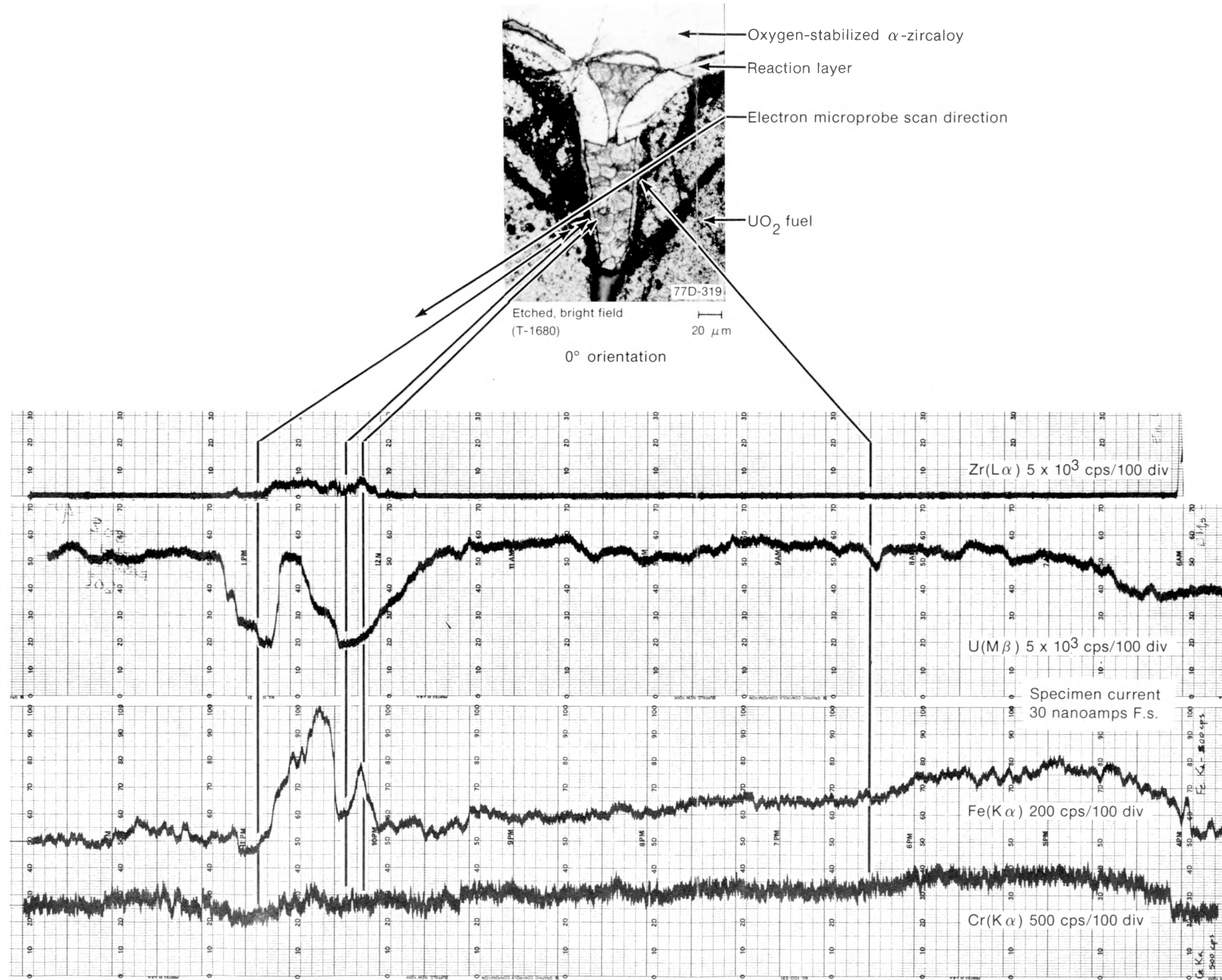
Fig. D-43 Electron microprobe scan across the reaction material associated with the cladding collapse at a fuel pellet interfacial gap in Rod UTA-0015.
