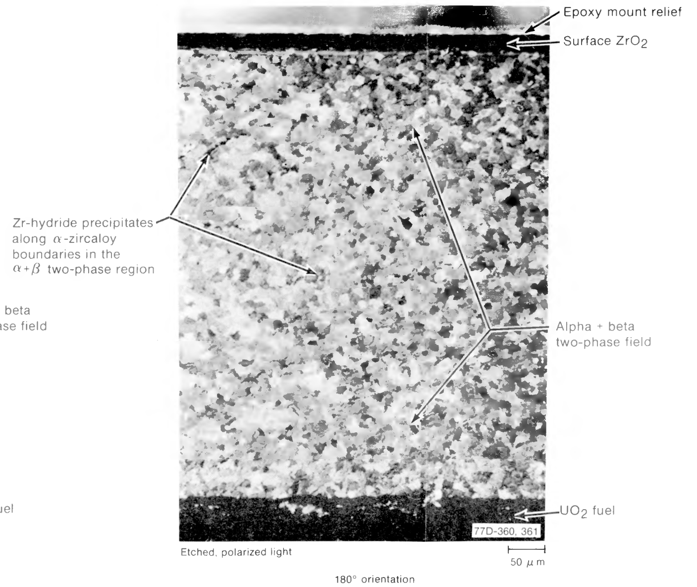
Fig. D-60 Hydriding in the alpha + beta two-phase field in Sample Z-2 of Rod A-0017.
