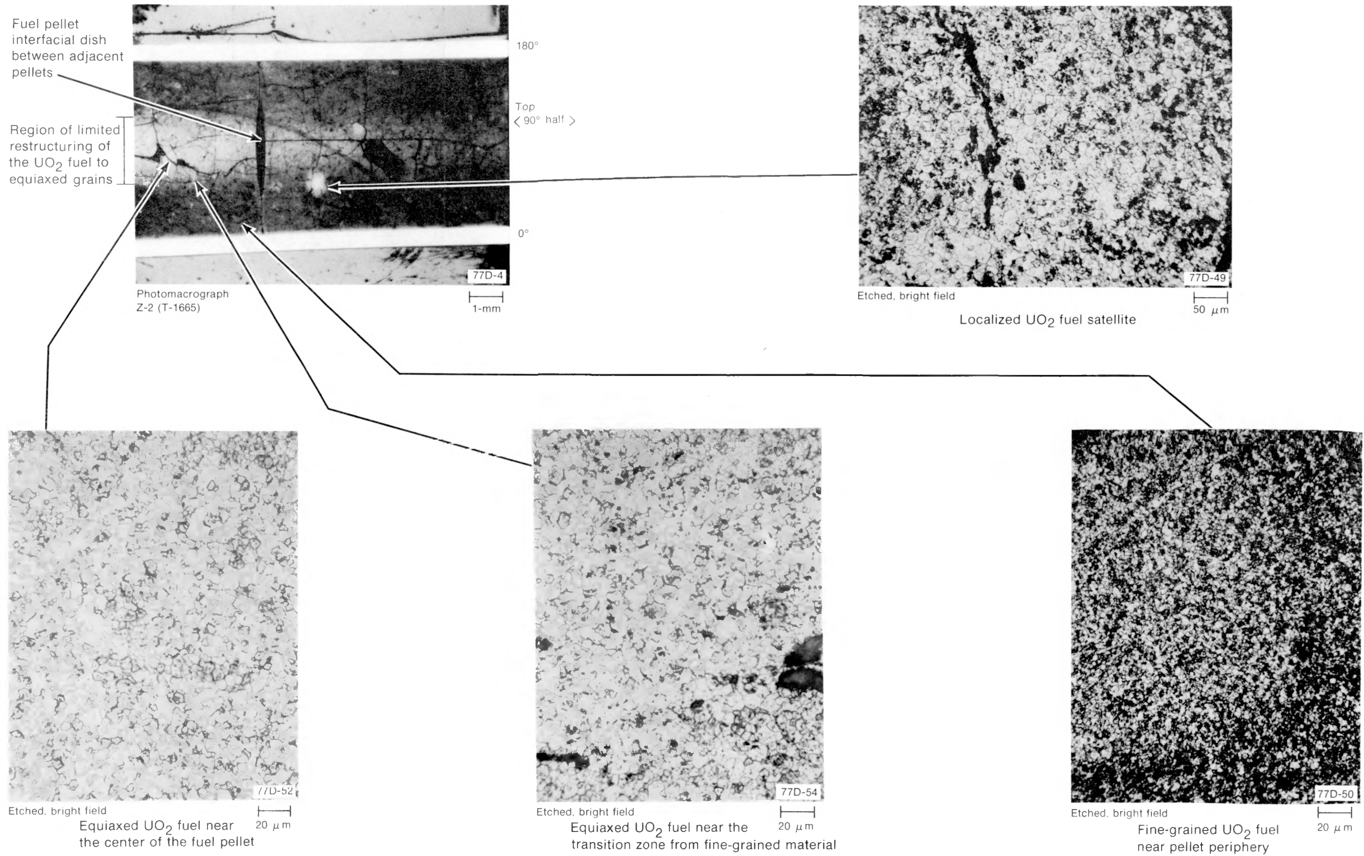
Fig. D-39 Longitudinal section (Z-2) of Rod A-0017 showing fuel restructuring.
