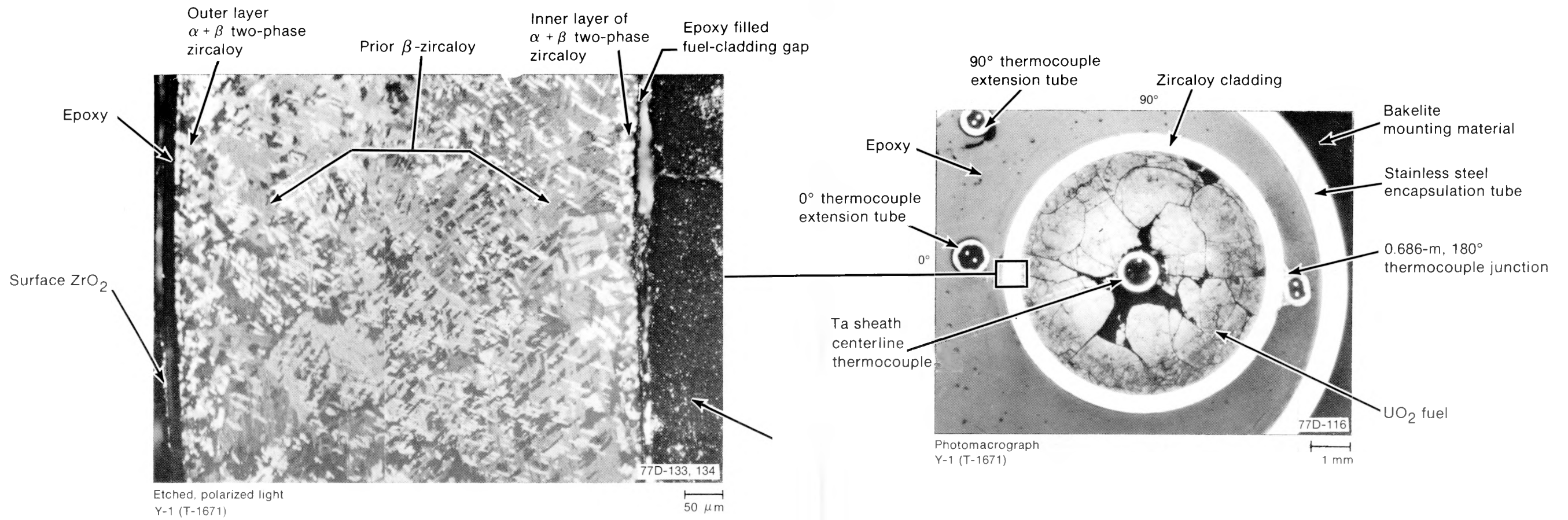
Fig. D-1 Transverse section (Y-1) of Rod UTA-0014 at 0.686 m.
