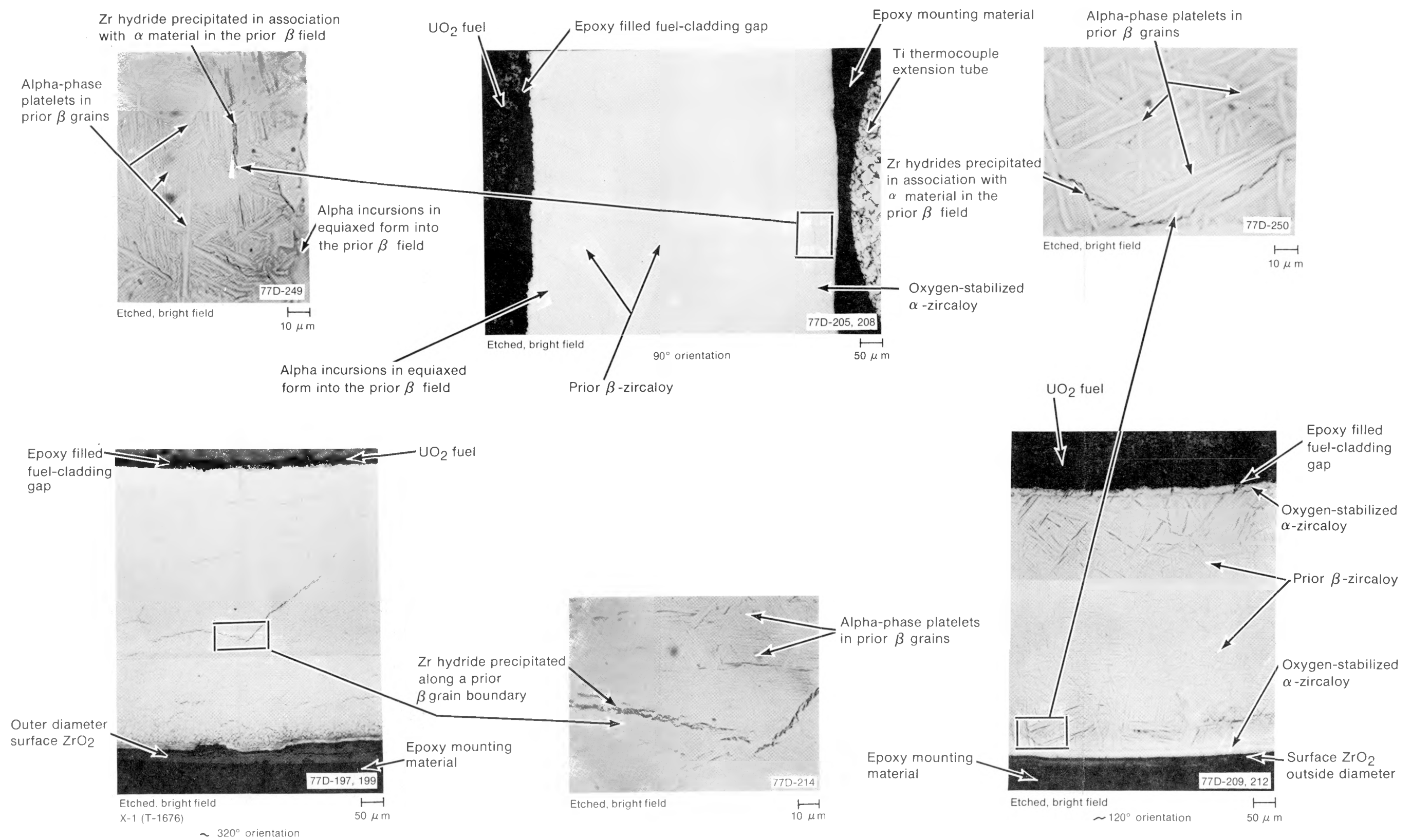
Fig. D-12 Transverse section (X-1) of Rod UTA-0015 showing cladding hydriding.
