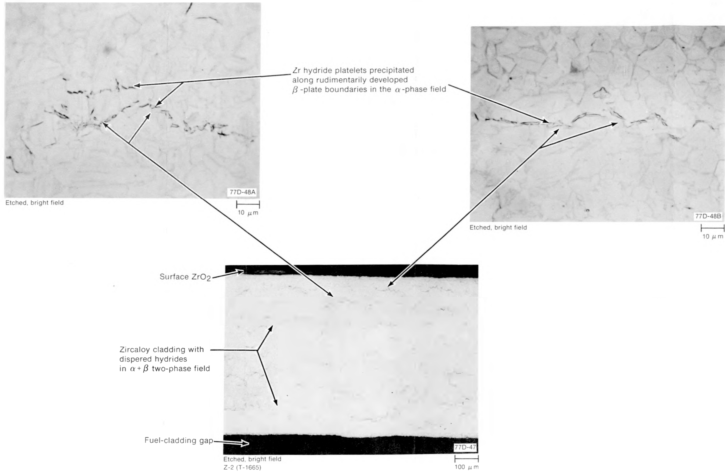
Fig. D-59 Hydride precipitation in the alpha + beta two-phase field at 0.768 m in Sample Z-2 of Rod A-0017.
