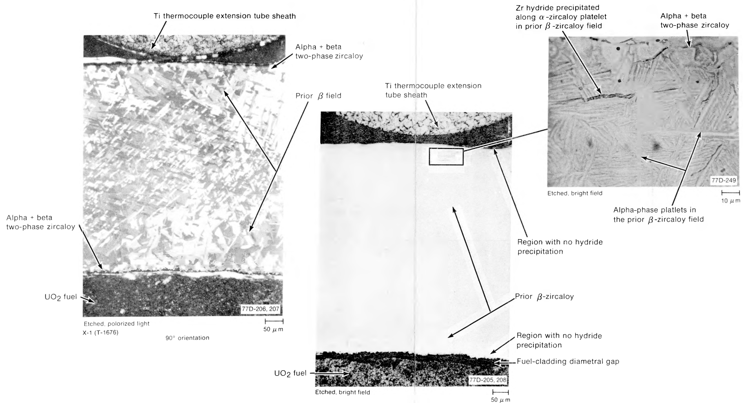
Fig. D-54 Hydride precipitation at 0.686-m and 90° circumferential orientation in Sample X-1 of Rod UTA-0015.
