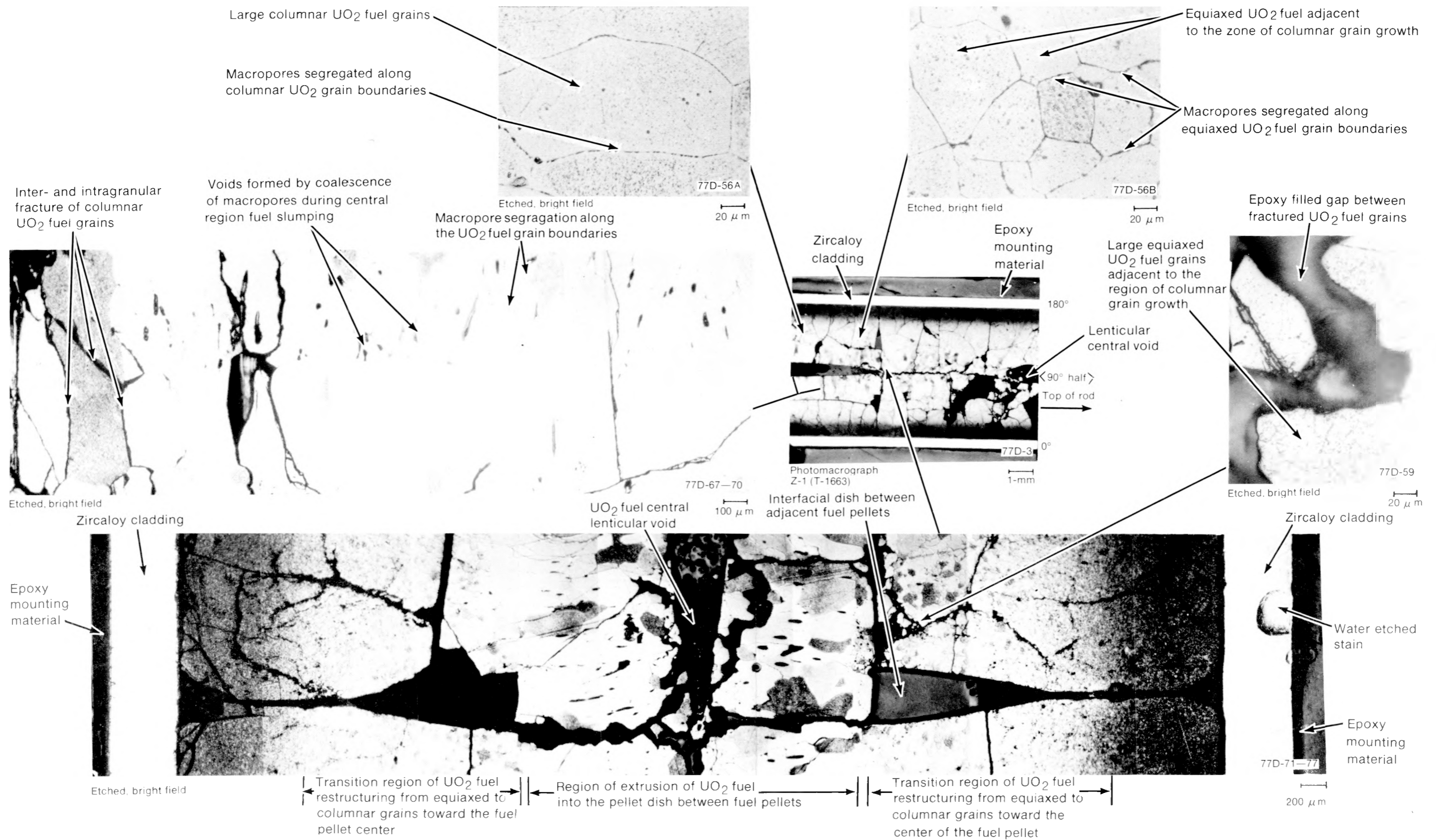
Fig. D-36 Longitudinal section (Z-1) of Rod A-0017 showing fuel restructuring and fuel melting zone.
