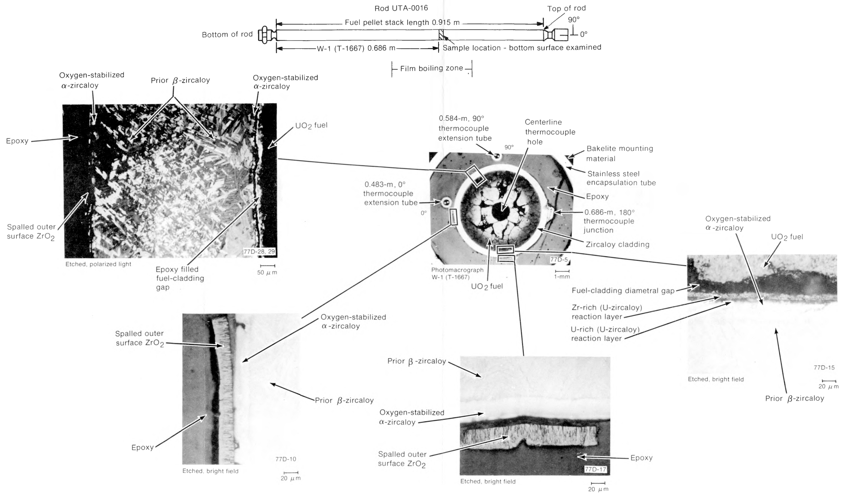
Fig. D-26 Transverse section (W-1) of Rod UTA-0016 (0.686 m) showing cladding microstructure.
