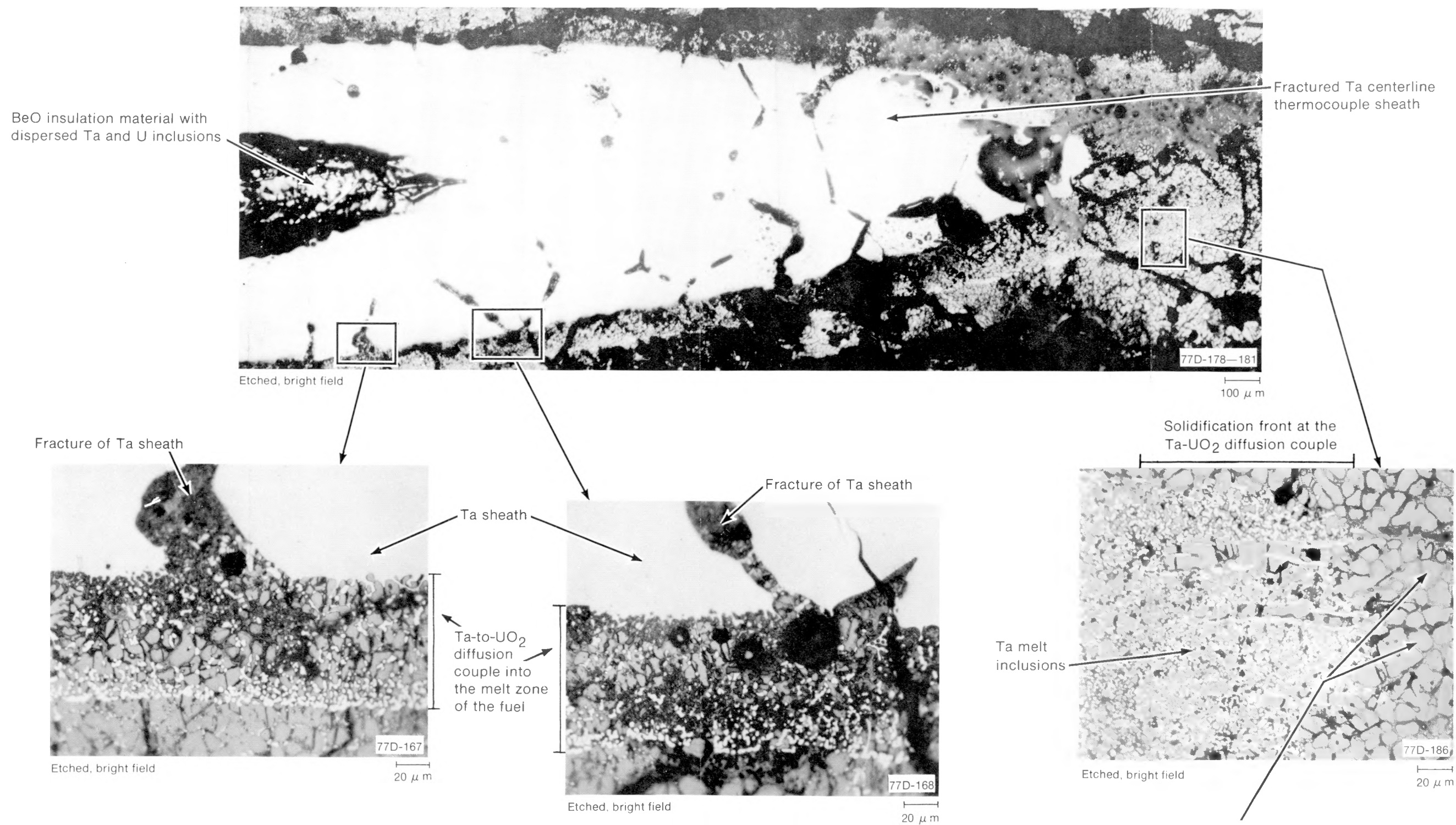
Fig. D-9 Longitudinal section (Y-4) of Rod UTA-0014 showing fuel and tantalum thermocouple sheath melt zone diffusion couple.
