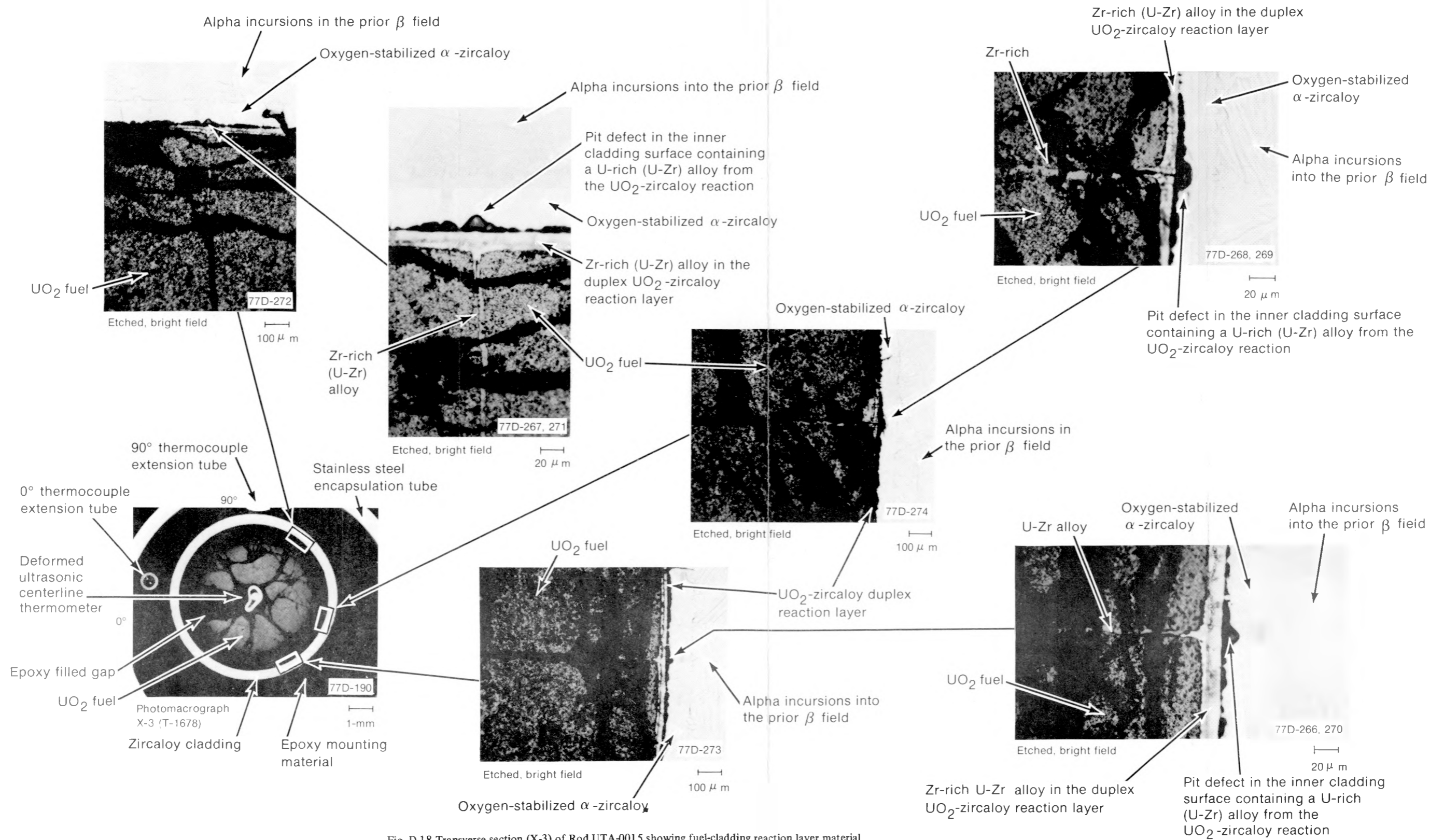
Fig. D-18 Transverse section (X-3) of Rod UTA-0015 showing fuel-cladding reaction layer material.
