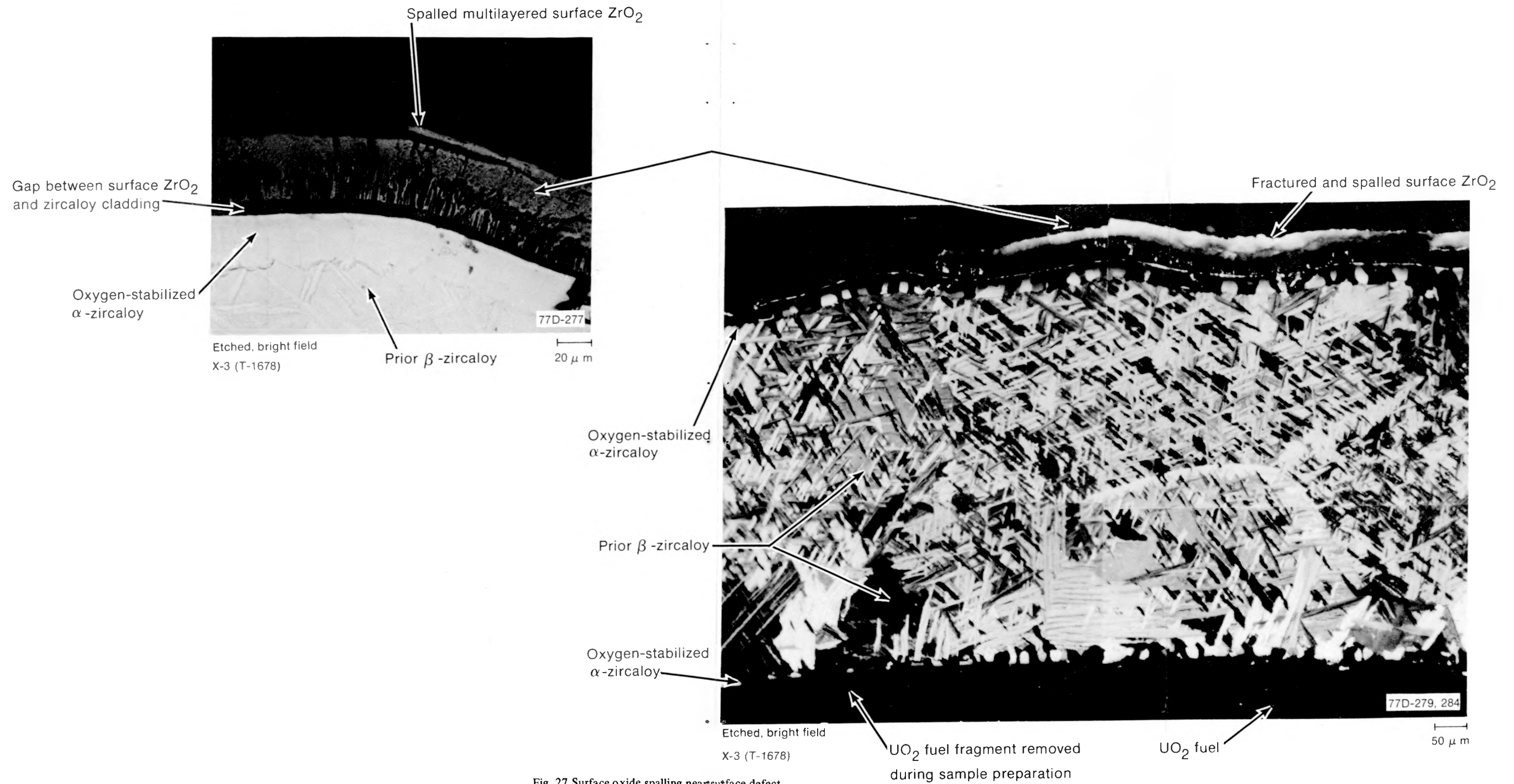
Fig. 27 Surface oxide spalling near surface defect.
