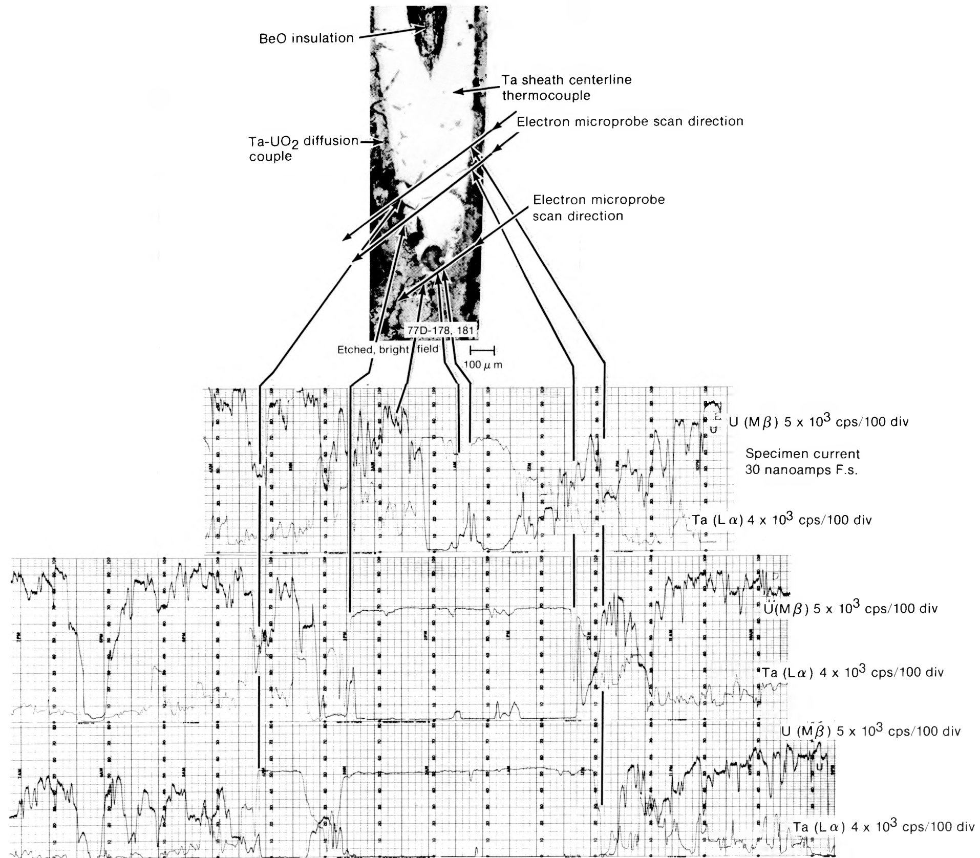
Fig. D-50 Electron microprobe scan across the tantalum thermocouple sheath and the tantalum-UO 2 diffusion couple of Rod UTA-0014.
