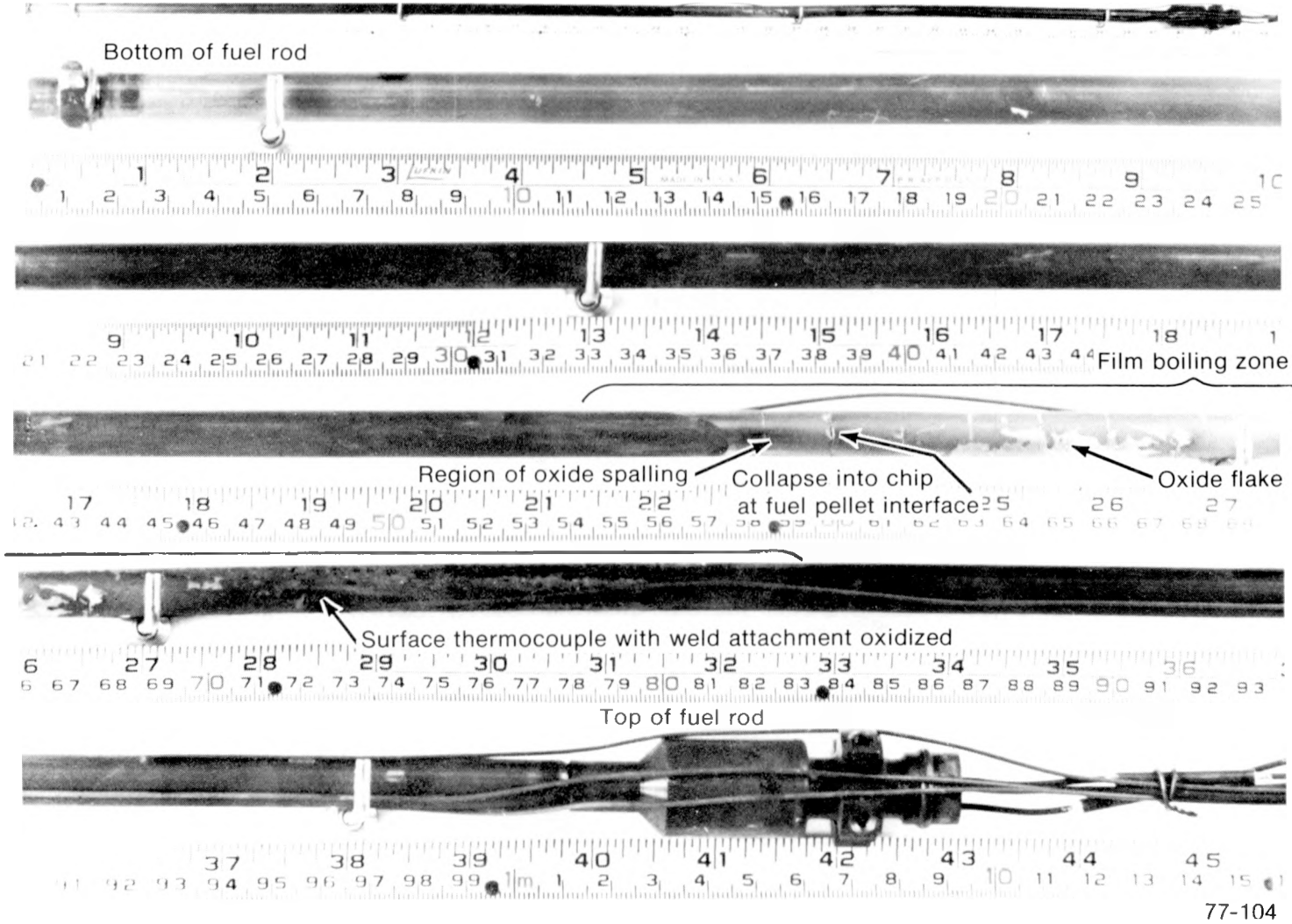
Fig. 4 Rod UTA-0015, showing the posttest condition at the 180° orientation.
