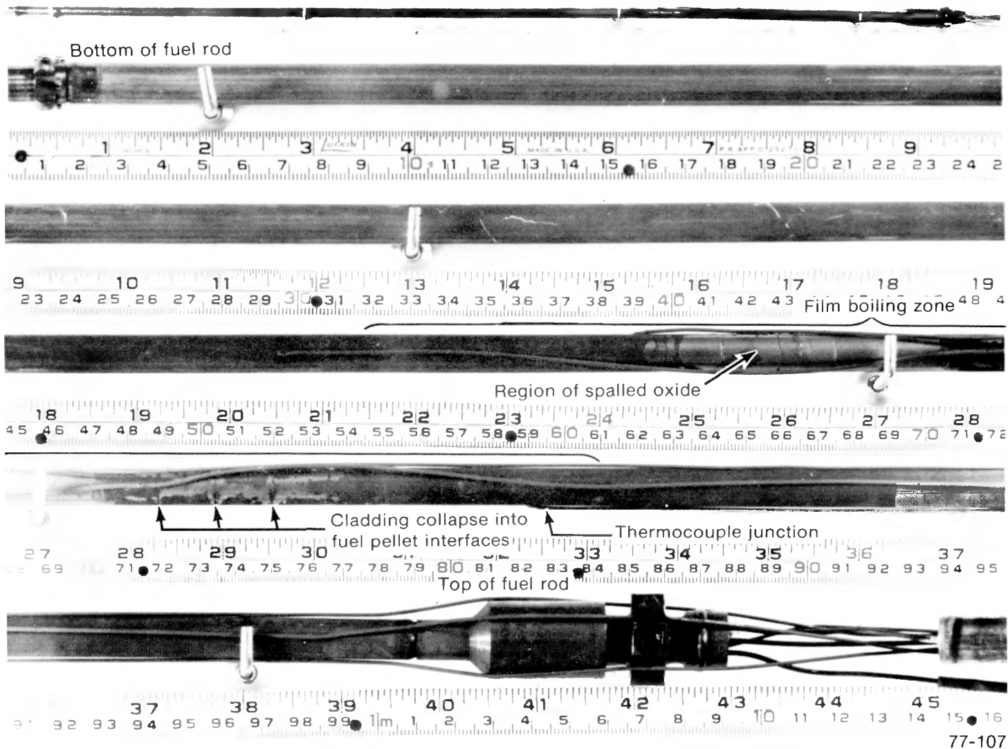
Fig. 1 Rod UTA-0014, showing the posttest condition at the 0° orientation.
