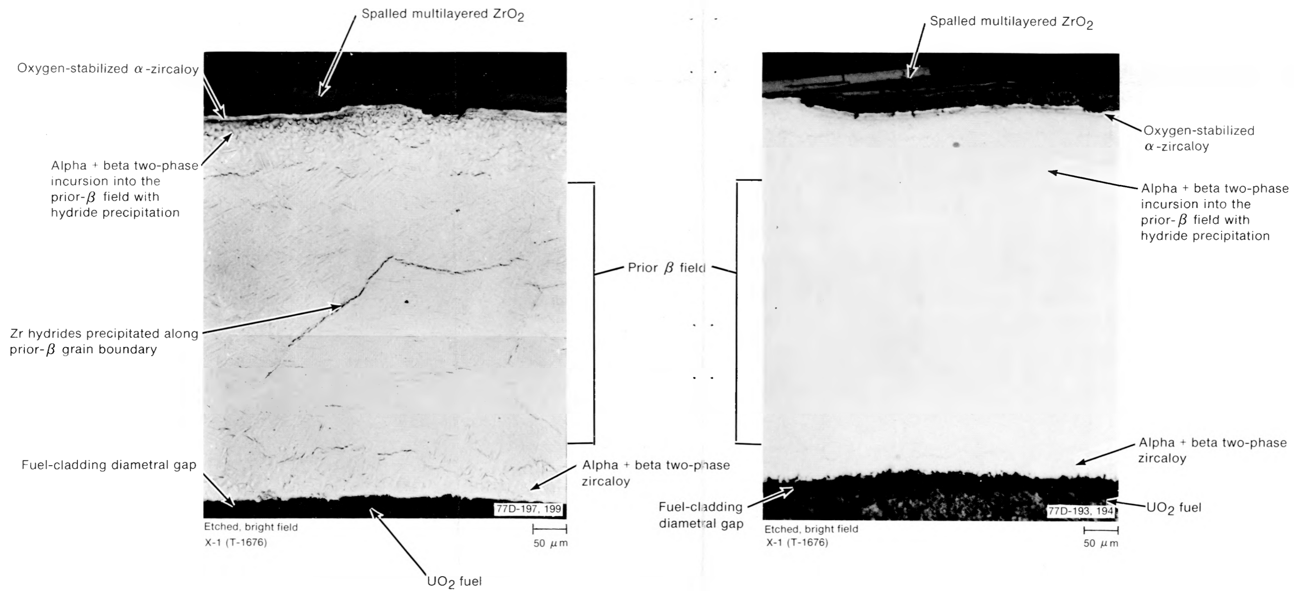
Fig. 28 Spalling of multilayered surface oxide.
