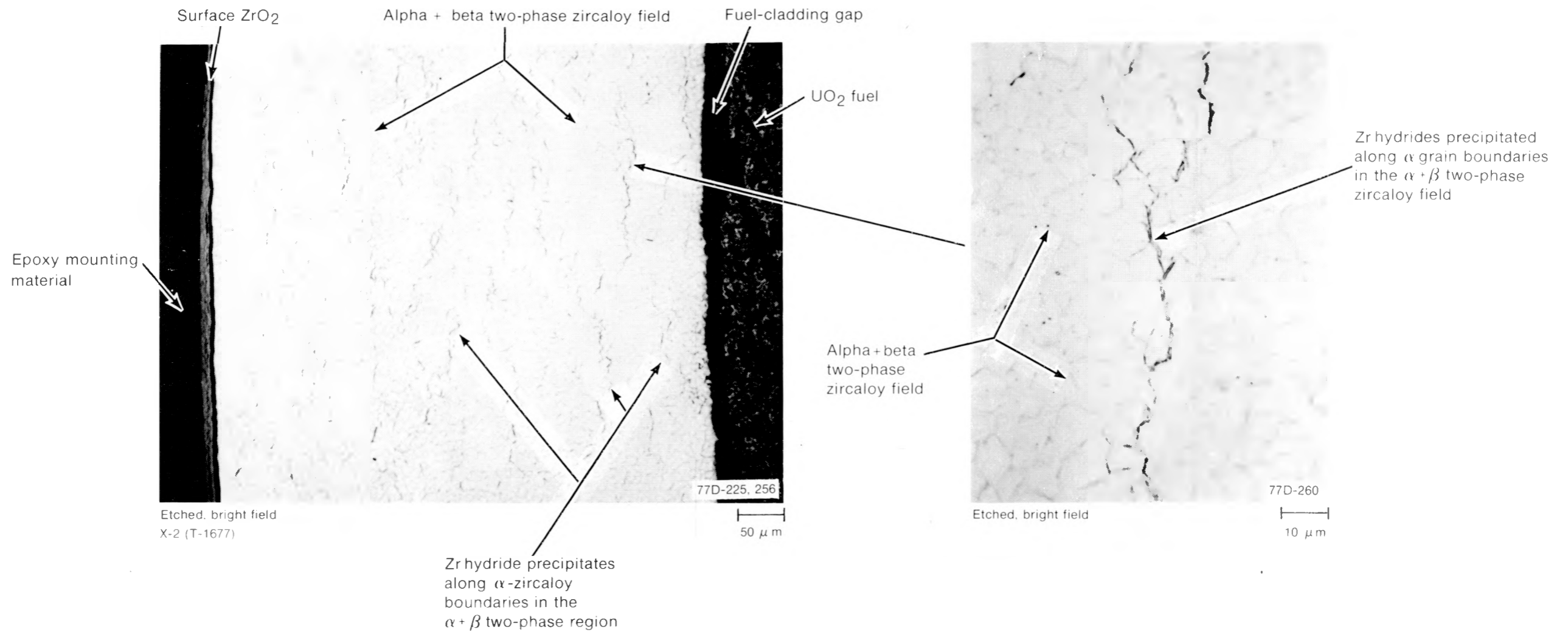
Fig. D-15 Transverse section (X-2) of Rod UTA-0015 showing cladding hydriding.
