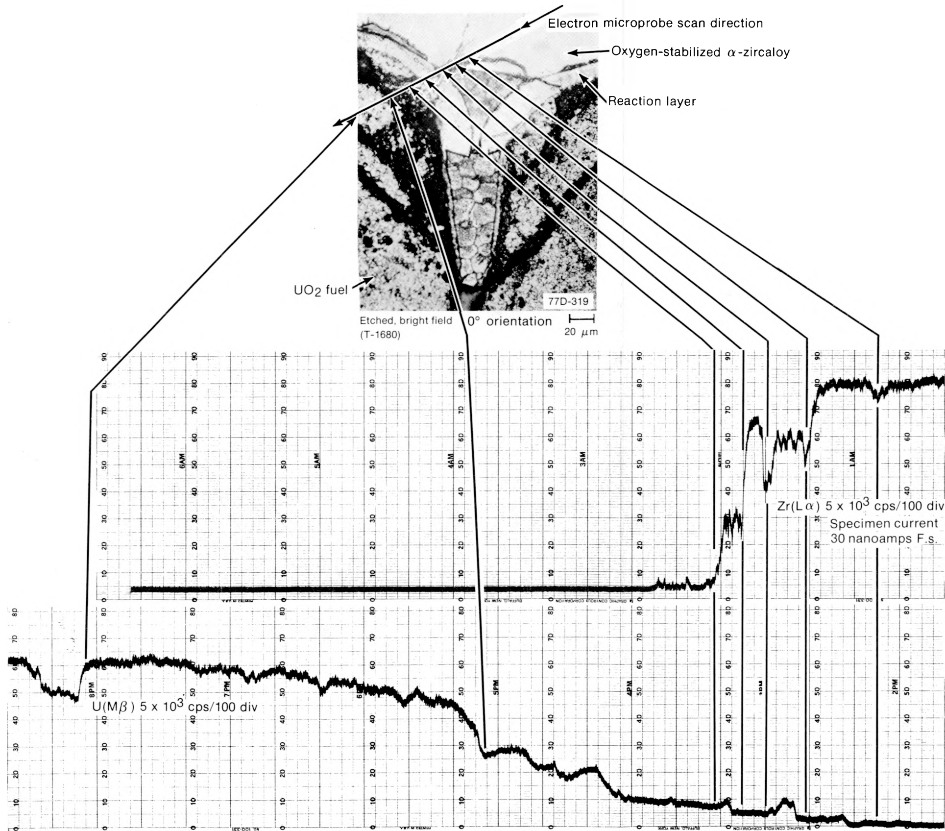
Fig. D-41 Electron microprobe scan of the fuel and cladding near a fuel pellet gap in Rod UTA-0015.
