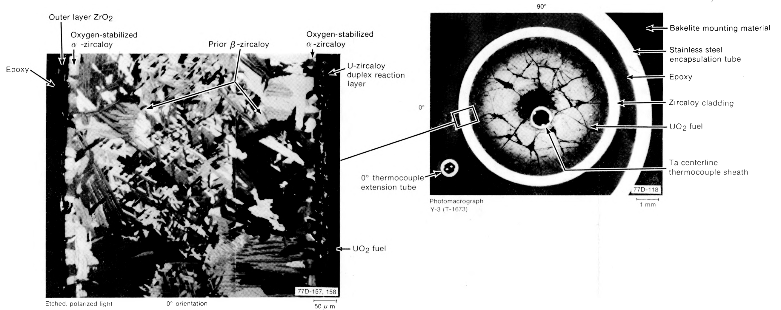
Fig. D-5 Transverse section (Y-3) of Rod UTA-0014 (0.638 m) showing cladding microstructure.
