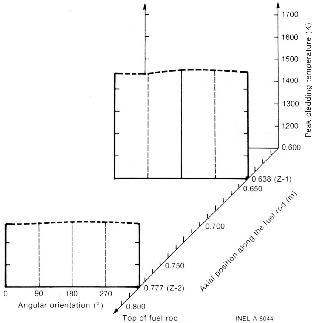
Fig. 16 Isometric plot of the modified BUILD5 peak cladding temperature as a function of angular orientation and axial position for Rod A-0017.
