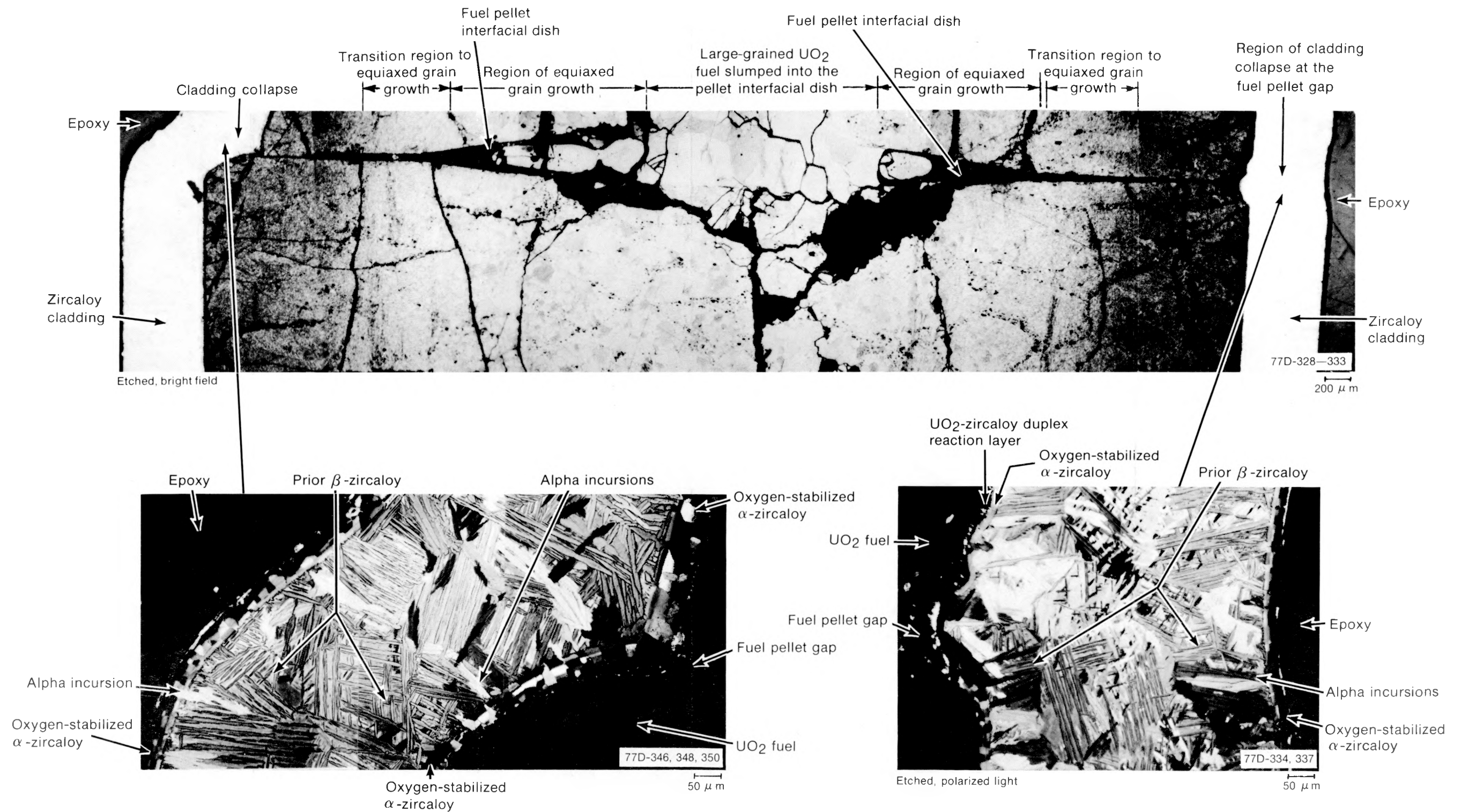
Fig. D-24 Longitudinal section (X-5) of Rod UTA-0015 showing cladding collapse and fuel restructuring.
