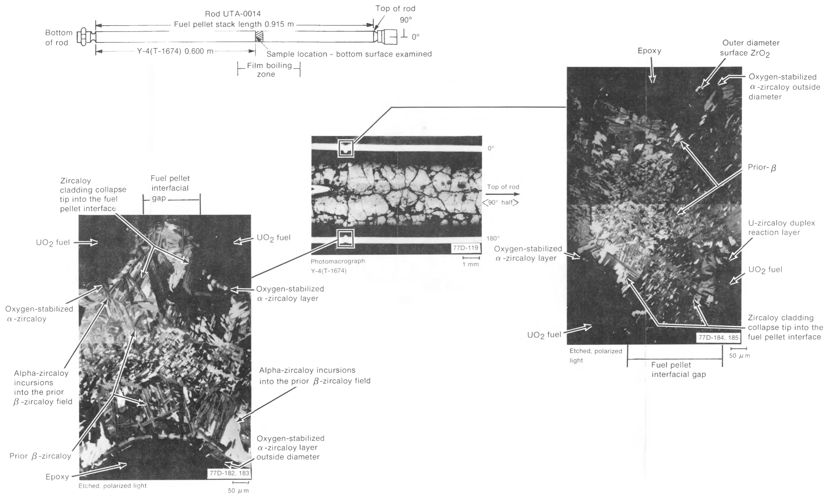
Fig. D-7 Longitudinal section (Y-4) of Rod UTA-0014 (between 0.600 and 0.619 m) showing cladding waisting.
