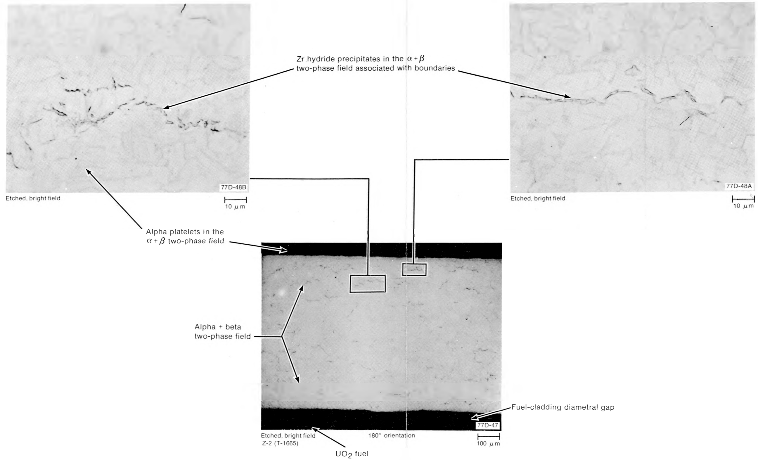
Fig. D-38 Longitudinal section (Z-2) of Rod A-0017 showing cladding hydriding.
