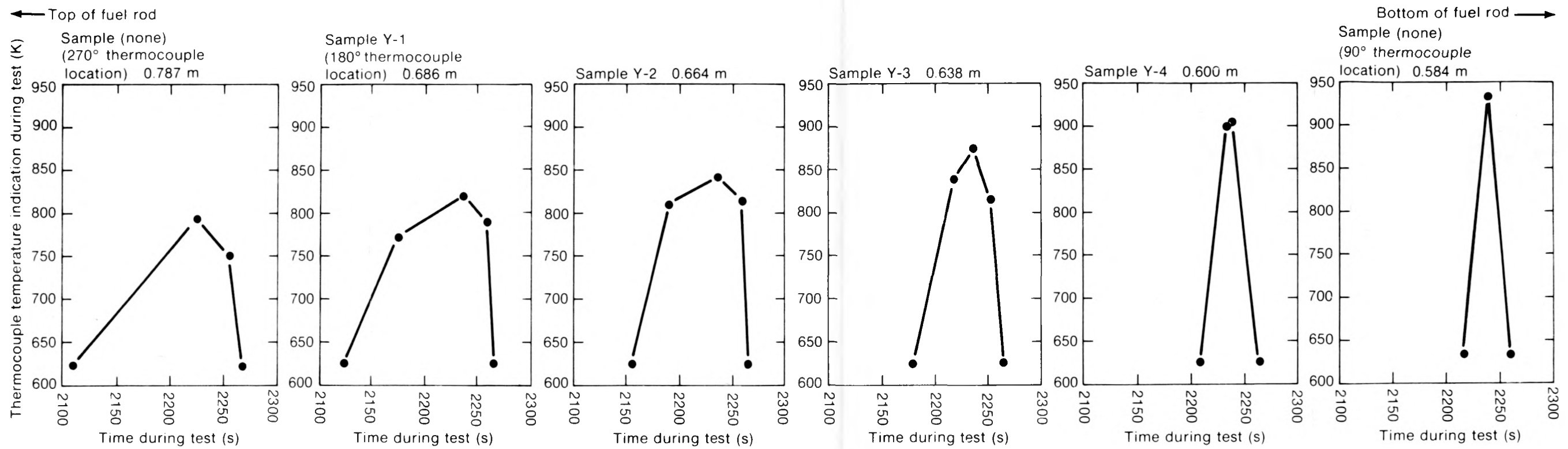
Fig. F-5 Linearized time-temperature profile computer code input for Rod UTA-0014.
