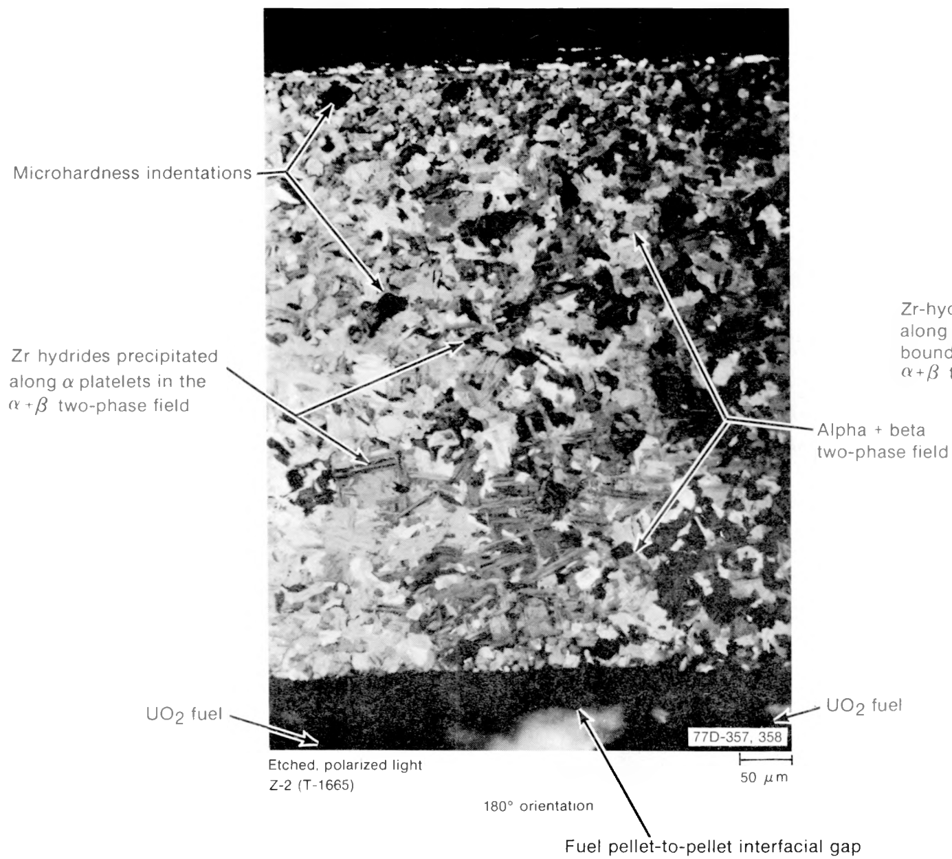
Fig. D-60 Hydriding in the alpha + beta two-phase field in Sample Z-2 of Rod A-0017.
