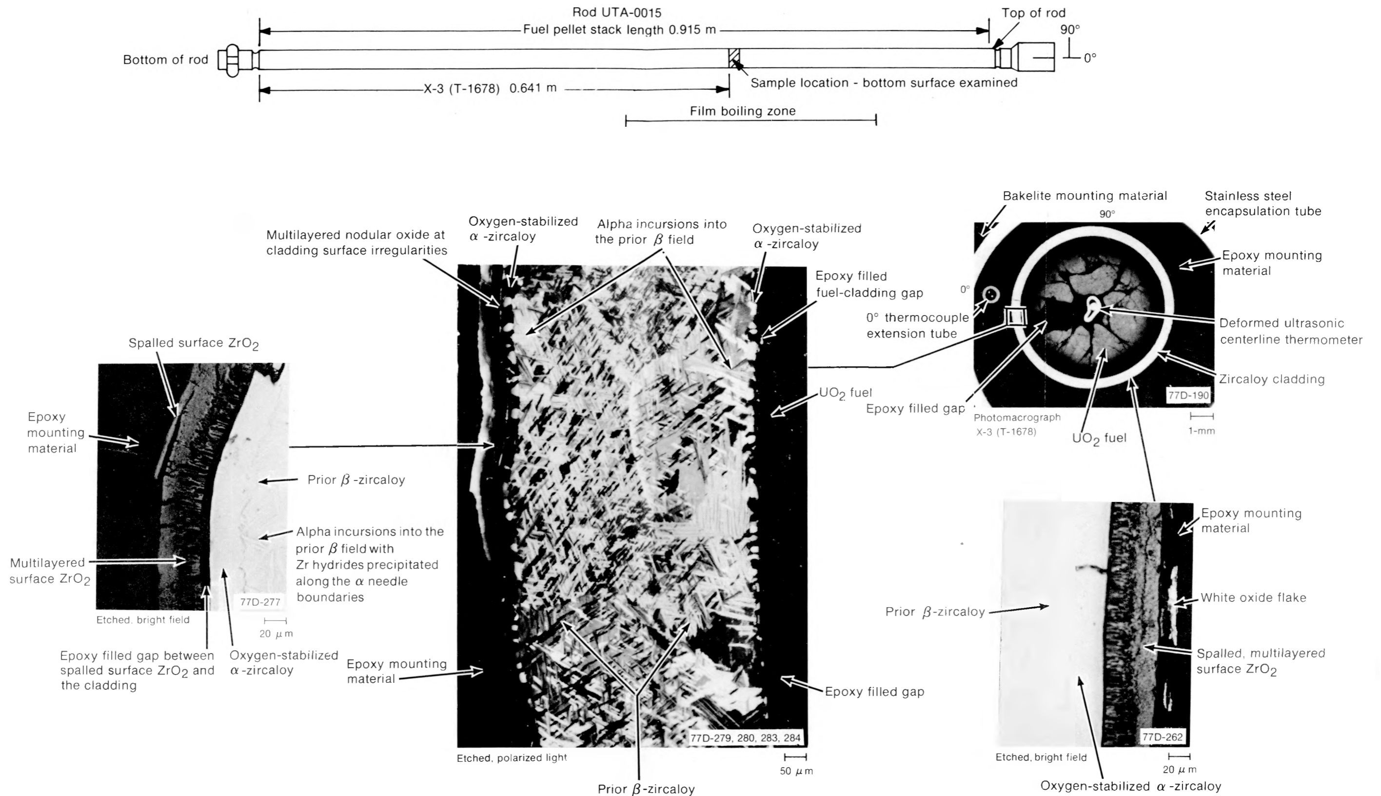
Fig. D-17 Transverse section (X-3) of Rod UTA-0015 showing cladding microstructure.
