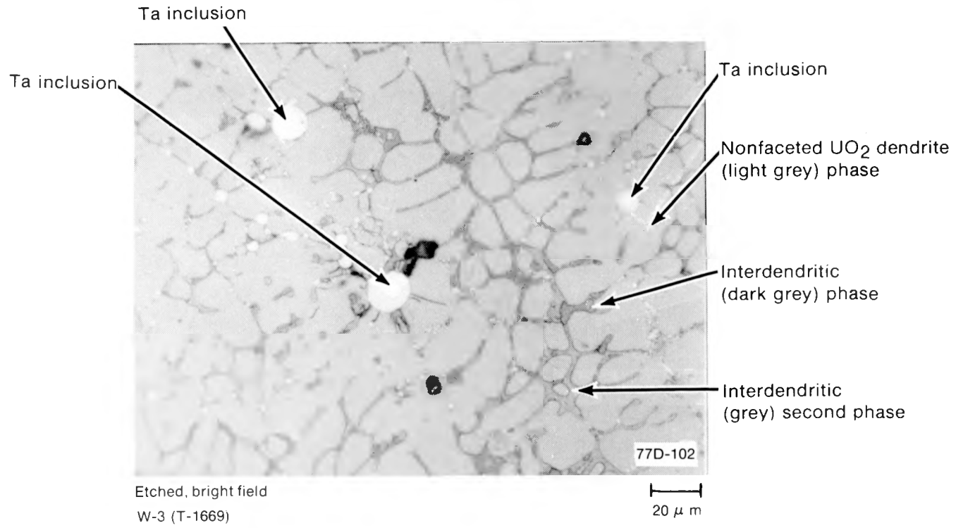
Fig. 38 Nonfaceted UO_2 dendrites with interdentritic tantalum inclusions in the tantalum UO_2 melt zone.
