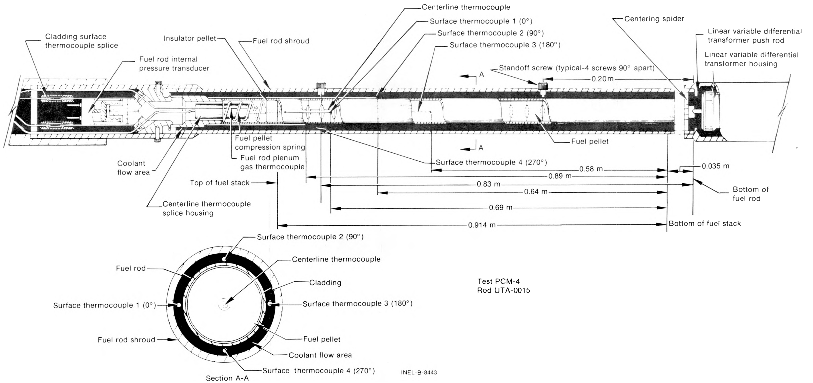
Fig. A-2 Test PCM-4 fuel rod and instrumentation shown installed in the flow shroud.
