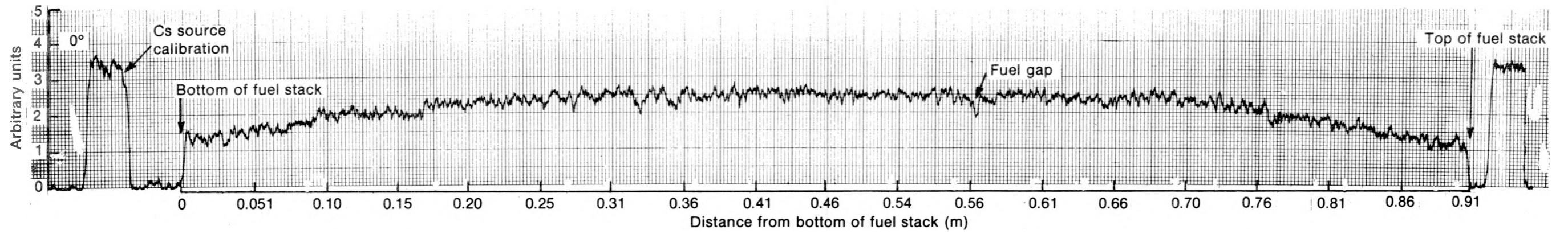
Fig. A-5 Gross gamma scan of Rod A-0017 at 0° orientation.
