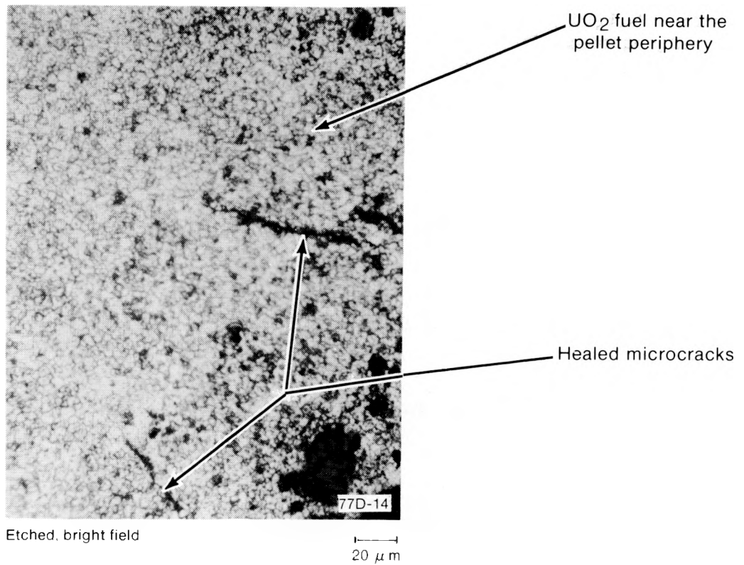
Fig. D-27 Transverse section (W-1) of Rod UTA-0016 showing fuel restructuring.
