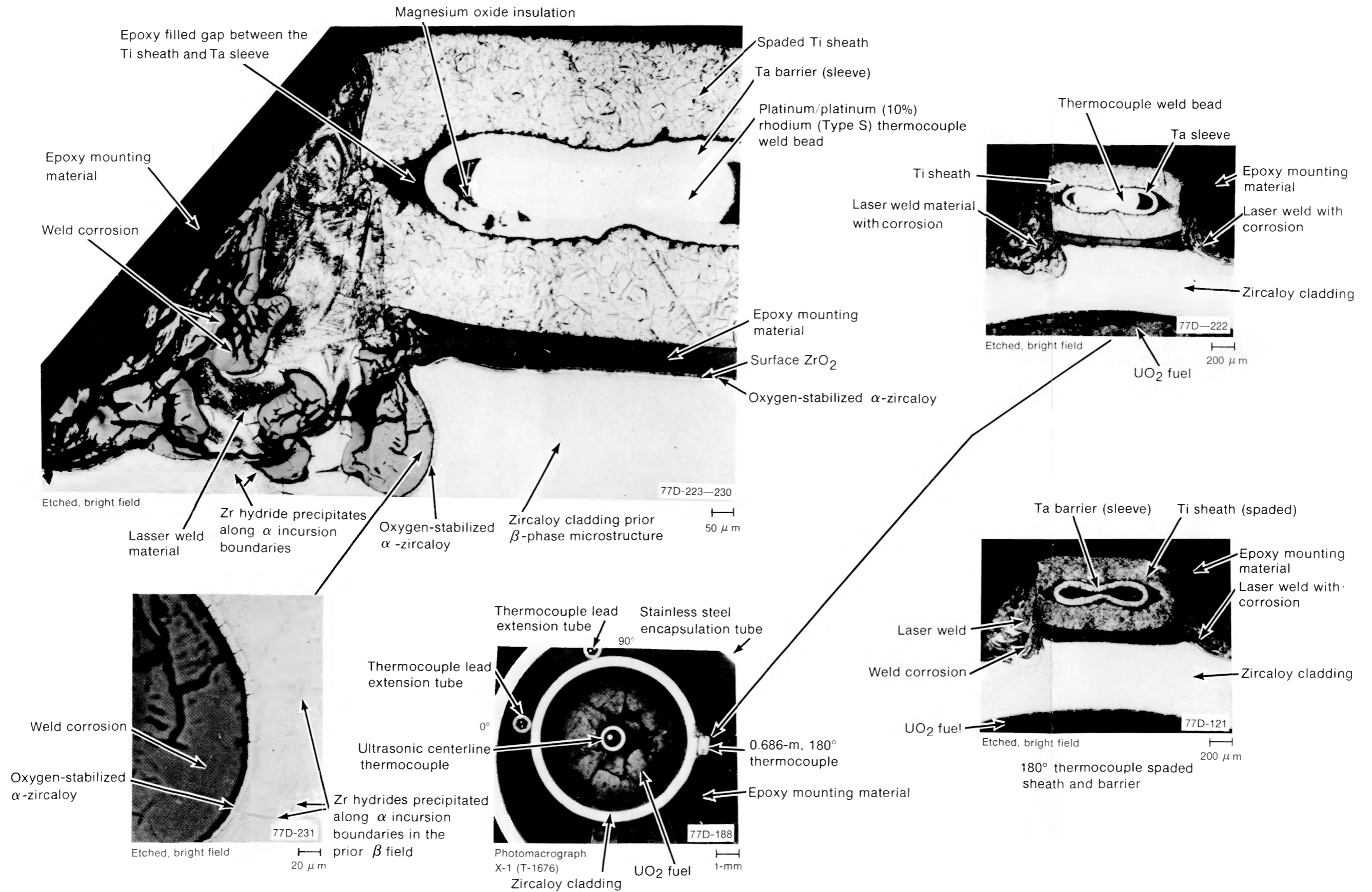
Fig. E-2 Cladding surface thermocouple junction at the 0.686-m, 180° position on Rod UTA-0015.
