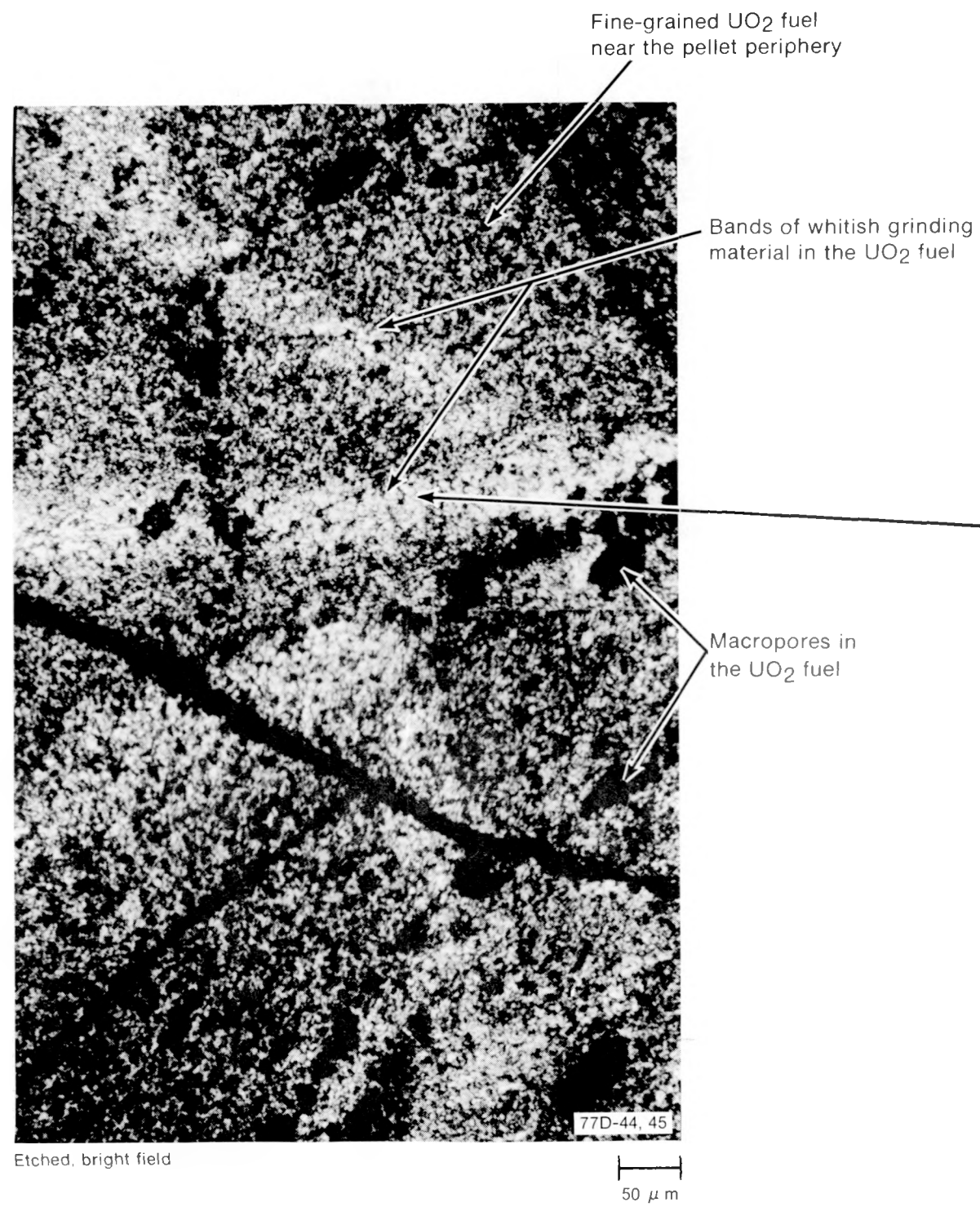
Fig. D-40 Longitudinal section (Z-2) of Rod A-0017 showing grinding compound inclusions in the UO_2 fuel.
