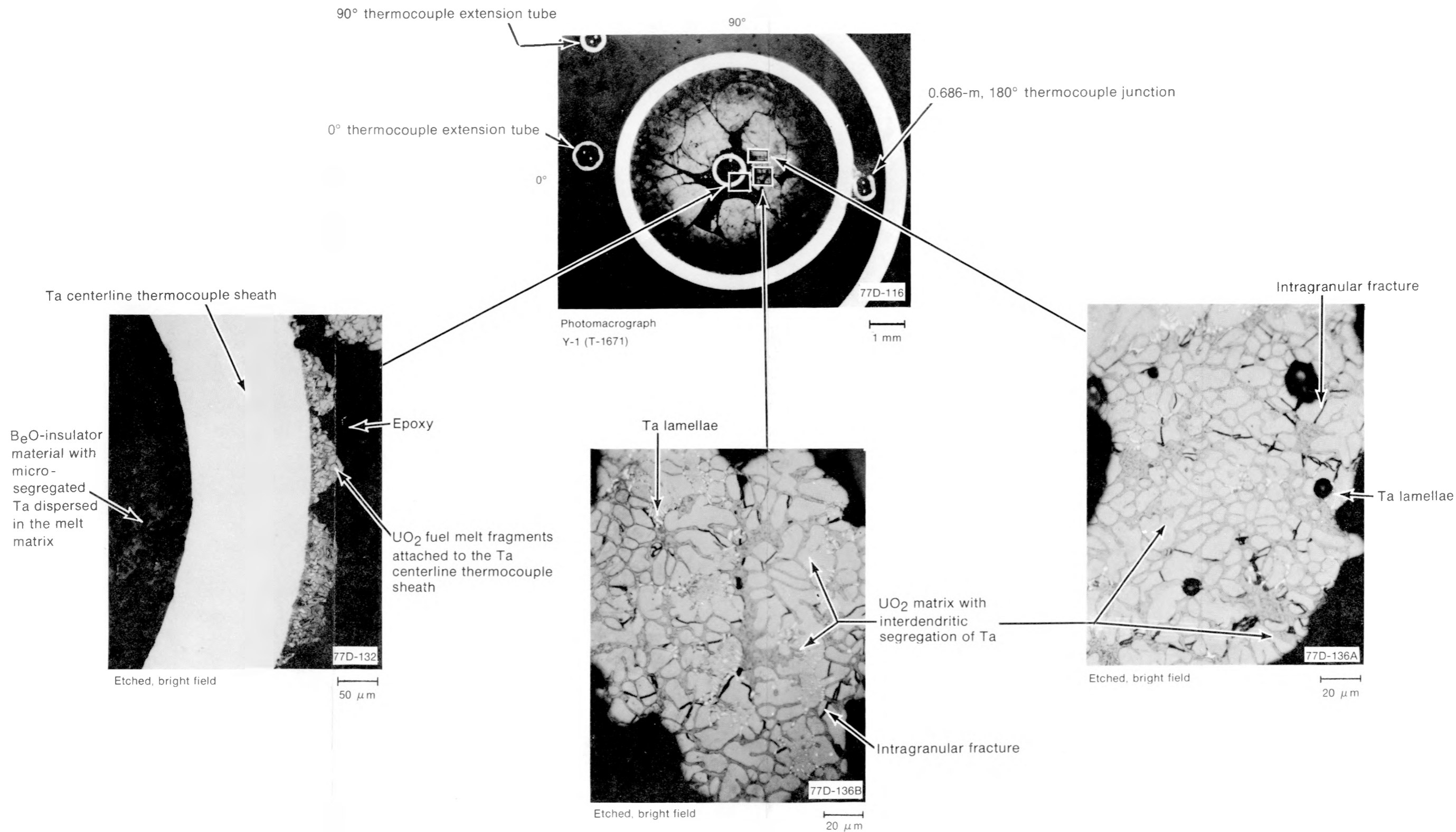
Fig. D-2 Transverse section (Y-1) of Rod UTA-0014 molten zone.
