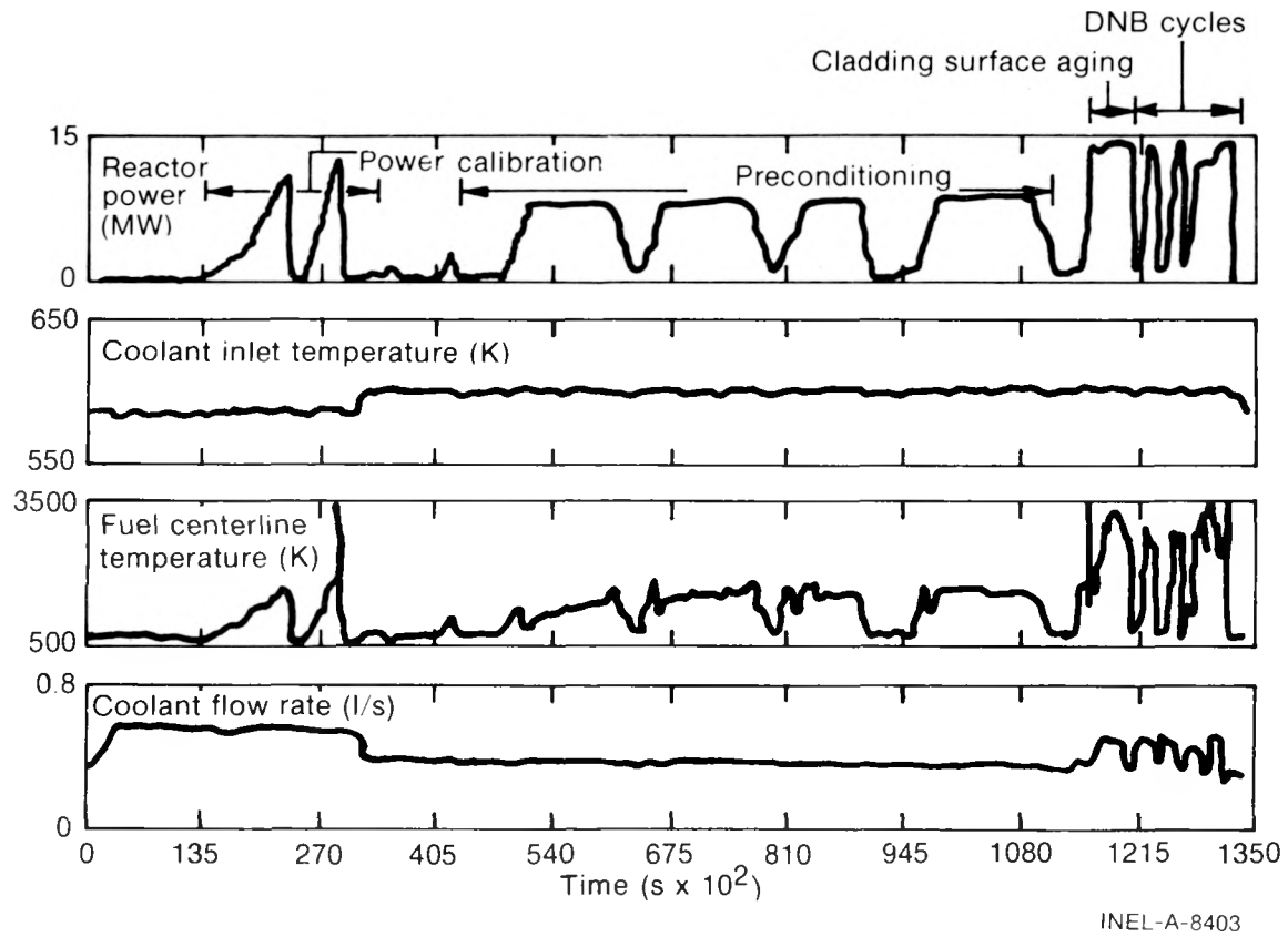
Fig. A-4 Composite plot of Test PCM-4 experimental conduct as a function of time during testing.
