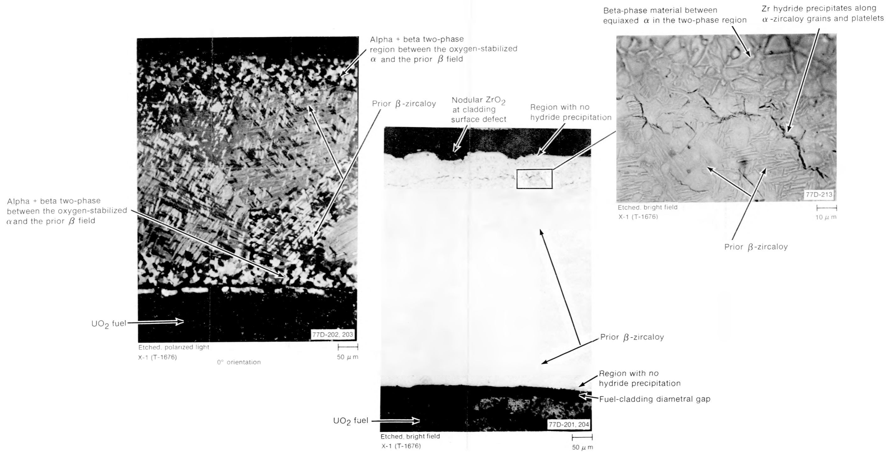
Fig D-52 Hydride precipitation at 0.686-m and 0° circumferential orientation in Sample X-1 of Rod UTA-0015.
