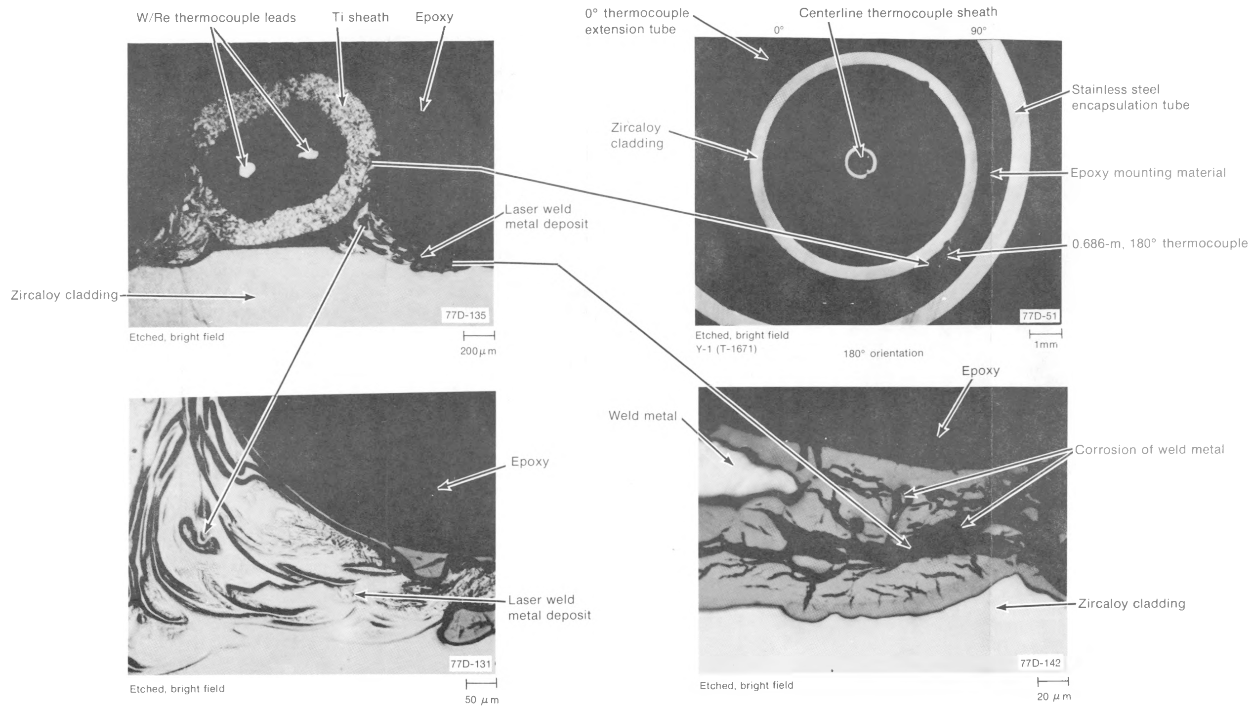
Fig. E-1 View of the 0.686-m, 180° thermocouple junction from Rod UTA-0014.
