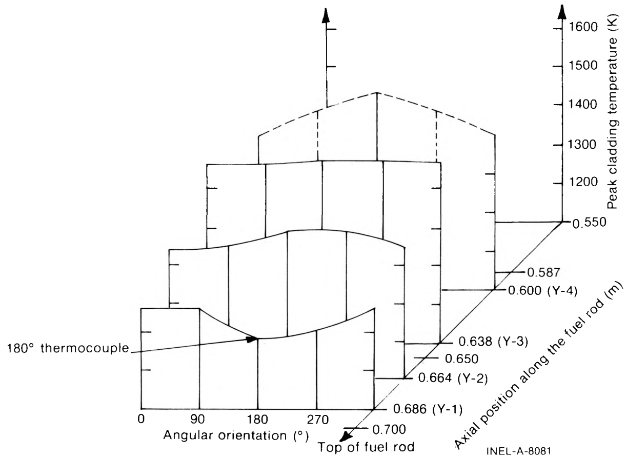
Fig. 13 Isometric plot of the modified BUILD5 peak cladding temperature as a function of angular orientation and axial position for Rod UTA-0014.
