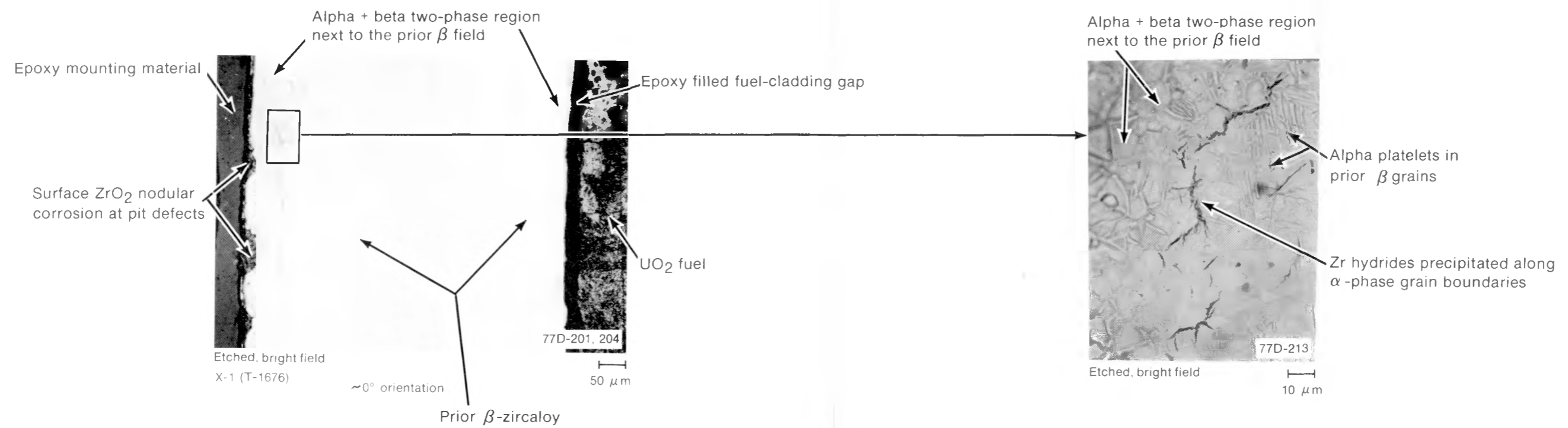
Fig. D-11 Transverse section (X-1) of Rod UTA-0015 showing cladding hydriding.
