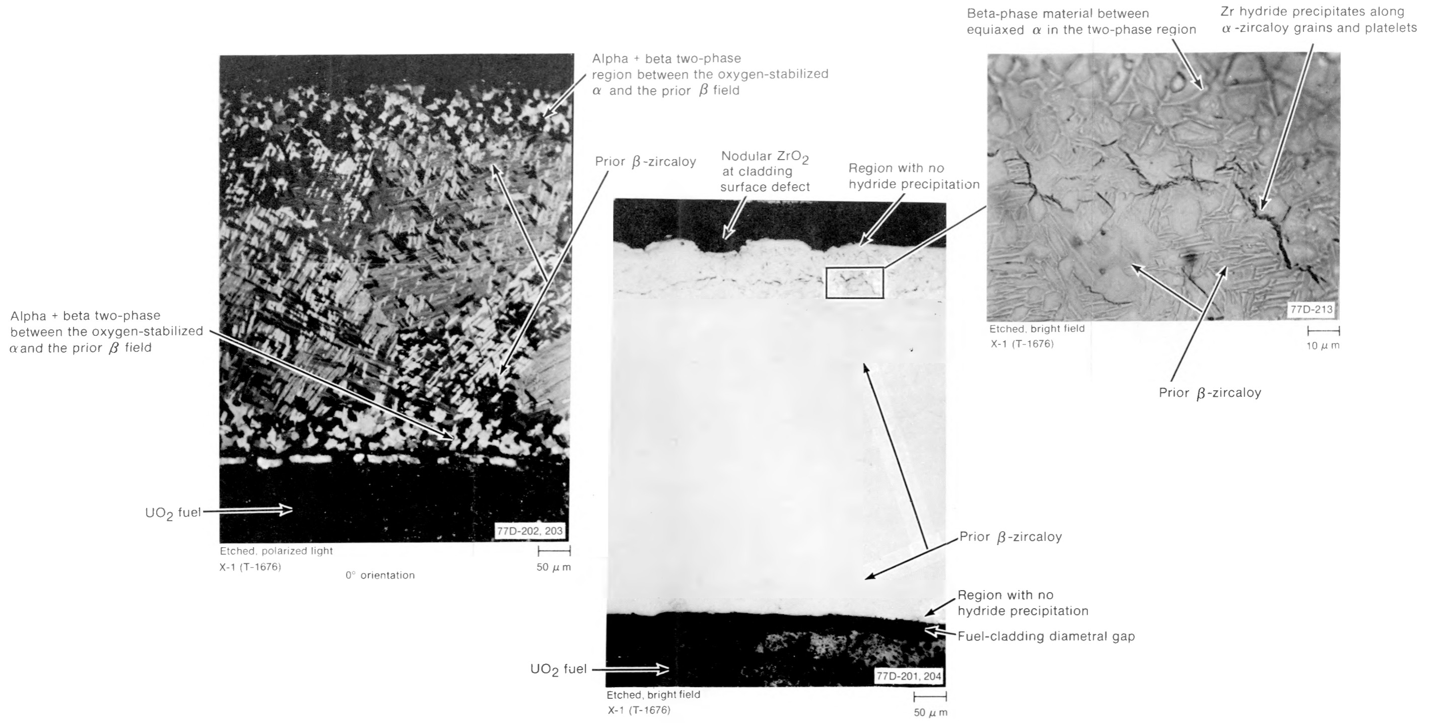
Fig. 35 Hydride precipitation at 0.686-m and 0° circumferential orientation in Rod UTA-0015.
