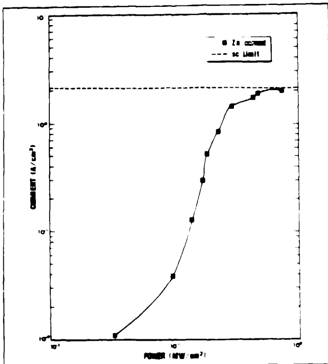
Fig. 4. Variance in the current density ( \text{A/cm}^2 ) as a function of incident laser power ( \text{MW/cm}^2 ).
