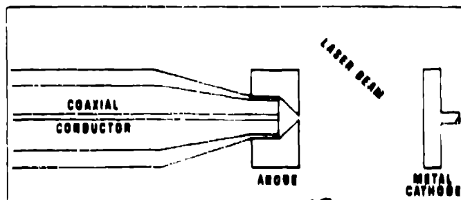
Fig. 2. Anode-cathode arrangement.
