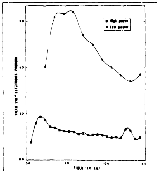
Fig. 1. Quantum efficiency vs electric field.
