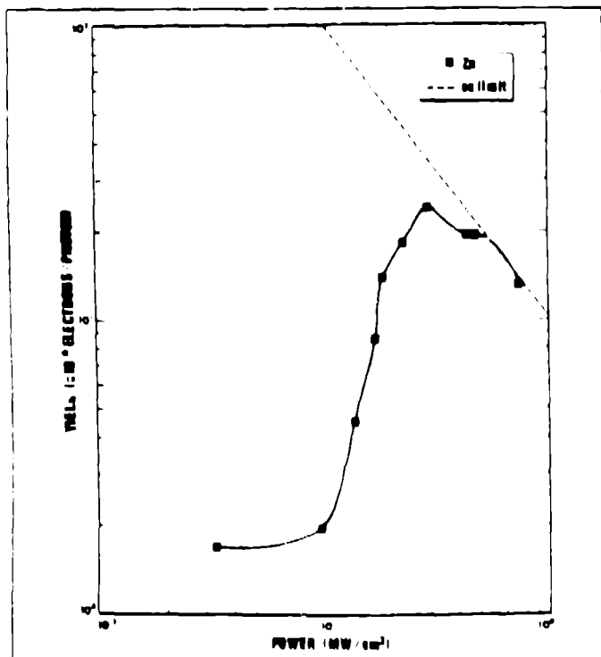
Fig. 5. Quantum yield (electrons/photon) vs light intensity ( \text{MW/cm}^2 ).
