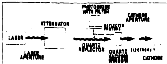
Fig. 1. Light path components.
