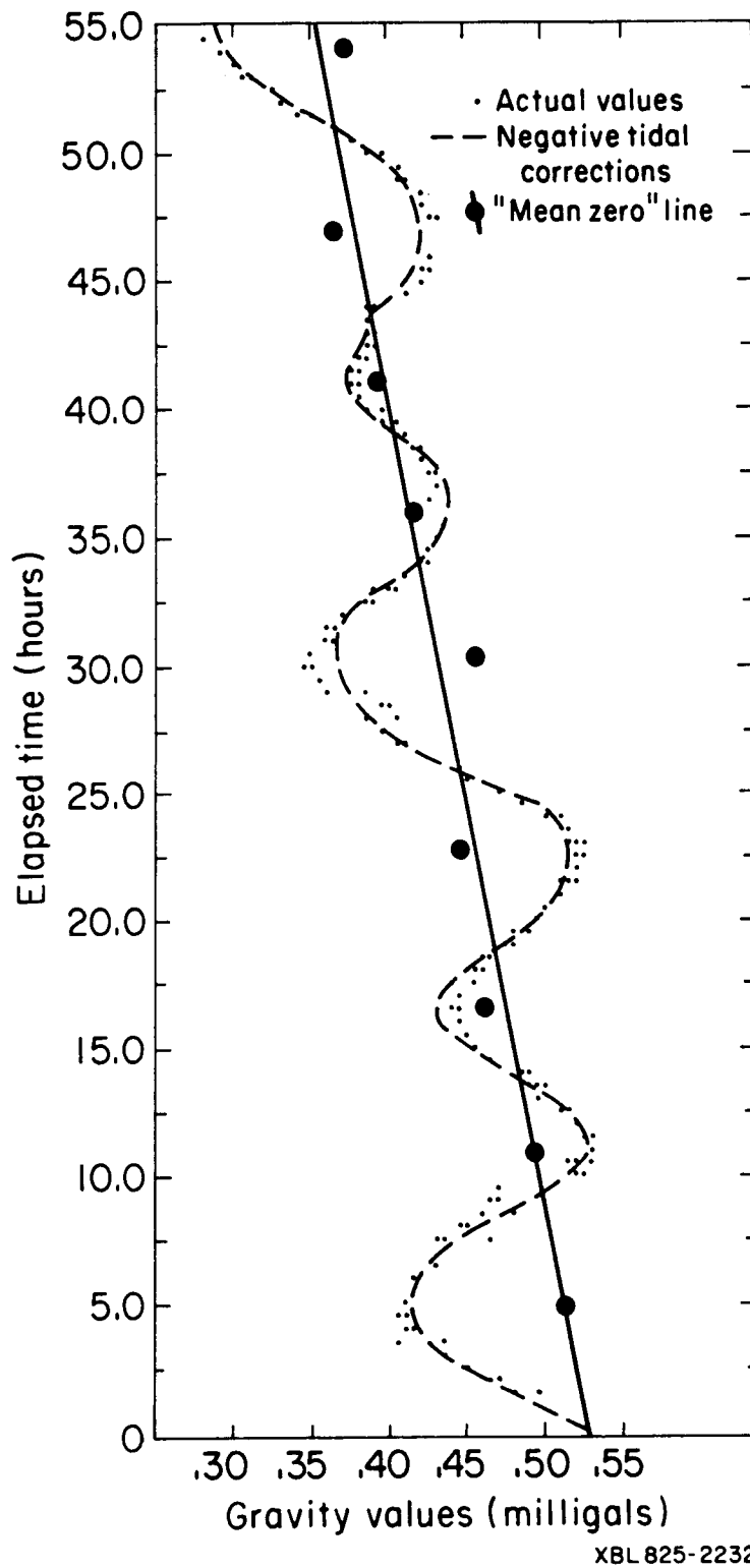
Figure 3. Graphs of tidal monitoring values and tidal corrections. The negative tidal corrections were superimposed on the actual gravity values after construction of the "mean zero" line, a line of zero corrections which is slanted because of drift in the strip chart recorder used for monitoring.
