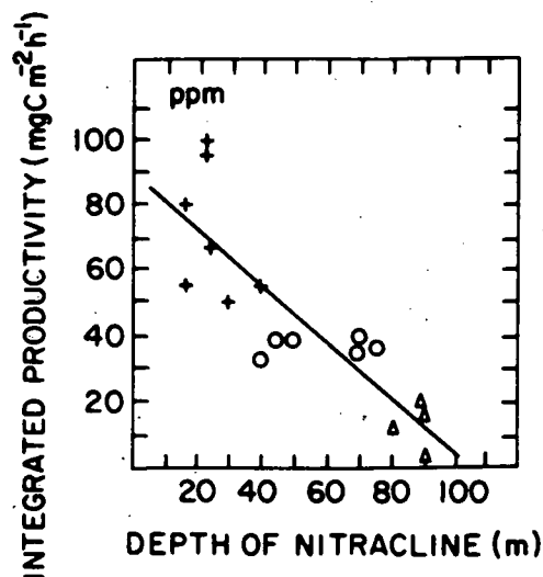
B. Linear regression between the depth of the nitracline and the integrated value of primary production in the water column.
